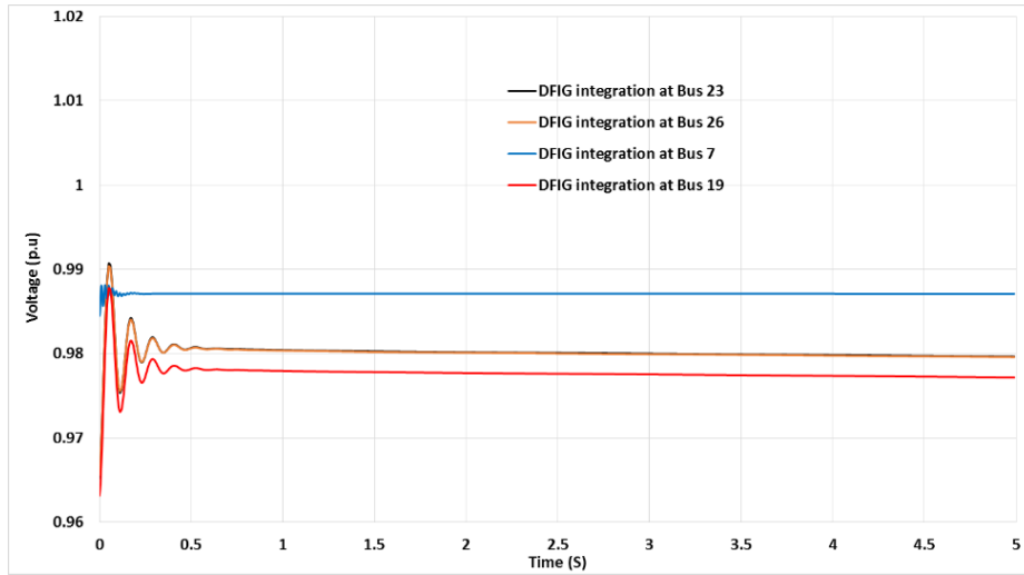
Figure 7-10: Voltage profiles at the PCC after DFIG-integration at selected buses in 33-bus network in the absence of fault in the network (Case 2)
