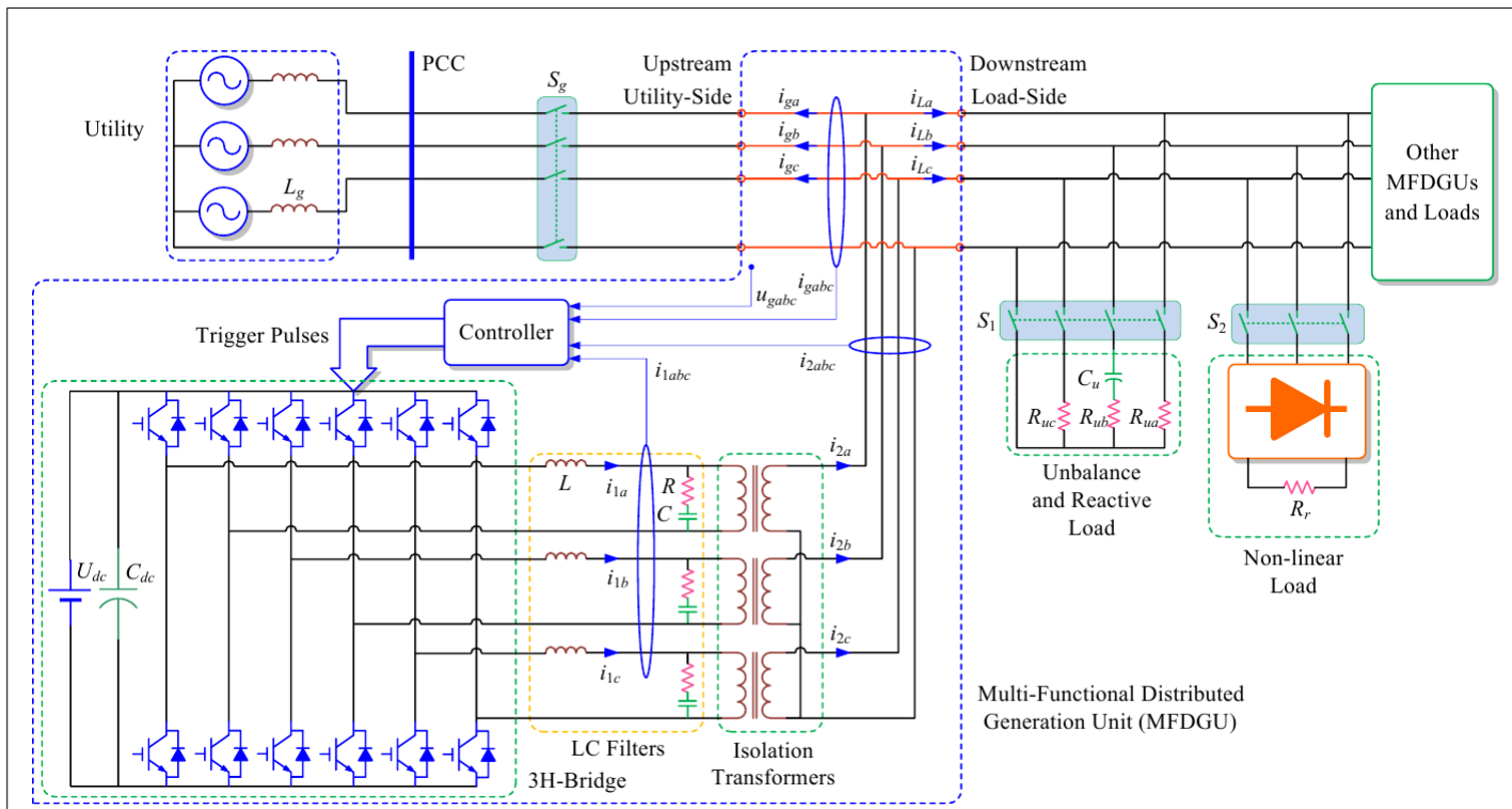
Figure 2-8: The configuration of the MFDGU topology used to enhance the PQ of grid integrated DG [41]
