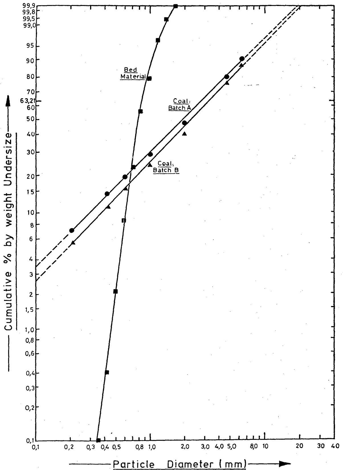
Figure C2 : Size Gradings of the Coal and Bed Material Plotted on Rosin-Rammler Paper.
