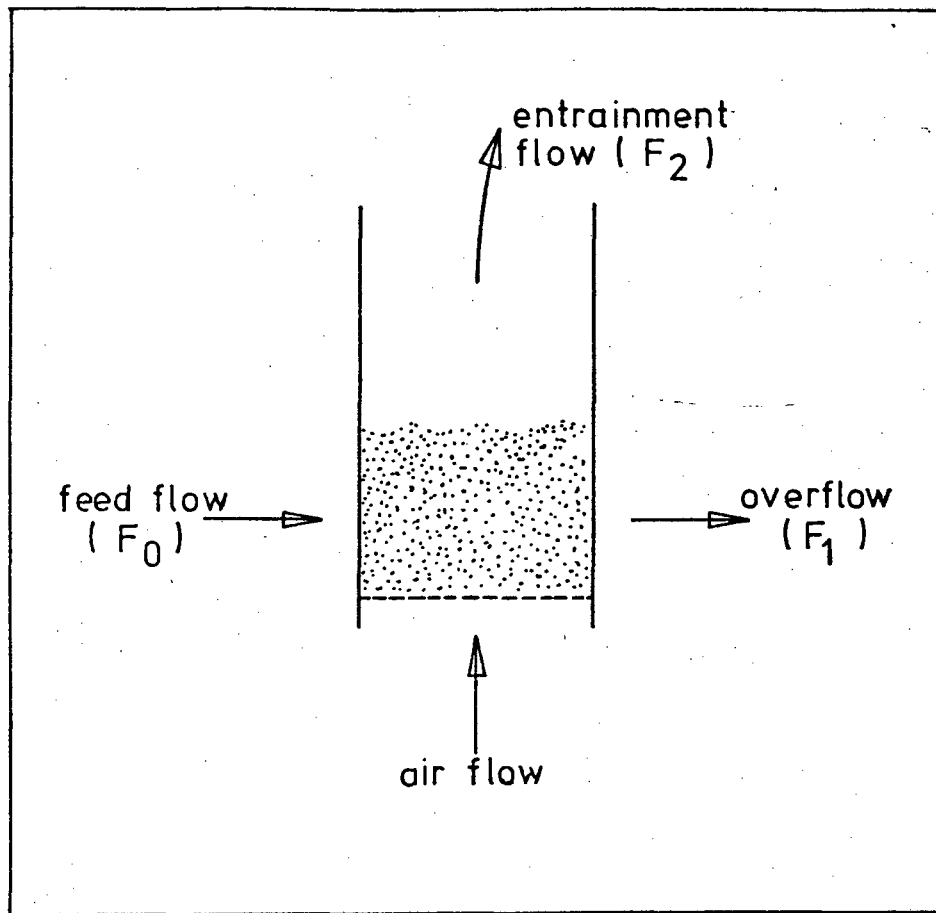
Figure 27 : Diagrammatic Representation of a Fluidized Bed to Illustrate the Components of the Mass Balance.
