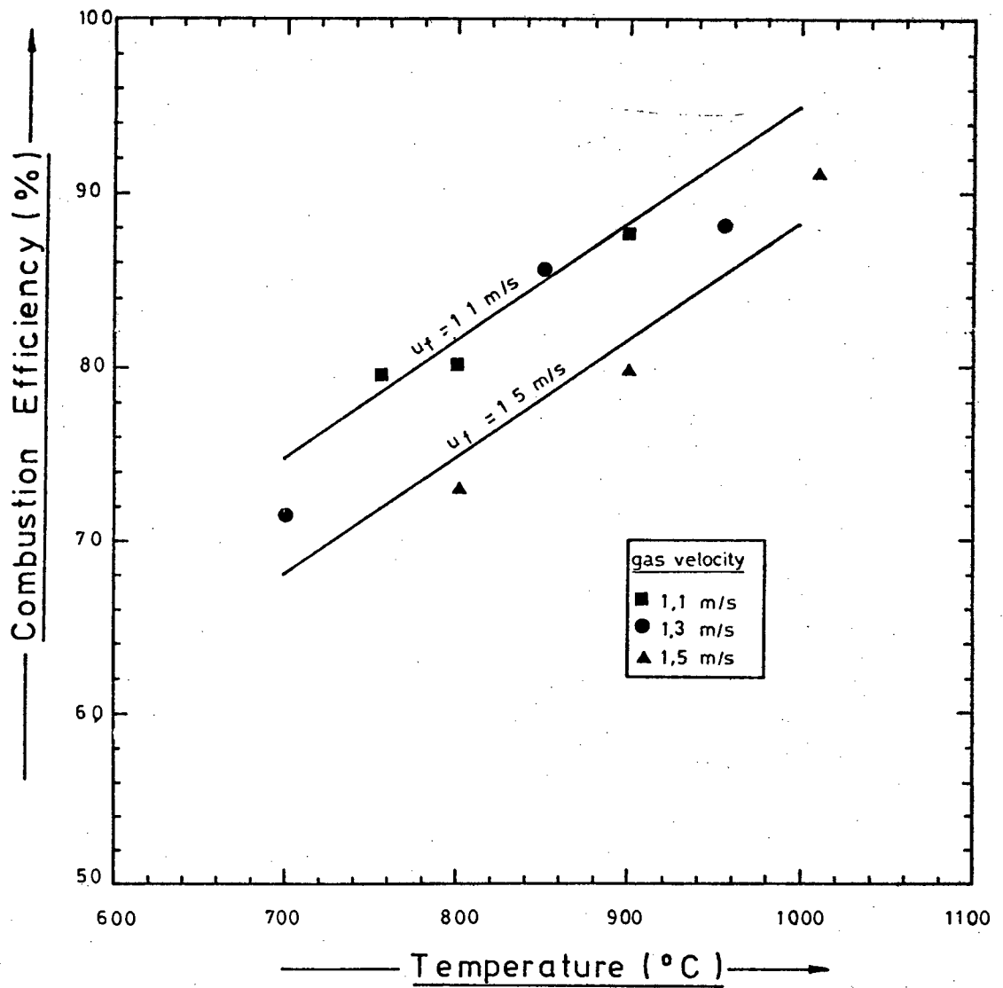
Figure 22 : Combustion Efficiencies when Burning Duff Coal in a 155 mm Deep Bed.
