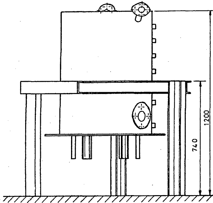
SIDE ELEVATION
