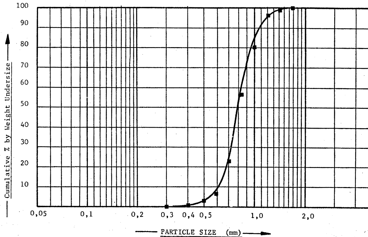
FIGURE 16 : Size Grading of Silica Sand used as Bed Material for Runs 7,8,9 and 10
