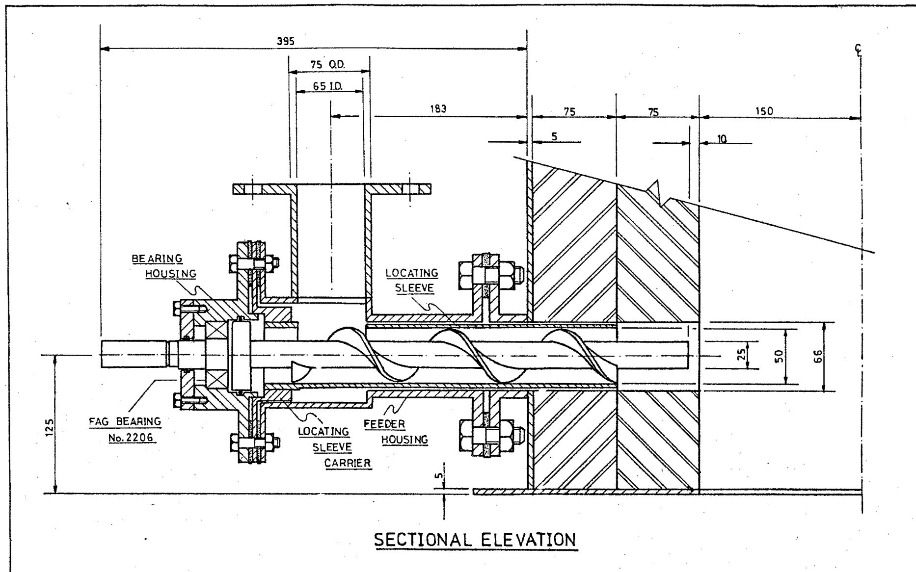
Figure A3 : Sectional Elevation of the Coal Feeder
