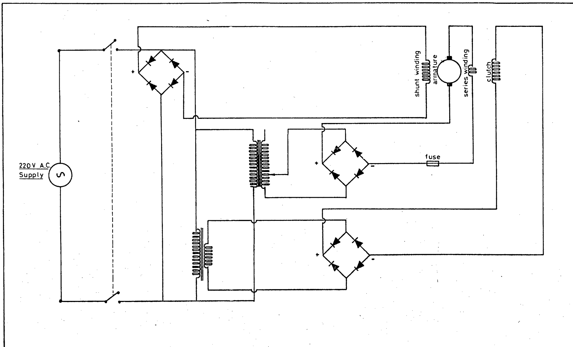
Figure A4 : Circuit Diagram for DC Motor Control
