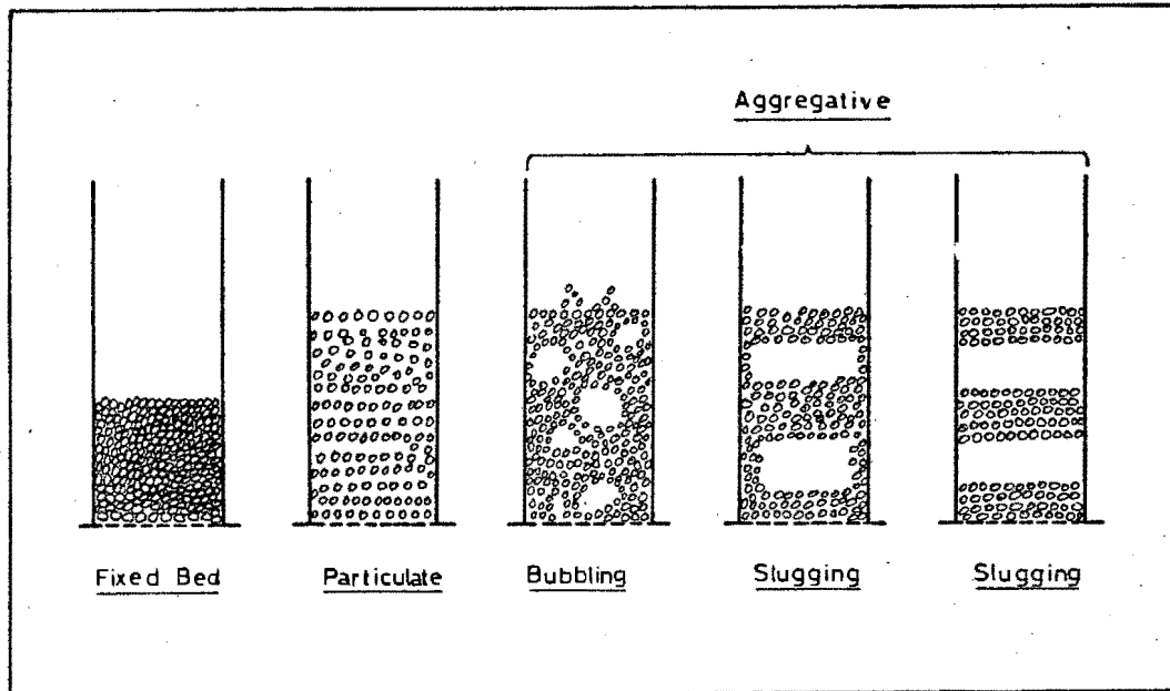
Figure 1 : Qualitative Representation of the Different Regimes of Fluidization
