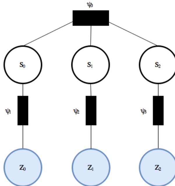
FIGURE 2.6: A generic factor graph structure. This graph factors the joint distribution as a product of four potentials,
