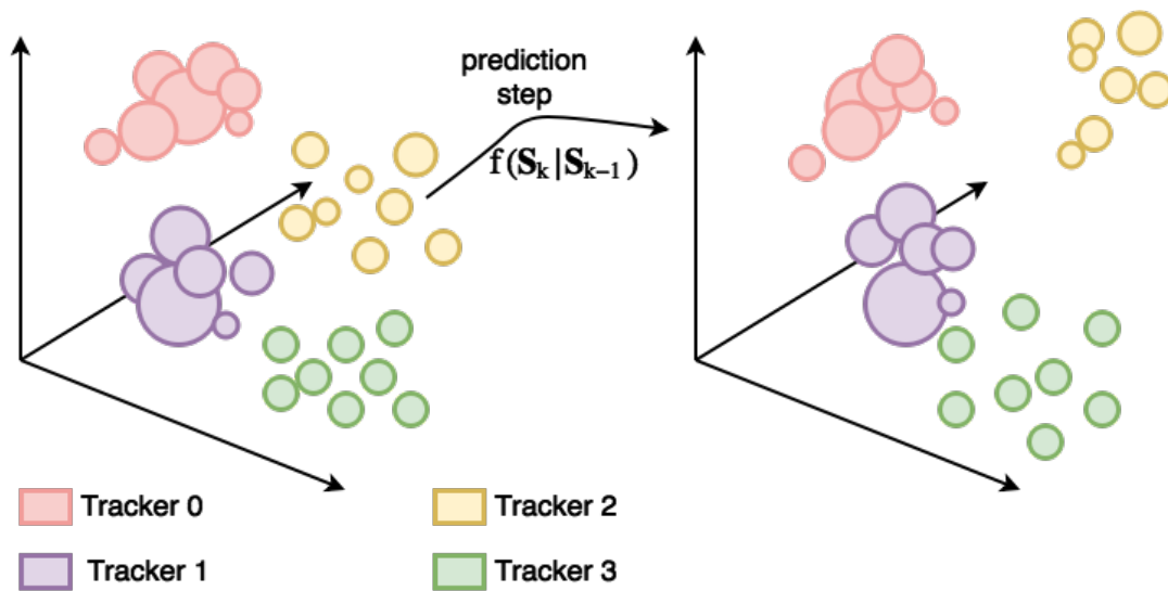
FIGURE 5.5: The particle filter internal representation of the posterior distribution. Each colour represents a different tracker: Tracker_0 , Tracker_1 , Tracker_2 and Tracker_3 . The size of each particle represents the importance or weight of each particle. The motion model f(\mathbf{S}_k|\mathbf{S}_{k-1}) propagates the particles which performs the prediction step. There are four trackers, however the ROI only contains two targets.
