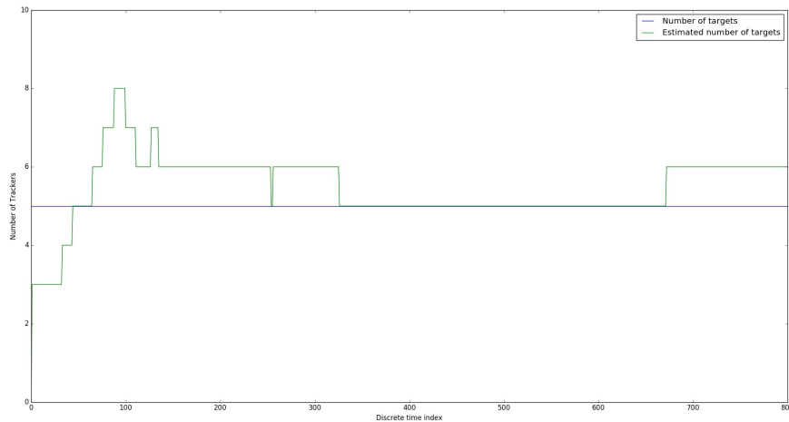
FIGURE 1.4: Cardinality estimation with simulation parameters N_t = 5 , u = 10 and d = 0.8 . The number of targets is N_t , expected number of false alarms per scan is u and probability of detection is d .
