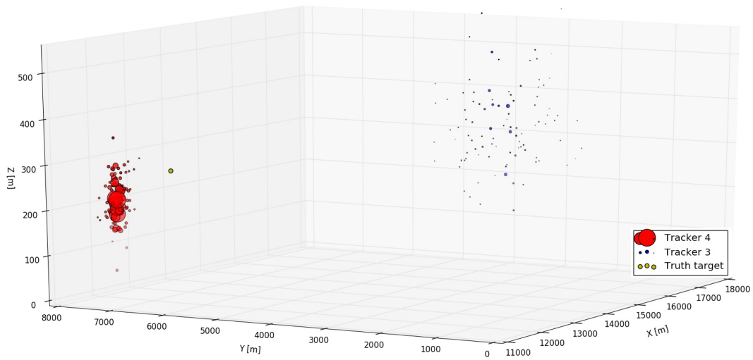
FIGURE 8.1: The posterior distribution as output by the PF.
