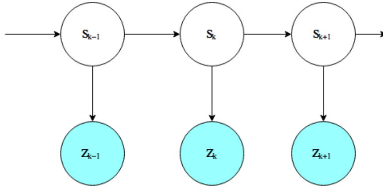
FIGURE 2.4: A Kalman filter (KF) depicted as a hidden Markov model (HMM).
