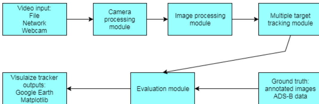
FIGURE 3.3: Visual object tracking processing pipeline.
