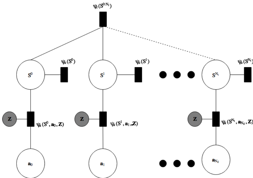
FIGURE 6.2: Factor graph describing the data association problem
