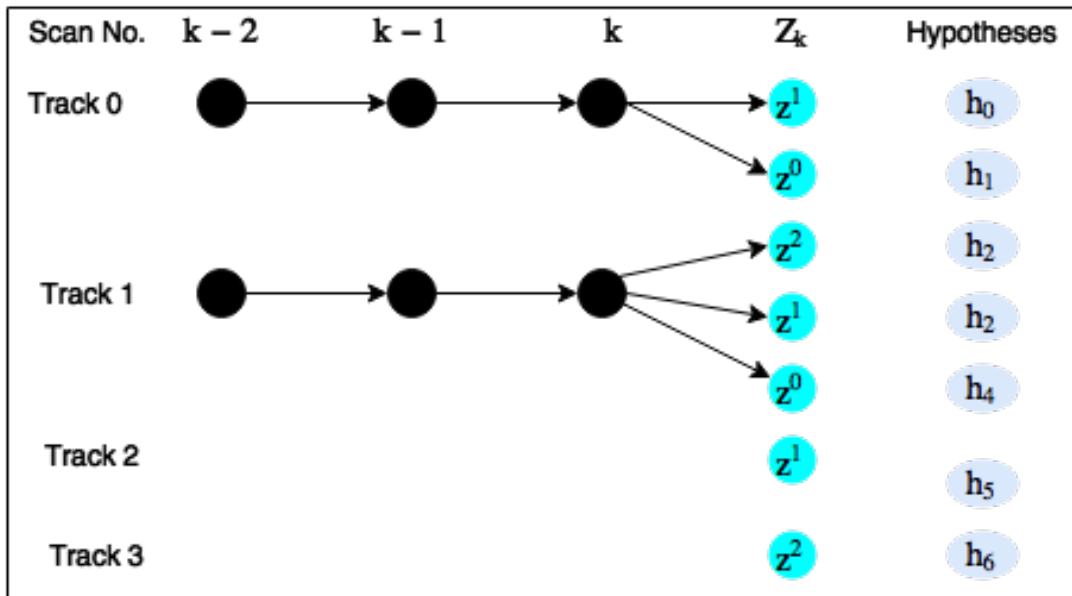
(B) Multiple hypothesis tracking hypothesis tree. At time instant k there are two trackers present in the scene and two detections are made z^1, z^2 . Based on the gating in figure 2.5a tracker_0 ( S^0 ) can only be associated with one detection z^1 or assigned a missed detection z^0 . Tracker_1 ( S^1 ) can be associated with either detection z^1 or z^2 or the missed detection z^0 . For each tracker the hypotheses are shown as well as the case for birthing new trackers. These hypotheses are denoted by h_i .
