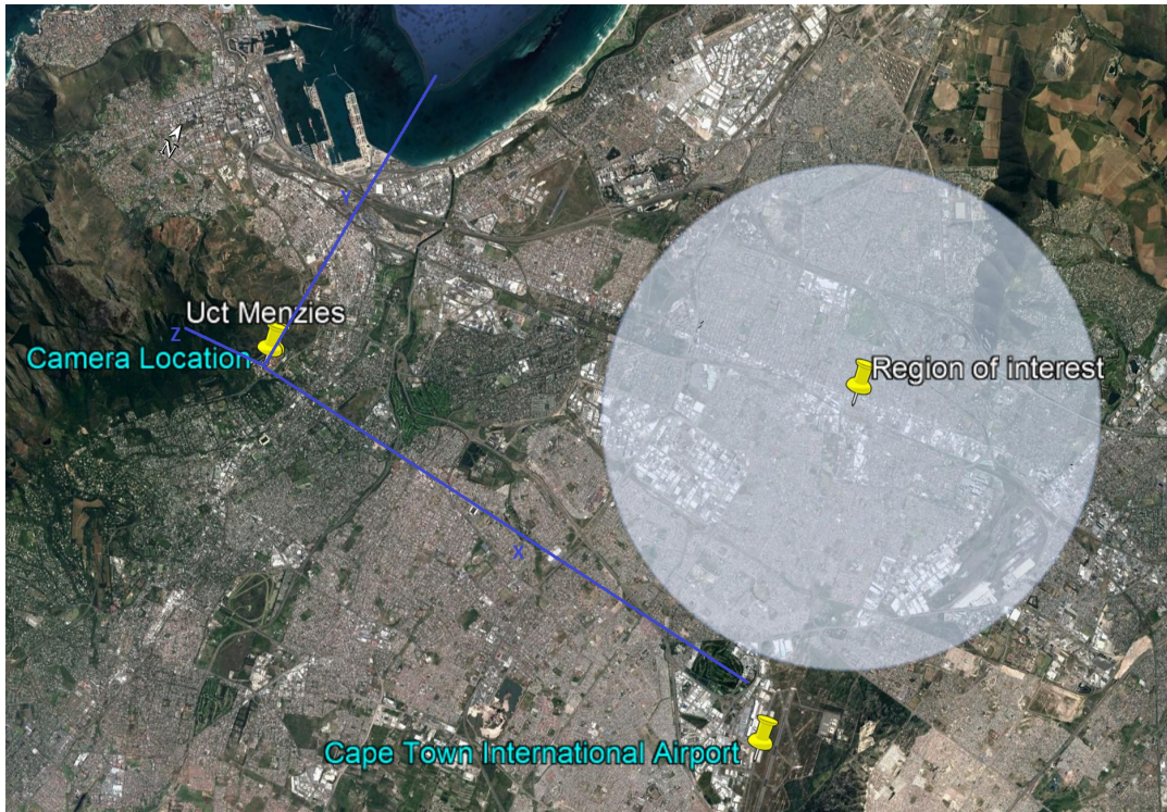
(A) The VOT system layout with a North referenced local world coordinate system
