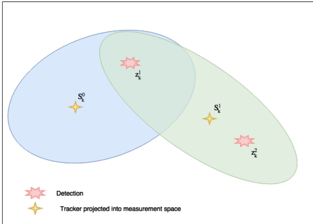
(A) Multiple hypothesis tracking hypothesis gating scheme. The gating scheme limits the possible tracker detection associations.
