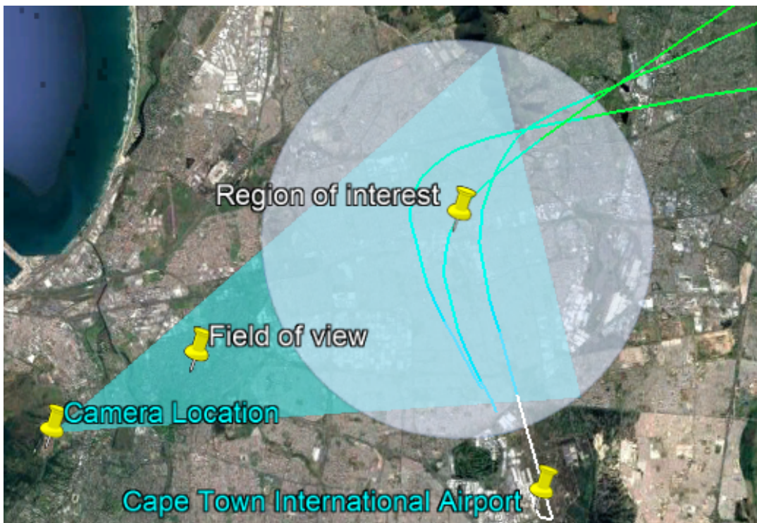
FIGURE 3.2: Site layout and typical flight paths
