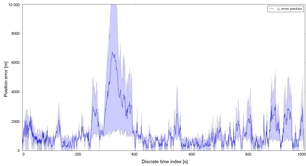
FIGURE 7.4: Position error of the mean estimate from the tracker and one standard deviation band.
