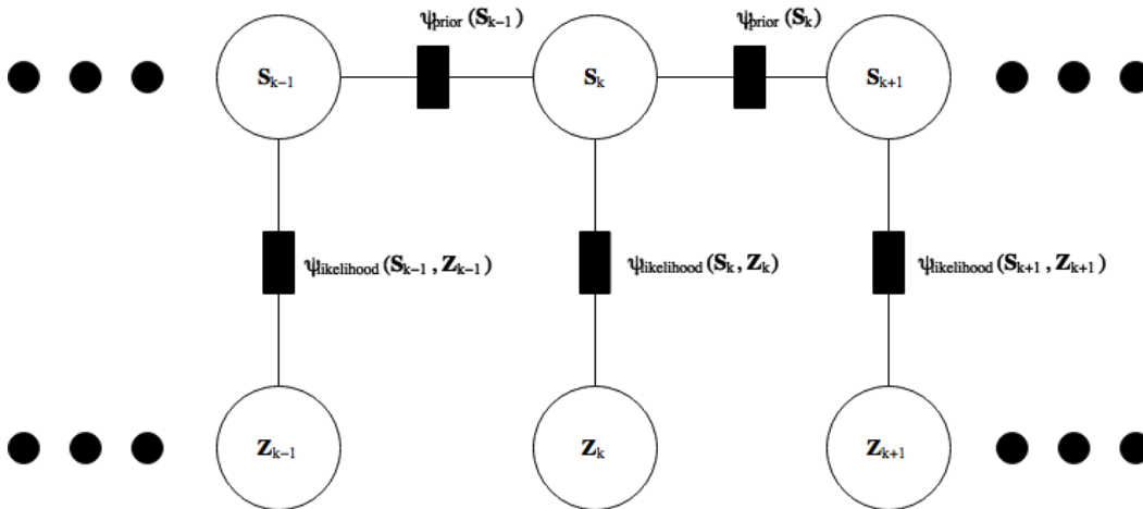
FIGURE 5.1: Factor graph overview.
