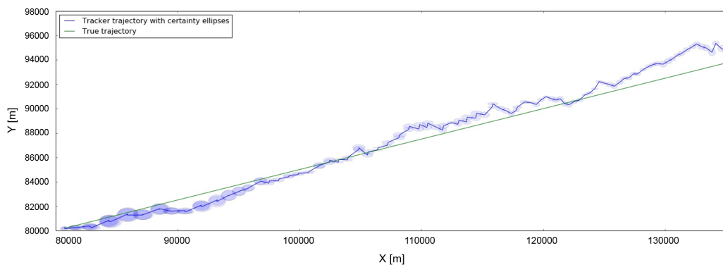
FIGURE 7.3: Tracker trajectory with covariance error ellipse and the ground truth of the target.
