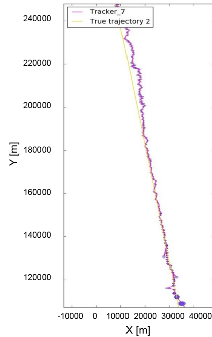
(B) Tracker 7's trajectory with covariance error ellipses plotted against the true target path.
