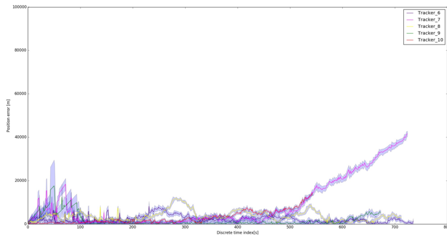
FIGURE 7.7: Position error and the first standard deviation band for all 5 long running trackers.
