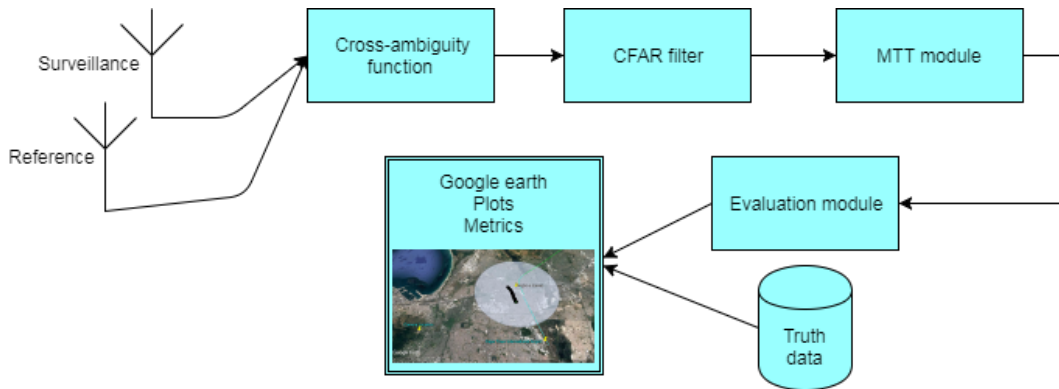
FIGURE 1.2: ( Peralex ) passive radar system system overview. The reference antenna receives the direct path signal from the illuminator. The surveillance antenna receives the time delayed and Doppler shifted signal echoed off the target and other objects in the scene. These two signals are processed by applying the cross ambiguity function and the result is passed through a constant false alarm rate filter to form detections. These detections are fed to the MTT module.
