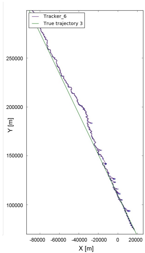
(A) Tracker 6's trajectory with covariance error ellipses plotted against the true target path.
