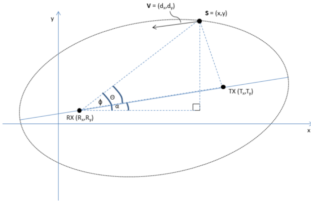
FIGURE 7.2: Geometry of the bistatic passive radar system in a two-dimensional Cartesian plane[17]. A point target is at position S = (x, y) and travelling with a velocity of V = (d_x, d_y) . The receiver and transmitter are R_X(R_x, R_y) and T_X(T_x, T_y) respectively. The angle measured by the DOA module is \phi .
