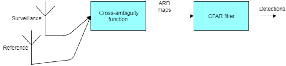
FIGURE 2.3: A schematic of the passive radar system for tracking aircraft.
