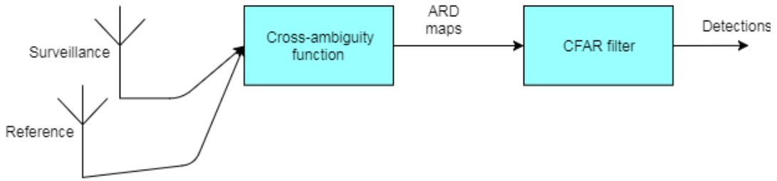
FIGURE 7.1: Passive radar processing pipeline.
