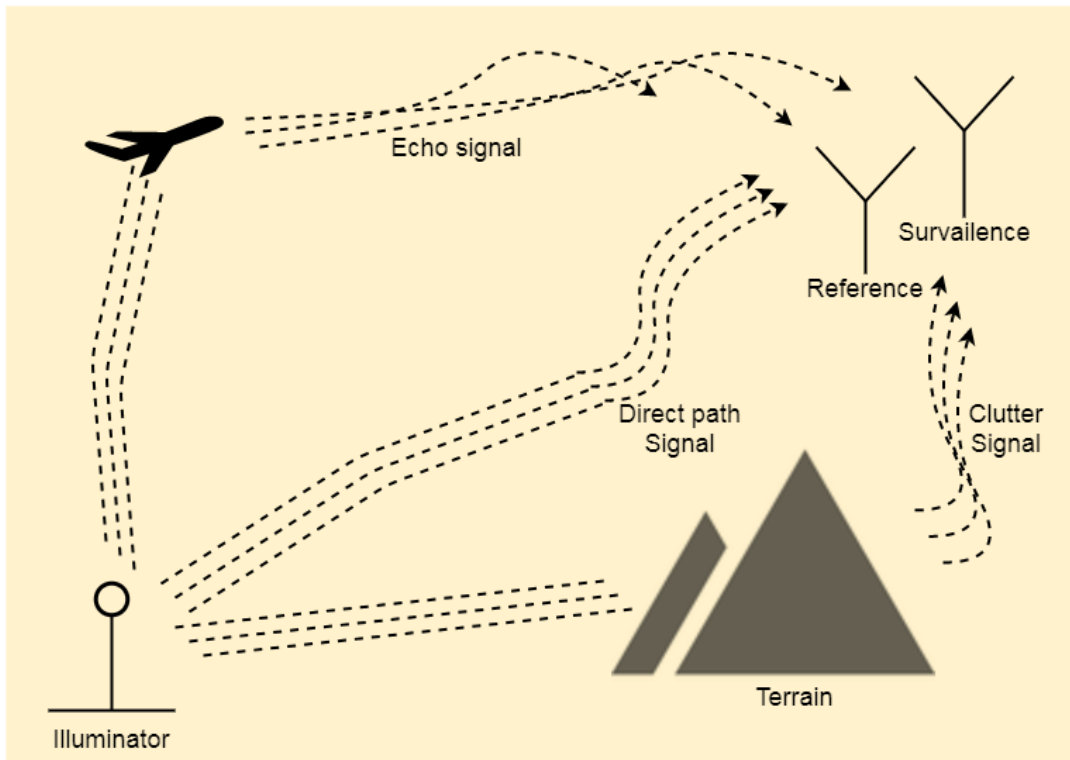
FIGURE 1.3: Bistatic passive radar setup.
