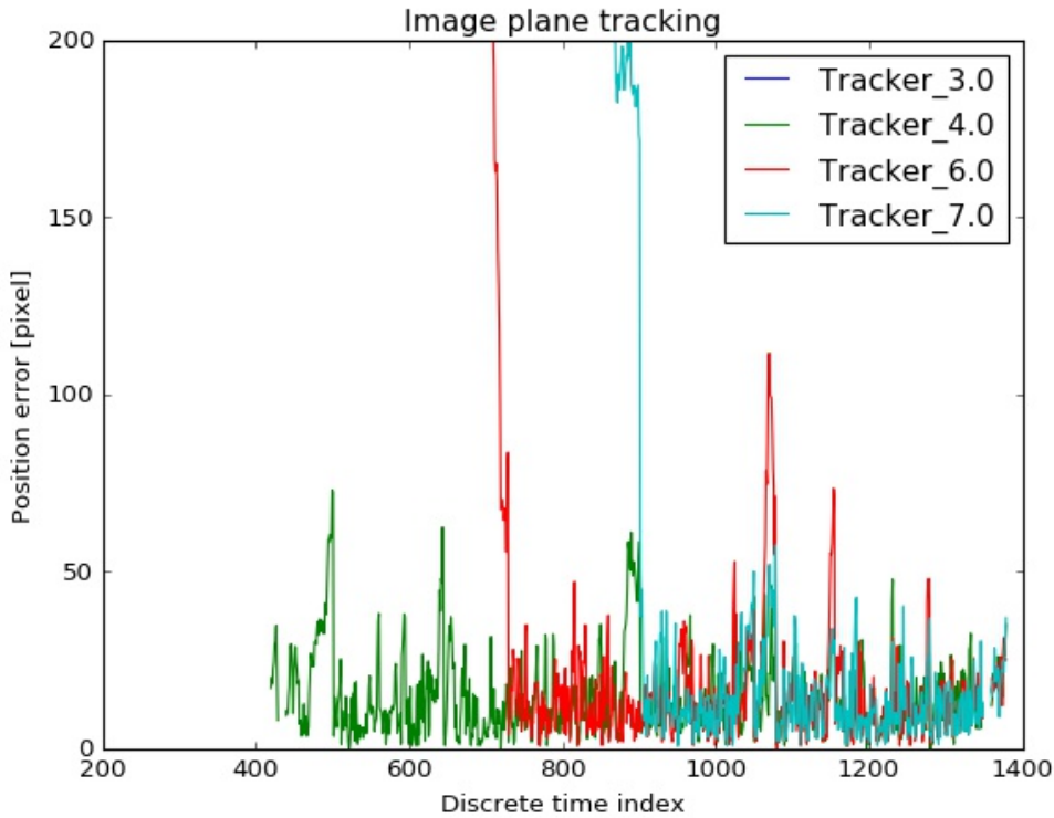
FIGURE 8.3: The re-projection error for the sequence 08112017_MVI_BA6419. Tracker 4 is the longest persisting. Trackers 6 and 7 converge to the same image frame positions. The mean and standard deviation error for each tracker is as follows:
