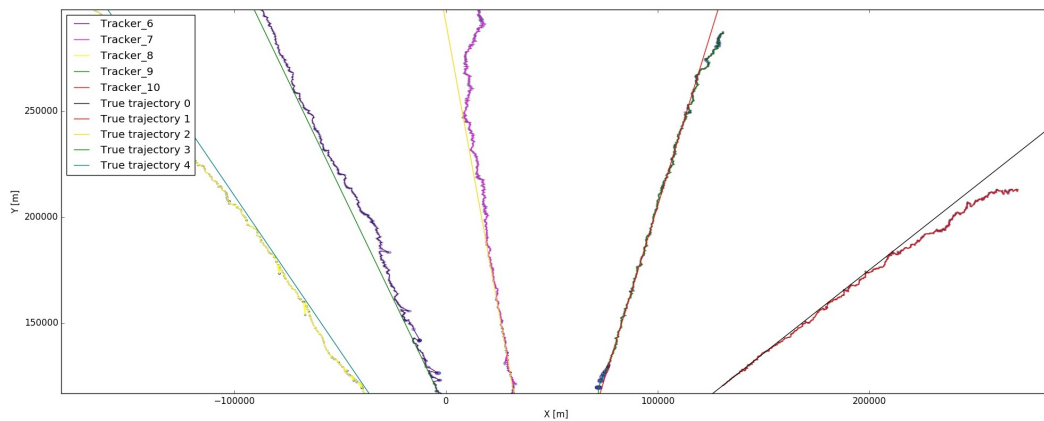
FIGURE 1.5: Passive radar simulated scene with simulation parameters N_t = 5 , u = 10 and d = 0.8 .
