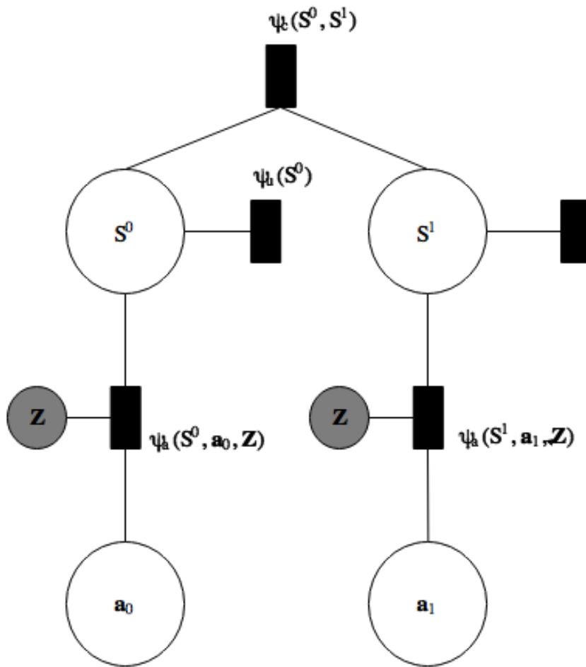
FIGURE 6.1: Data association graphical model for the two-aircraft example.
