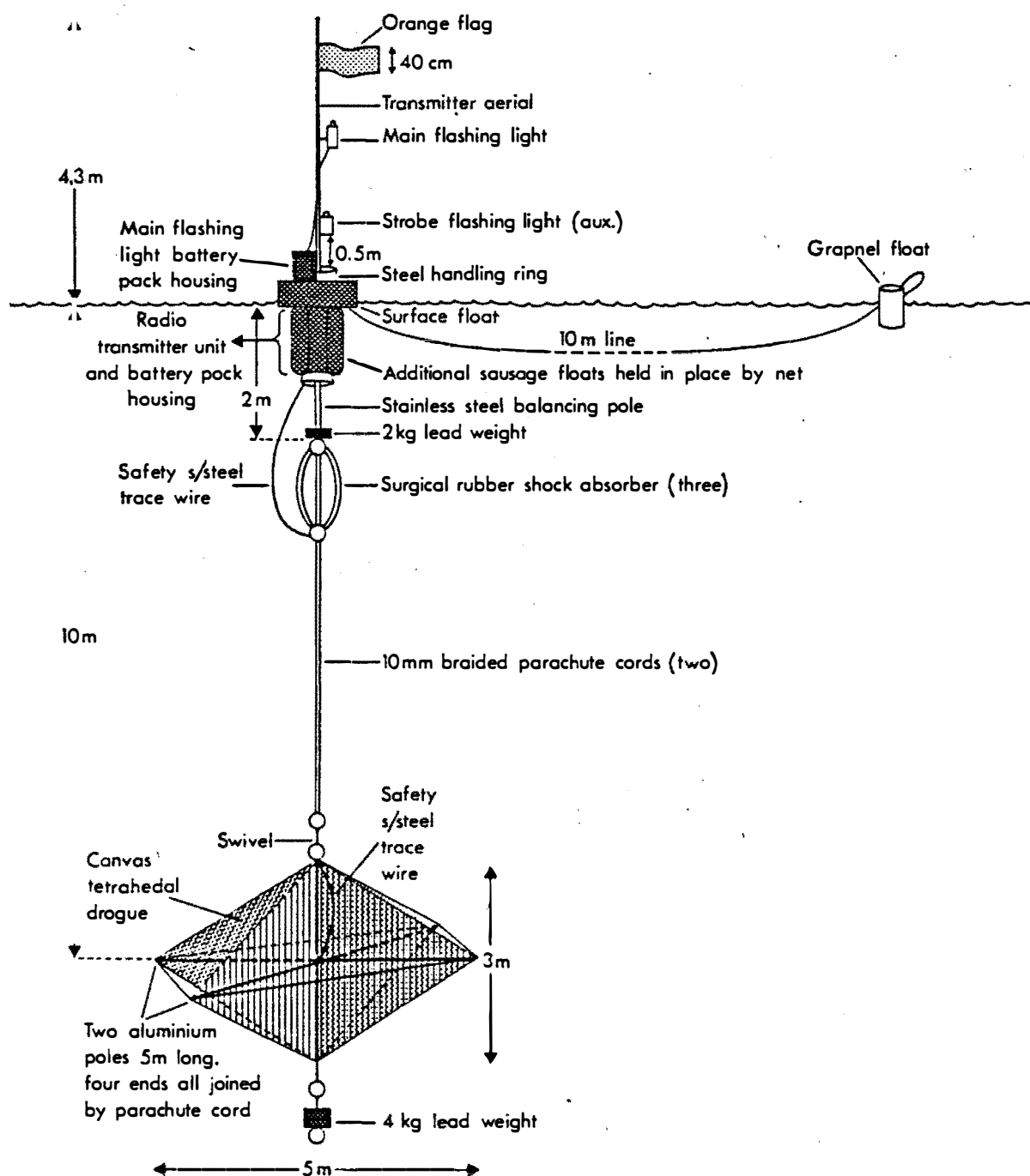
Fig.4.2: The drogue
