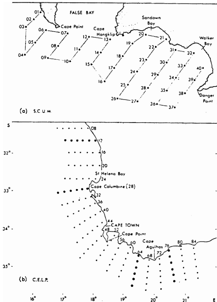
FIG. 6.— Station positions for: (a) the South Coast Upwelling Monitoring (SCUM) cruises from January to December 1975, and (b) for the Cape Egg and Larval Program (CELP) from August 1977 to August 1978. Heavy dots indicate the lines (12, 28, 64 and 76) used for vertical sections.
