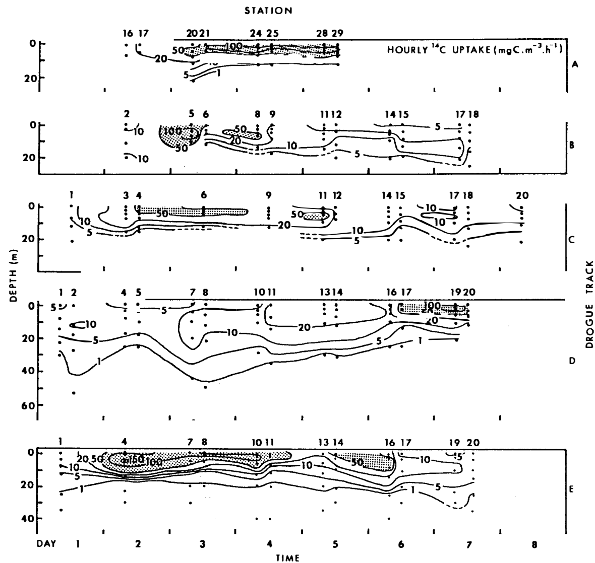
Fig.8.1: Vertical sections of hourly ^{14}\text{C} -uptake productivity measurements along Drogue tracks A-E (shading indicates rates greater than 50 \text{ mg C.m}^{-3}.\text{h}^{-1} ).
