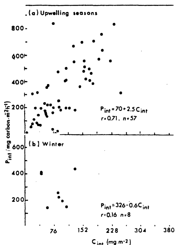
Fig. 4: Plots of P_{int} versus C_{int} during (a) the upwelling seasons and (b) winter
