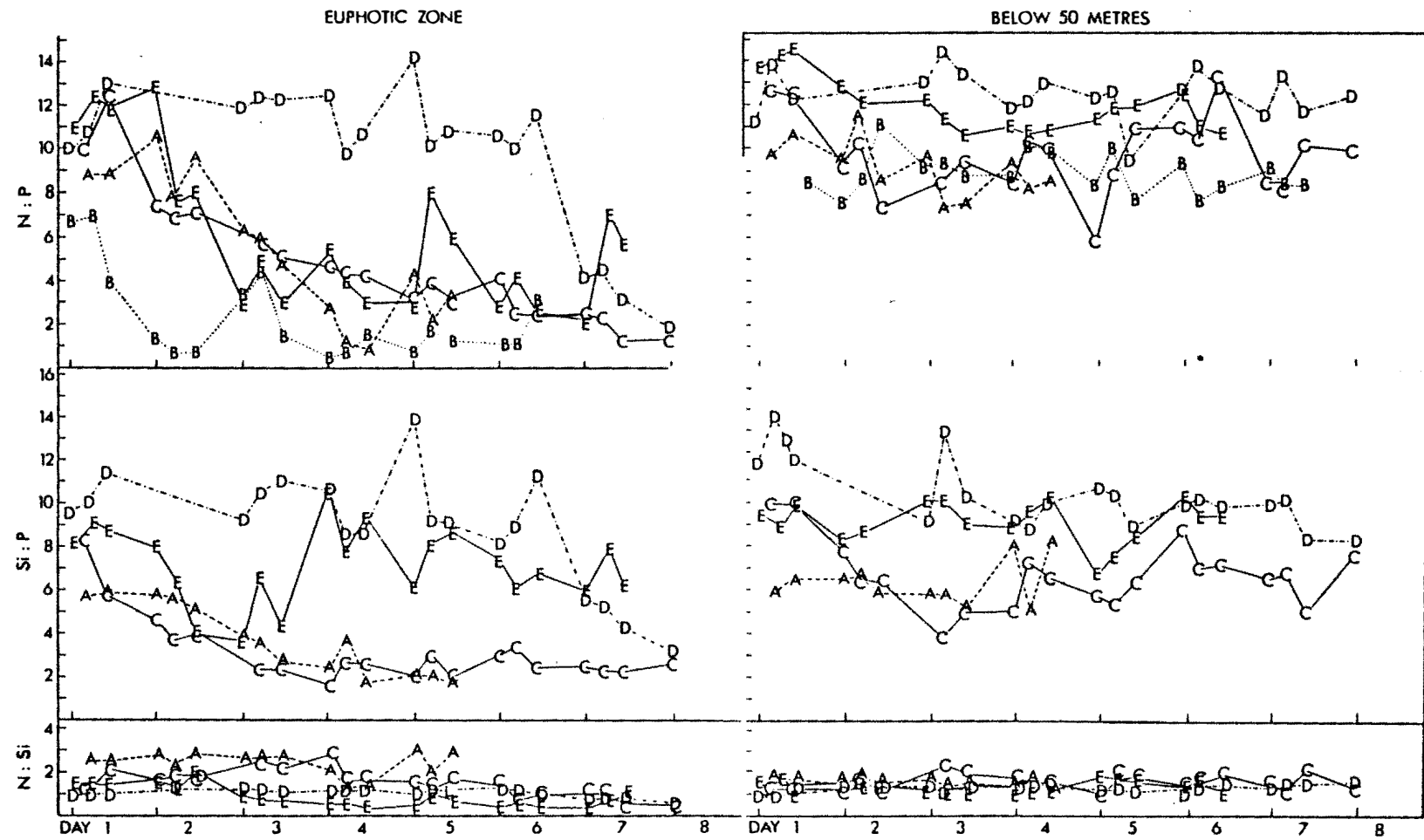
Fig.7.2: Mean atomic ratios (of occurrence) of the major nutrients (N:P, Si:P and N:Si) in the euphotic zone and below 50 m along Droque tracks A-E.
