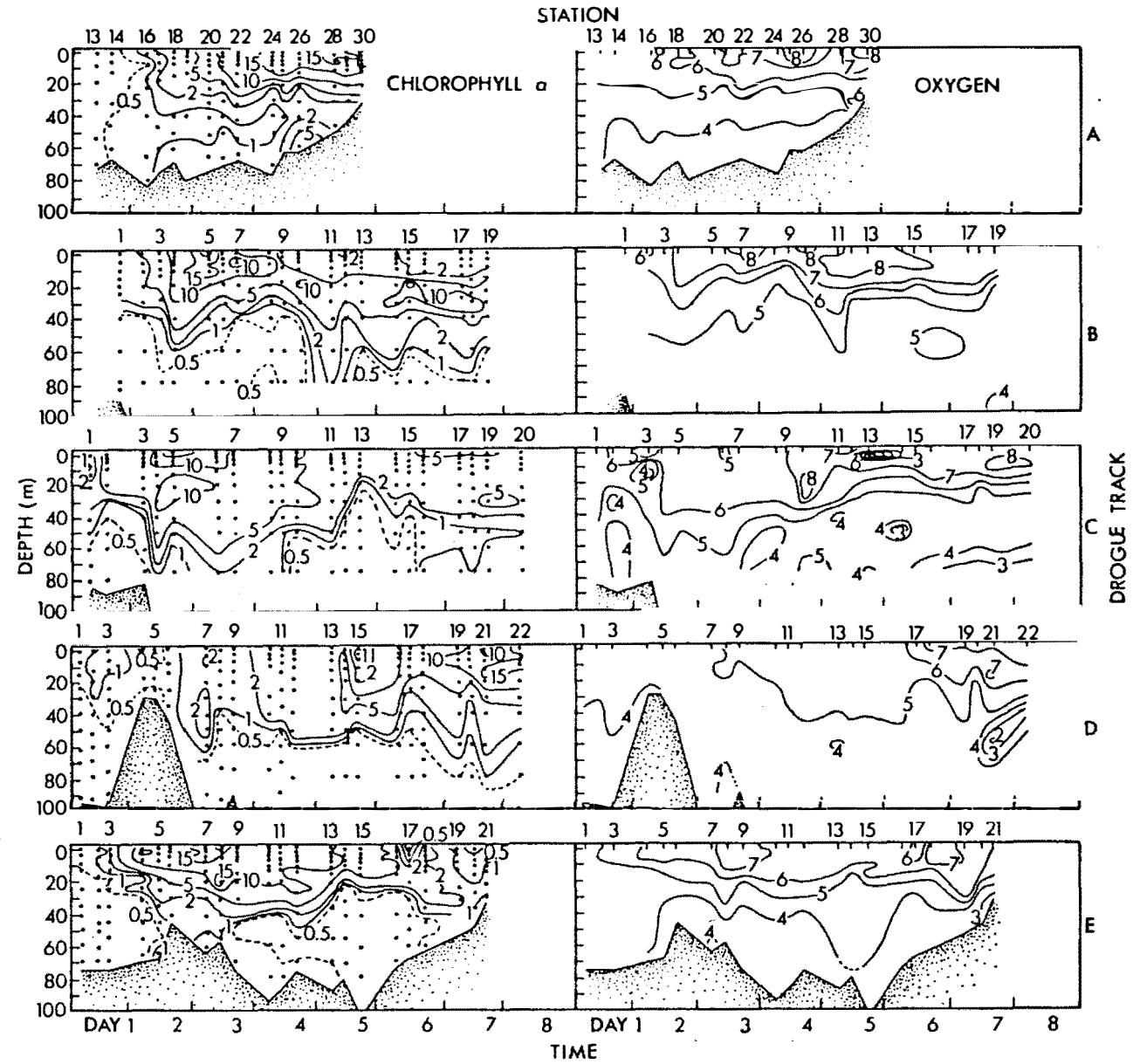
Fig.6.2: Vertical sections of chlorophyll a (mg.m -3 ) and dissolved oxygen (dm 3 .m -3 ) concentrations along Drogue tracks A-E.
