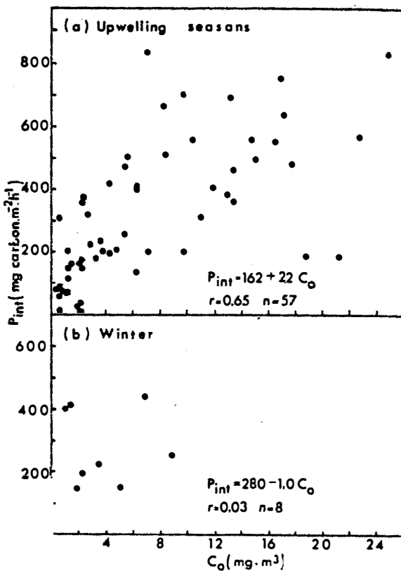
Fig. 6: Plots of P_{int} versus C_o during (a) the upwelling seasons and (b) winter
