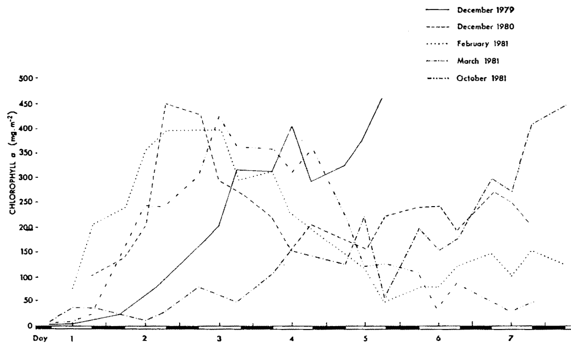
FIG. 9. — Phytoplankton biomass (mg chl a · m -2 from 0-40 metres) during five drogue-tracking Plankton Dynamics cruises.
