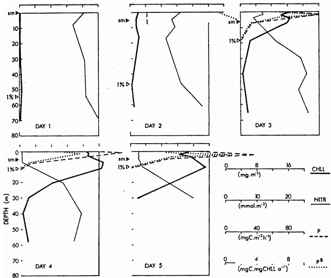
Fig.8.6: Representative depth profiles of phytoplankton biomass (CHLL), the hourly rate of ^{14}\text{C} productivity (P), biomass standardized productivity ( P^B ) and nitrate concentrations (NITR) with the depths of surface mixing (sm) and the 1% light level (1%) for each day of Cruise A.
