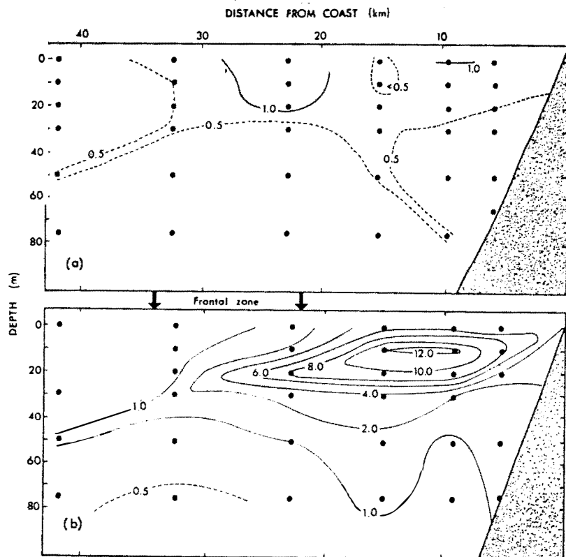
FIG. 3.— Vertical distribution of phytoplankton (mg chl. a ·m -3 ) along Line 4 of the 1969 Upwelling Cruise: (a) during upwelling on 16 December, and (b) during downwelling on 13 December. (From ANDREWS and HUTCHINGS, 1980.)
