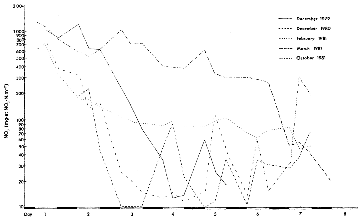
FIG. 11. — Distribution of nitrates (mg-at NO-N·m -2 ) in the euphotic zone during five drogue-tracking Plankton Dynamics cruises.
