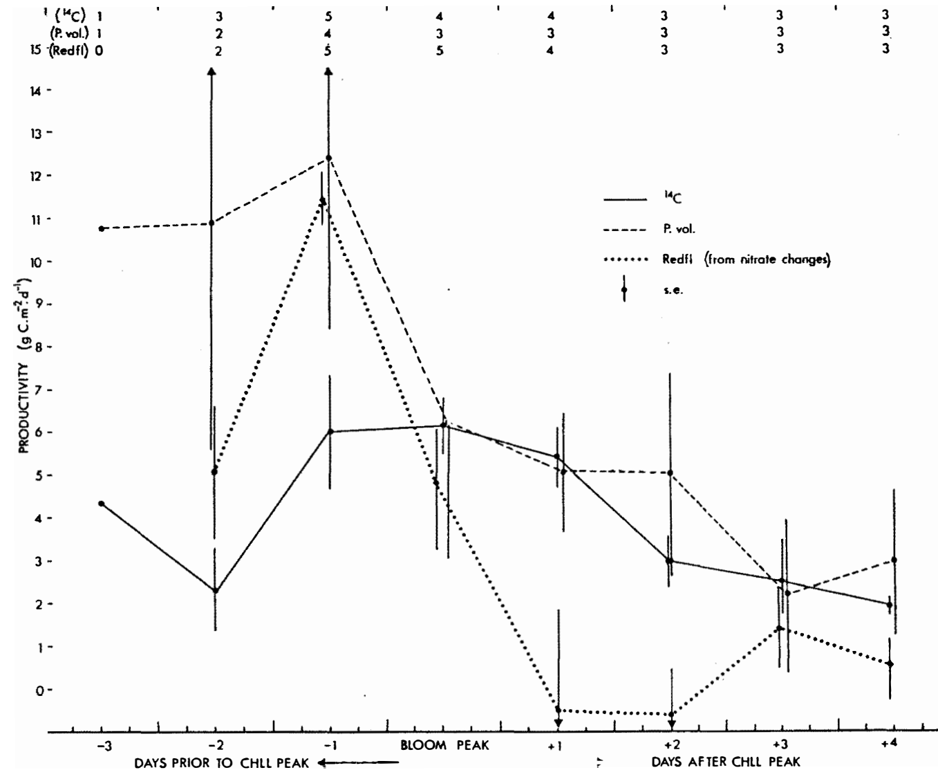
Fig.9.2: Mean productivity estimates, using the ^{14}\text{C} -uptake ( ^{14}\text{C} ), particle volume (P.vol) and Redfield (Redfl) methods, during the build up and decline of a phytoplankton bloom using data for Cruises A-E (n is the number of data from which each mean is calculated and s.e. is the standard error). The "bloom peak" and days prior to and after the peak coincide with those in Fig.9.1.
