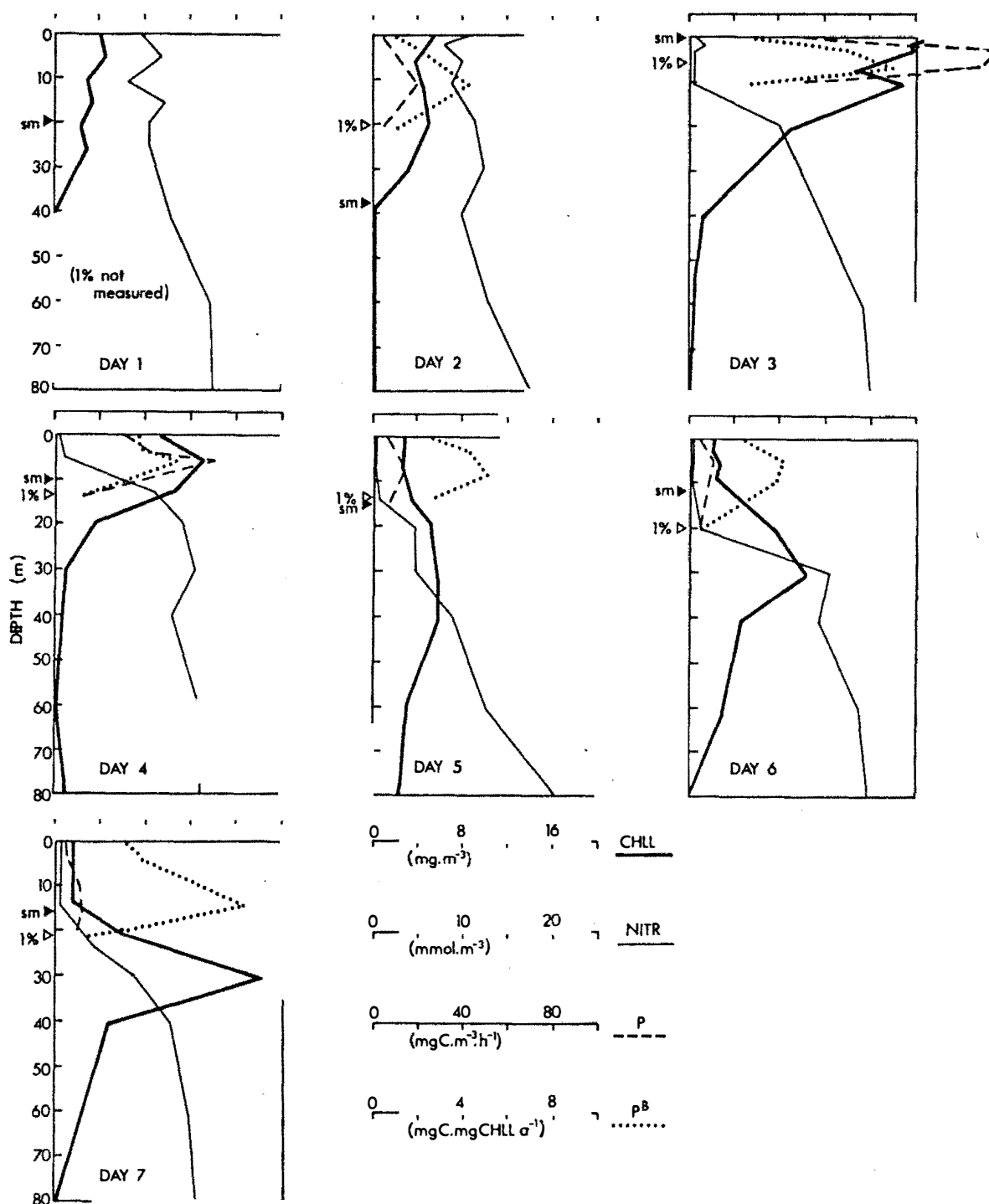
Fig.8.10: Representative depth profiles of phytoplankton biomass (CHLL), the hourly rate of 14 C productivity (P), biomass standardized productivity (P B ) and nitrate concentrations (NITR) with the depths of surface mixing (sm) and the 1% light level (1%) for each day of Cruise B.
