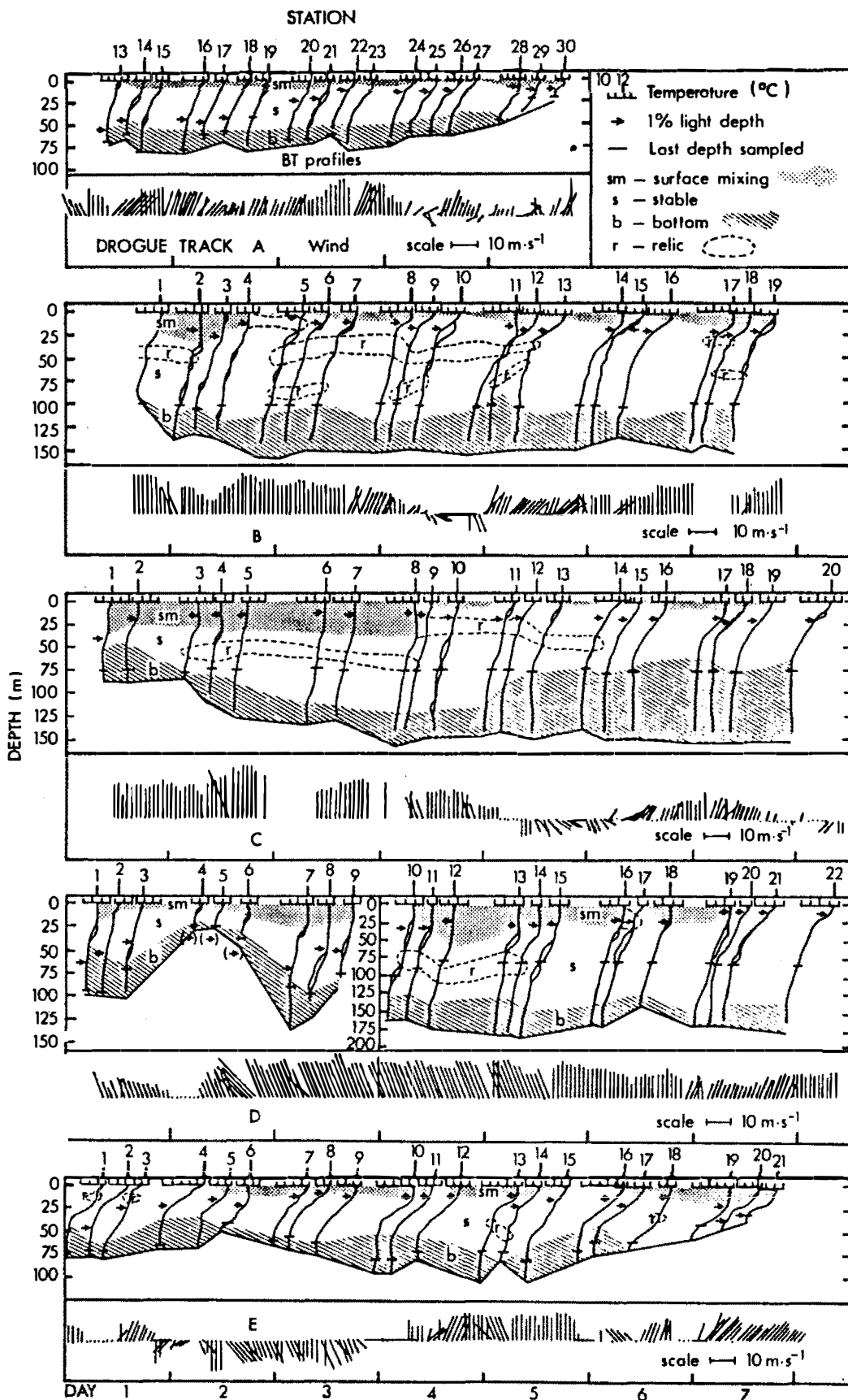
Fig.5.12: Hourly wind stick-vector diagrams and bathythermograph profiles along Drogue tracks A-E. The water column is partitioned into surface mixing (sm), relic (r) and bottom (b) mixed layers, with a stable (s) layer between the sm and b layers. The 1% light depth and the last depth at which water samples were drawn, are also indicated. Wind vectors show the direction in which the wind is blowing.
