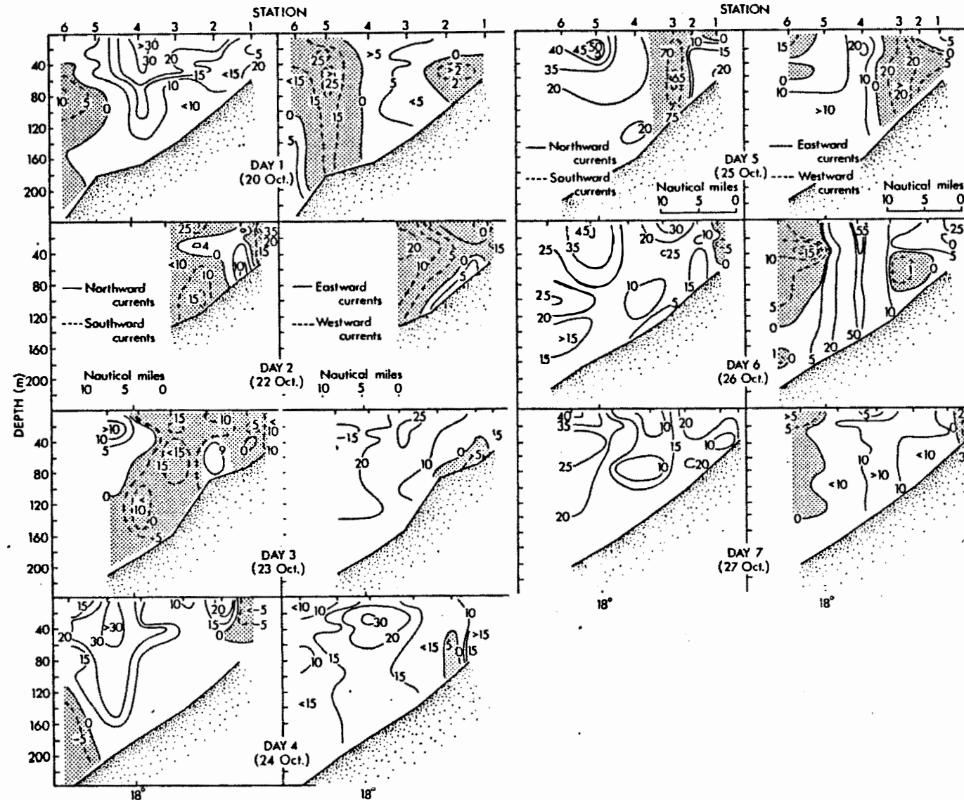
Fig.5.7: Daily transects of current measurements across the path of Droque E showing north-south and east-west components of the current (after Holden 1981). Shading represents southward and westward flow. The drogue position was between stations 3 and 4.
