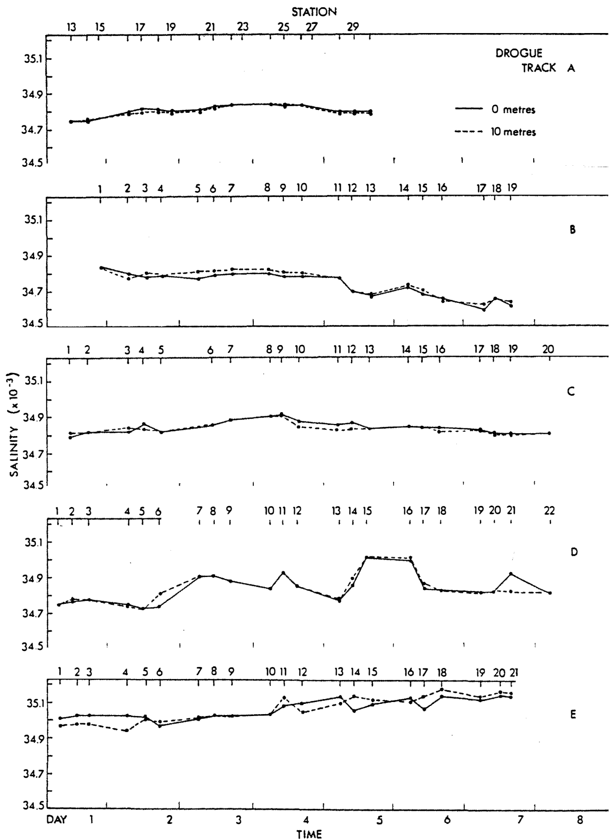
Fig.5.10: Salinity at 0 m and 10 m along Drogue tracks A-E.
