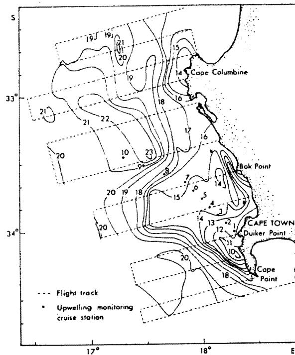
FIG. 4. — Surface temperature ( ^{\circ}\text{C} ) distribution (from Airborne Radiation Thermometer data) of the southern Benguela Current during upwelling on 14 January 1973, with station positions for the Upwelling Monitoring cruises. (From ANDREWS and HUTCHINGS, 1980.)
