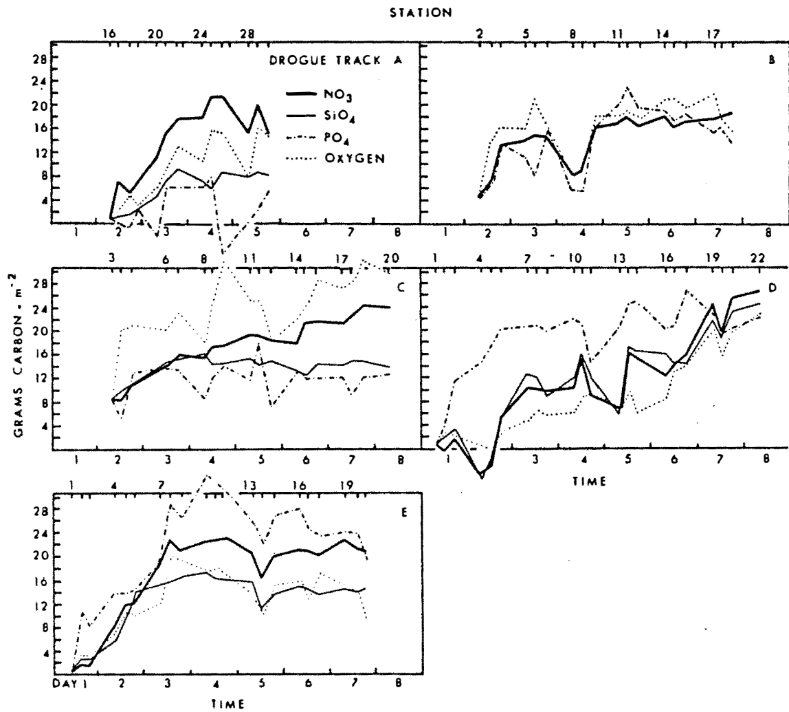
Fig.8.4: Redfield productivity (g C.m -2 ) estimated from changes in the nutrient (nitrate, silicate and phosphate) and oxygen content of the upper 20 m layer along Drogue tracks A-E.
