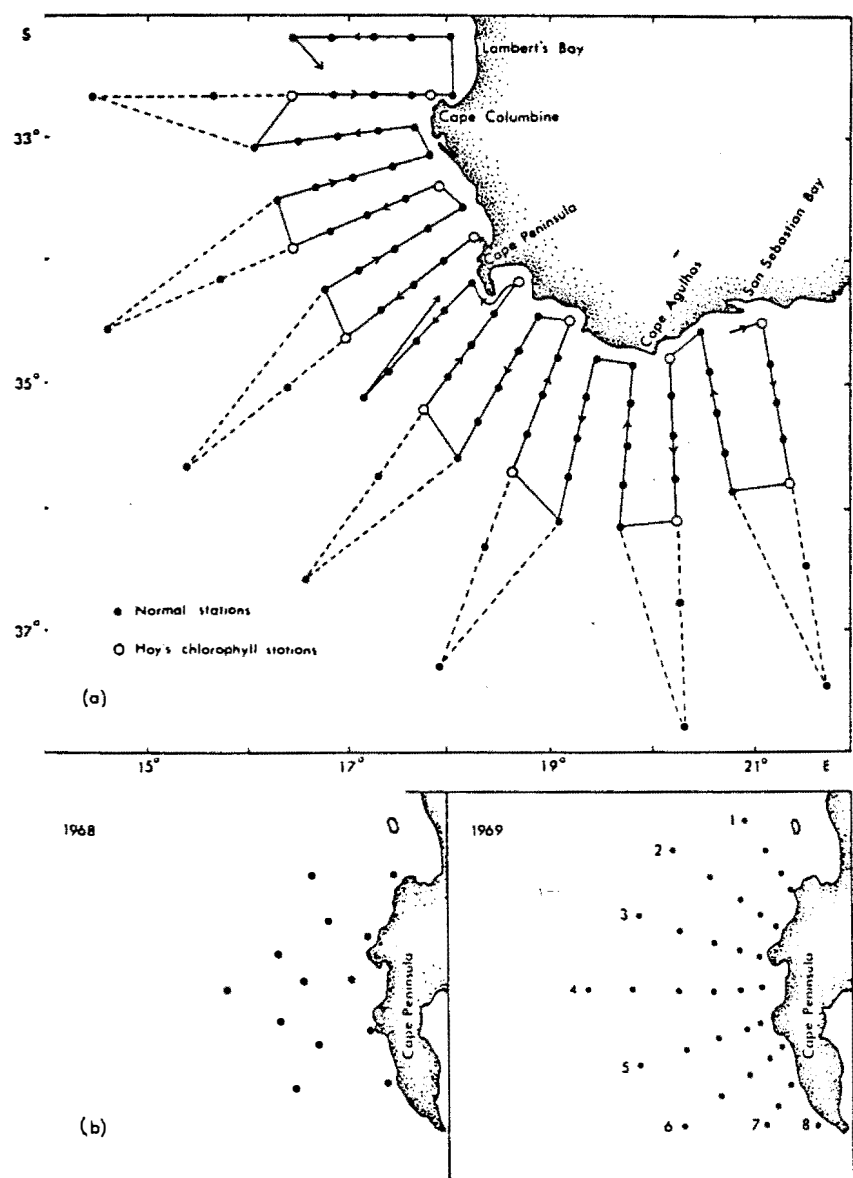
FIG. 2. — Station positions for: (a) the Routine Grid between July 1963 and December 1967 (station positions for the period from 1961 to July 1963 were slightly different), and (b) the Upwelling Cruises in November 1968 and December 1969, showing the station line numbers for the 1969 cruise.
