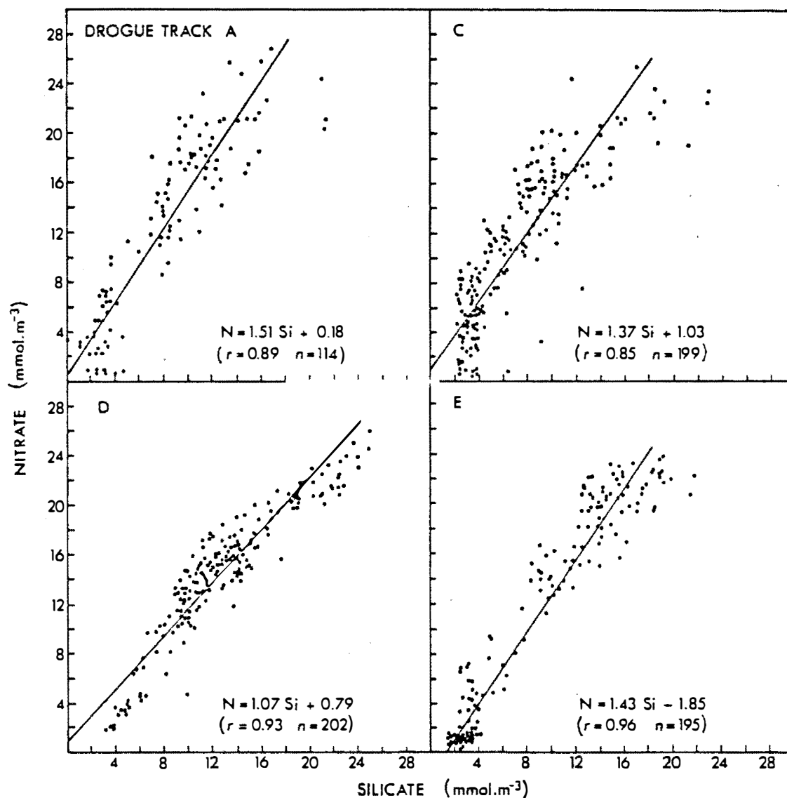
Fig.7.7: Relationships between nitrate and silicate concentrations along Drogue tracks A-E. The geometric regression equation for the combined data sets (A-E) is N = 1.27 Si - 0.2 , r = 0.90 , n = 710 .
