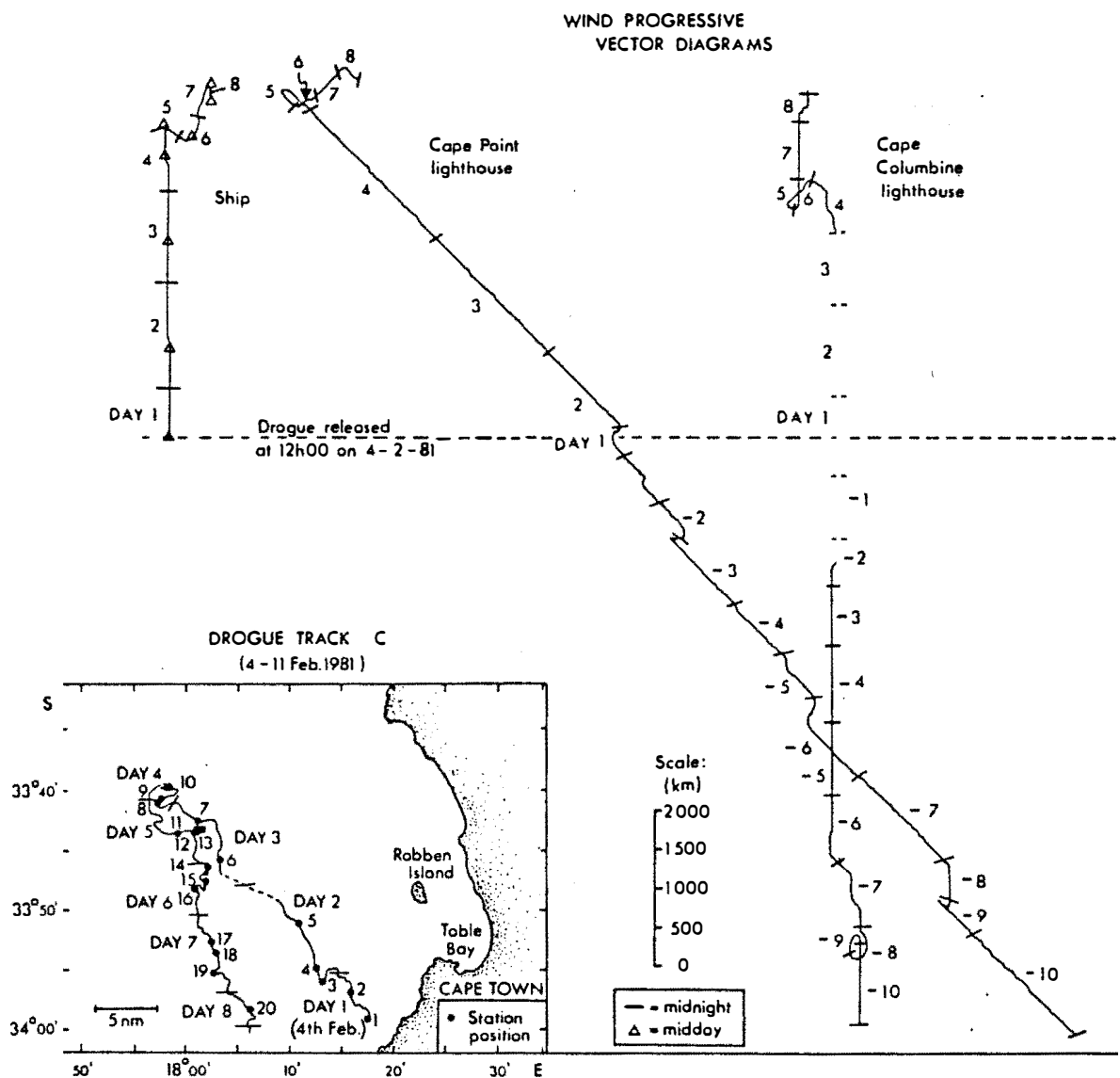
Fig.5.4: Drogue track C (February 1981) showing station positions, and progressive vector diagrams for hourly wind measurements on board ship and at the Cape Point and Cape Columbine lighthouses.
