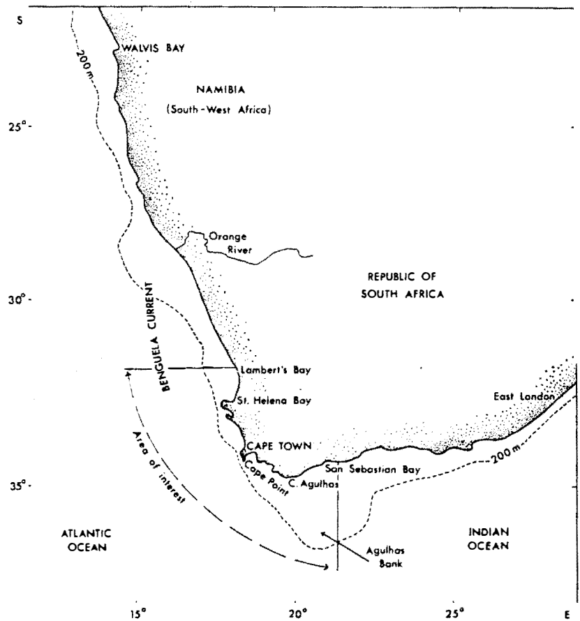
FIG. 1.— The south and west coast of southern Africa showing the area between Lamberts Bay and San Sebastian Bay where most phytoplankton research in the southern Benguela Current region has been done.
