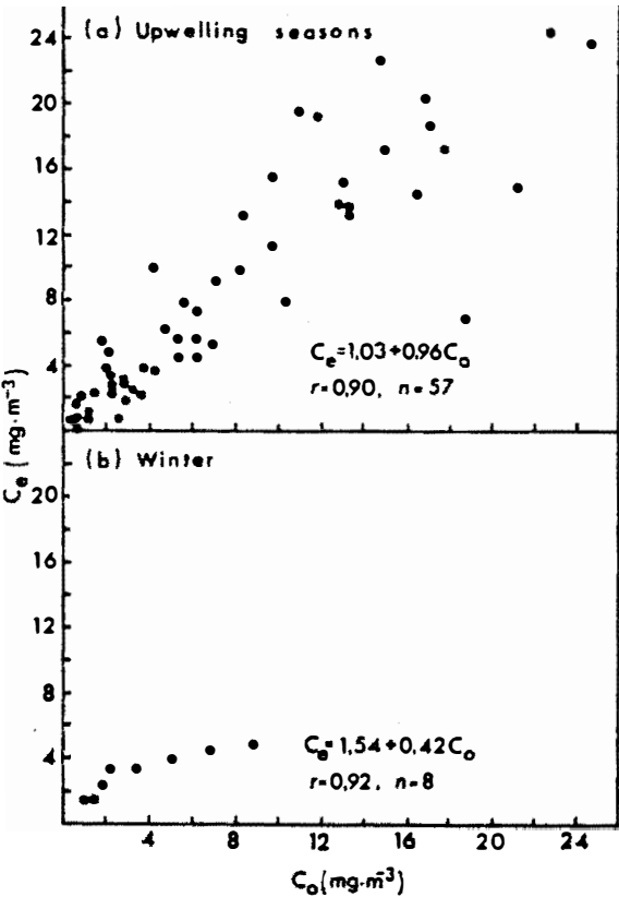
Fig. 2: Plots of C e versus C s during (a) the upwelling seasons and (b) winter
