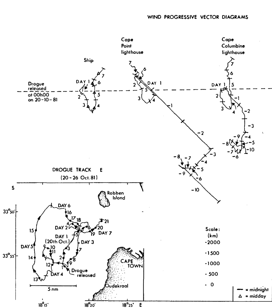
Fig.5.6: Drogue track E (October 1981) showing station positions, and progressive vector diagrams for hourly wind measurements on board ship and at the Cape Point and Cape Columbine lighthouses.
