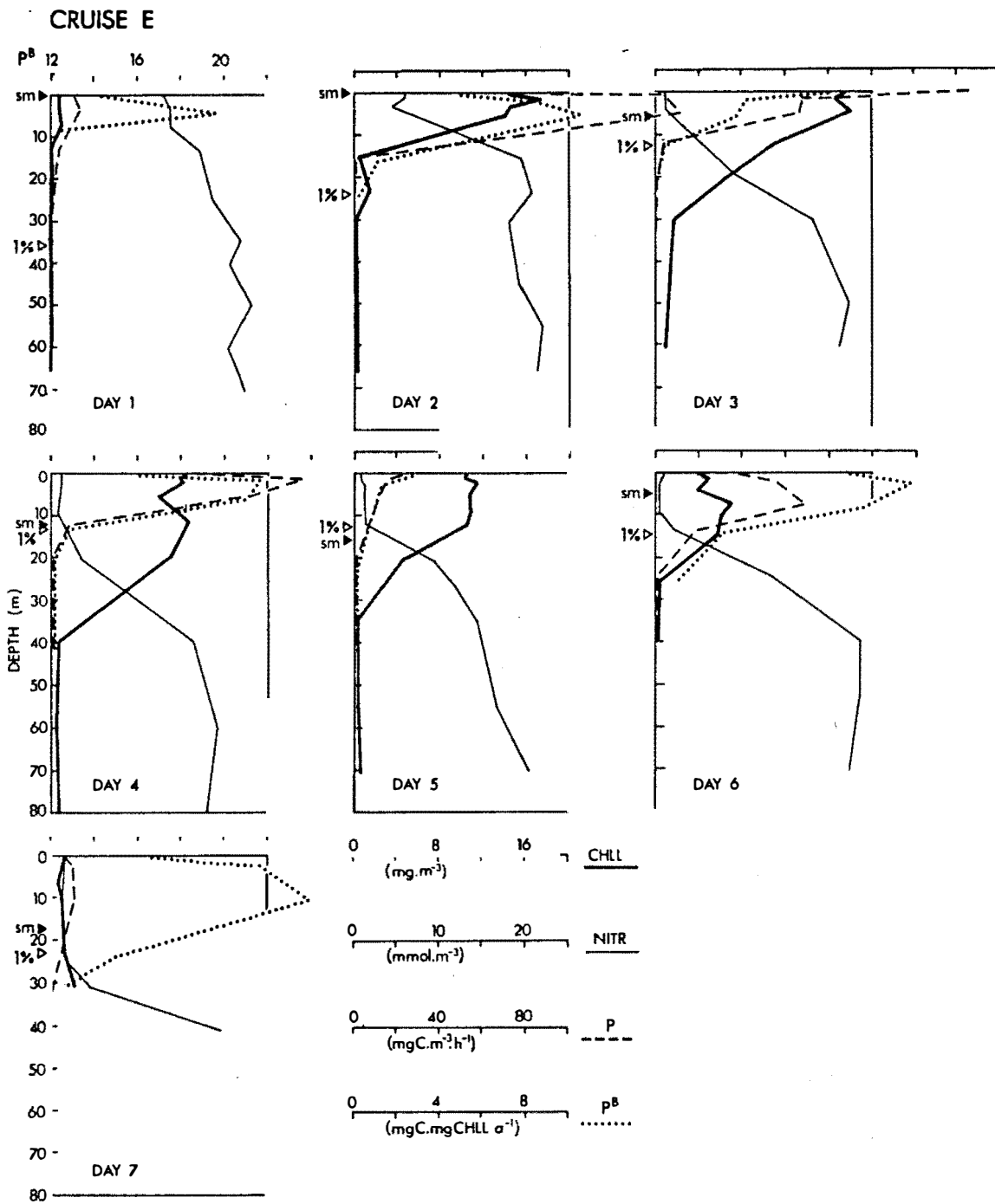
Fig.8.7: Representative depth profiles of phytoplankton biomass (CHLL), the hourly rate of ^{14}\text{C} productivity (P), biomass standardized productivity ( P^B ) and nitrate concentrations (NITR) with the depths of surface mixing (sm) and the 1% light level (1%) for each day of Cruise E. Note that the P^B for Day 1 has been shifted to accommodate the high values on the graph.
