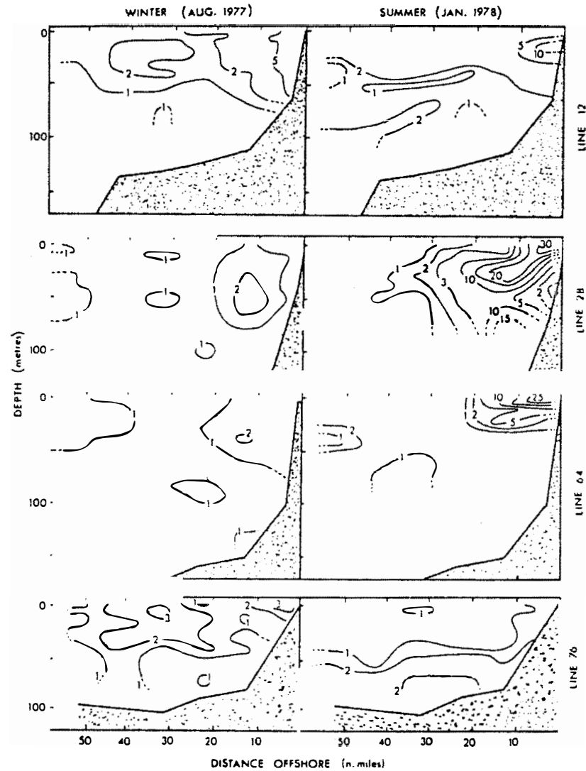
FIG. 7. — Vertical distribution of phytoplankton ( \text{mg chl } a \cdot \text{m}^{-3} ) during winter and summer along four lines of stations (12, 28, 64, 76) on the CELP grid.
