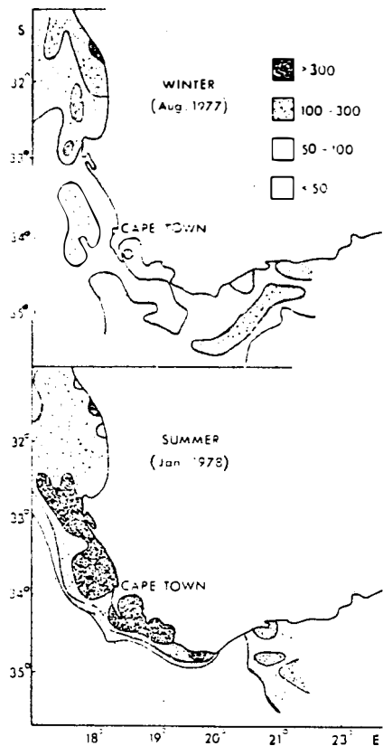
FIG. 8. — Distribution of phytoplankton biomass (mg chl a · m -2 from 0-50 metres) in the southern Benguela area during winter and summer.
