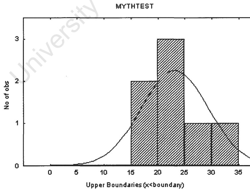
Figure 34: Histogram showing the learning scores for the non-VR participants. The solid curve indicates the expected normal.
