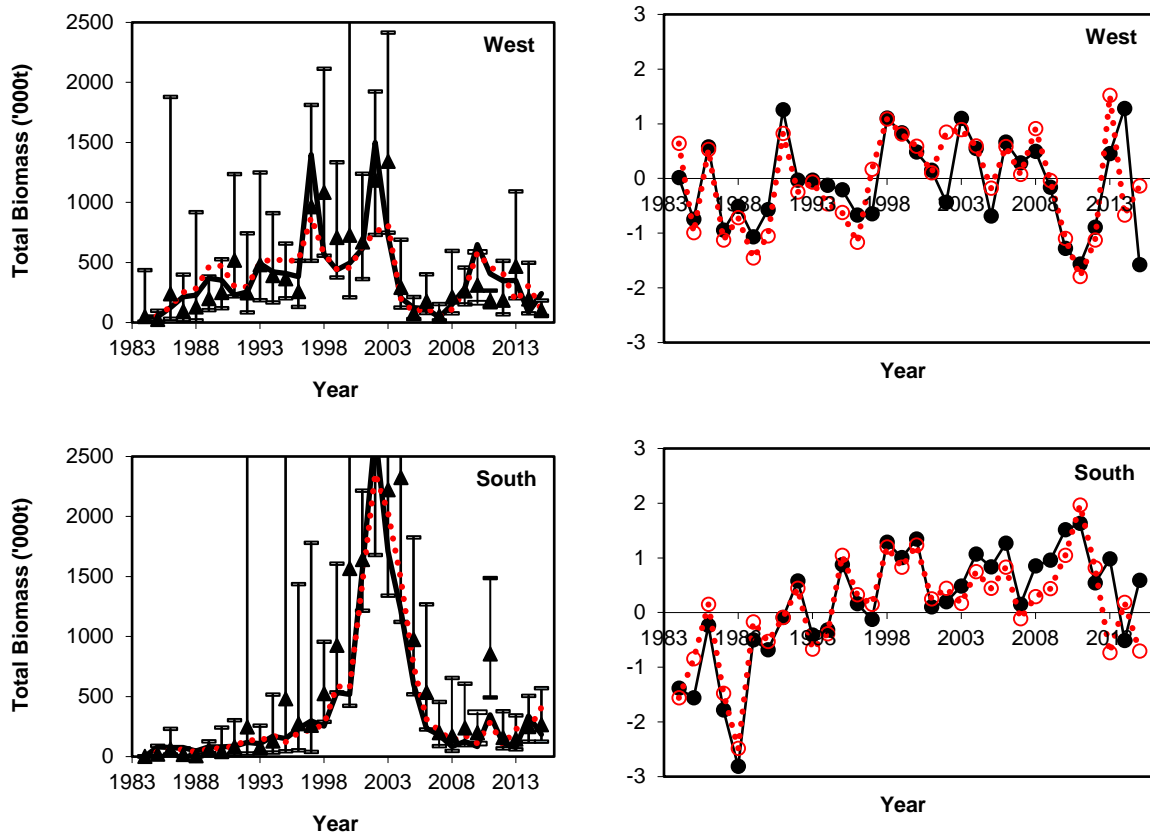
Figure 2. Acoustic survey estimated and model predicted November sardine 1+ biomass from 1984 to 2015 for the two mixing stock hypothesis fitted to parasite prevalence-by-length data east of 20°E (red dotted lines) and east of 22°E (black solid lines). The observed indices are shown with 95% confidence intervals. The standardised residuals from the fits are given in the right hand plots.
