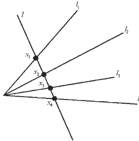
Figure 2.1: Cross-ratio of four lines: \{l_1, l_2, l_3, l_4\} = \{x_1, x_2, x_3, x_4\} . Figure obtained from [8].
