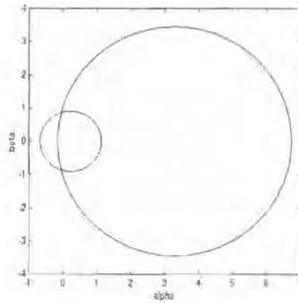
Figure 6.9: Constraint Circles.
