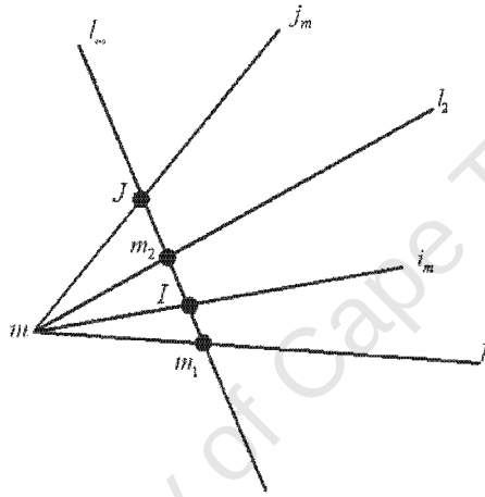
Figure 2.4: Illustration of the Laguerre formula in \mathcal{P}^2 . Figure obtained from [8, 9].
