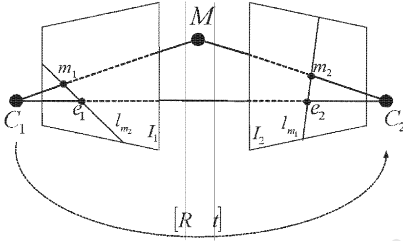
Figure 3.3: Epipolar Geometry.
