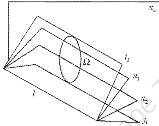
Figure 2.5: Illustration of the Laguerre formula in \mathcal{P}^3 . Figure obtained from [8].
