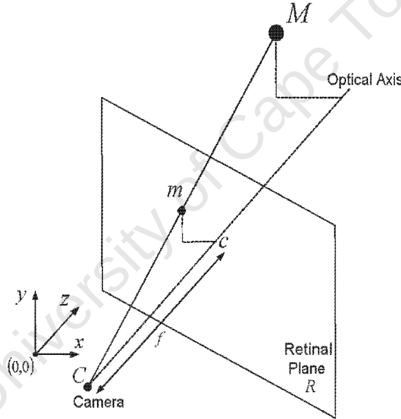
Figure 3.1: Perspective Projection.
