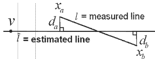
Figure B.1: Maximum Likelihood Estimate of Vanishing Point [28].
