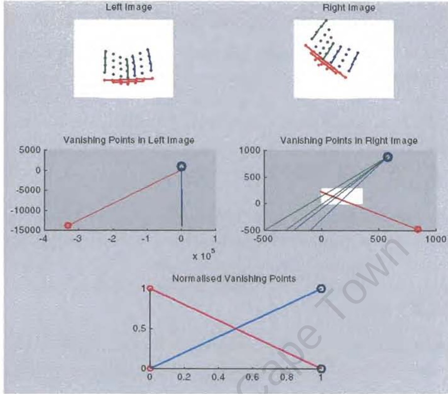
Figure 7.1: Synthetic corner illustrating the vanishing points.
