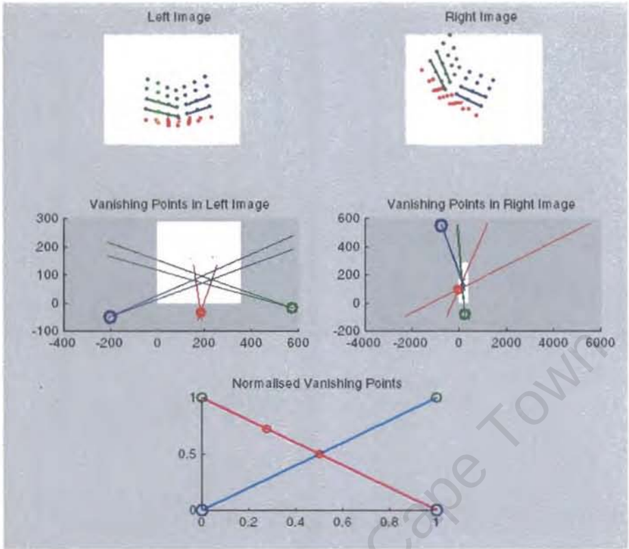
Figure 7.2: Vanishing points defining one line.
