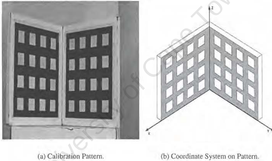
Figure 6.1: Common Calibration Pattern.
