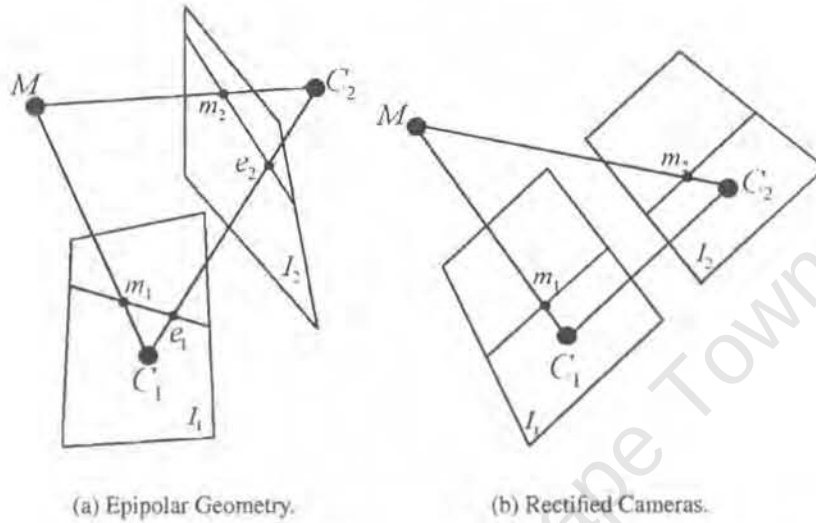
Figure 7.7: Rectification Process. Figure obtained from [13, 14].
