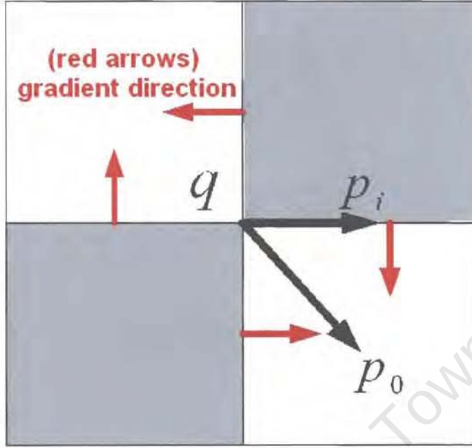
Figure A.1: Illustration of subpixel corner estimation (©2000 Intel Corporation).
