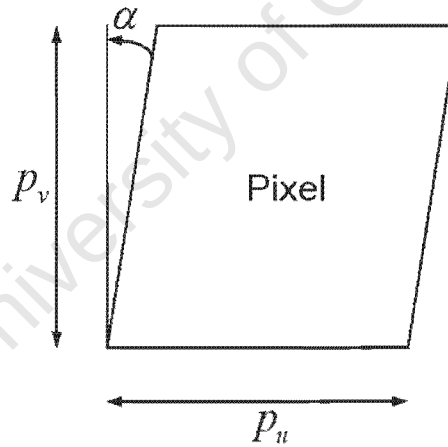
Figure 3.2: Illustration of pixel skew.
