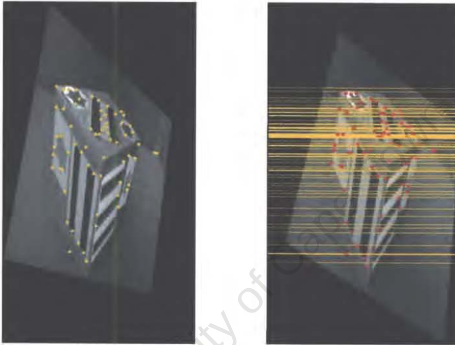
Figure 7.8: Rectified stereo image pair with horizontal epipolar lines.
