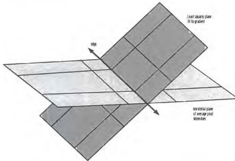
Figure A.3: Two planes intersecting in a straight line. Figure obtained from [4].
