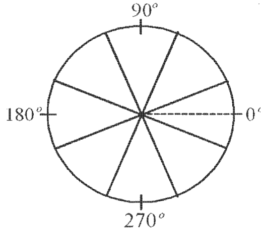
Figure A.2: Gradient Space Partitioning. Figure obtained from [4].
