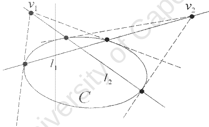
Figure 2.2: Points v_1 and v_2 , with polars l_1 and l_2 . The points v_1 and v_2 are conjugate with respect to the conic C . Figure obtained from [29].
