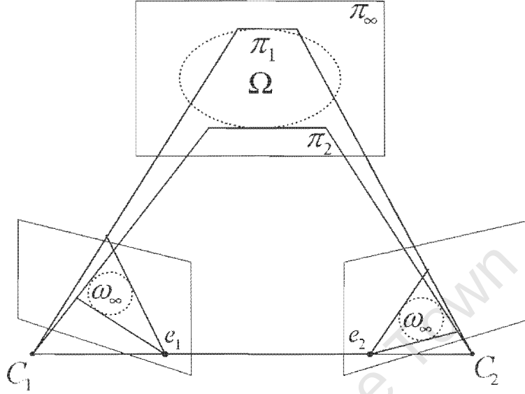
Figure 6.3: The Image of the Absolute Conic.
