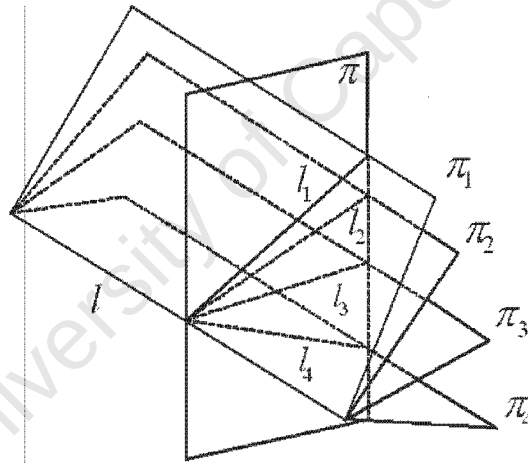
Figure 2.3: Cross-ratio of four planes: \{\pi_1, \pi_2; \pi_3, \pi_4\} = \{l_1, l_2; l_3, l_4\} . Figure obtained from [8].
