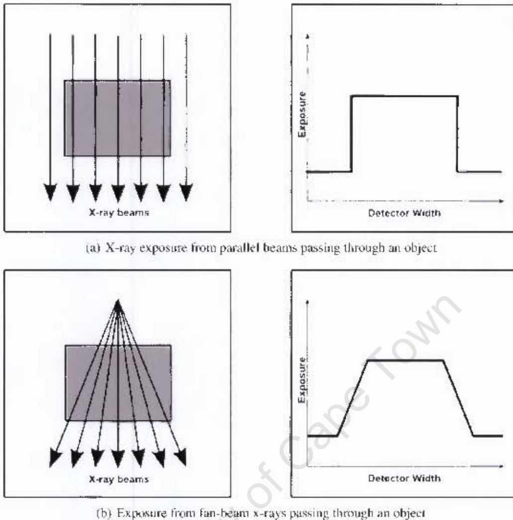
Figure 1: Comparing the exposure of parallel beam and fan beam x-rays passing through equivalent objects.
