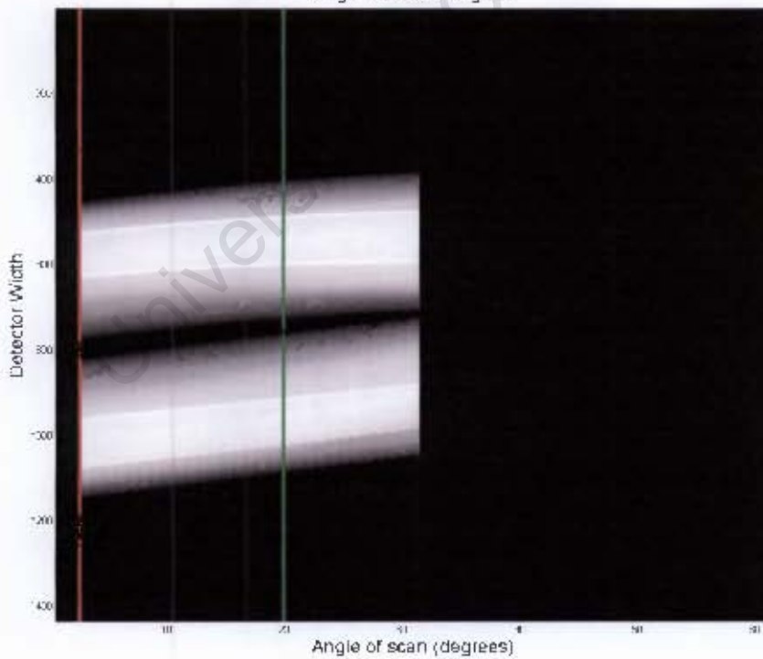
Figure 37: Sinogram constructed from knee scans with lines at corresponding angles highlighted.
