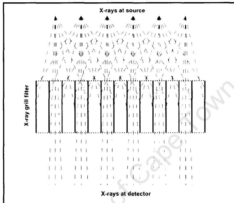
Figure 23: X-ray grill filtering out non-parallel x-ray beams.
