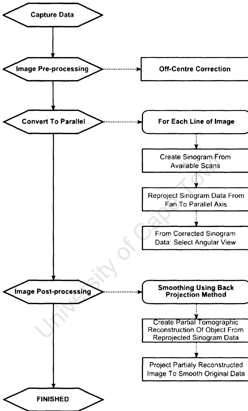
Figure 44: Flowchart of Implementation Steps.
