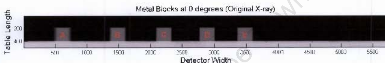
Figure 46: X-ray image of calibrated metal blocks taken at 0^\circ rotation
