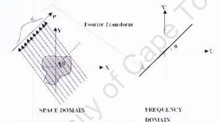
Figure 8: Illustration of the Fourier Slice Theorem.
