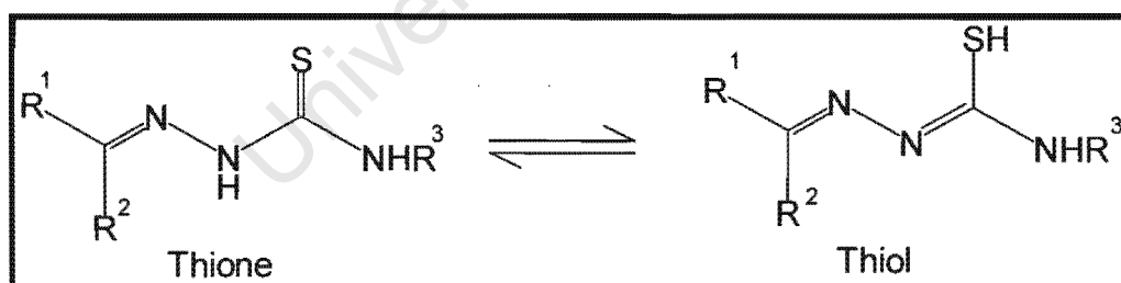
Figure 2 - 11: Thione and thiol tautomers of thiosemicarbazones
