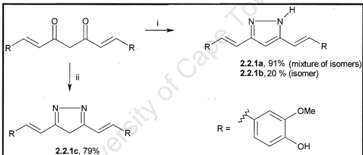
Scheme 2 - 1: Reagents and conditions i) \text{NH}_2\text{NH}_2 , acetic acid, rt, 72 h; ii) \text{NH}_2\text{NH}_2 , NaOH, EtOH, 65°C, 15 min.
