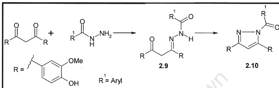
Figure 2 - 15: Aryl hydrazone methanone (2.9) and pyrazole-1-methanone (2.10) derivatives of curcumin.
