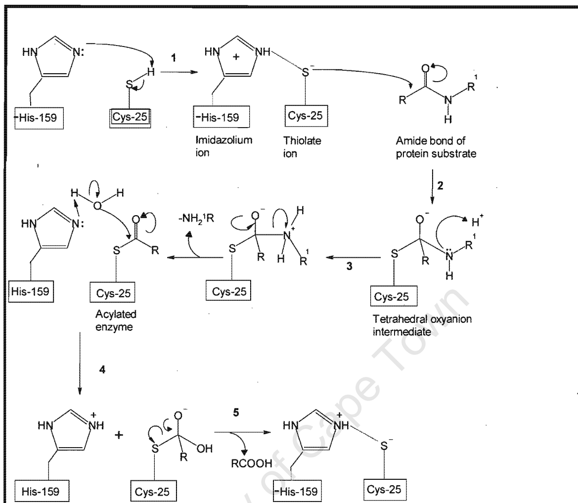
Figure 1 - 16: Mechanism of proteolysis by cysteine proteases 138, 152
