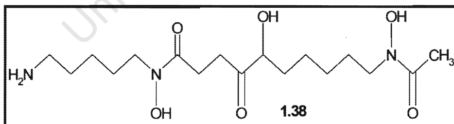
Figure 1 - 19: Chemical structure of desferrioxamine (1.38).
