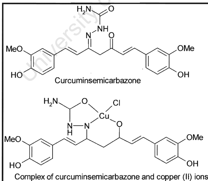
Figure 2 - 14: Structure of curcuminsemicarbazone and its copper complex 49
