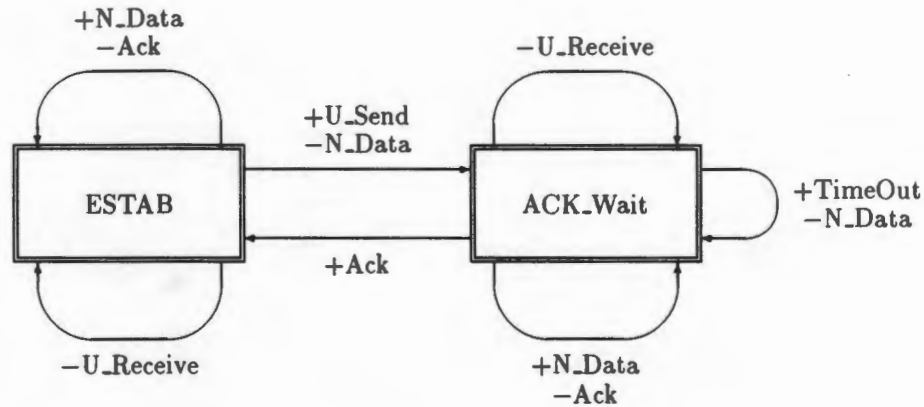
Figure 19: Combined and reduced AB-protocol FSM
