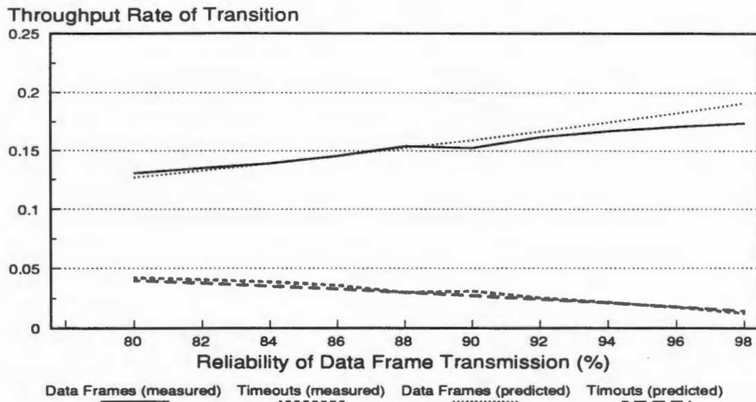
Figure 22: Measured and Predicted Values (Poisson Delays)
