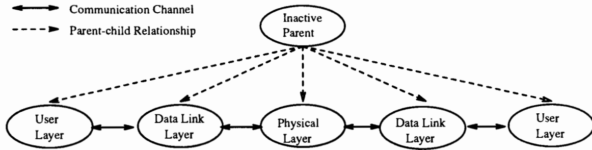
Figure 2: The Process Structure of a Three-Layer Point-to-Point Communication System
