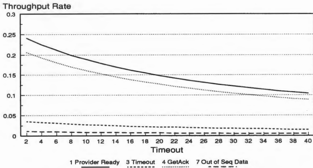
Figure 29: Selected Predicted Transition Throughputs (Constant Delays)
