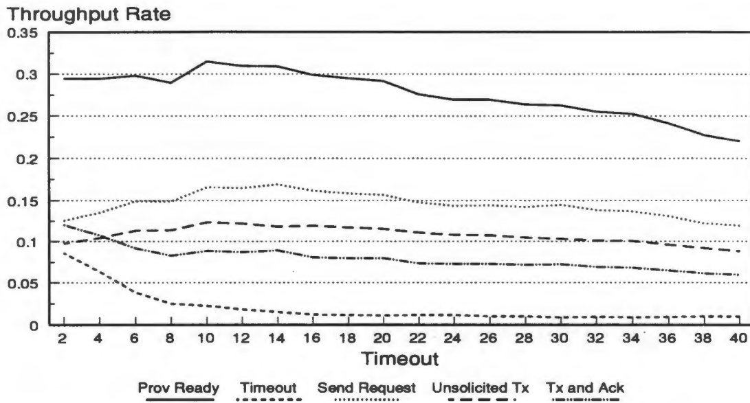
Figure 31: Measured Transition Throughputs for Loopback SLAP Protocol using Poisson Provider Delays
