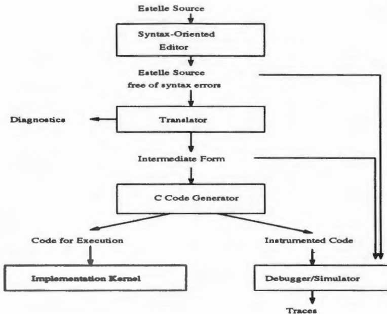
Figure 17: Architecture of the EDT System
