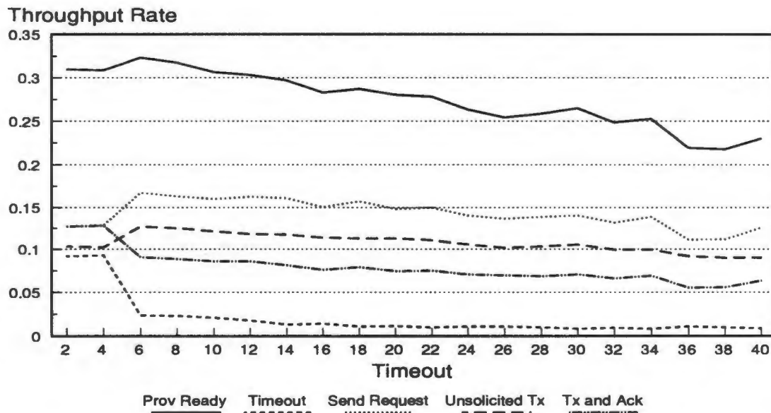
Figure 32: Measured Transition Throughputs for Loopback SLAP Protocol using Constant Provider Delays
