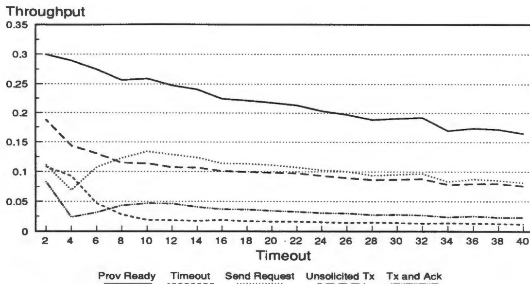
Figure 34: Measured Throughputs of Selected Transitions in SLAP Protocol
