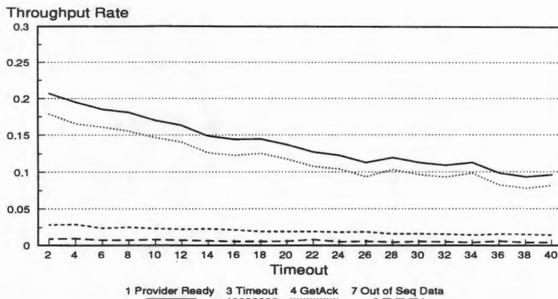
Figure 27: Selected Measured Transition Throughputs (Poisson Delays)
