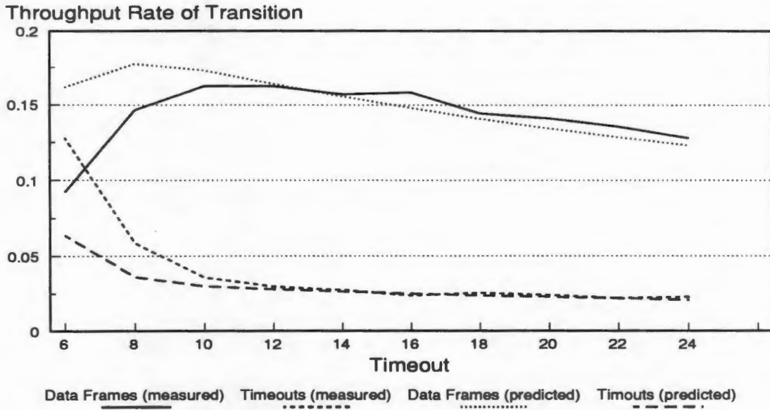
Figure 23: Measured and Predicted Values (Exponential Delays)
