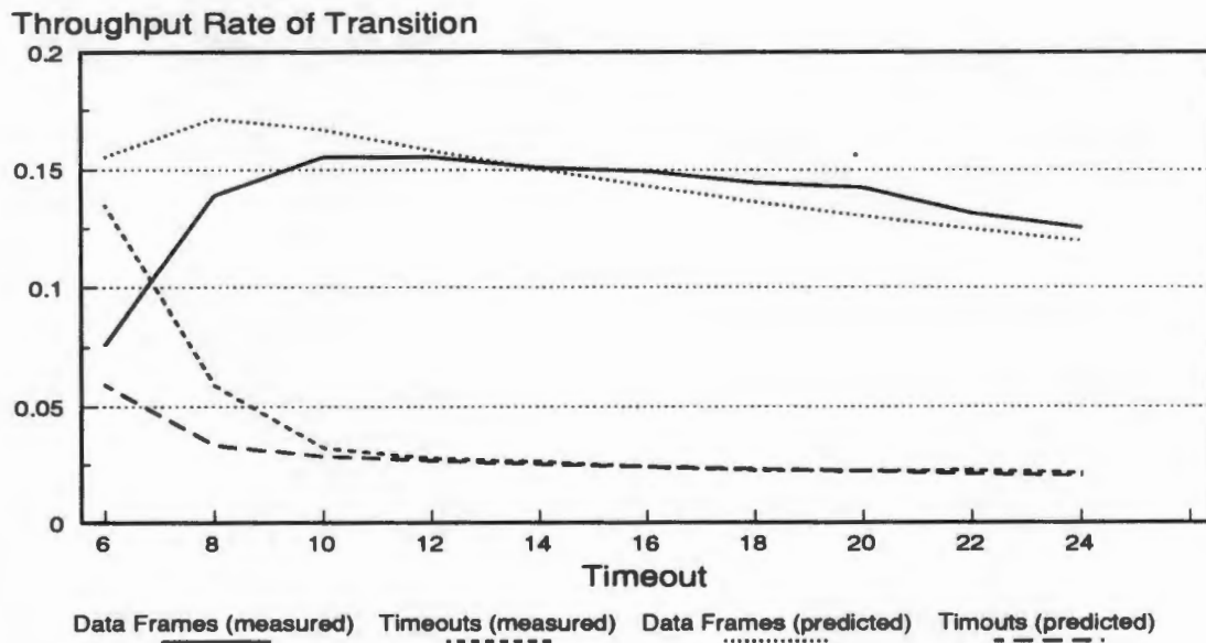
Figure 24: Measured and Predicted Values (Poisson Delays)
