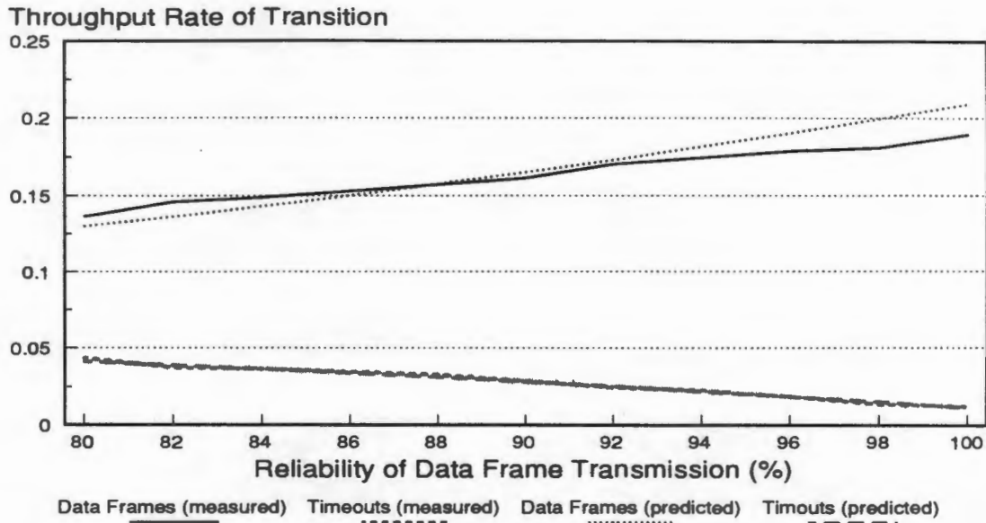
Figure 21: Measured and Predicted Values (Exponential Delays)
