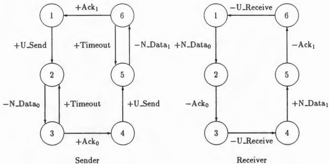
Figure 18: AB-protocol Send and Receive FSMs
