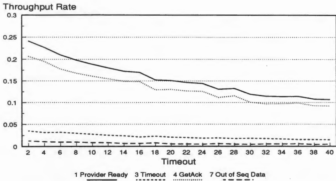
Figure 28: Selected Measured Transition Throughputs (Constant Delays)
