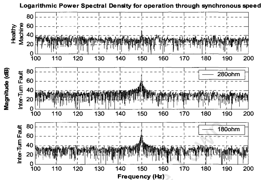
Figure 5.8: Spectrum of stator currents for operation through synchronous operation
