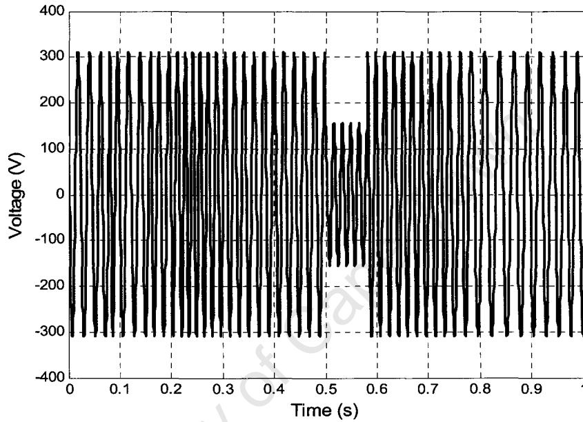
Figure 6.4: Supply voltage
