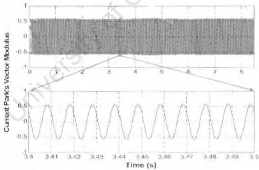
Figure 5.17: Magnified fault sinusoid for the greater fault condition
