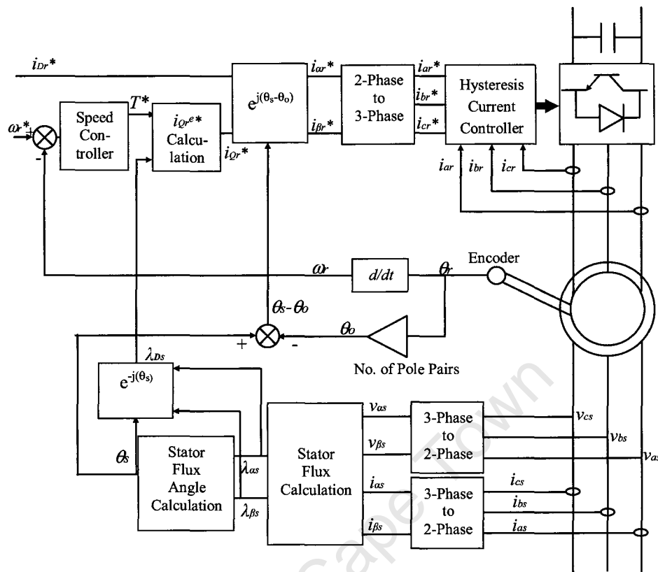
Fig. 5.4: Schematic of vector control for the rotor-side converter
