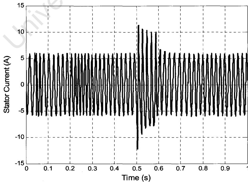
Figure 6.5: Stator current
