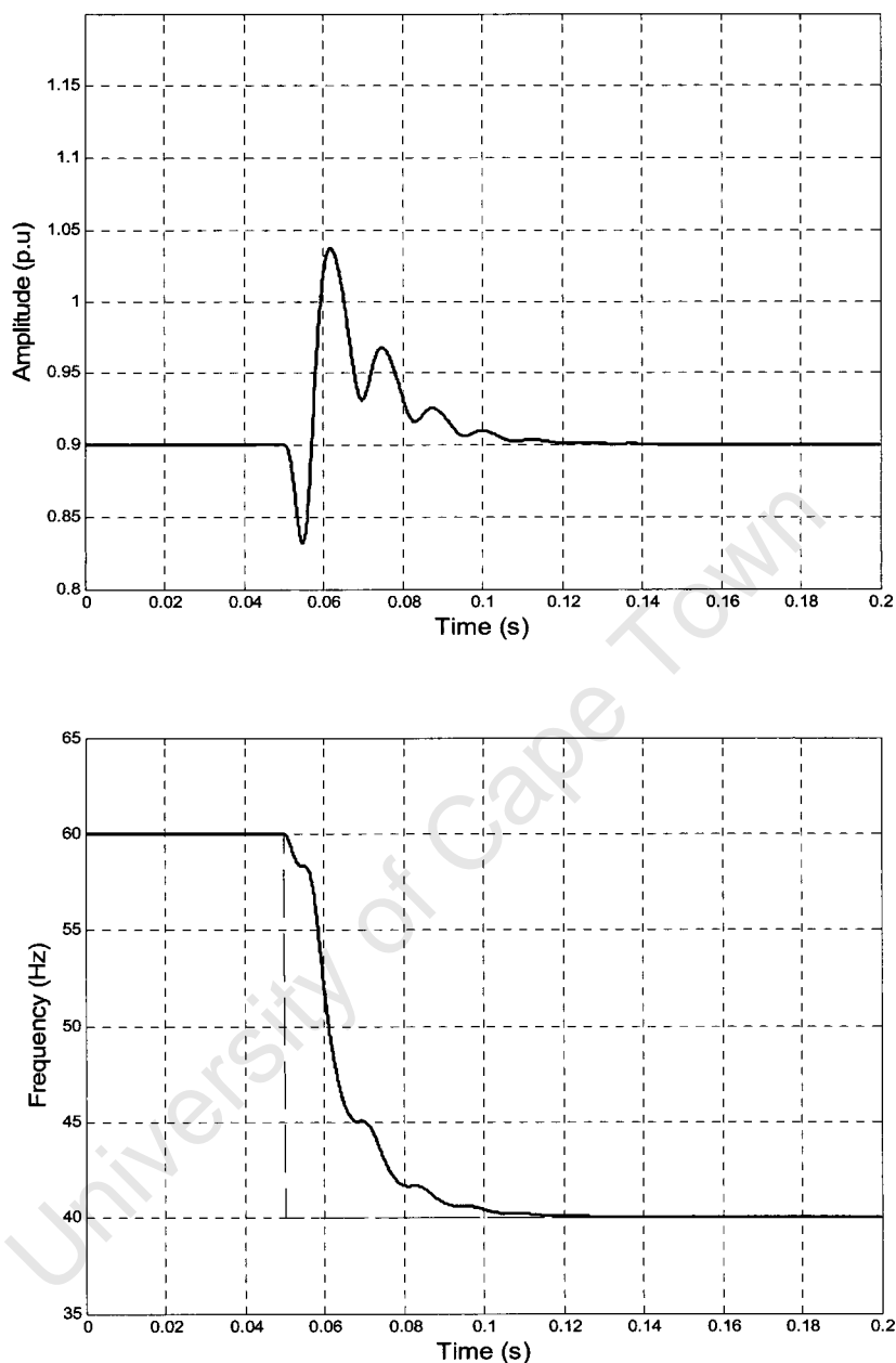
Figure 2.6: Frequency-locking property of the algorithm
