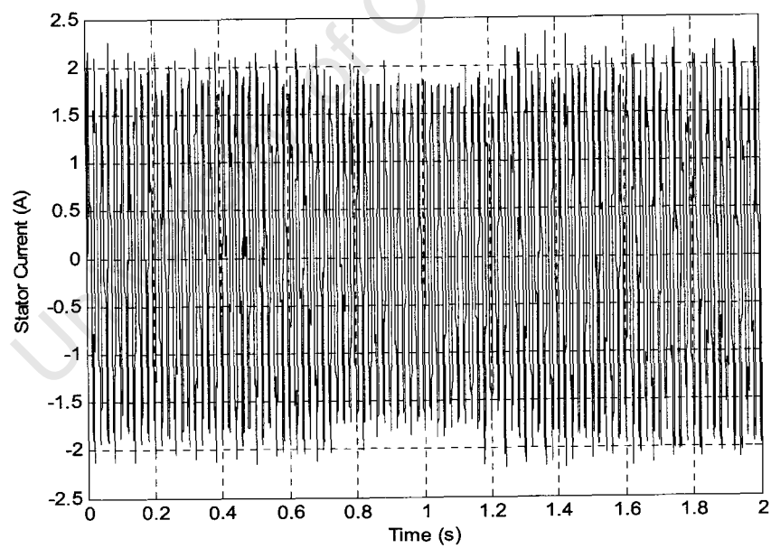
Figure 6.18: Stator current
