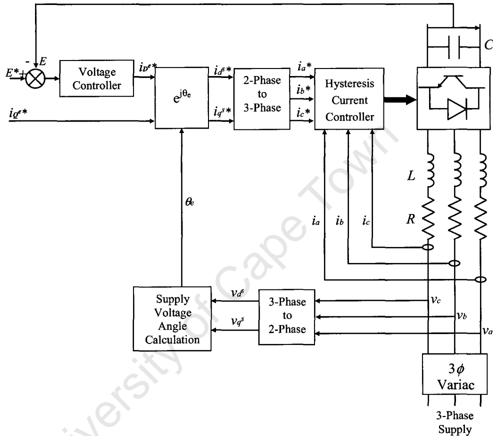
Figure 5.3: Schematic of vector control for the supply-side converter
