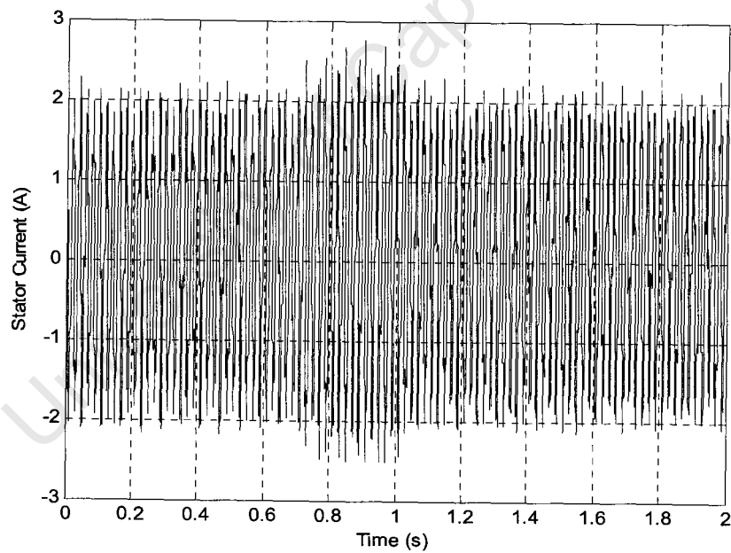
Figure 6.13: Stator current
