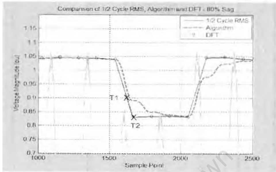
Figure 6.2: T1 shows that the algorithm is able to detect the sag much faster than the \frac{1}{2} cycle RMS and DFT methods
