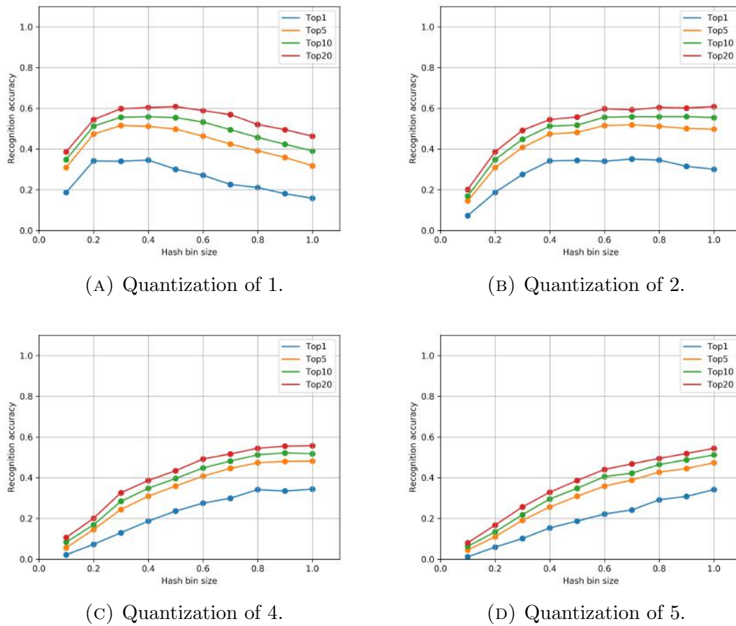
FIGURE 5.10: Results of different quantization values for projective transformation and non-probabilistic voting technique.
