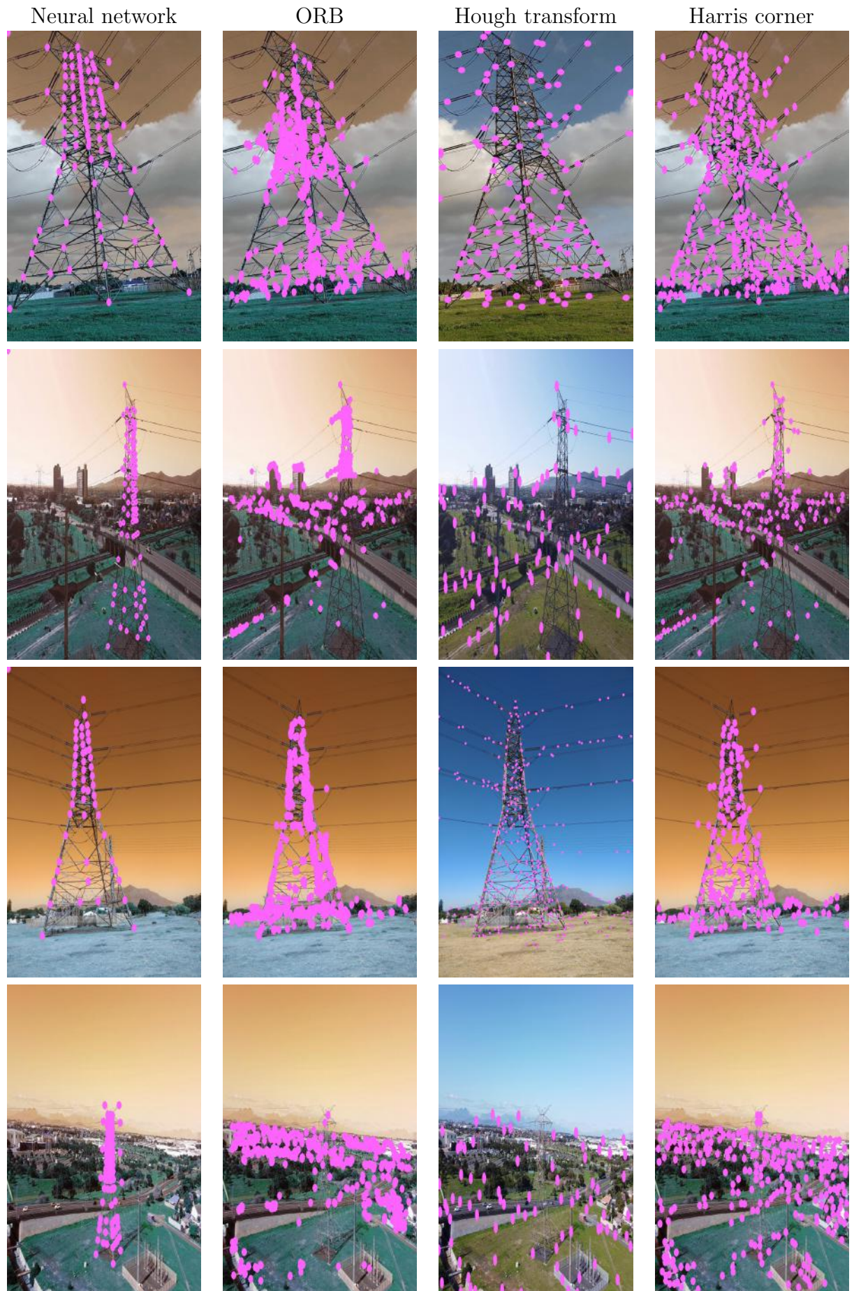
FIGURE 4.14: Detection of vertices using different techniques.
