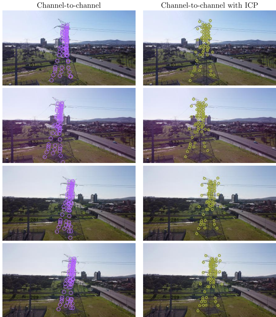
FIGURE 6.26: Results of the 3D model of the pylon registering onto the image of the pylon with channel-to-channel as the means for data association .
