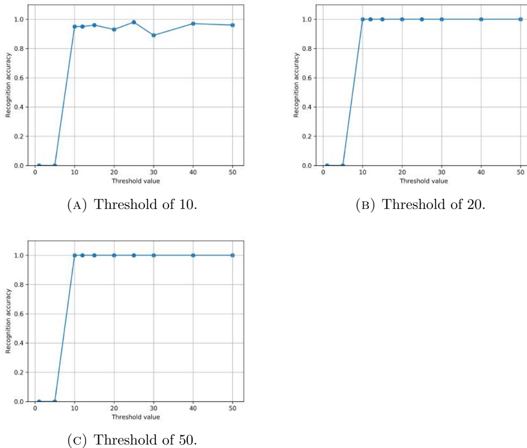
FIGURE 5.12: Set of experiments with different threshold values.
