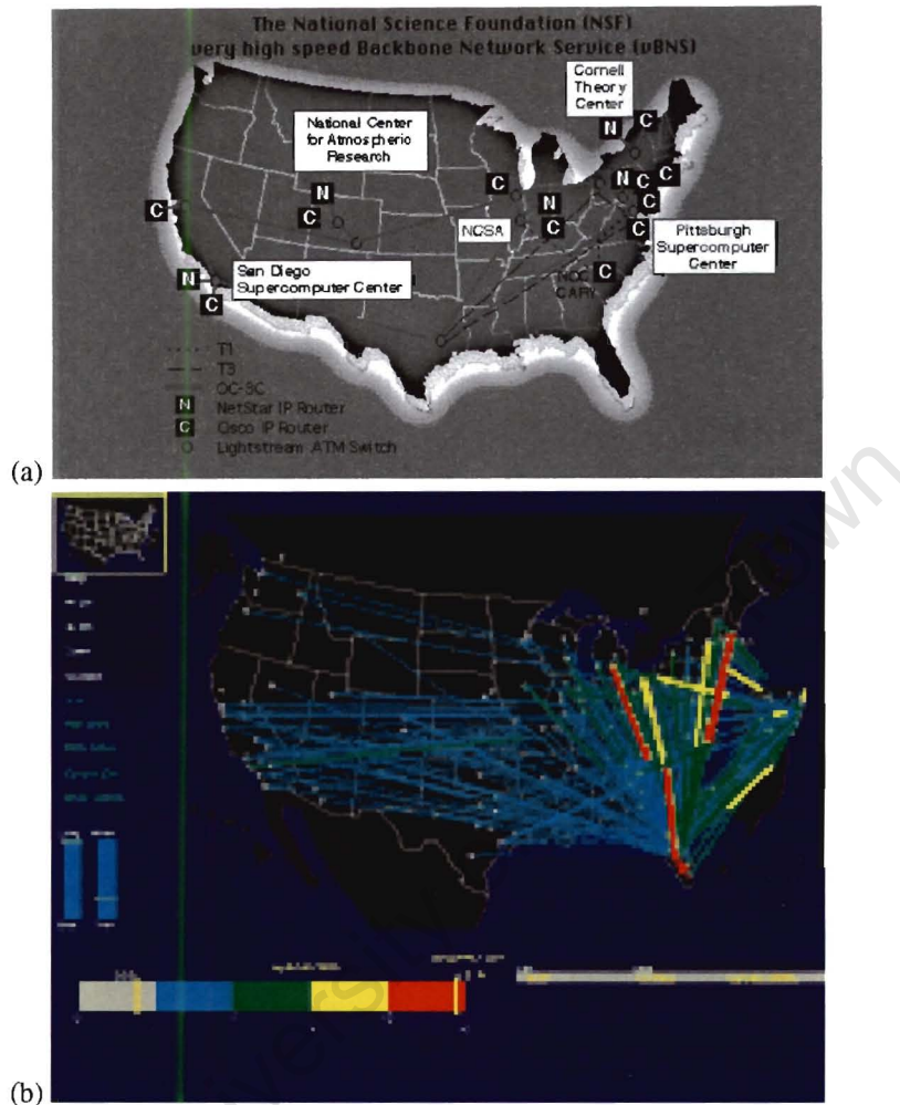
Figure 28: (a) Uncluttered network map : this metaphor works well for sparse static networks with few routes. It uses a geographic node placement algorithm where nodes corresponds to major cities in the US. (b) Cluttered network map : this network map shows the traffic on Christmas day 1994. This map was generated by the SeeNet software. It is evident that a links overlap particularly on the right side of the network map along the western US seaboard. This cluttering makes identifying interesting or abnormal network conditions difficult. Overall network context is maintained by the image in the top left hand corner.
