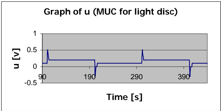
Figure AP6.3 Input signal ( u ) for heavy and light disc models
