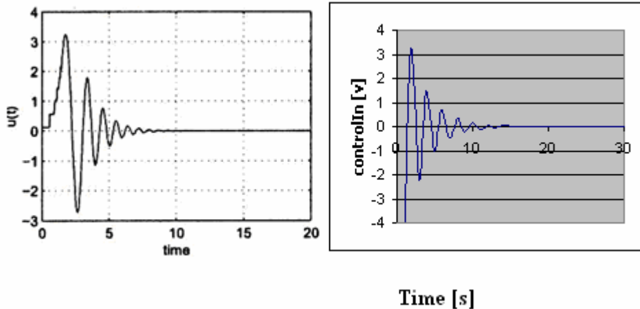
Figure 5.6 The MUC control input, u (Left graph from [23])
