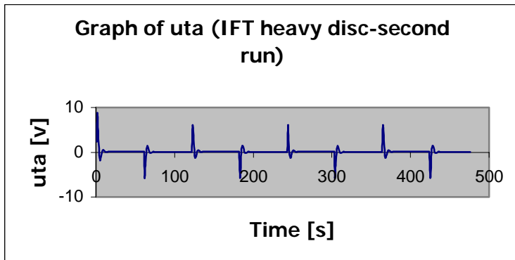
Figure AP6.1 Input signal ( u_{ta} ) for heavy disc model
