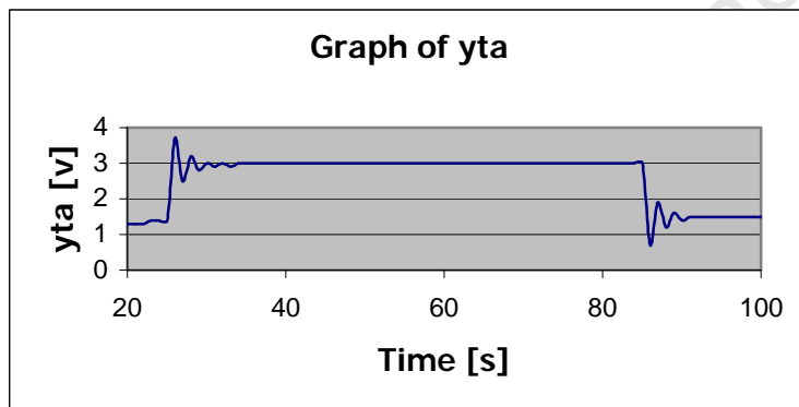
Figure 6.7 IFT DC Motor (light disc) output response, y_{ta}
