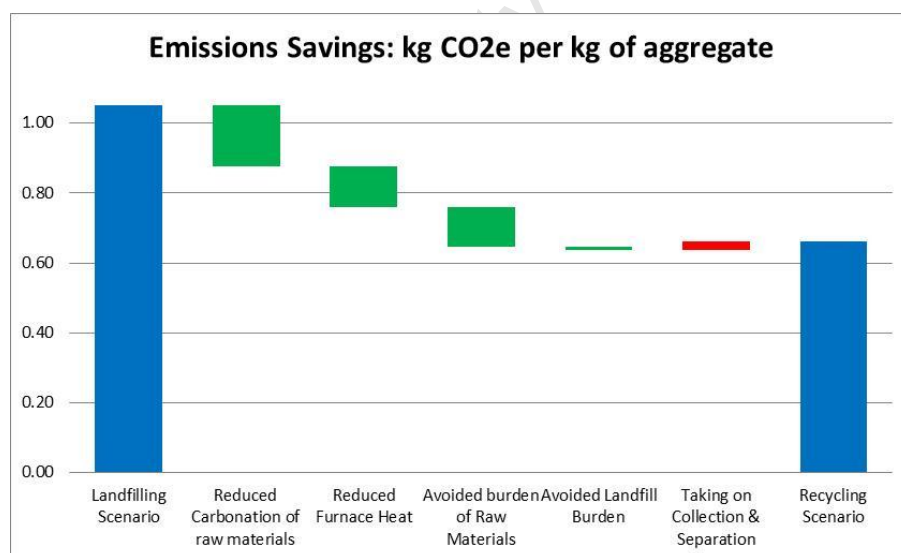
Figure 33: Bridging the GWP Difference between Recycling and Landfilling
