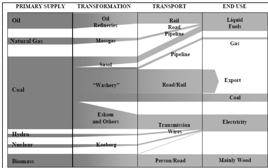
Figure 3: South Africa's Energy Supply Flow (Department of Minerals and Energy, 2003)
