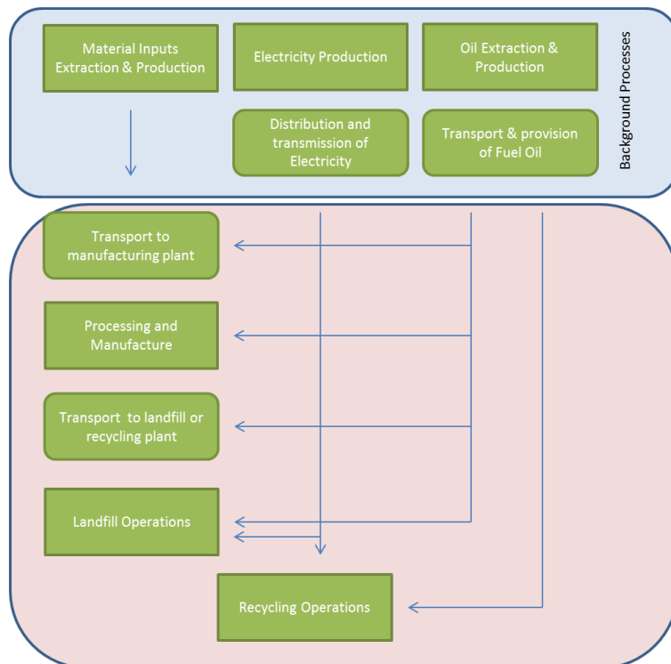
Figure 19: Foreground and Background Processes
