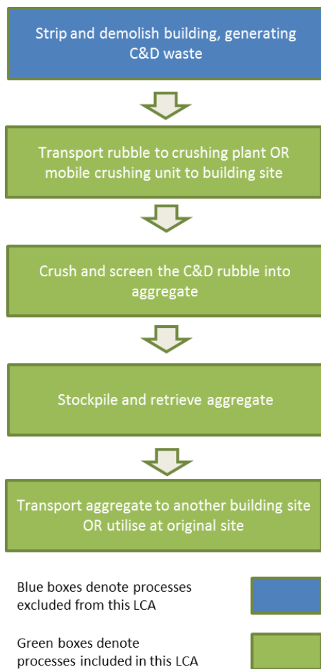
Figure 12: Life Cycle Process for Recycled Aggregate
