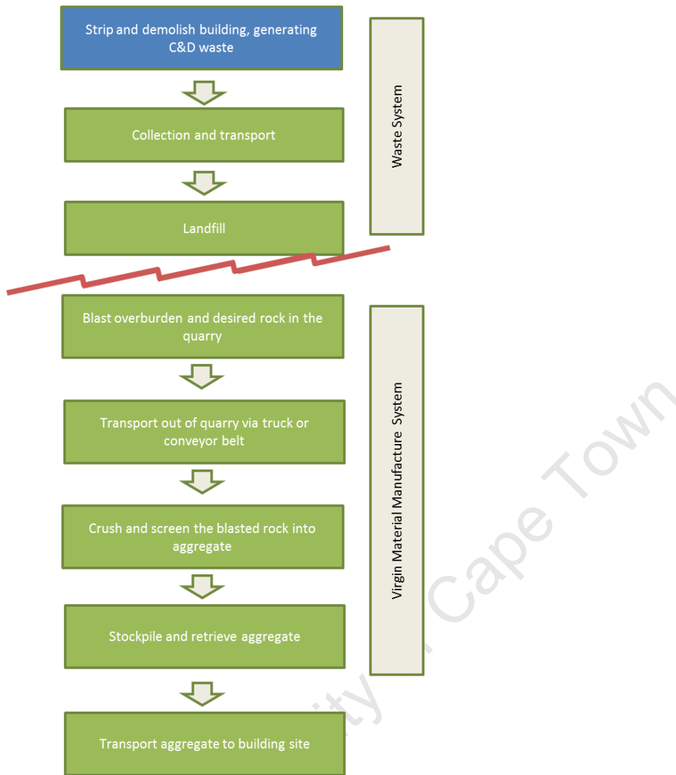
Figure 14: Life Cycle Stages of Landfilling C&D Waste and Producing Aggregate from Raw Material
