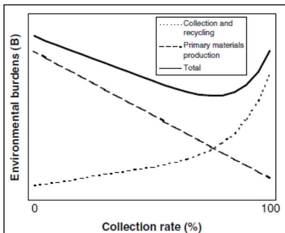
Figure 35: The Non-linear Relationship between Burden and Collection Rate
