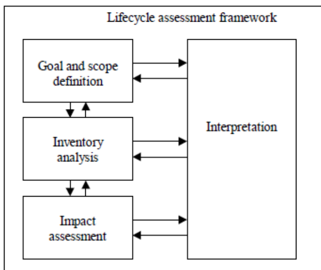
Figure 10: Life Cycle Assessment Framework (ISO, 2006)
