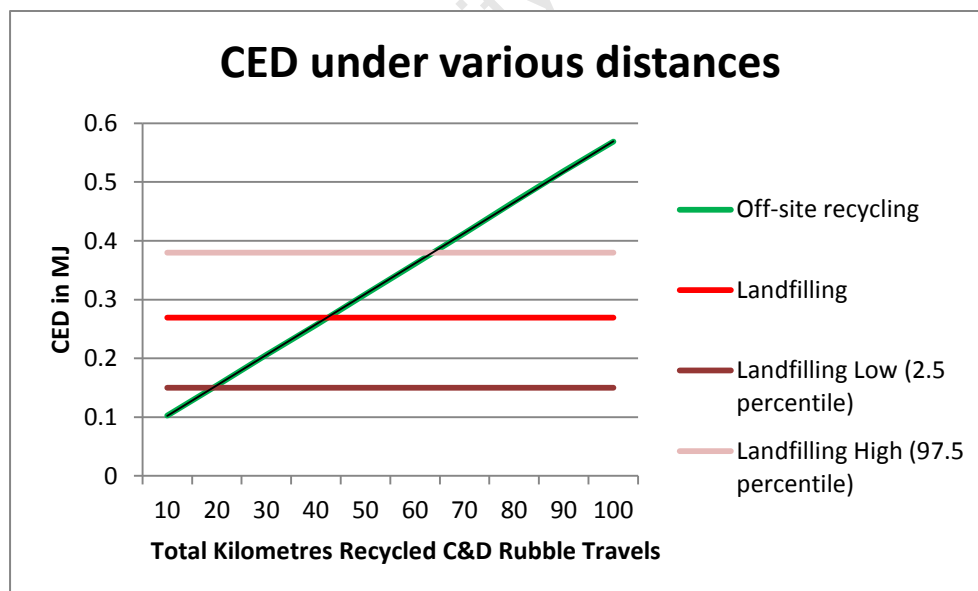
Figure 26: The Effect of Transportation Distance on C&D Waste Recycling
