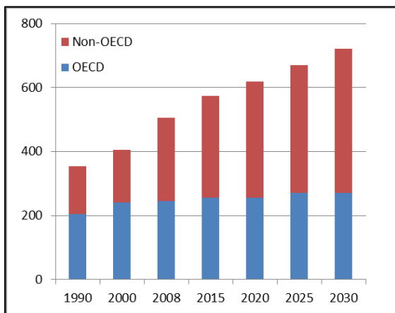
Figure 1: World Energy Consumption (Quadrillion Btu) (U.S. EIA, 2011)
