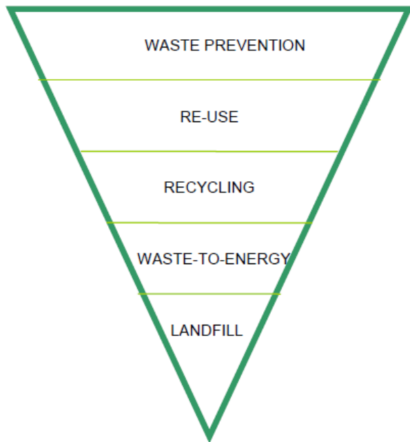
Figure 5: The Waste Hierarchy (UNEP, 2010b)
