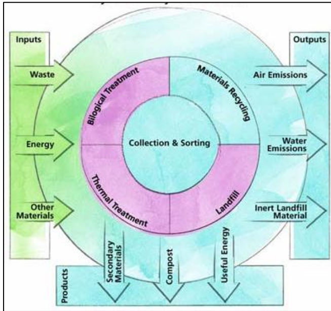
Figure 11: System Boundaries for LCI of Solid Waste (P&G, UK, 2011)
