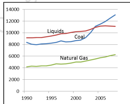
Figure 2: World CO 2 Emissions (Million tonnes) (U.S. EIA, 2011)
