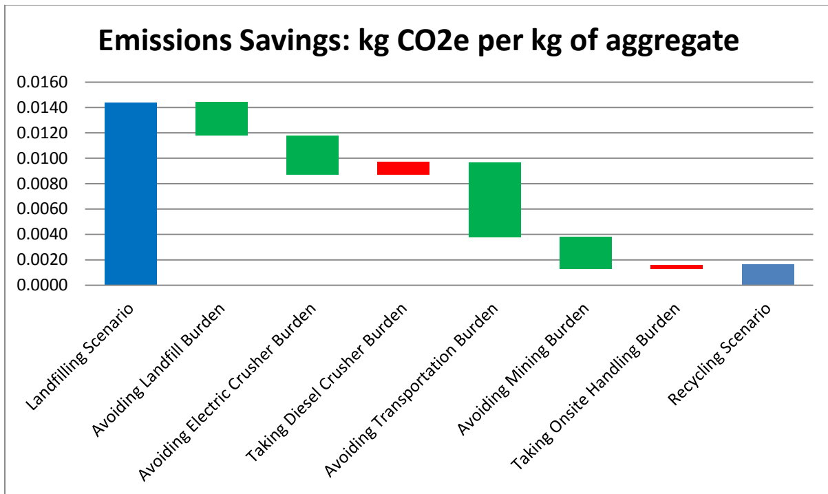
Figure 25: Bridging the GWP Difference between Recycling Onsite and Landfilling
