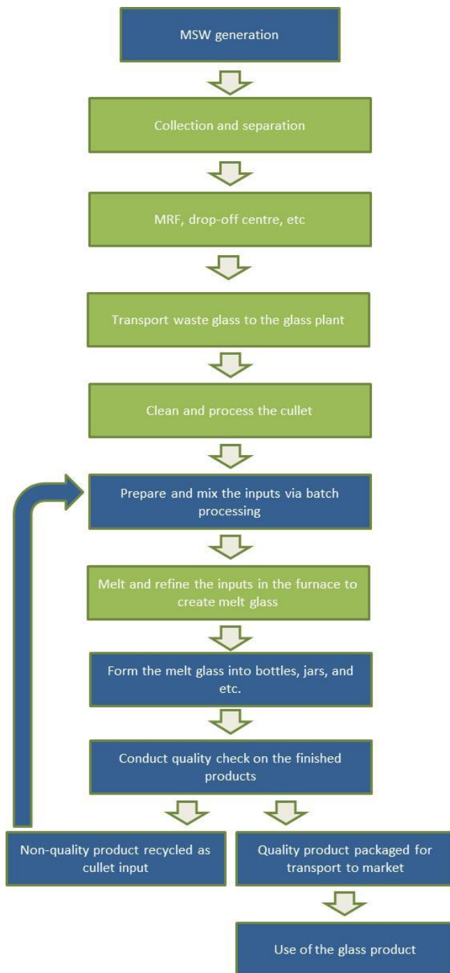
Figure 16: Life Cycle of Recycled Container Glass
