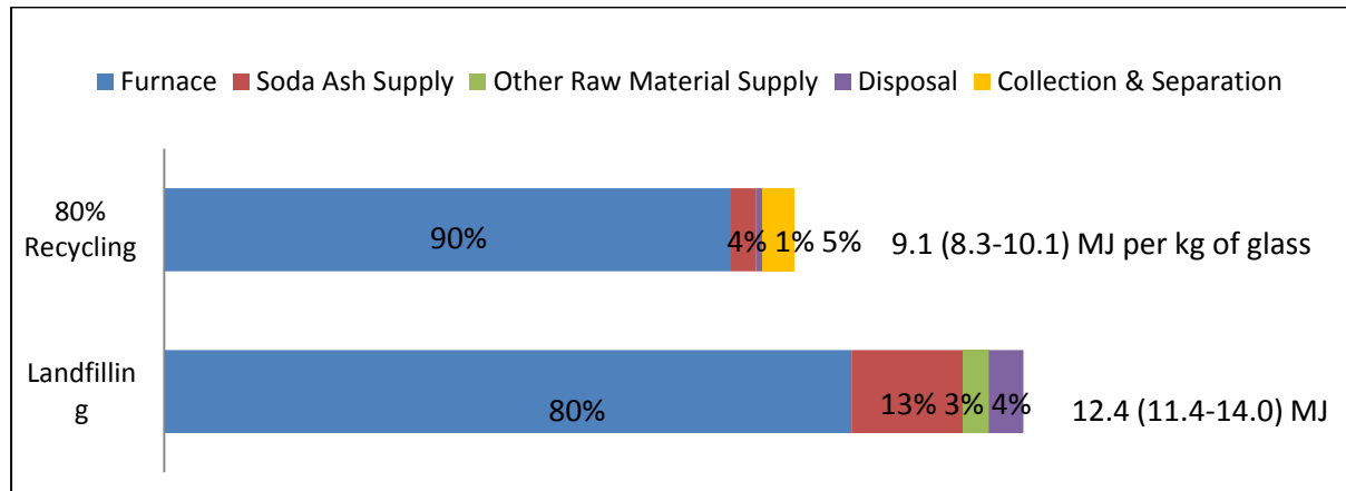
Figure 29: CED Process Contributions for Container Glass Scenarios
