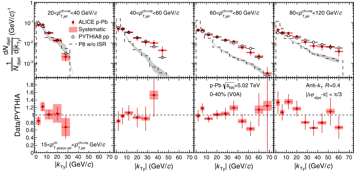
Fig. 1. Dijet |k_{Ty}| distributions in p-Pb collisions in the 0–40% V0A multiplicity event class for several kinematic intervals of the full jet ( p_{T,jet}^{ch+ne} ). The measurement is compared to PYTHIA8 (tune 4C, K = 0.7 ) with and without initial state radiation. The lower panels show the ratio between the measurement and PYTHIA8 including initial state radiation.
