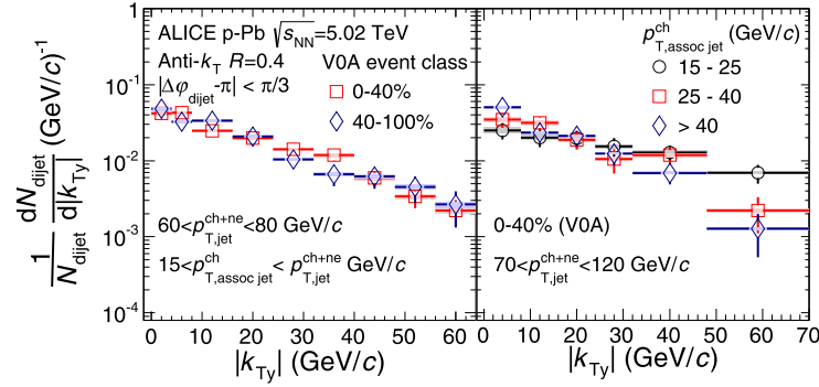
Fig. 2. Distributions of |k_{Ty}| for two V0A event classes (left panel) and three p_{T,\text{assoc jet}}^{\text{ch}} ranges (right panel).
