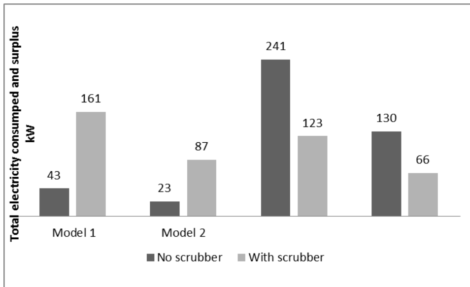
Figure 4-5: Influence of upgrading biogas on electricity consumption
