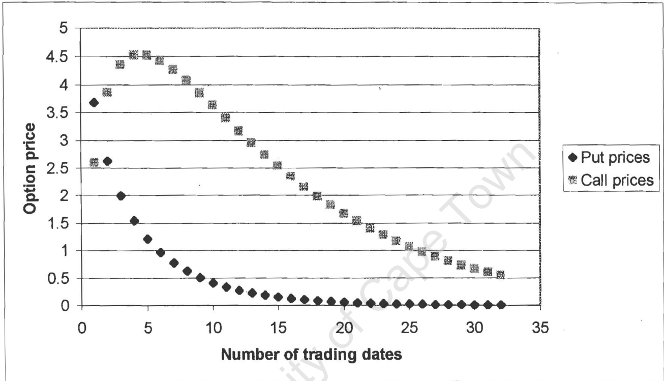
Figure A.3: European call and put option prices with strike 100, expiry 1, on a stock with initial price 100 and volatility 10%, priced using the trinomial tree method with increasing numbers of trading dates.
