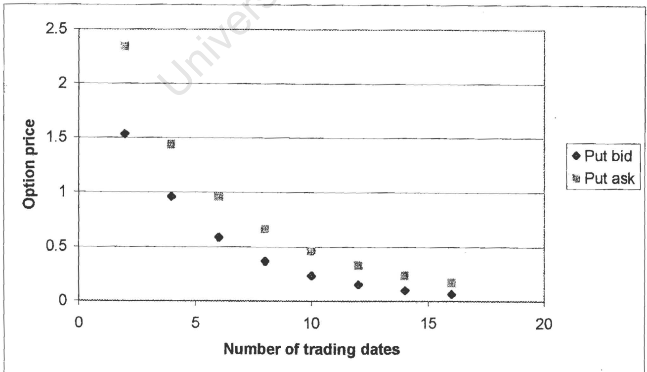
Figure A.5: The bid and ask prices for a European put option with strike 100 on a stock with volatility 10%
