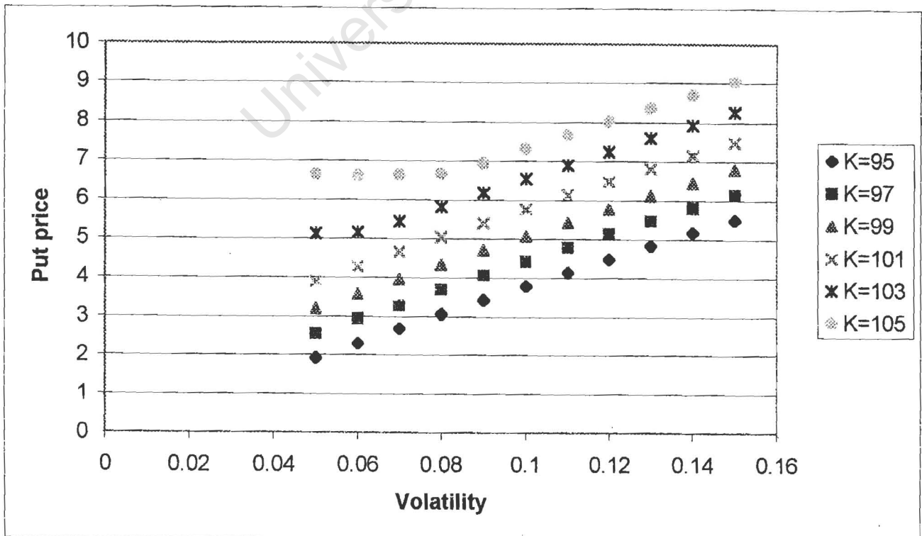
Figure A.2: Trinomial model prices for a European put option with varying strike on a stock with varying volatility
