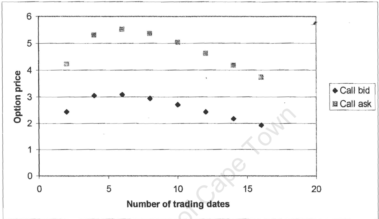
Figure A.4: The bid and ask prices for a European call option with strike 100 on a stock with volatility 10%
