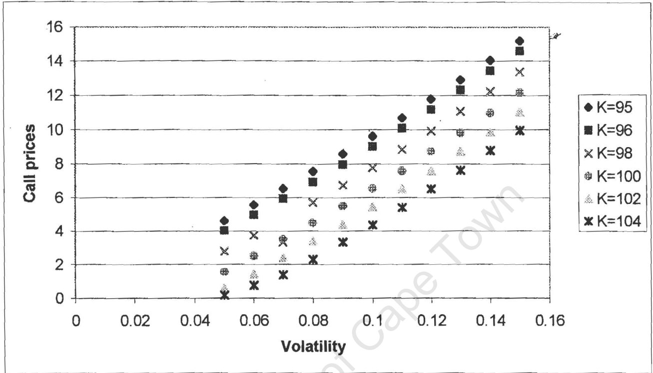
Figure A.1: Trinomial model prices for a European call option with varying strike on a stock with varying volatility
