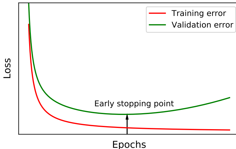
Figure 4.10: Demonstration of early stopping in practice.
