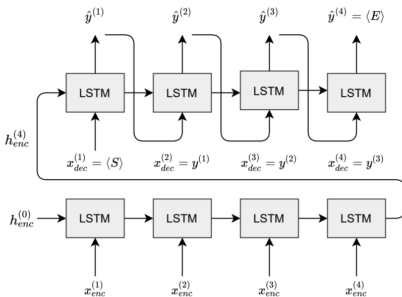
Figure 4.8: Encoder-decoder RNN.
