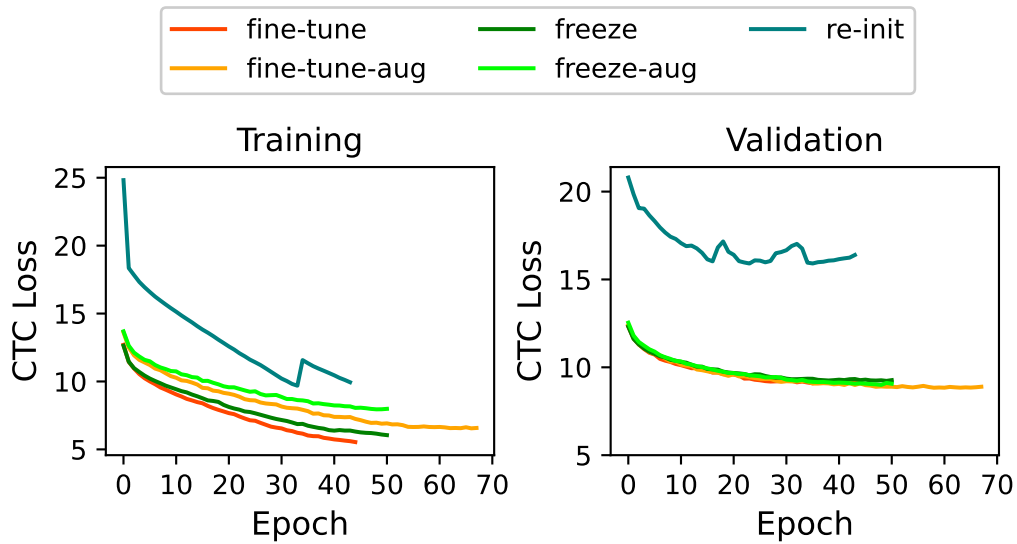
Figure 5.1: Training and validation CTC loss as a function of epoch for the Deep Speech based models.
