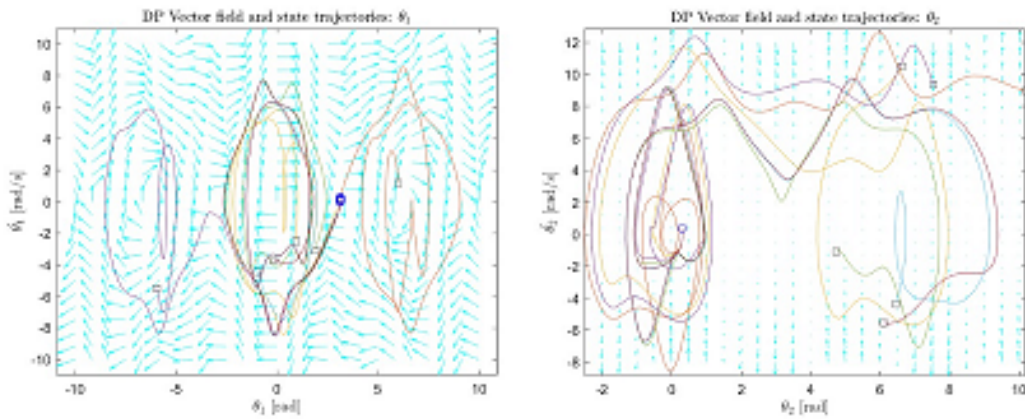
Figure 16: Illustrative phase state diagrams for the double pendulum model with the associated vector fields (shown as the cyan coloured arrows). The generalised coordinates of the position of the top and lower point masses are \theta_1 and \theta_2 respectively. Investigations were done using this model to provide simulated data for a two link serial planar mechanism, however this work did not fall within the scope of this project.
