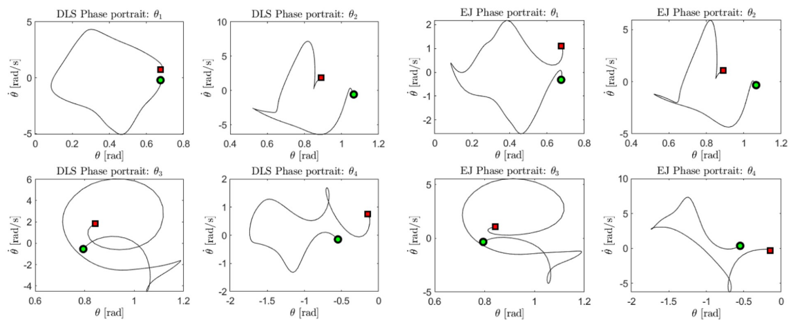
Figure 76: Joint trajectory estimates in \theta phase space by the gradient projection method.
