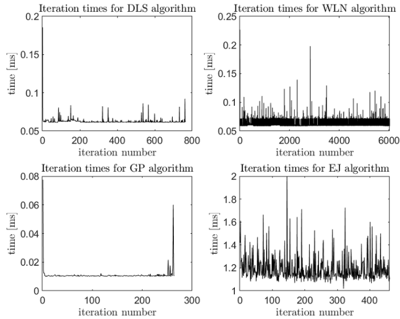
Figure 60: The iteration times for all of the IK models.
