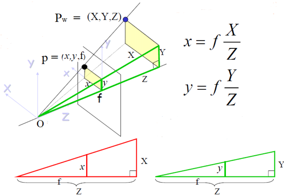
Figure 3: The simple linear geometry that is fundamental in obtaining the image coordinates of a point in space.
