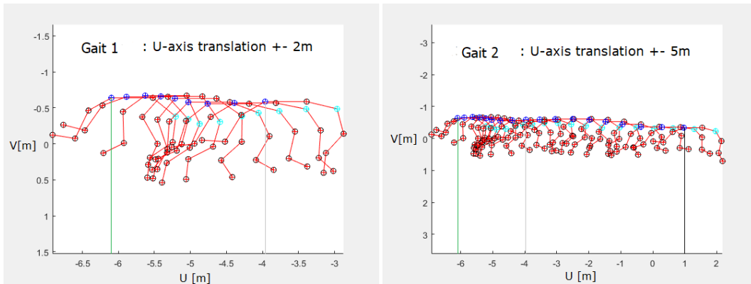
Figure 44: The composite side views of the quadruped for the first gait (left) and the first two gaits (right) in its local UVW coordinate system. The reference joints observer coordinates have been included so the origin of the UVW shows the corresponding shift.
