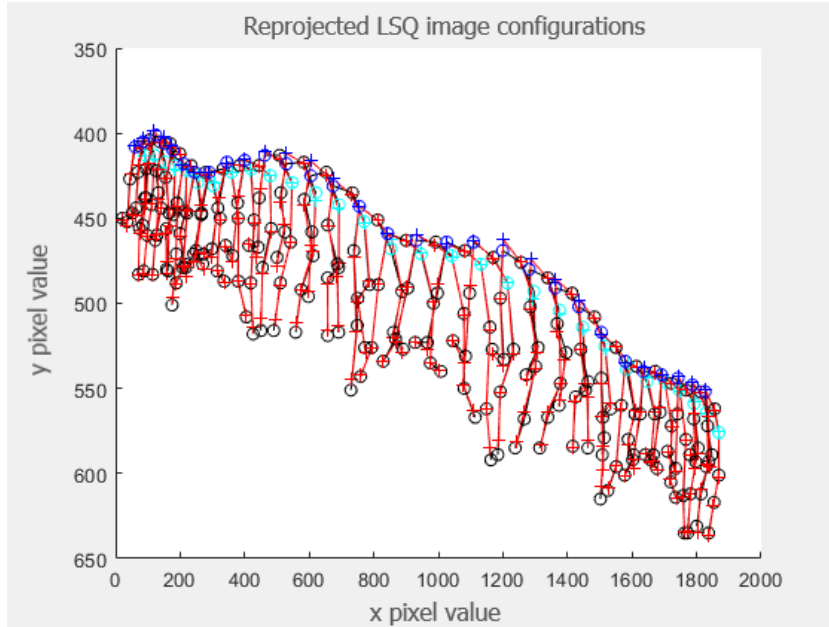
Figure 43: A composite graphic of the estimated reprojected images in pixel coordinates. The estimated 3D poses by the solver are input into the camera model to give each of the pixelated configurations.
