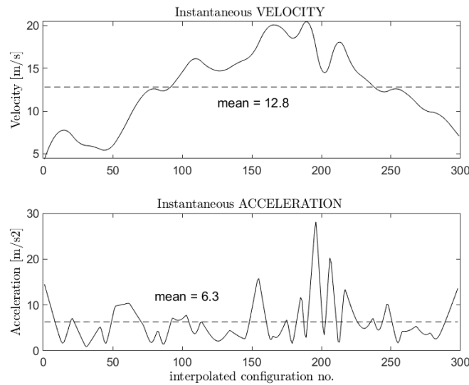
Figure 45: The magnitude of the velocity and acceleration of the reference joint. All three linear motion components were calculated from its position data and interpolated and using the higher sample rate the linear velocity and accelerations were obtained.
