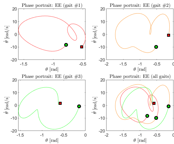
Figure 68: The phase states of the joint angle of the end effector link of the front leg as determined by the solver. Three gait cycles have been isolated here and the full cycle (lower right) shows convergence to a limit cycle.
