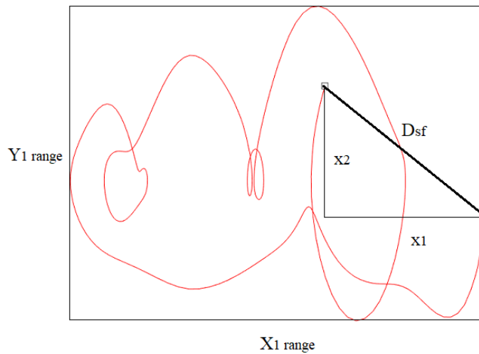
Figure 17: The diagram describing the parameter D_{sf} metric for state trajectory closure. Y1 relates angular rates for the given angle domain X1 for the state space of a particular variable. The distance between the start (circle) and end (square) points indicates the degree of closure of an orbital path.
