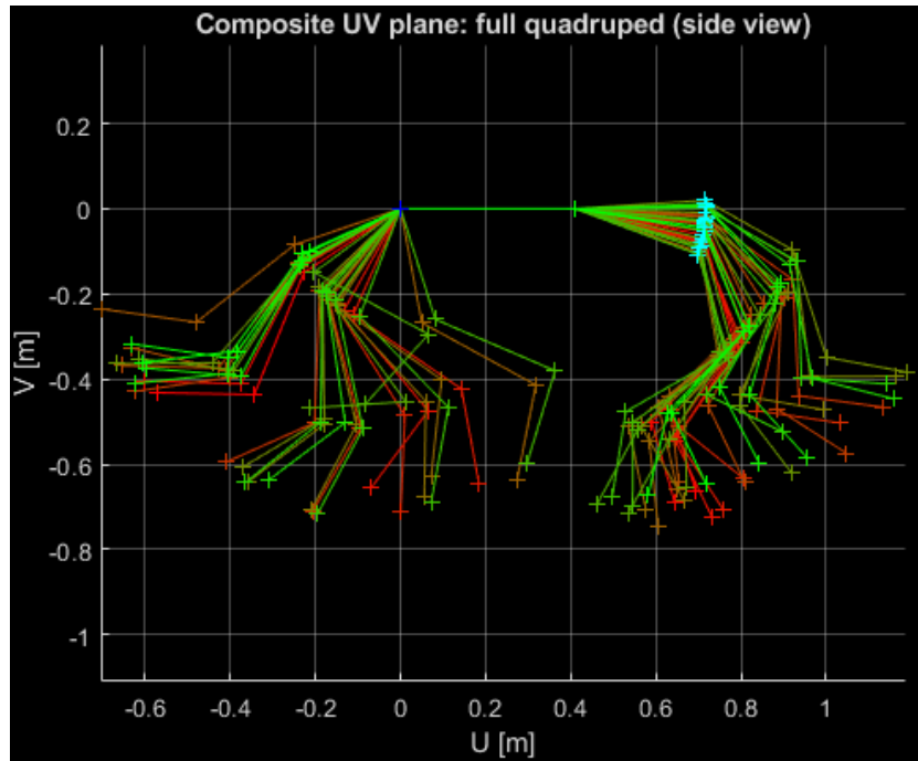
Figure 48: A composite of the full quadruped configurations in the UV plane (side view) with the reference joint located at (0, 0, 0) in the local system.
