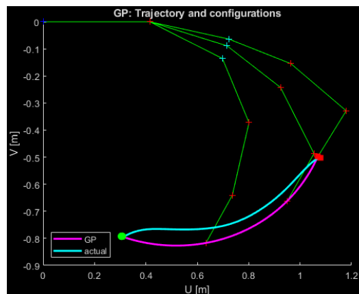
Figure 66: The gradient projection algorithm produced this trajectory in only 264 iterations with each iteration taking on average 0.36 microseconds. Every hundredth configuration is shown too.
