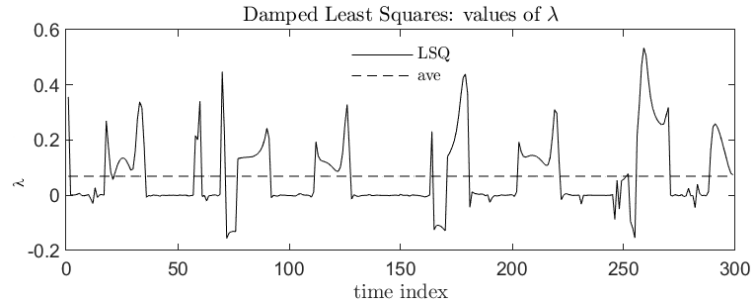
Figure 54: Inverse kinematics parameter \lambda as determined by a non-linear least squares optimisation for the damped least squares method.
