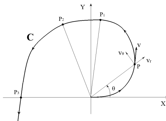
Figure 5: An arbitrary curve trajectory C , showing the radial and tangential components of the tangential velocity of a point P on C .
