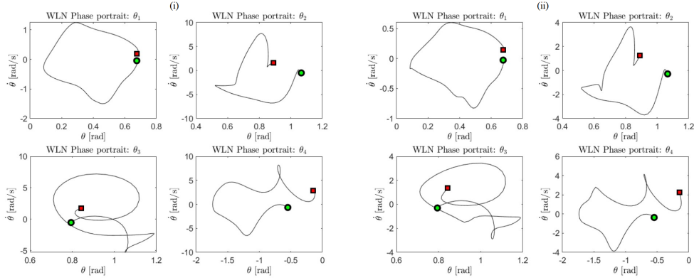
Figure 73: The effects of computing the scaling factor online and applying it to the angular rates vector shows similar to a very slight degradation in performance (ii) with slightly less smooth trajectories and nominal to increased DOCs when using the WLN method.
