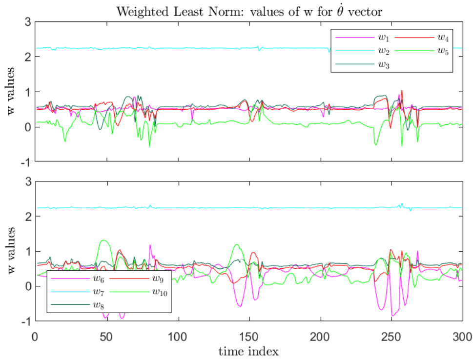
Figure 55: Inverse kinematics constants as determined by a non-linear least squares optimisation for the Weighted Least Norm method. The variables that comprise the diagonals of the weighting matrix W are w_1, \dots, w_{10} .
