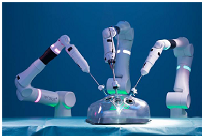
Figure 75: The Versius Surgical System (Image credit: CMR Surgical).
