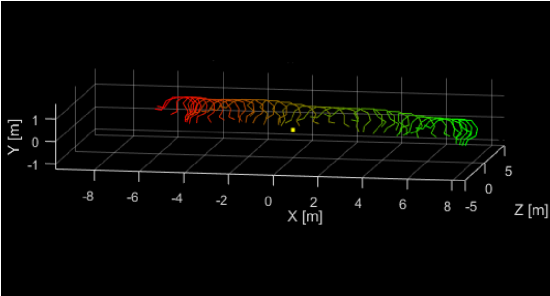
Figure 52: The full configuration sequence of the quadruped mechanism in the camera frame system with origin (0, 0, 0) represented by the yellow dot. The start position is at left (red) and it traverses through space until its final position at right (green) after an estimated distance of 12.8m after 0.9667 seconds. It achieves an estimated maximum speed of 21m.s^{-1} .
