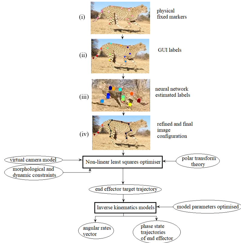
Figure 19: Flowchart with the design elements, processes, methods and key outputs of this project. The graphics (i) to (iv) show how the video image of the subject is used to obtain the input image for the least squares optimiser.
