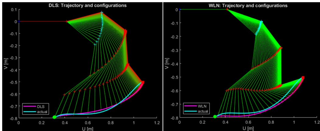
Figure 62: All the configuration sequences and proposed solution trajectories are similar for the DLS and WLN algorithms.
