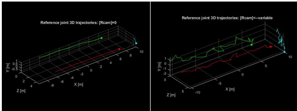
Figure 51: Estimated reference joint trajectories. At left are the three dimensional components of the reference joint trajectory, with all camera extrinsics fixed to zero, in the observers XYZ -coordinate frame. The trajectories at right are the result of the solver having the camera angles as variables.
