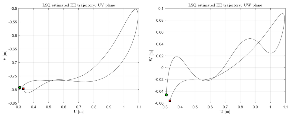
Figure 70: The nearly closed trajectories of the end effector, in Cartesian coordinates, for the second gait.
