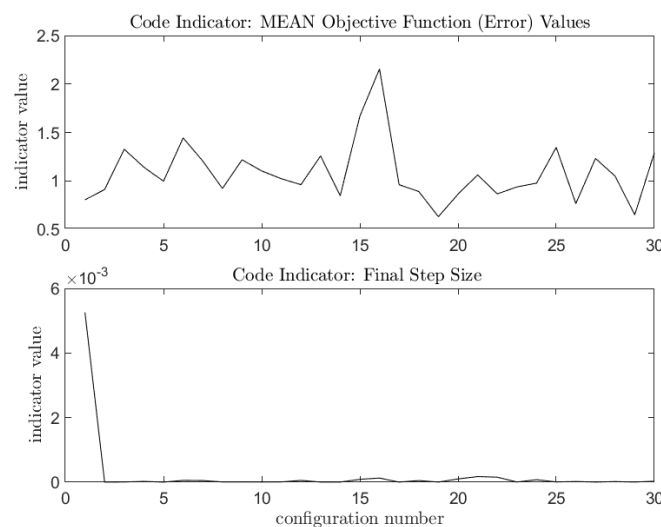
Figure 32: The mean objective function residuals and final step sizes. The mean residuals or errors are the average displacements in hyperspace between the estimated vector and solution points. The final step sizes are sufficiently close to zero and contribute to the validation statements of the solver. Notice the improvement after the first iteration. From the second iteration angular rates can be computed and the contributions of the other vector functions are now included in the solution.
