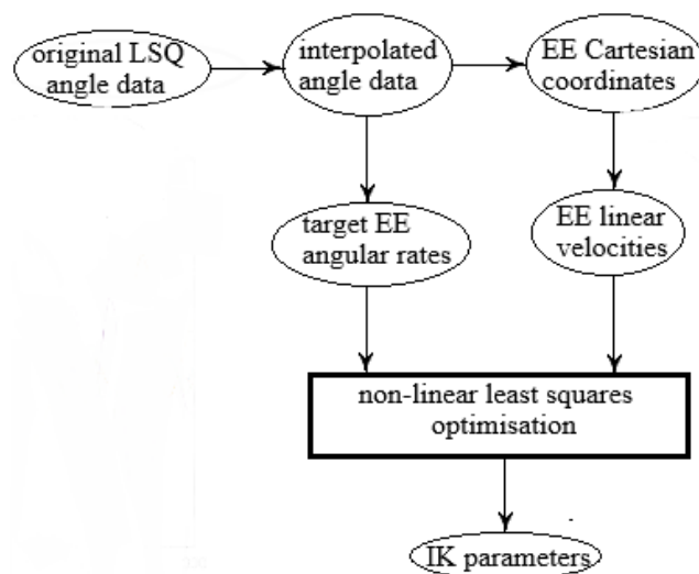
Figure 18: Flowchart for determining the parameter values for an inverse kinematics method.
