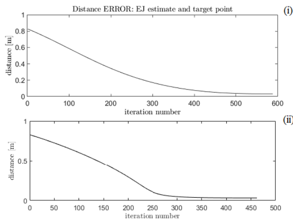
Figure 64: By using a suitable harmonic augmenting function with the extended Jacobian method, quick convergence to the target is achieved with no singularities. The computation of \alpha online (ii) results in a faster convergence to the target than using \alpha = 0.643 constant (i).
