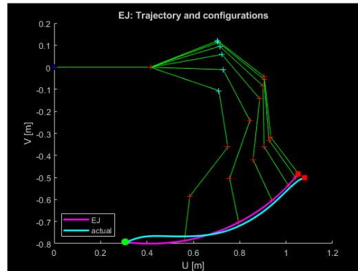
Figure 65: The optimal trajectory produced by the extended Jacobian method. The optimisation function took the form of a harmonic augmenting function with the variables being selected relative motion angles. Every hundredth configuration is shown.
