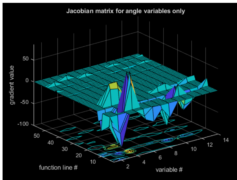
Figure 35: The average of the Jacobian matrix element values for only the angle variables of the quadruped mechanism. Note the smaller values for all the \phi variables (variable numbers 8 to 14).
