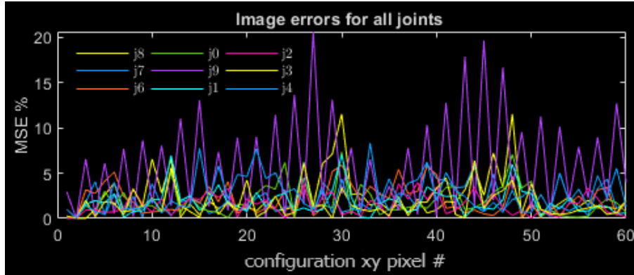
Figure 37: The mean error values for the joint image estimates are shown for all configurations. Notice the peak for joint #9 (mid-spine joint). The data shown here is repeated in Figure 38 as a two dimensional image error data matrix with the joint index numbers corresponding to the joint numbers of the mechanism.
