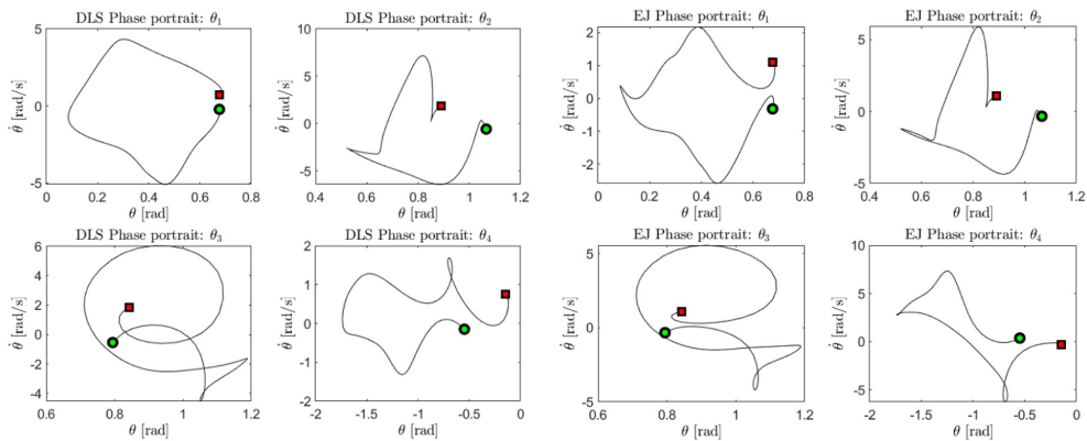
Figure 72: The primary phase states for all the joints as determined by the damped least squares (left set) and the extended Jacobian (right set) methods.
