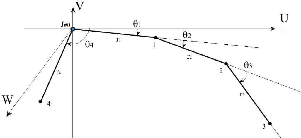
Figure 24: A sample mechanism showing link lengths, joints and angle definitions within the UVW local system. The variables here are used to define the 3D joint positions according to the transform equations.
