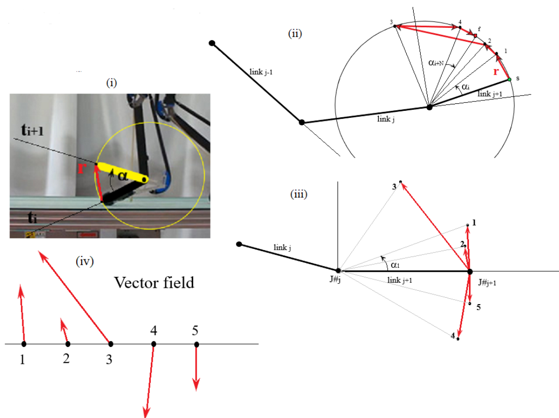
Figure 6: The vector field generation for the incremental movement of the robot link in (i) from time t_i to t_{i+1} . Schematics (ii), (iii) and (iv) show how the field is created for a generic link_{j+1} as it undergoes five incremental movements which are relative to its prior link_j . The field is represented as a time line with the associated vectors (indicated by red arrows) at each interval.
