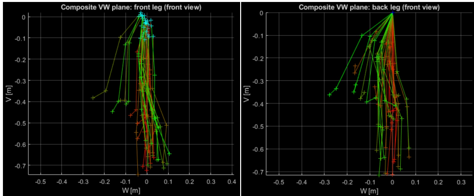
Figure 50: The front views (looking head-on to the quadruped) show the distributions of the legs. The back leg, particularly, shows a definite pattern; at high speeds (shown in green) there is a greater deviation from the sagittal plane, as is to be expected.
