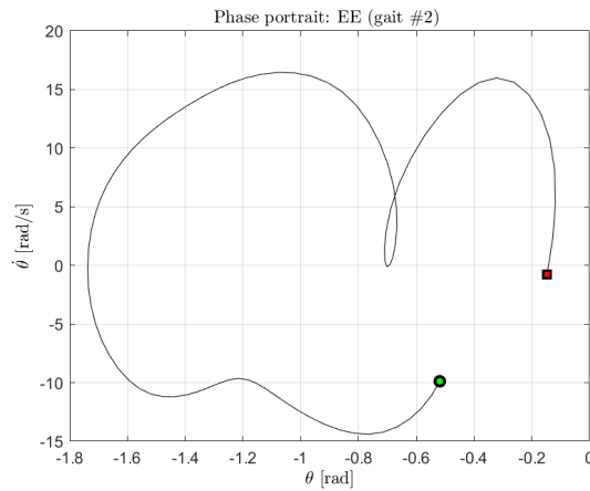
Figure 71: The phase states for the primary motion plane of the end effector as determined by the least squares solver.
