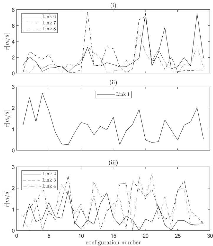
Figure 83: Polar velocity magnitudes for (i) front leg, (ii) spine and (iii) back leg links for all of the configurations.
