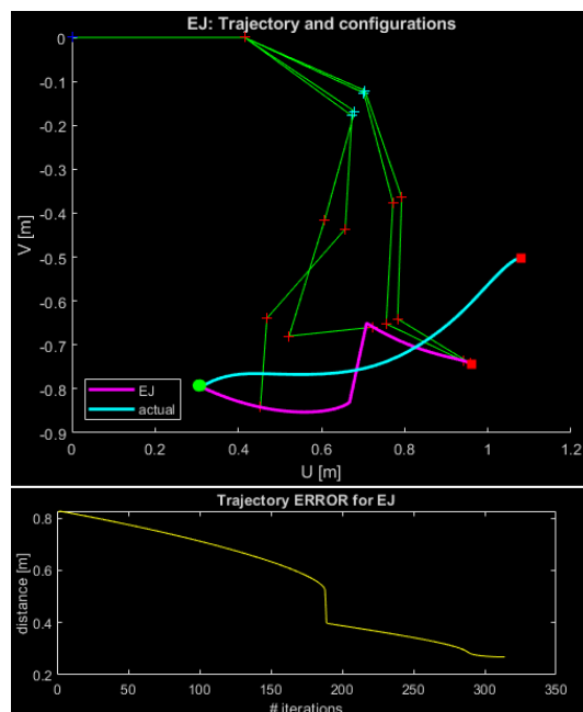
Figure 80: Discontinuous, non convergent trajectory resulting from an unsuitable cost function: g = (\theta_3 - \theta_2)(\theta_2 - \theta_3) + (\theta_3 - \theta_4)(\theta_4 - \theta_1) . The graphic below it shows the distance between the current and target points confirming failure to converge.
