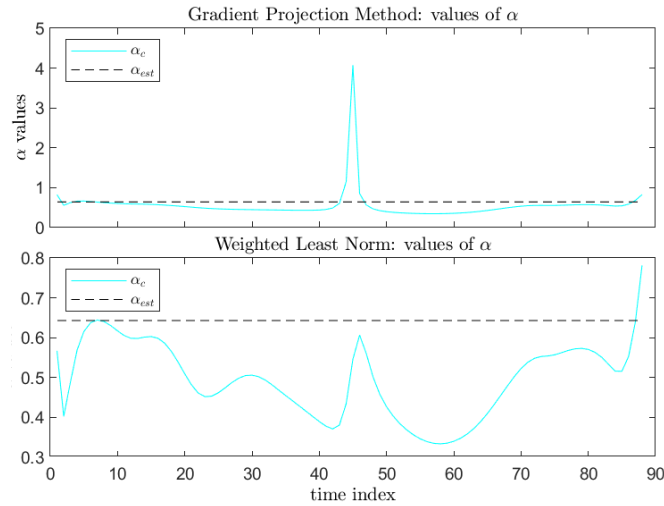
Figure 58: The variation of the scaling factor \alpha as computed online for the GP and WLN methods. The mean estimated value as determined by the EJ method is indicated by the dashed line.
