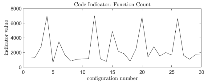
Figure 33: The high number of function evaluations due, in part, to the use of centrally based gradient computations by finite differences.
