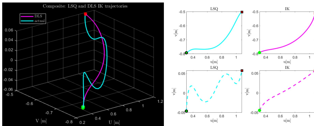
Figure 59: The DLS method produced this trajectory (magenta) given a target point (red). A similar result was obtained with the WLN method. The cyan coloured trajectory is the actual path taken by the end effector. Notice how the IK determined path of the end effector is smoother and less oscillatory, particularly in the UV plane, than the original actual trajectory.
