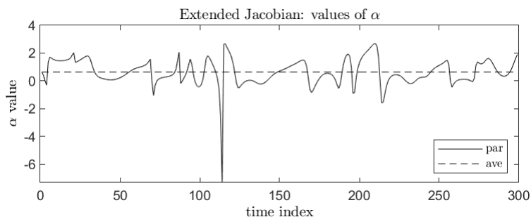
Figure 57: The estimated parameter \alpha values for the extended Jacobian method together with its average of 0.643.
