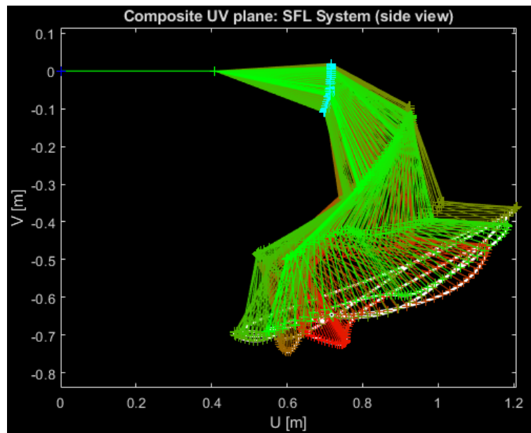
Figure 53: The target trajectory for the inverse kinematics models is generated by the front leg of the quadruped. The early phases of the trajectory are shown as red and terminate in green.
