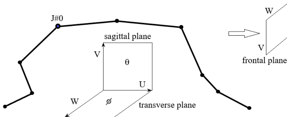
Figure 13: All the descriptor planes that relate the local link motion of the quadruped with respect to the reference joint ( J\#0 ). The three planes are the sagittal ( UV ) side, transverse ( UW ) top elevation and frontal ( VW ) planes. The permitted angle rotations \theta and \phi are shown in their operational planes. Link twist angles \gamma are all assumed zero for simplicity.
