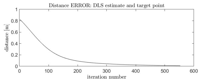
Figure 61: The rapid convergence to the target is shown by the distance in task space between the current model estimate and the target. The data shown here was for the DLS with the WLN method showing a similar trend.
