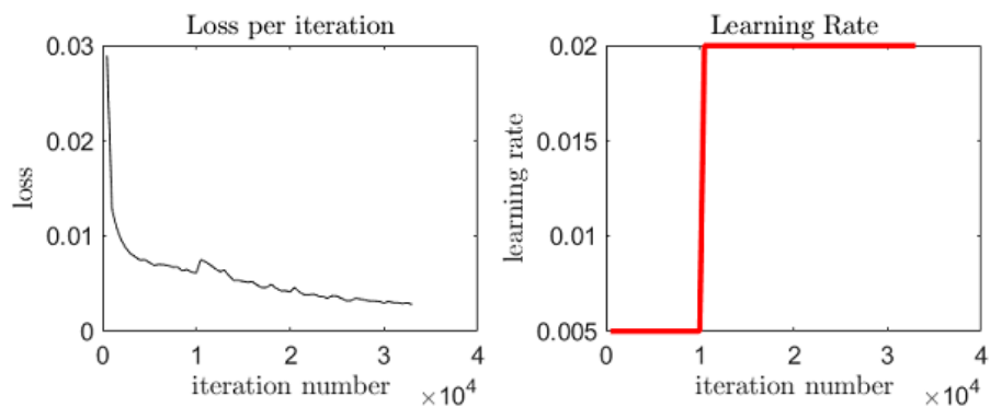
Figure 22: Learning rate data for a typical network training session showing the reduction in errors (loss) and the learning rate variation as the number of iterations progresses.
