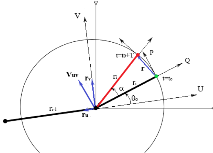
Figure 8: The vector \mathbf{V}_{uv} is the projection (using polar transforms) of \mathbf{r} onto the local UV axis of the parent link. In this way relative motions can be displayed for all links and the sequence of vectors obtained thus generating a field.
