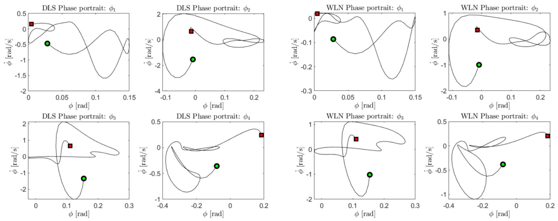
Figure 77: Joint trajectory estimates in \phi phase space by the damped least squares method.
