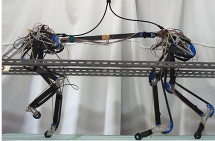
Figure 1: The PneuPard is an experimental light weight, biomimetic pneumatic powered quadruped similar to the proposed model presented in this publication (Image credit: Osaka University).
