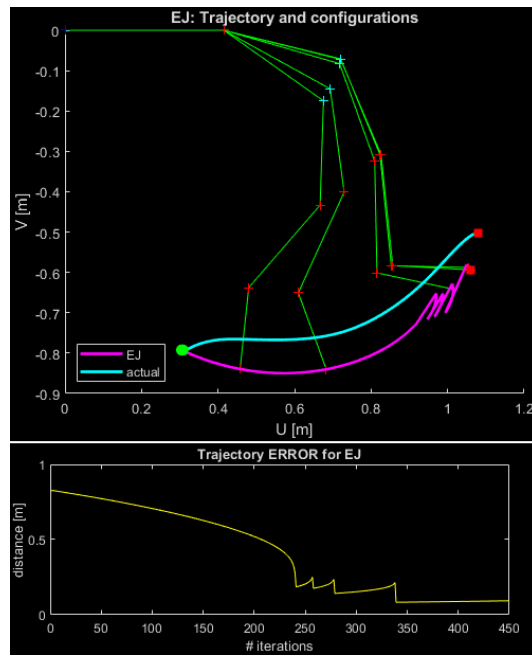
Figure 79: Chaotic, non convergent trajectory resulting from an unsuitable cost function: g = (\theta_2 - \theta_1)(\theta_2 - \theta_3) + (\theta_3 - \theta_4)(\theta_4 - \theta_1) . The graphic below it shows the distance between the current and target points confirming failure to converge.
