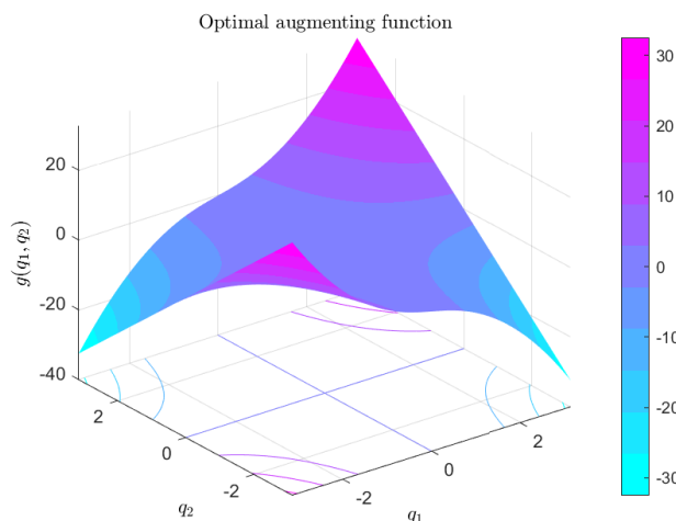
Figure 63: The optimal augmenting function that is a harmonic kinematics mapping for the EJ algorithm. The variables q_1 and q_2 are relative angles corresponding to two links.
