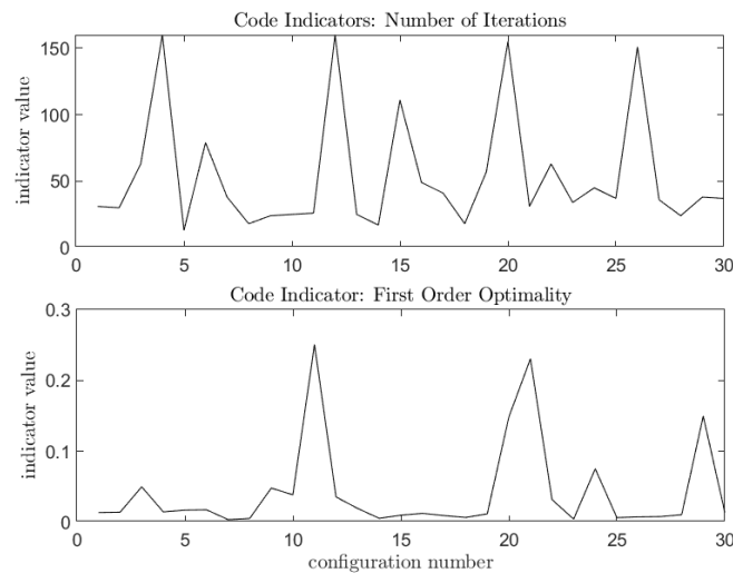
Figure 31: The number of iterations and first-order optimalities for all the configurations. Low first-order optimality values close to zero are a good indication that the solutions are near to being optimal.
