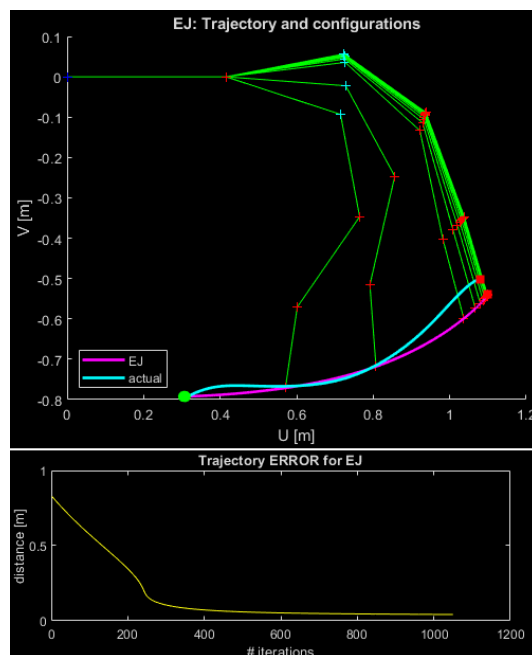
Figure 78: Non convergent trajectory resulting from an unsuitable cost function: g = (\theta_2 - \theta_1)^2(\theta_1 - \theta_3)^2 + (\theta_3 - \theta_4)^2(\theta_4 - \theta_1)^2 . The graphic below it shows the distance between the current and target points confirming failure to converge.
