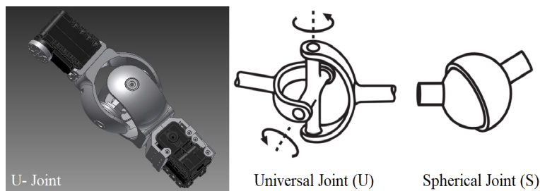
Figure 11: Universal ( U ) and spherical ( S ) joints. All joints for the quadruped serial link mechanism are based on universal joints. If spherical joints were to be used an additional rotational axis would be introduced allowing the links to twist relative to their parent links.
