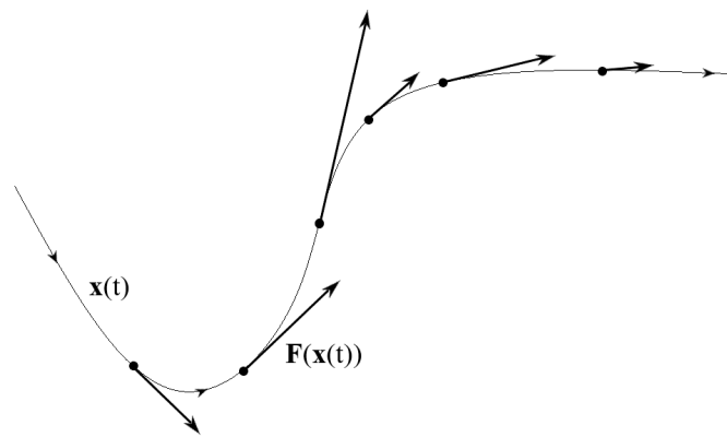
Figure 7: Solution integral curve x(t) with the associated vector field F(x(t)) at the specific solution points.
