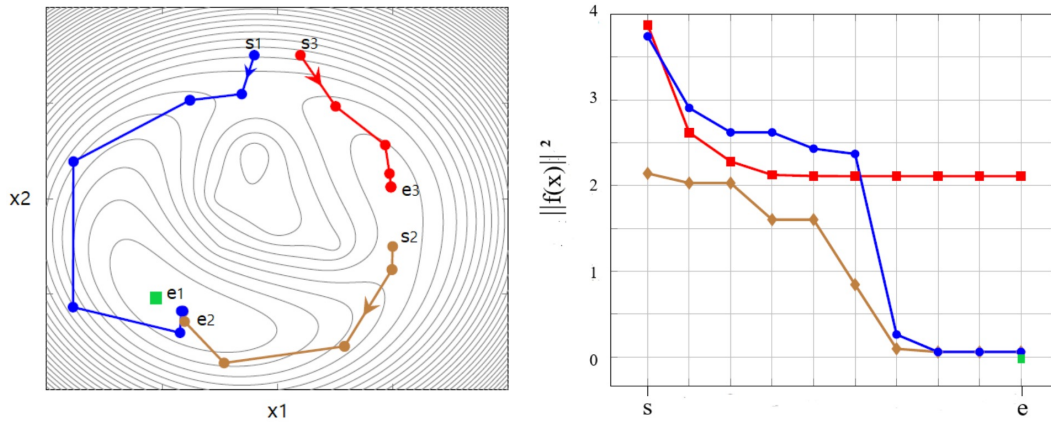
Figure 10: Another illustrative two parameter model example and how the initial guesses of the solution vector at the start of the algorithm search may affect the outcome. The initial search position for the red path results in a sub-optimal solution and this is confirmed by the magnitude of the squares of the residuals at this solution. The other two searches terminate at near optimal solutions (blue and brown paths). The actual solution is shown by the green square.
