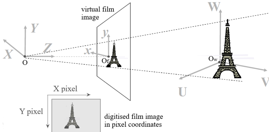
Figure 2: Camera model showing the virtual image generated from a real world 3D object. The desired pixel image is processed from the film image according to the physical properties of the actual camera being used. The respective origins of the frames are indicated by O , O_f and O_w .
