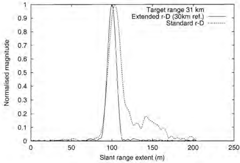
Figure 4.13: The magnitude of the range profile after processing the 31 km target with the extended algorithm (30 km reference) and the standard range-Doppler algorithm.
