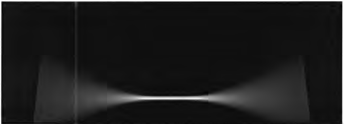
Figure 3.5: The magnitude of the signal in the range-Doppler domain after the range curvature correction operation (Simulation A). Only the first 100 of the 528 slant range bins are displayed (range increases vertically). The full 250 Hz sampling bandwidth is represented by the horizontal extent of the image.
