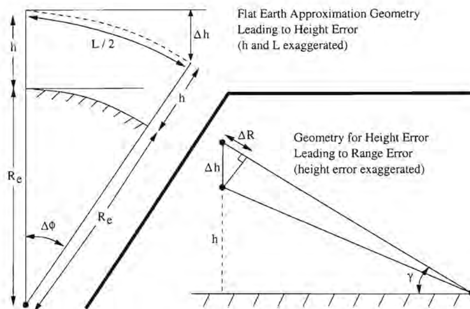
Figure 5.2: The flat earth approximation resulting in a height error over the synthetic aperture.
