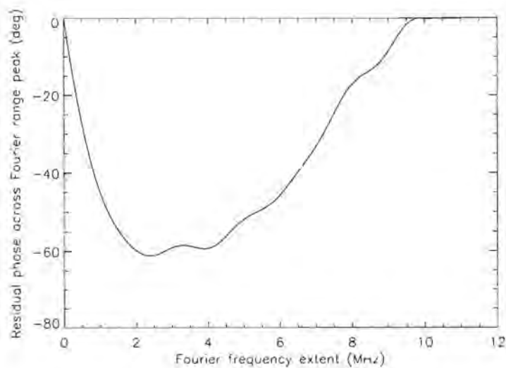
Figure 4.12: The quadratic- and higher order range Fourier phase error for the standard range-Doppler processor and 31 km target.
