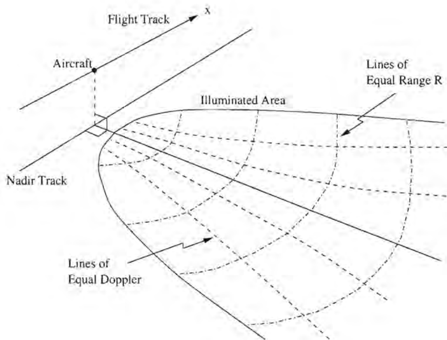
Figure 2.1: The imaging geometry for a wide beam, airborne stripmap SAR.
