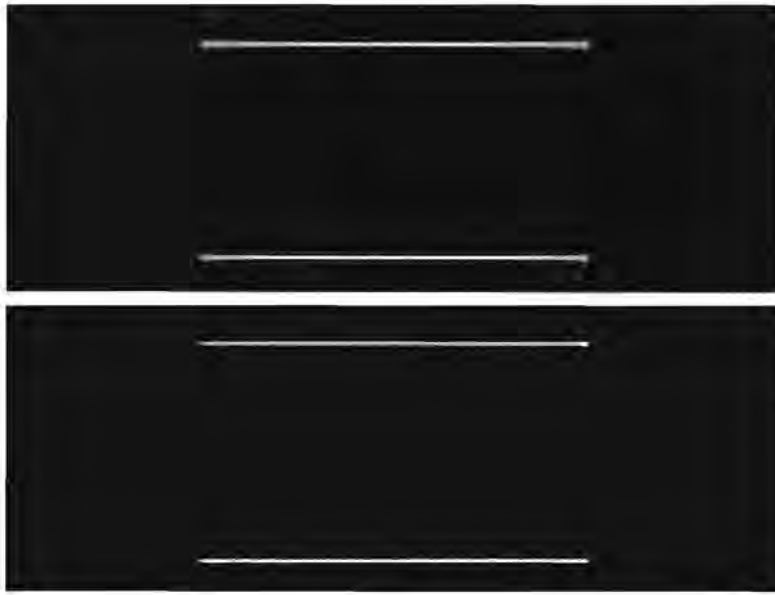
Figure 4.7: The data in the range-Doppler domain (zero-centred) after residual range curvature correction (Step G). Top is for the 25 km reference range and bottom for the 30 km reference range. Slant range increases vertically with the targets 1 km apart and the full 250 Hz sampling bandwidth is displayed horizontally.
