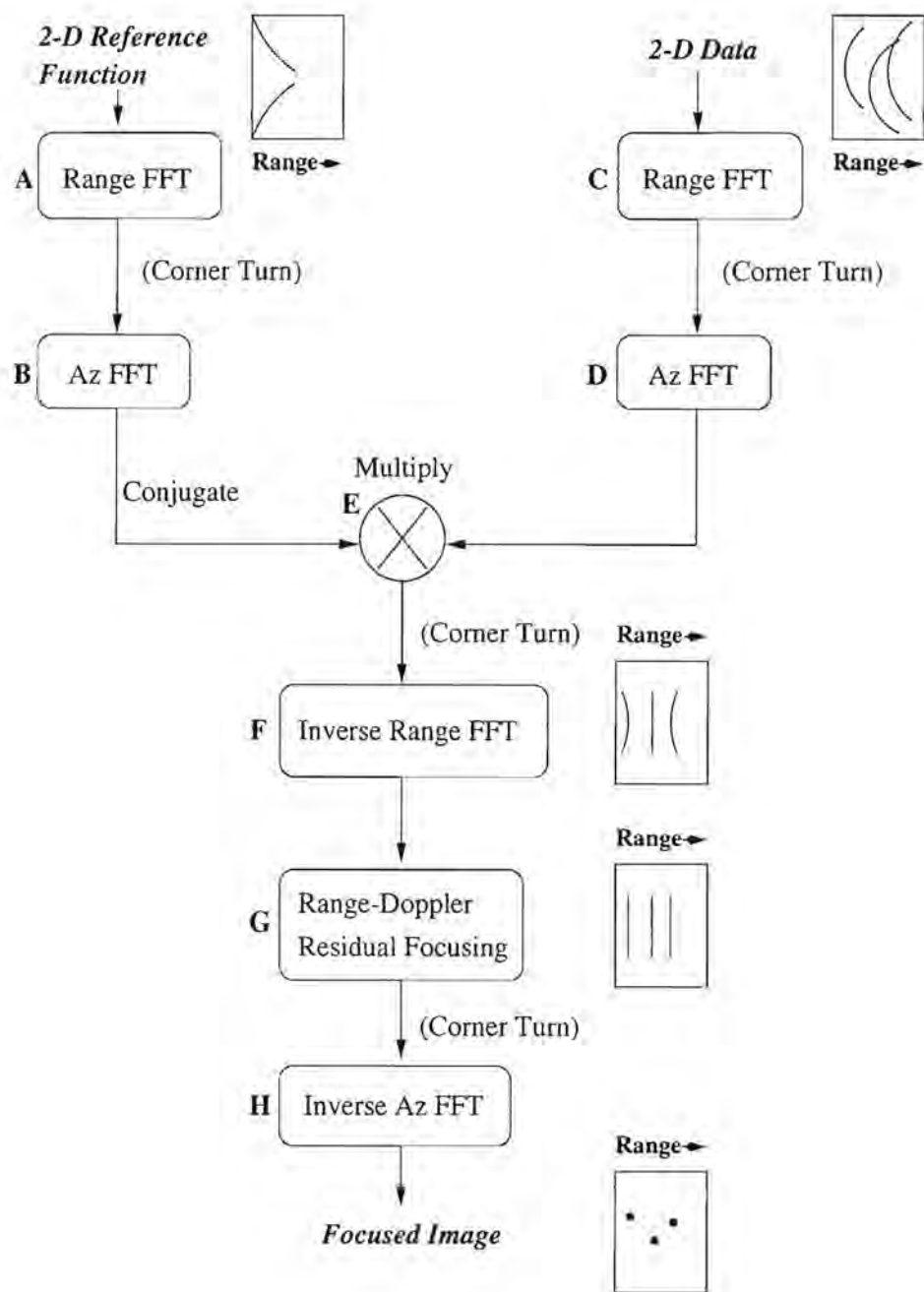
Figure 4.1: The extended range-Doppler algorithm.
