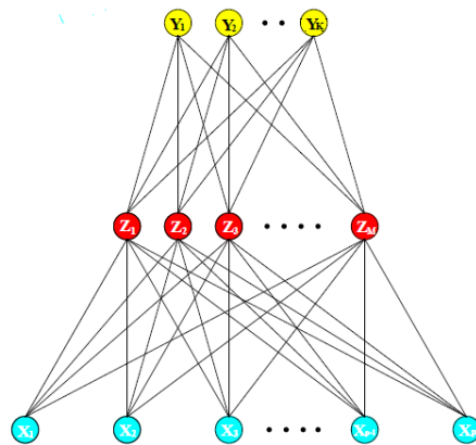
Figure 3: Diagram illustrating a feed-forward neural network with a solitary hidden layer. Figure taken from Friedman, et al. [37]
