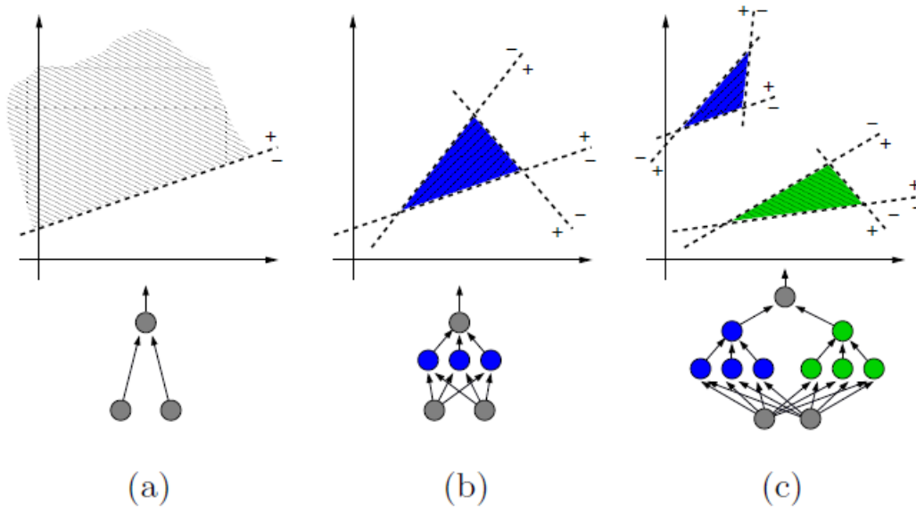
Figure 2: Illustrations depicting the amount of network structure required to bound isolated sections of a 2D decisions space. Figure (a) depicts how a single layer divides the decision space in half. Figure (b) depicts how a triangular section of the decision space can be bounded with the addition of three hidden nodes. Figure (c) depicts the significantly more complex network structure with two hidden layers and 8 nodes that would be required to bound two separate triangular regions. Figure taken from Kohl, et al. [2].
