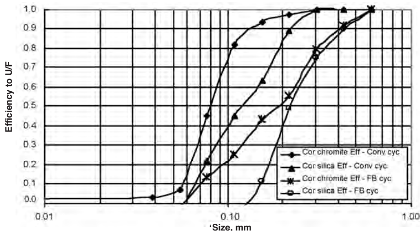
Figure 6—Corrected efficiency curves for conventional and flat bottom cyclones for silica and chromite
