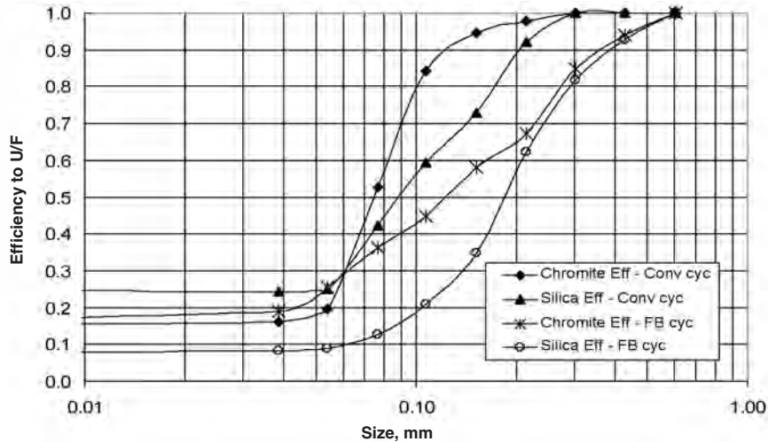
Figure 5—Actual efficiency curves for conventional and flat bottom cyclones for silica and chromite
