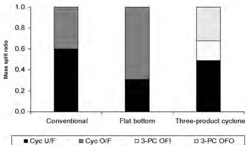
Figure 7—Mass splits to the respective cyclone products
