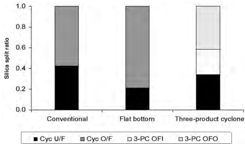
Figure 8—Average silica splits to the respective cyclone product streams
