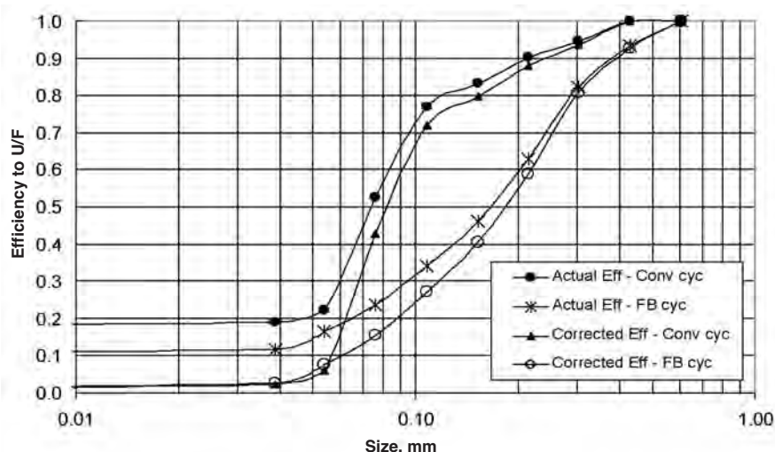
Figure 4—The actual and corrected efficiency curves for the conventional and flat bottom cyclones
