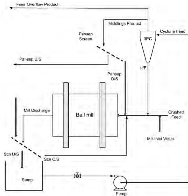
Figure 10—The pilot plant test rig set-up for application of the three-product cyclone
