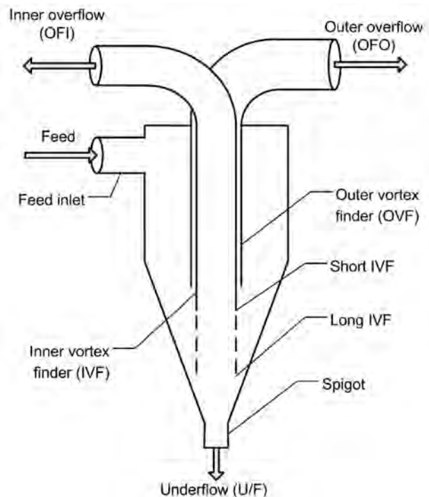
Figure 3—Schematic showing the main parts of the three-product cyclone
