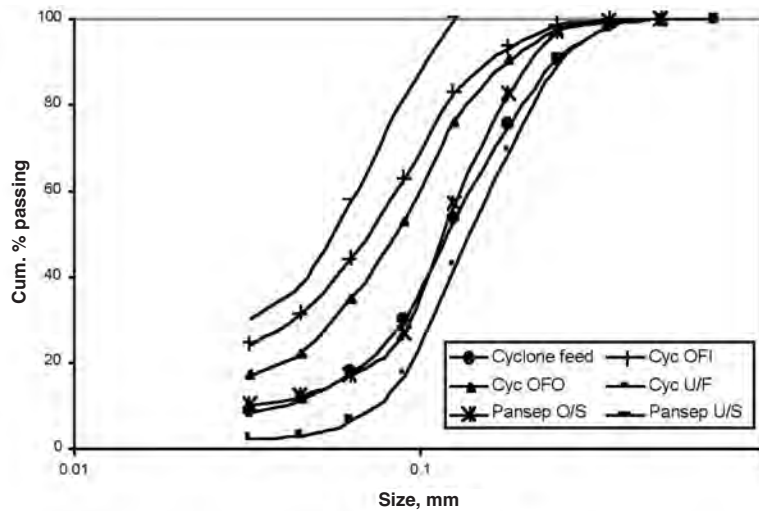
Figure 11—Particle size distributions for the three-product cyclone and Pansep screens obtained from the pilot plant tests
