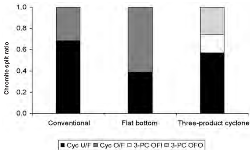
Figure 9—Average chromite splits to the respective cyclone product streams
