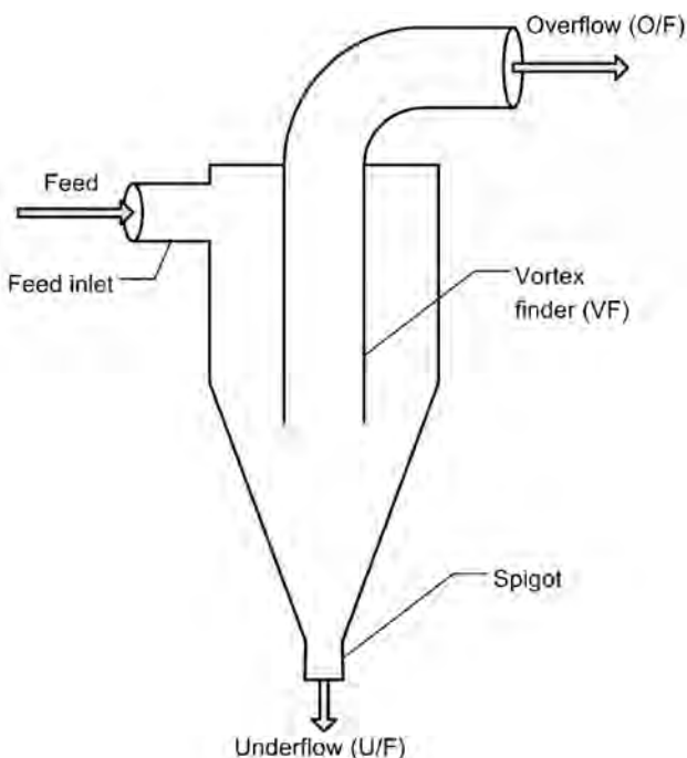
Figure 1—Schematic showing the main parts of the conventional hydrocyclone
