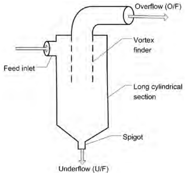
Figure 2—Schematic showing the main parts of the flat bottomed cyclone
