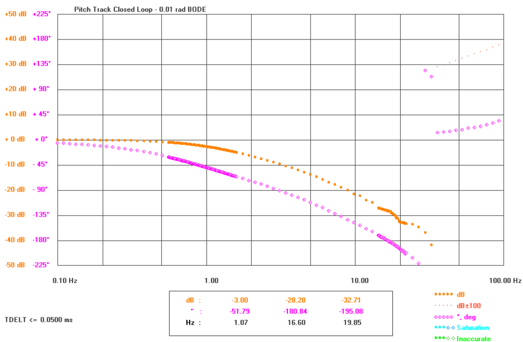
Figure 6-46: Pitch track closed-loop Bode plot - Linear Response
