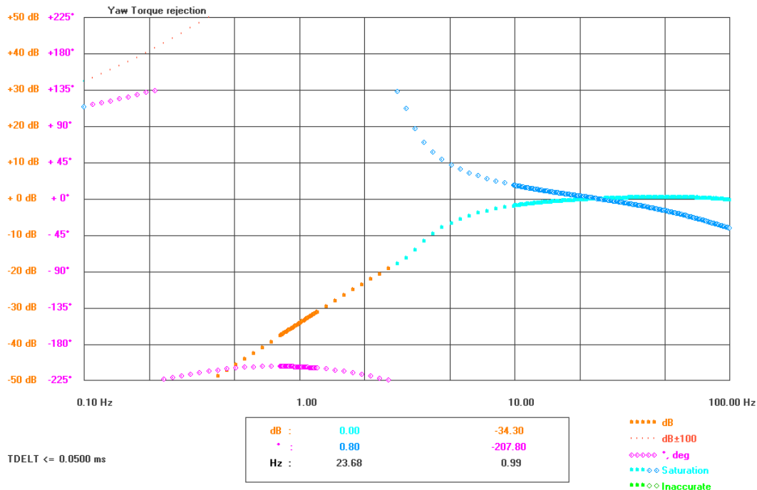
Figure 6-35: Yaw torque rejection– Yaw rate command to rate error (1.0 rad/s)
