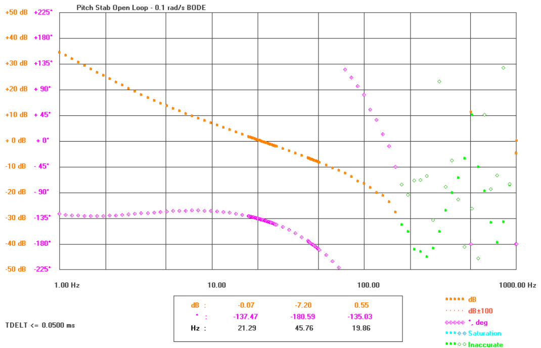
Figure 6-23: Pitch rate open-loop Bode plot - Linear Response
