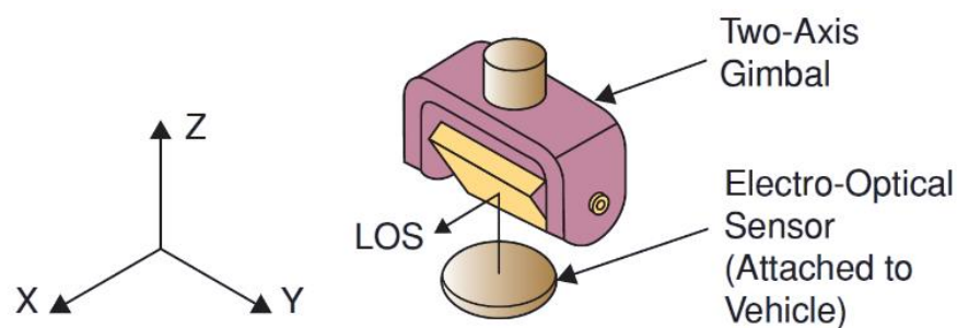
Figure 2-4: Mirror stabilisation mechanism [1]
