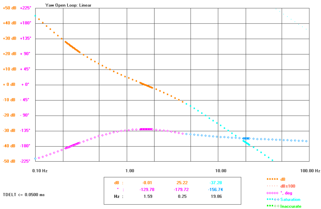
Figure 6-8: Linear open-loop responses of the yaw manual position controller
