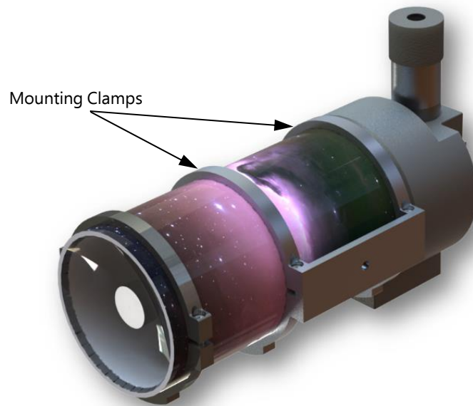
Figure 4-7: ETX90 Mounting Concept 2
