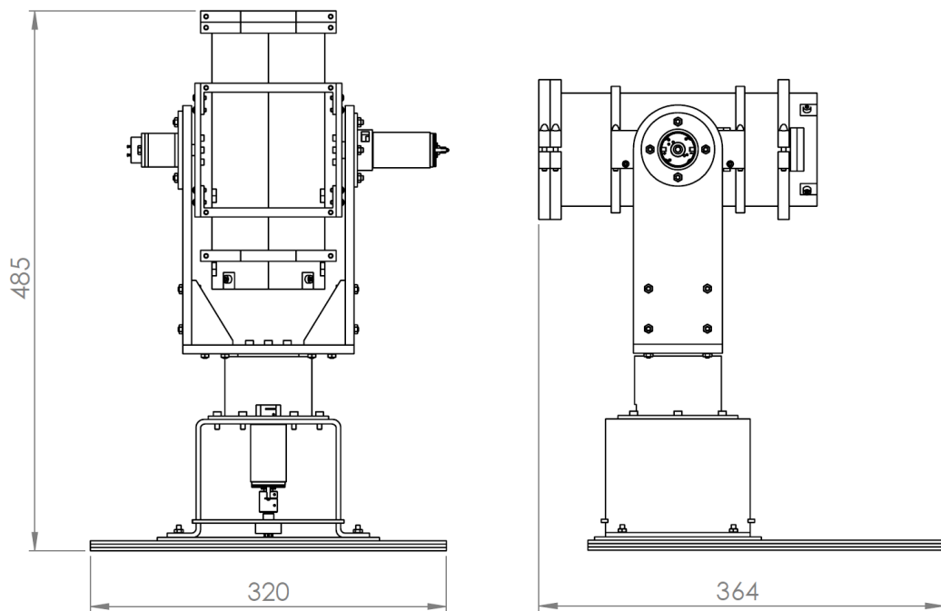
Figure 4-24: ISP system overall dimensions
