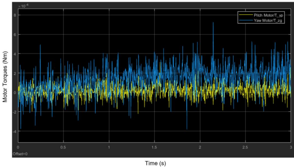
Figure 5-54: Motor torques for the home position
