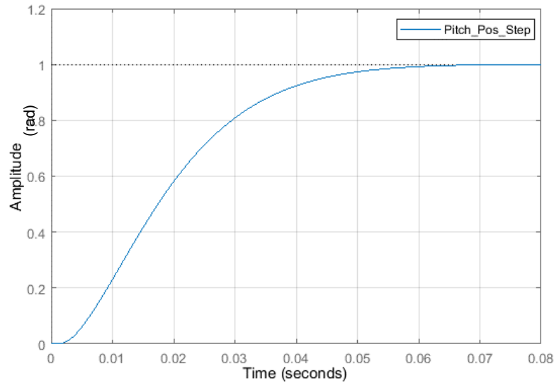
Figure 5-50: Motor selection simulation - Pitch position step following
