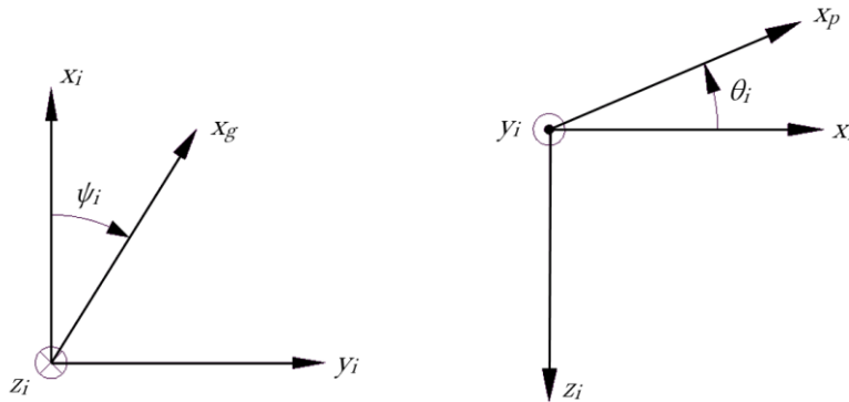
Figure 2-22: Inertial angle definitions
