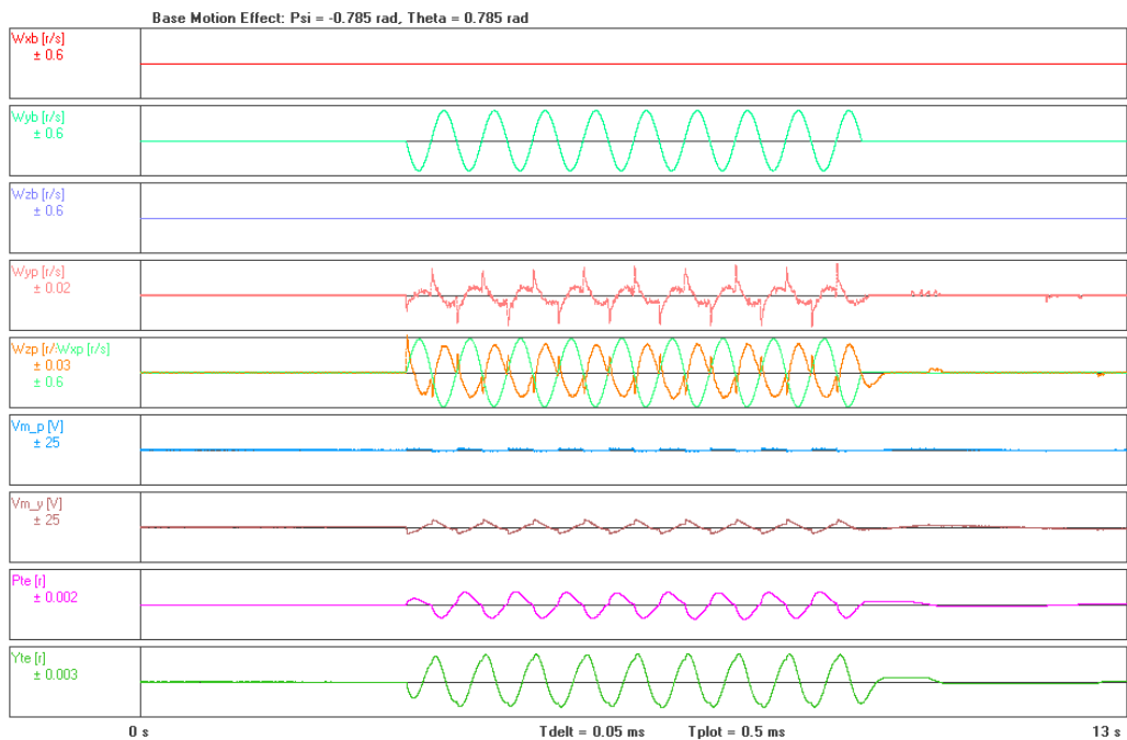
Figure 8-21: Base motion effects about the y_b axis in the worst-case orientation
