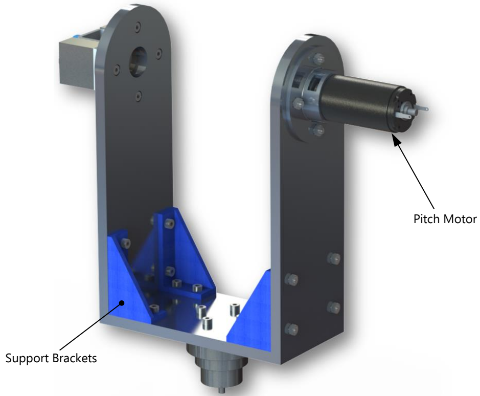
Figure 4-13: Yaw gimbal final design (front)
