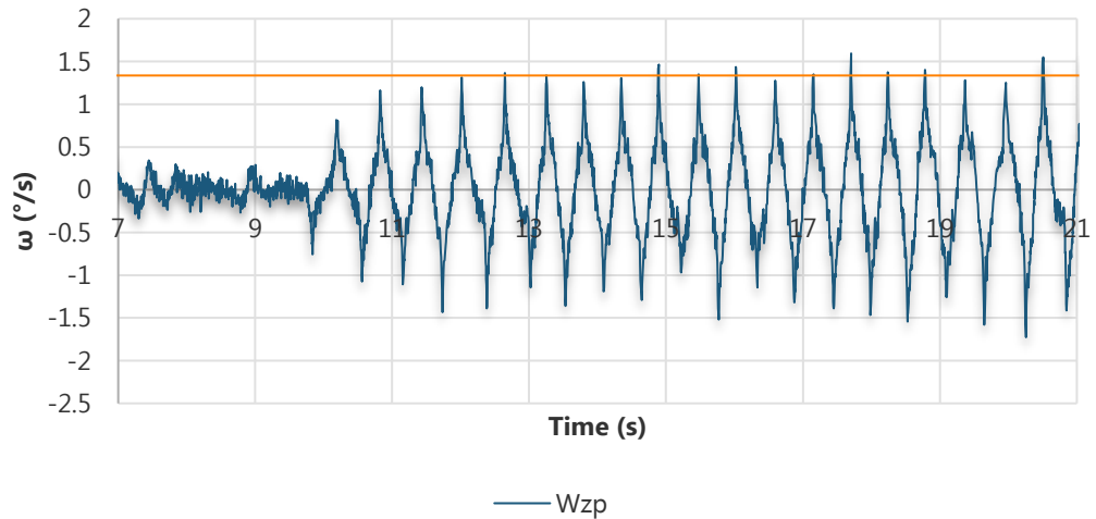
Figure 8-20: Inertial rate, \omega_{zp} , during the worst-case orientation BMI test
