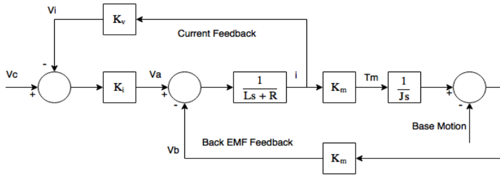
Figure 2-3: Current feedback minor loop
