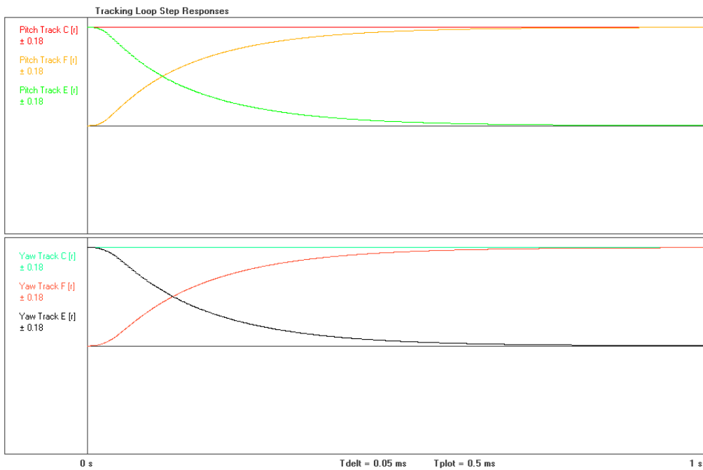
Figure 6-49: Tracking loops step following response
