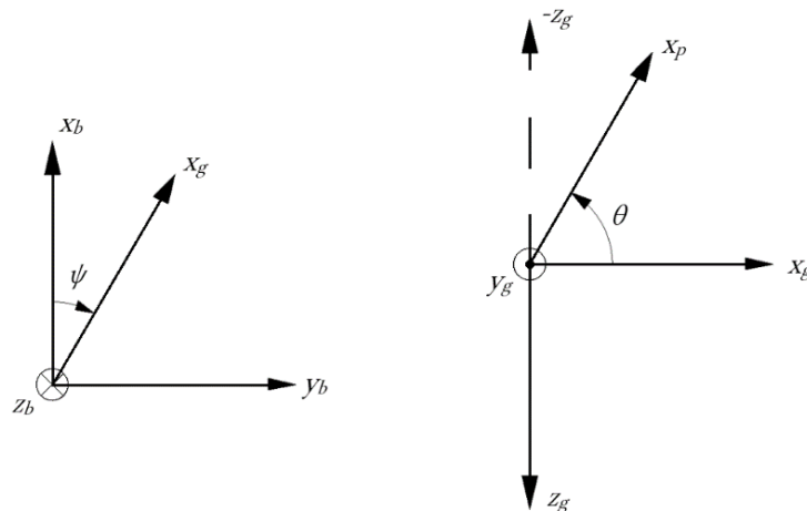
Figure 2-23: Relative angle definitions
