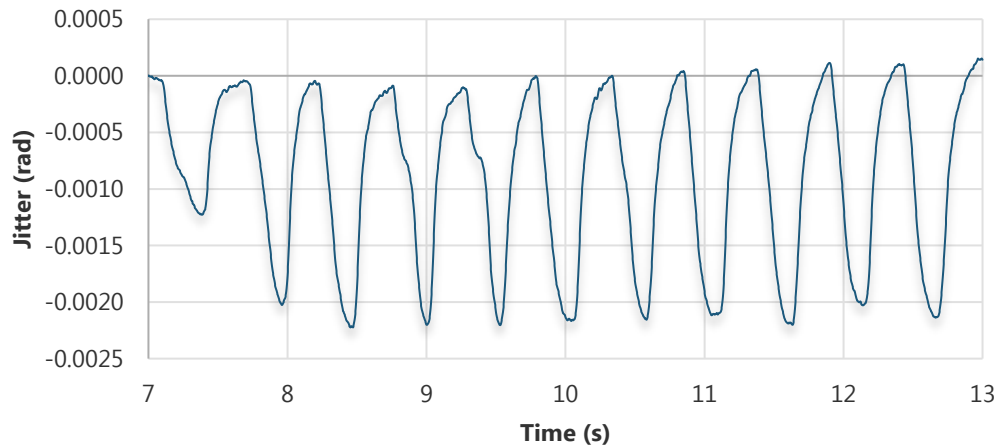
Figure 8-11: Pitch channel jitter estimation
