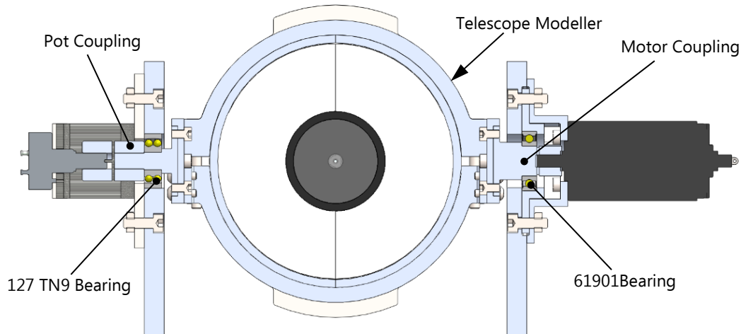
Figure 4-16: Section view of the telescope modeller to yaw gimbal coupling mechanism
