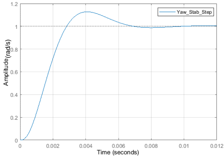
Figure 5-41: Motor selection simulation - Yaw rate step following
