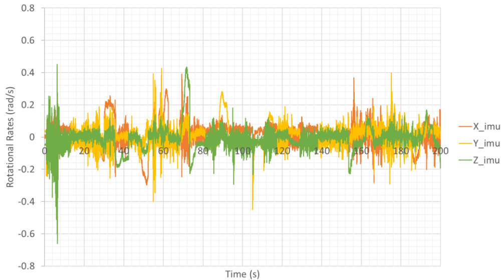
Figure 5-21: Vehicle motion from Base Motion Test 2
