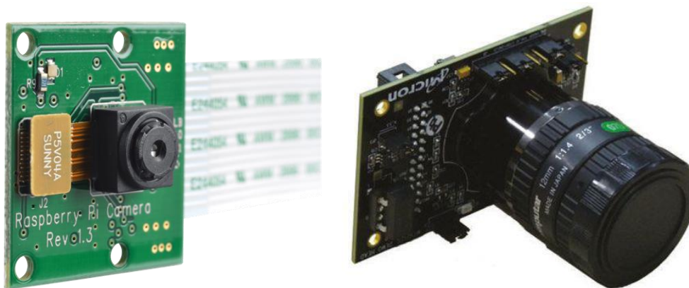
Figure 5-2: Raspberry Pi Camera [65] and Aptina MT9P031 Demo Kit 2 [66]
