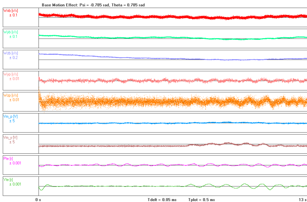
Figure 6-60: Base motion effect of the simulated base motion signal on the ISP in the worst-case position
