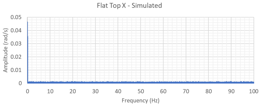
Figure 5-28: Frequency domain representation of the simulated signal x axis
