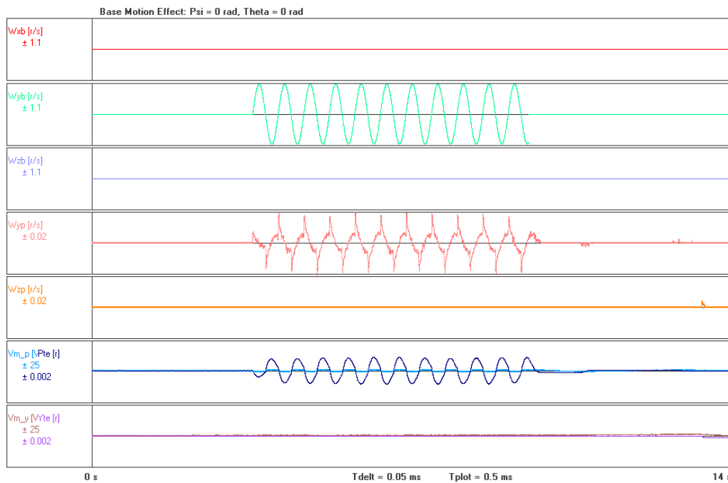
Figure 8-10: Pitch channel base motion isolation with corrected friction model
