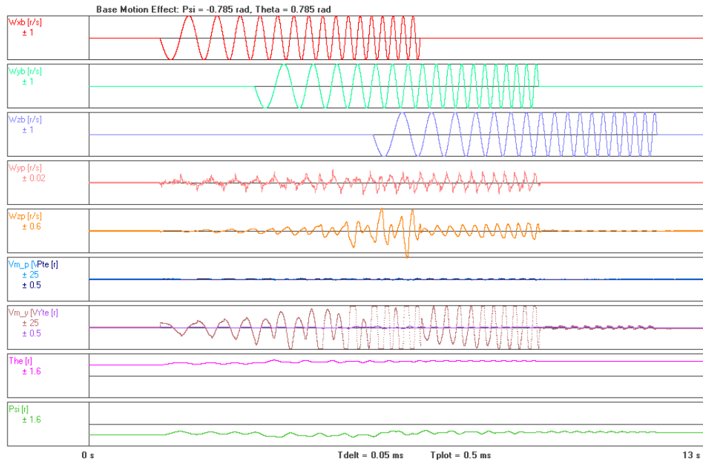
Figure 6-50: 1.0 rad/s base motion effect in the worst-case position
