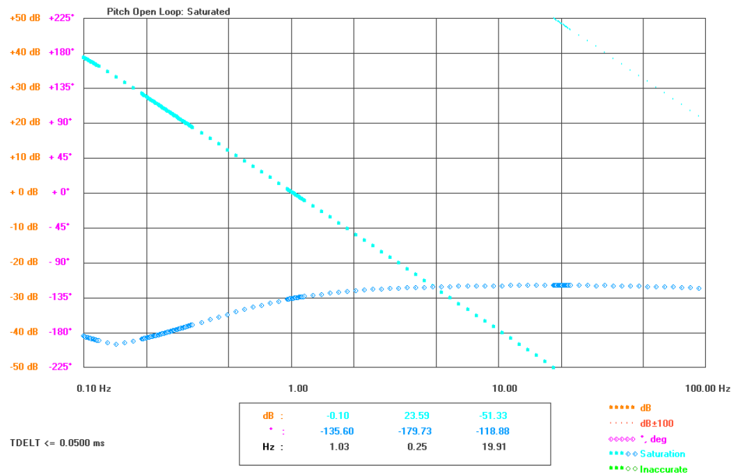
Figure 6-4: Saturated open-loop responses of the pitch manual position controller
