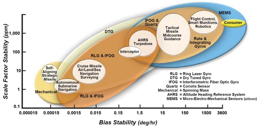
Figure 2-8: Types of gyro and their applications [25]
