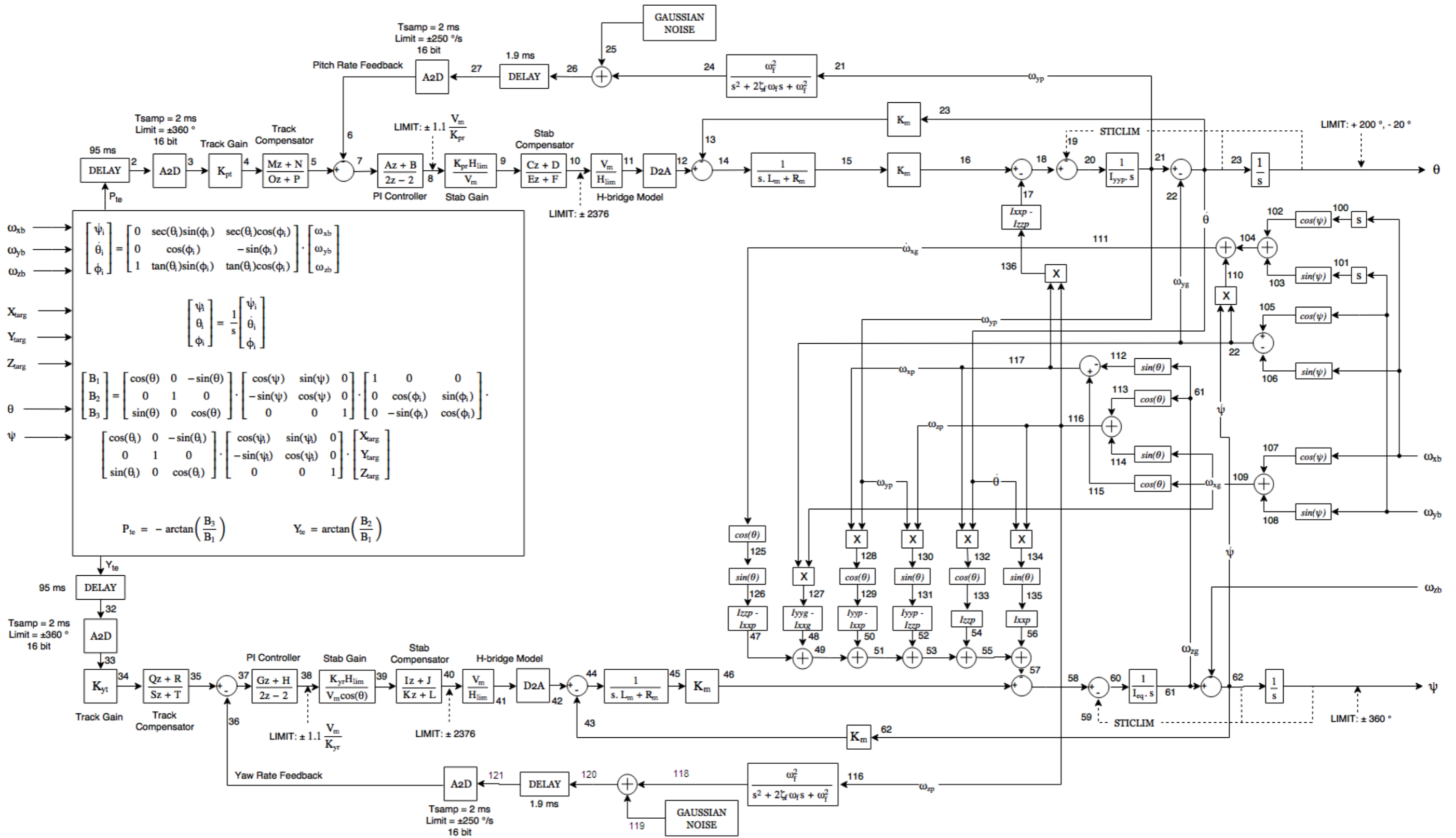
Figure 6-55: Final ISP simulation block diagram
