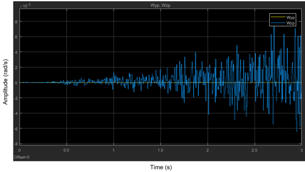
Figure 5-53: Inertial rates of the telescope for the home position
