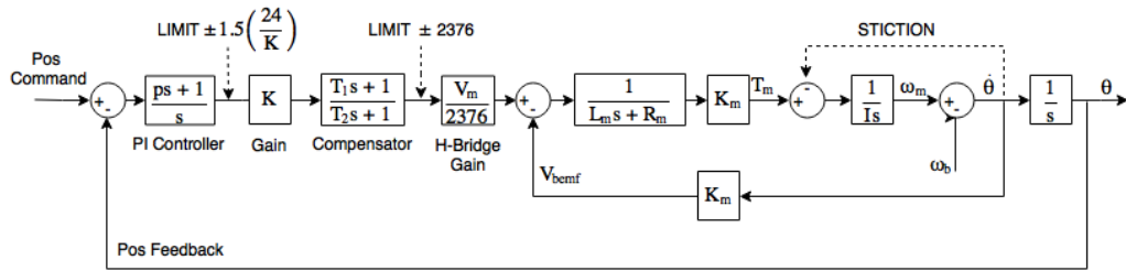
Figure 6-1: Manual position controller model
