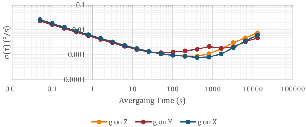
Figure 5-9: Z-Axis Allan Deviation
