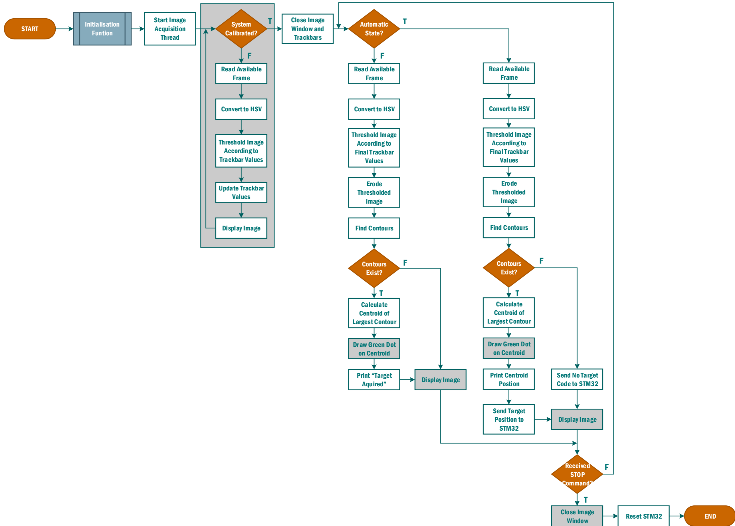
Figure 7-14: Image processing functional flowchart
