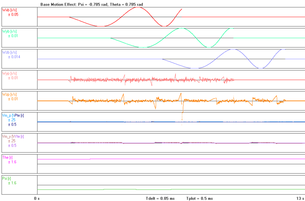
Figure 6-52: Base motion effect of the peaks of the simulated base motion signal at 0.1-0.2 Hz in the worst-case position
