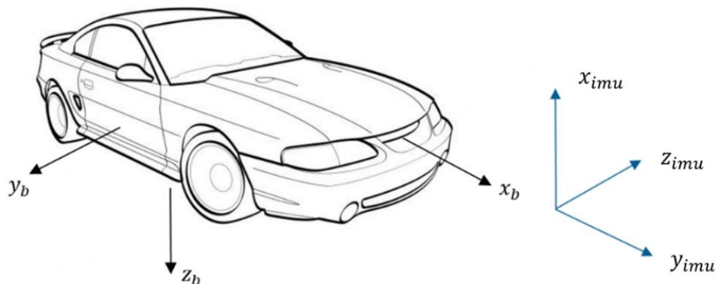
Figure 5-20: IMU axes alignment with vehicle axes (image adapted from [89])
