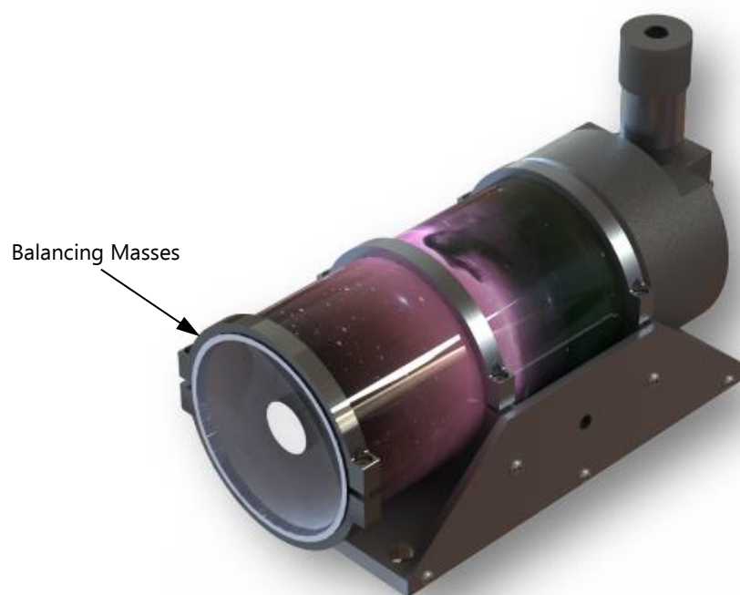
Figure 4-5: ETX90 Mounting Concept 1
