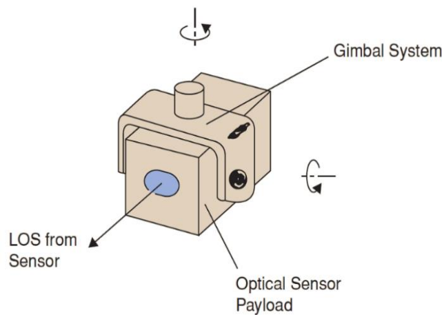
Figure 2-2: Mass stabilised sensor [7]
