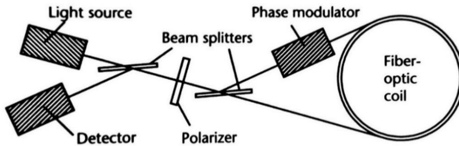
Figure 2-11: Schematic of an IFOG sensor [27]
