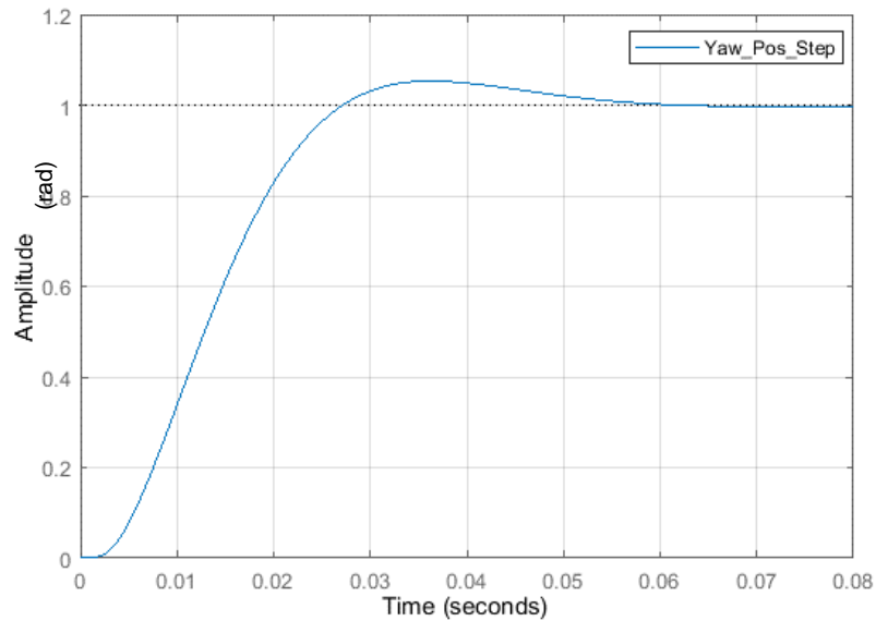
Figure 5-47: Motor selection simulation - Yaw position step following
