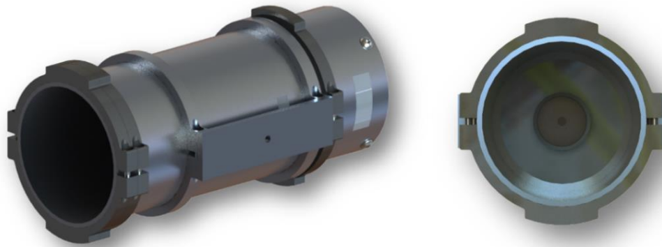
Figure 4-8: Raspberry Pi Camera mounted on Mounting Concept 2
