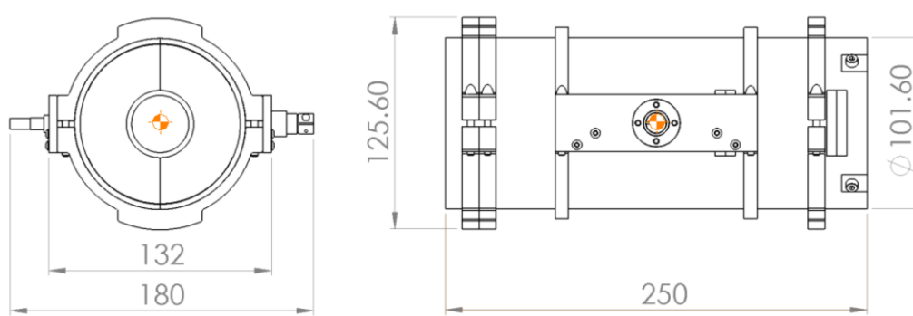
Figure 4-12: telescope modeller overall dimensions
