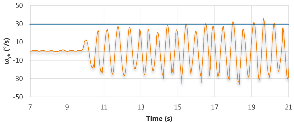
Figure 8-17: Base motion, \omega_{yb} , for the worst-case orientation BMI test
