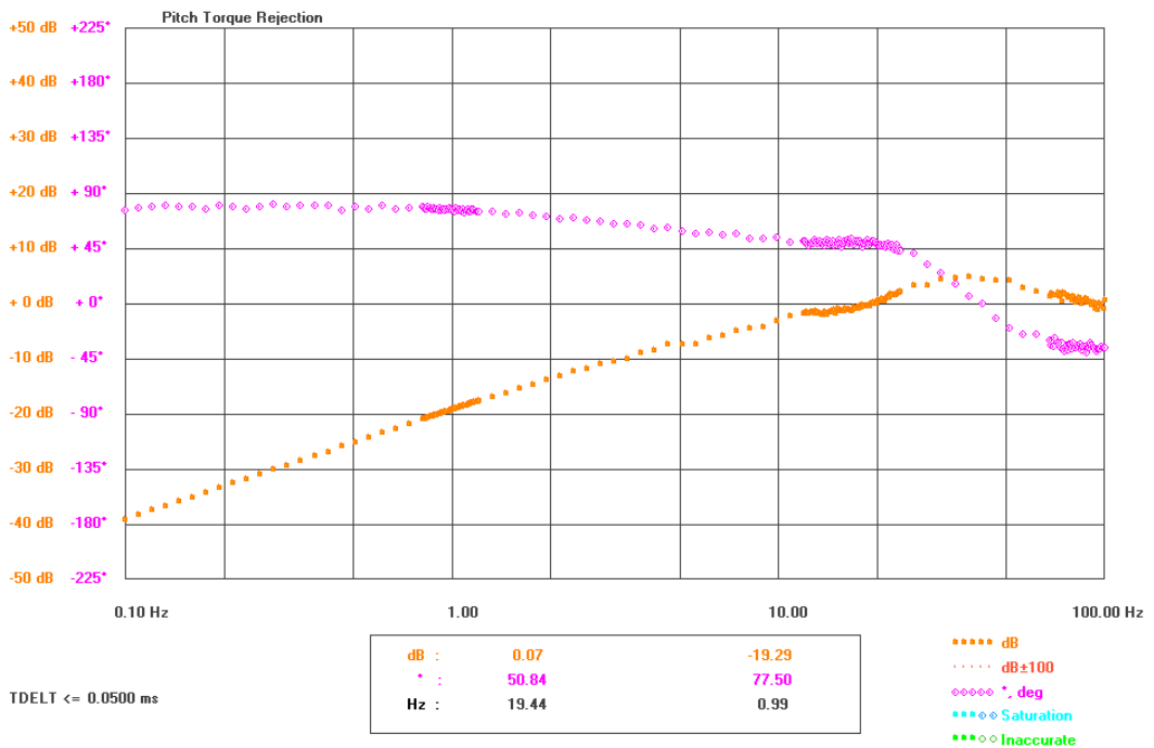
Figure 6-38: Pitch torque rejection- Pitch rate command to rate error (0.01 rad/s)
