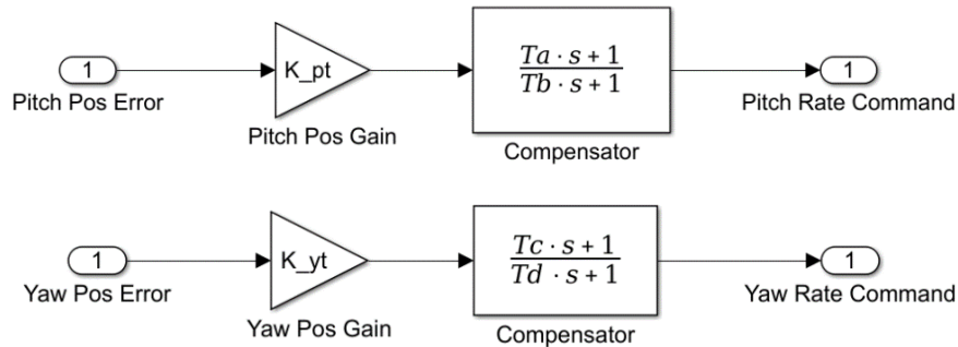
Figure 5-33: Pitch and Yaw position controllers
