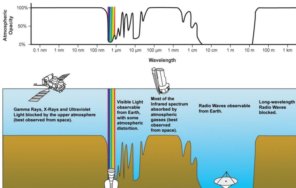
Figure 2-16: Telescopes across the EM spectrum [43]
