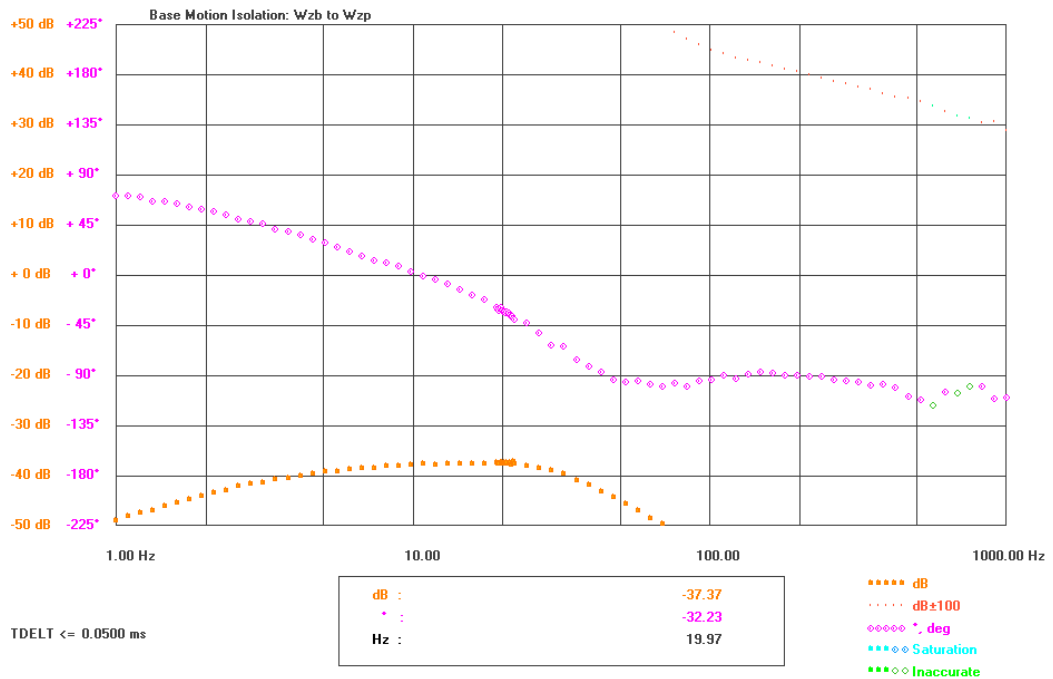
Figure 6-30: Yaw base motion isolation Bode plot with a 1.0 rad/s amplitude signal
