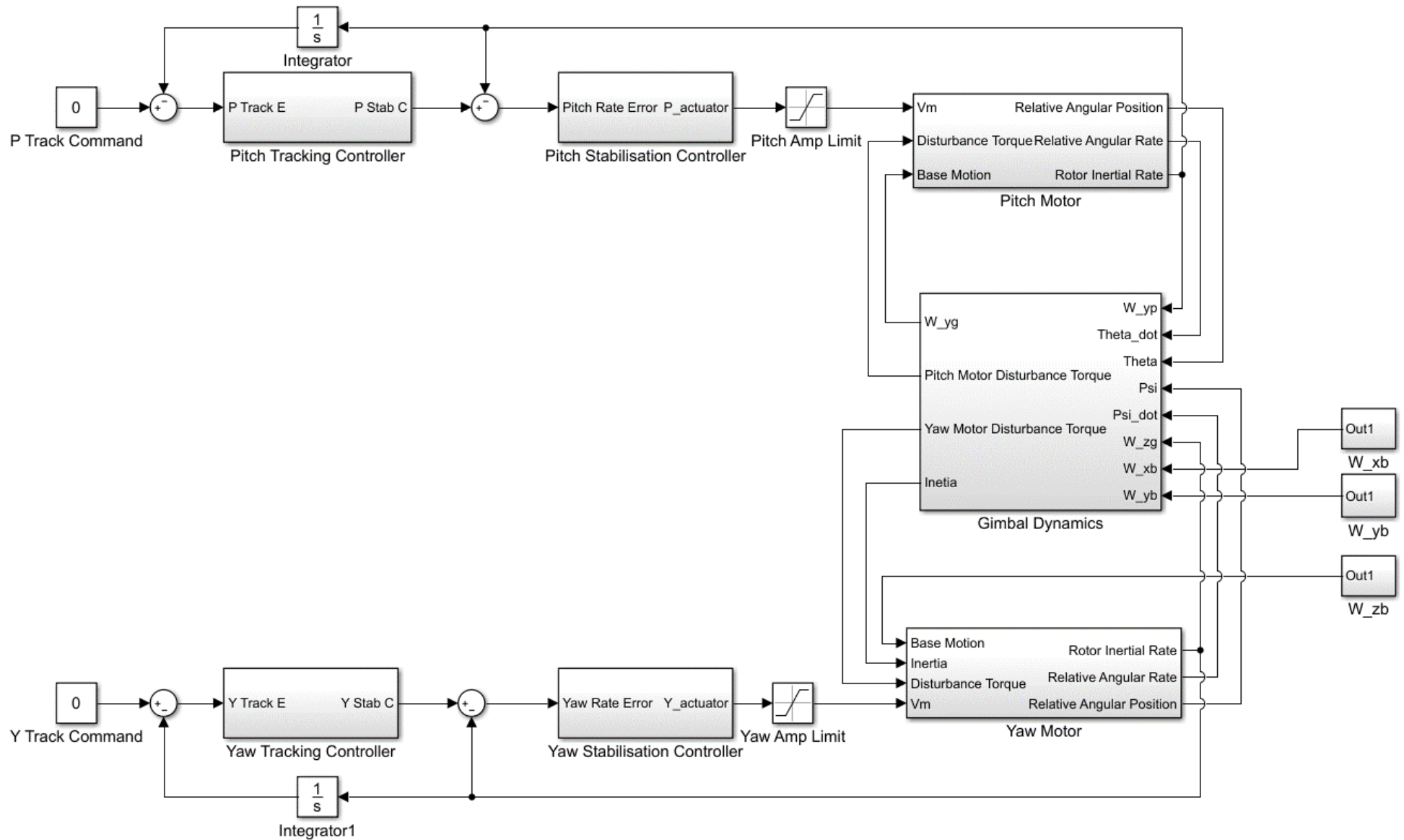
Figure 5-37: Motor selection Simulink block diagram
