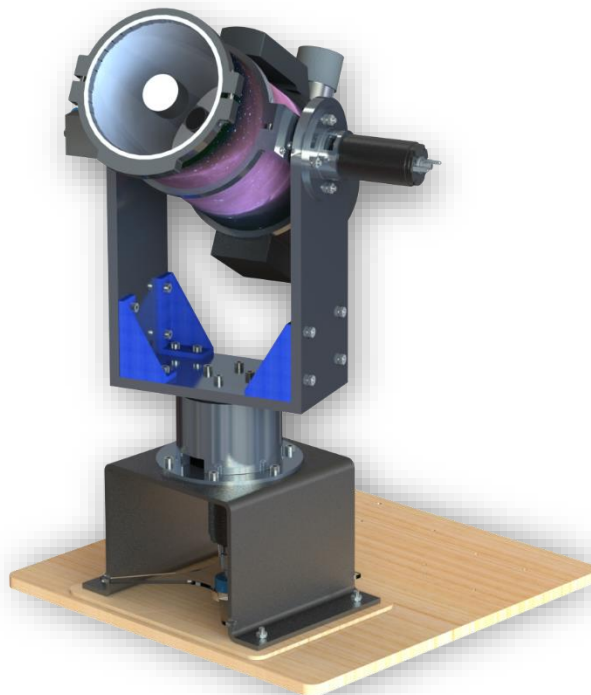
Figure 4-22: ISP assembly with the ETX90 telescope mounted
