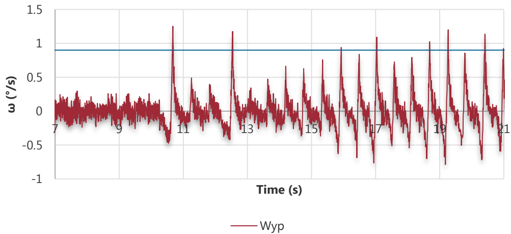
Figure 8-19: Inertial rate, \omega_{yp} , during the worst-case orientation BMI test
