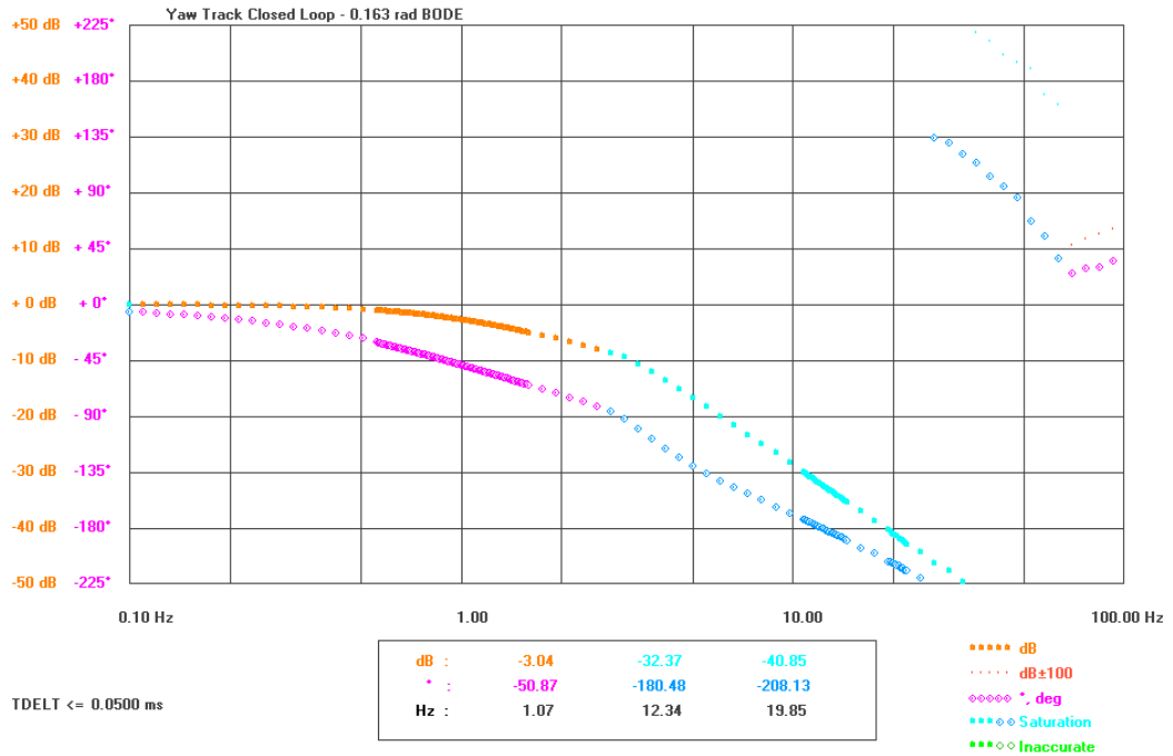
Figure 6-44: Yaw track closed-loop Bode plot - Saturated Response
