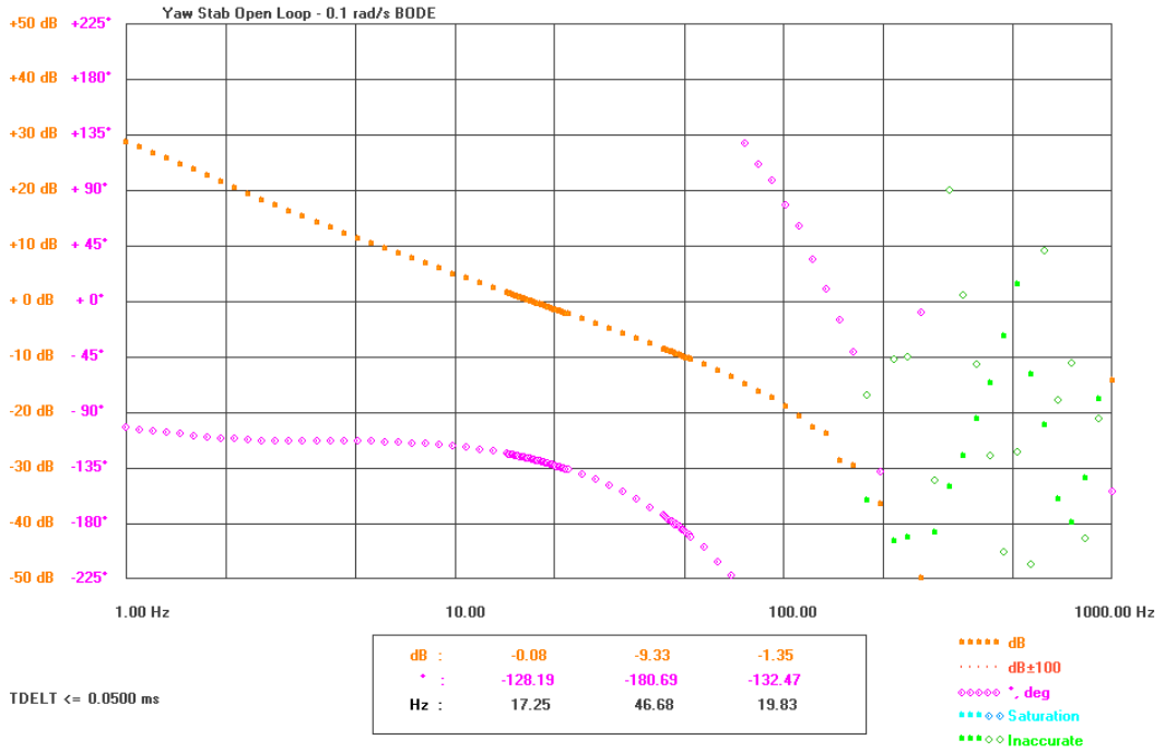
Figure 6-19: Yaw rate open-loop Bode plot - Linear Response
