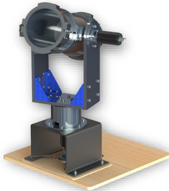
Figure 4-21: ISP assembly with the telescope modeller mounted
