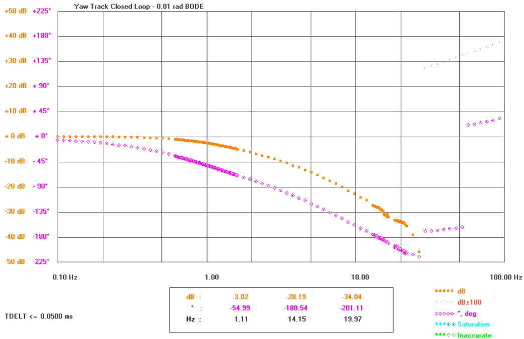
Figure 6-42: Yaw track closed-loop Bode plot - Linear Response
