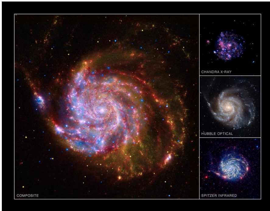
Figure 2-17: The Messier 101 galaxy observed with various frequency images [44]
