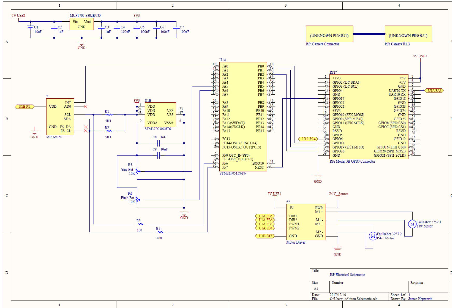
Figure 5-63: Overall electrical schematic for the ISP system
