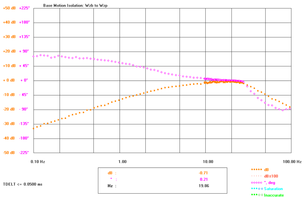
Figure 6-31: Yaw base motion isolation Bode plot with a 0.014 rad/s amplitude signal
