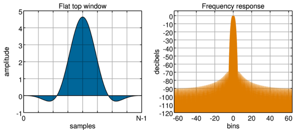
Figure 5-23: Flat Top window functions [92]
