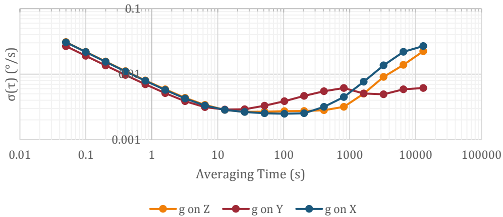
Figure 5-8: Y-Axis Allan Deviation
