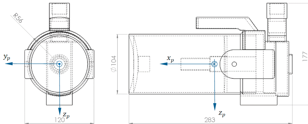
Figure 4-4: ETX90 overall dimensions
