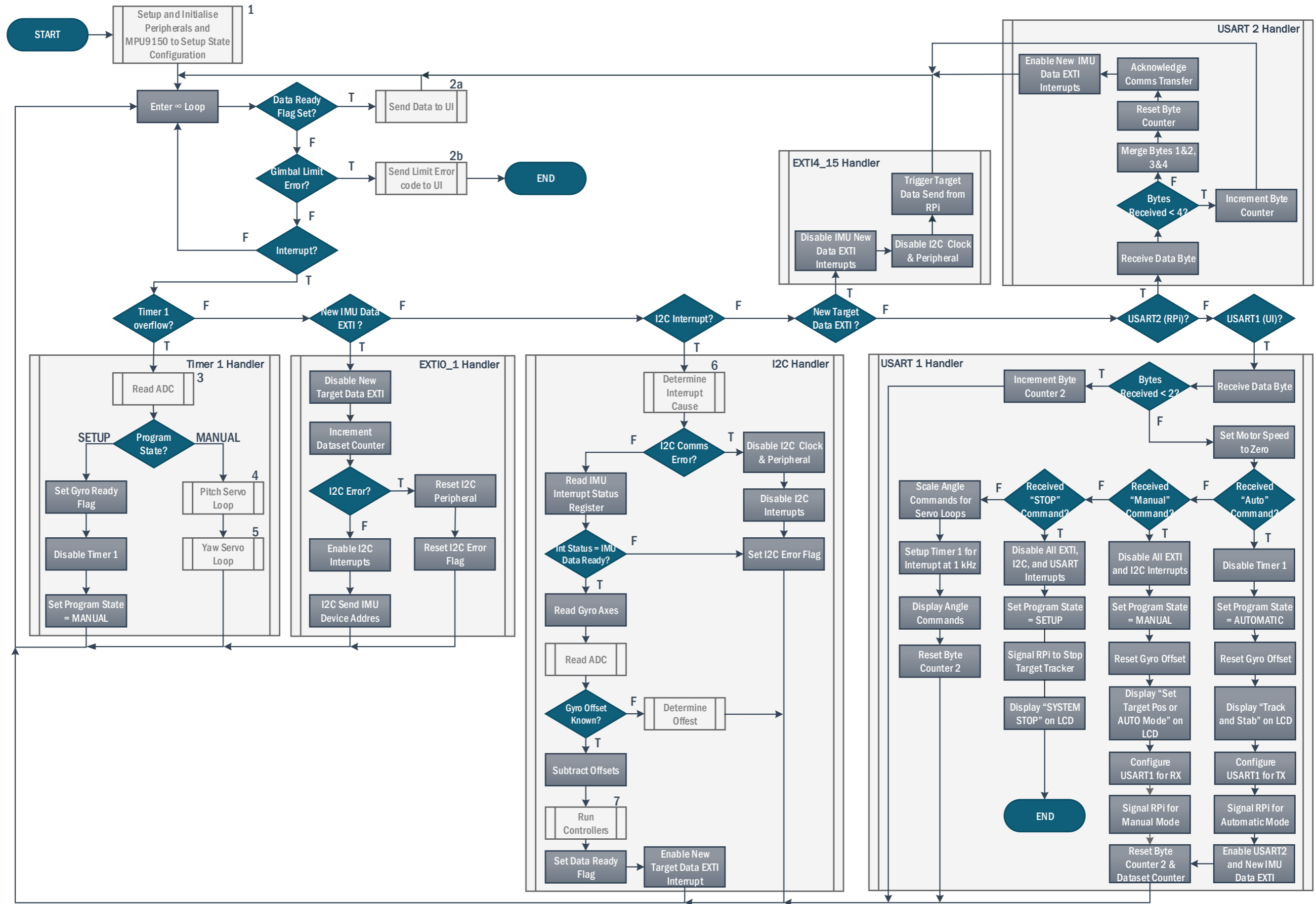
Figure 7-1: Overall Description of the STM32 Firmware
