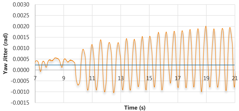
Figure 8-24: Yaw jitter from the worst-case test
