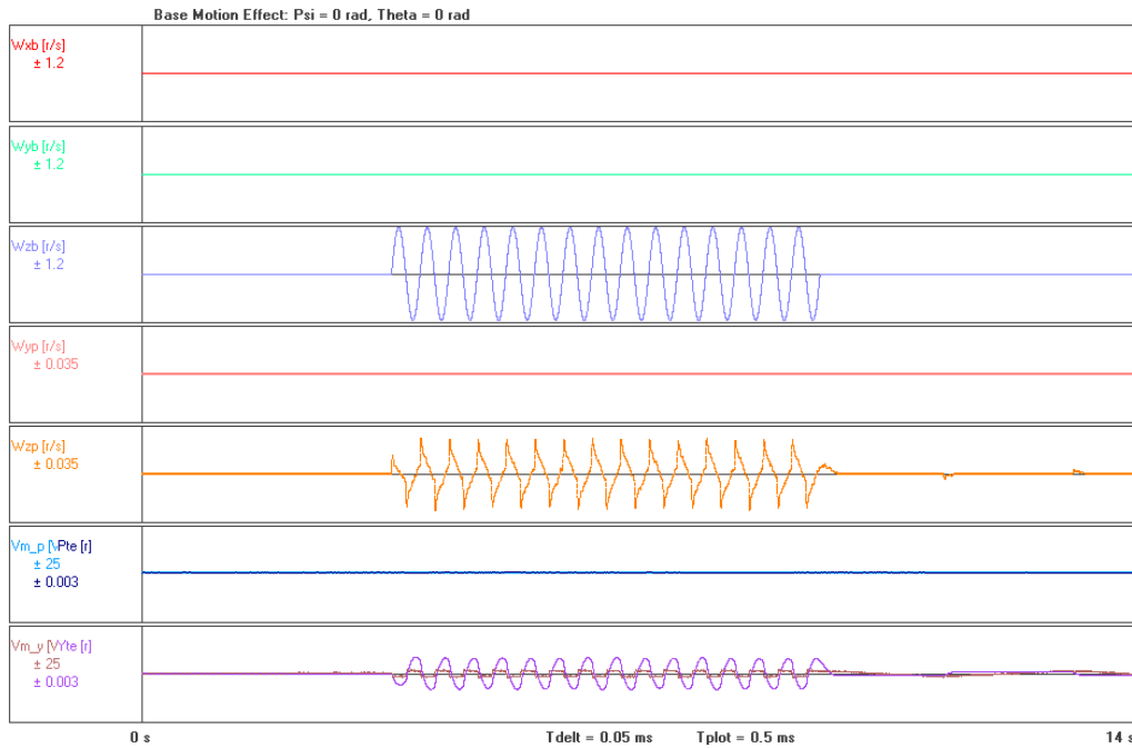
Figure 8-15: Yaw channel base motion isolation with corrected friction model
