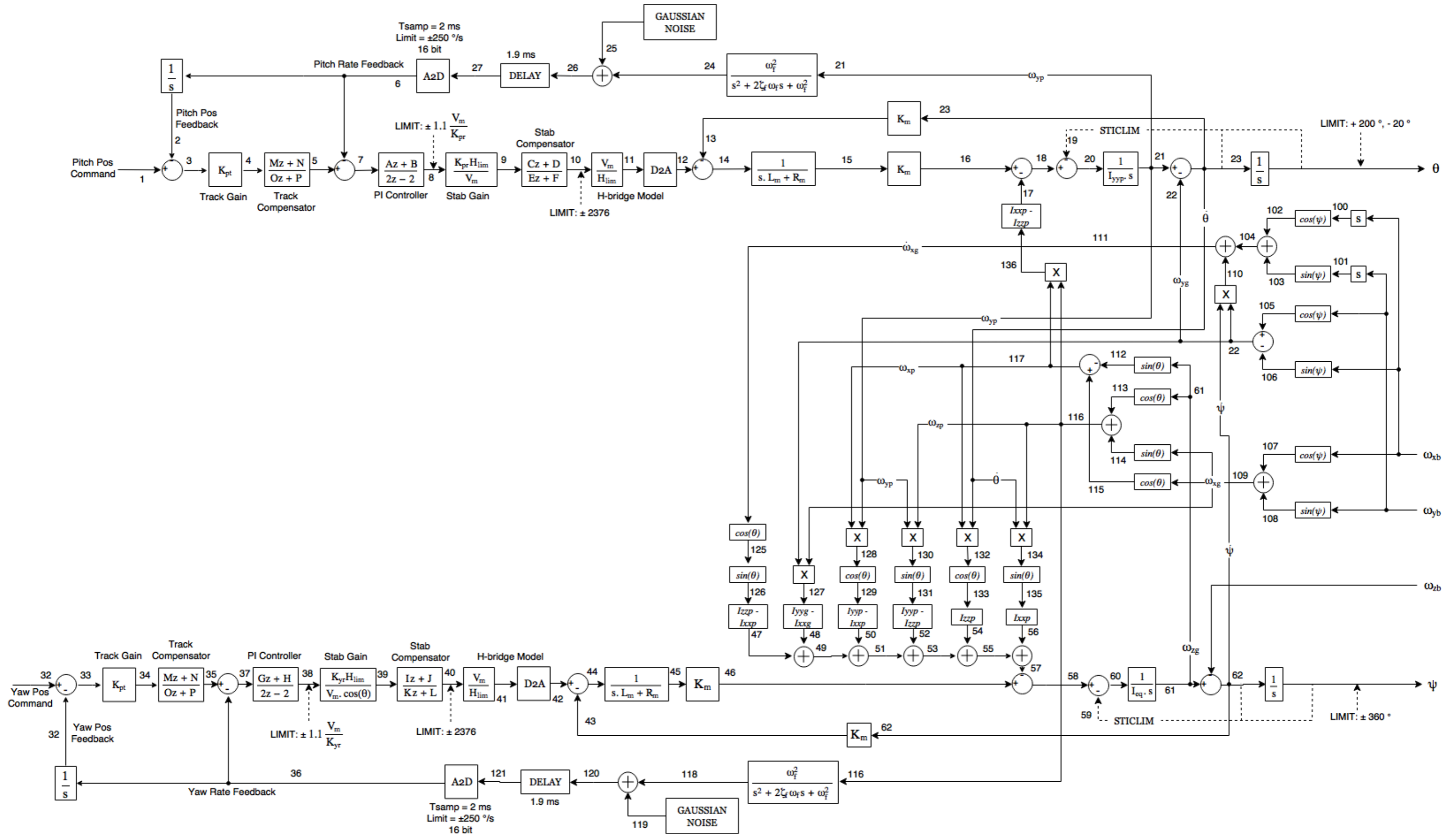
Figure 6-40: ISP model with tracking loops included around the stabilisation loops
