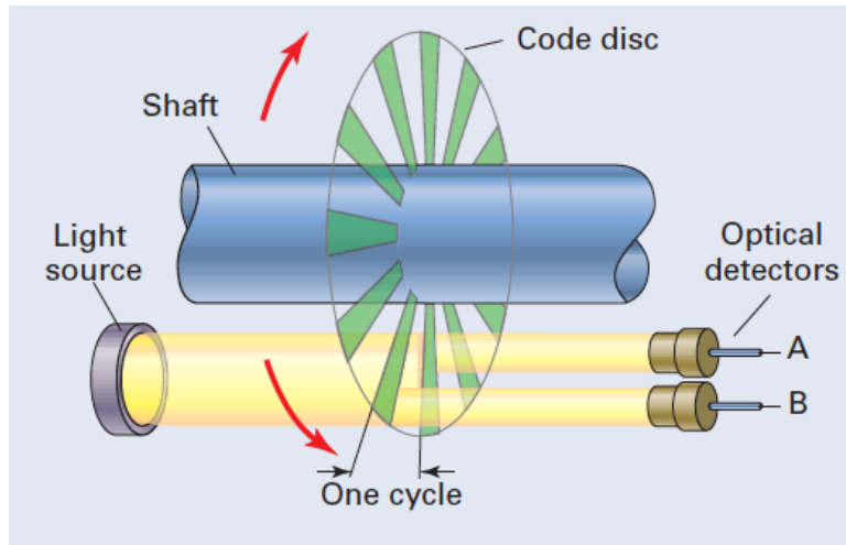
Figure 5-11: Workings of an Optical Encoder [76]
