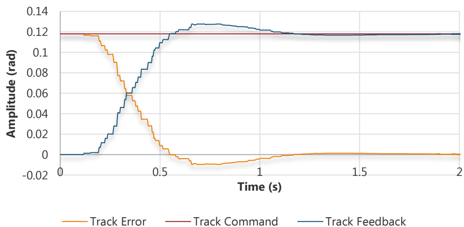
Figure 8-1: Step Tracking response of the yaw channel
