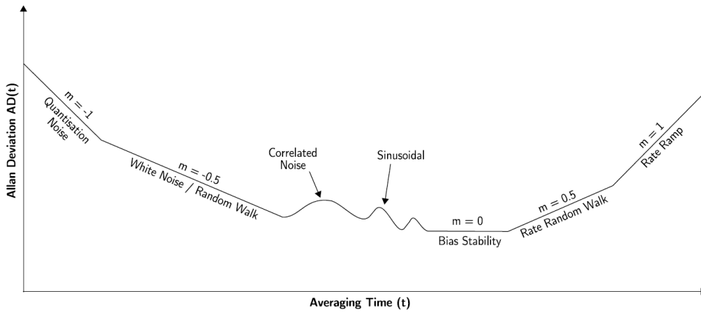
Figure 2-13: A typical Allan Variance plot [30]
