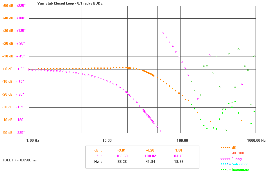
Figure 6-20: Yaw rate closed-loop Bode plot - Linear Response
