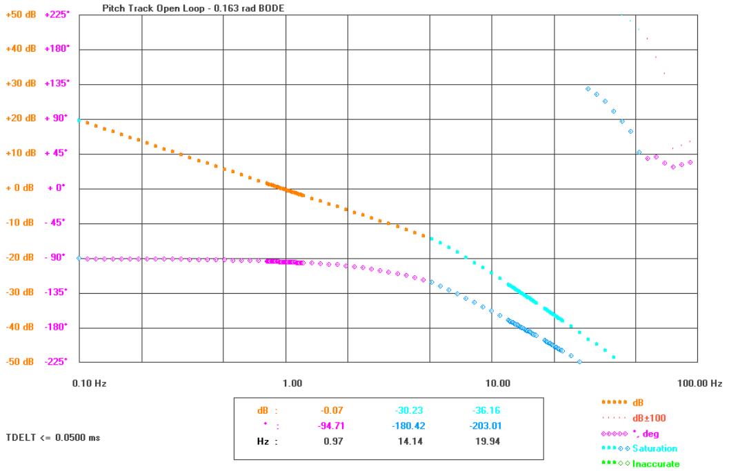
Figure 6-47: Pitch track open-loop Bode plot - Saturated Response
