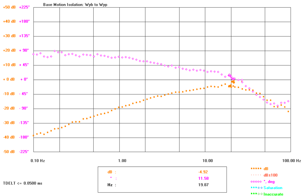
Figure 6-33: Pitch base motion isolation Bode plot with a 0.01 rad/s amplitude signal
