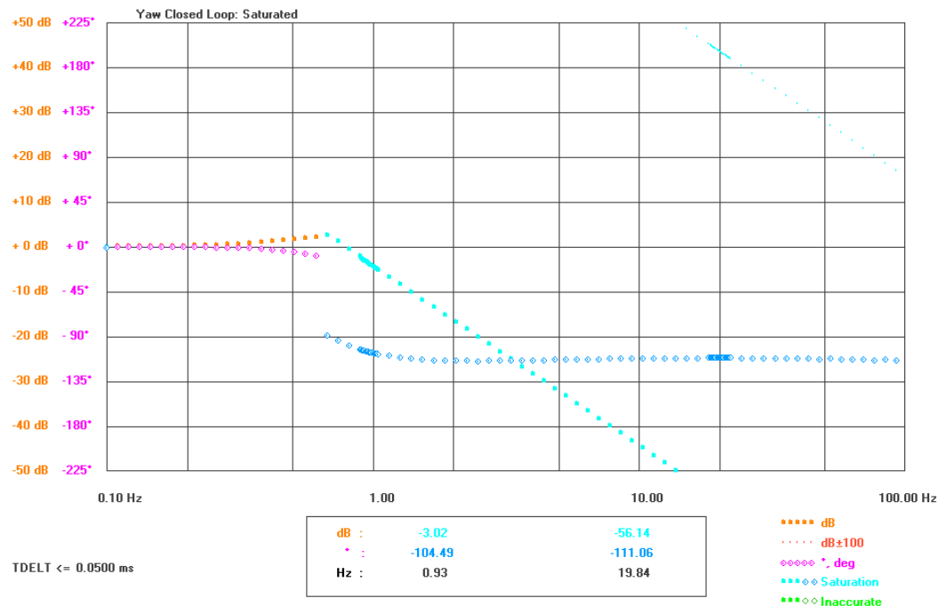
Figure 6-11: Saturated closed-loop response of the yaw manual position controller
