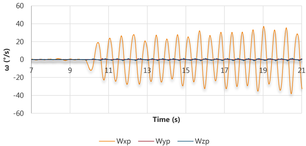
Figure 8-18: Inertial rates of the telescope modeller during the worst-case orientation BMI test
