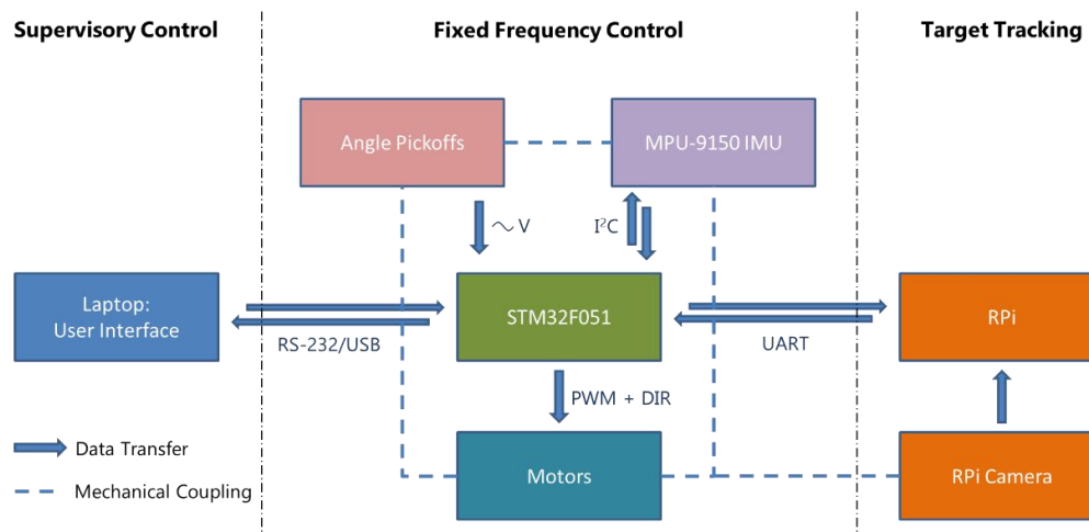
Figure 5-62: Control hardware configuration
