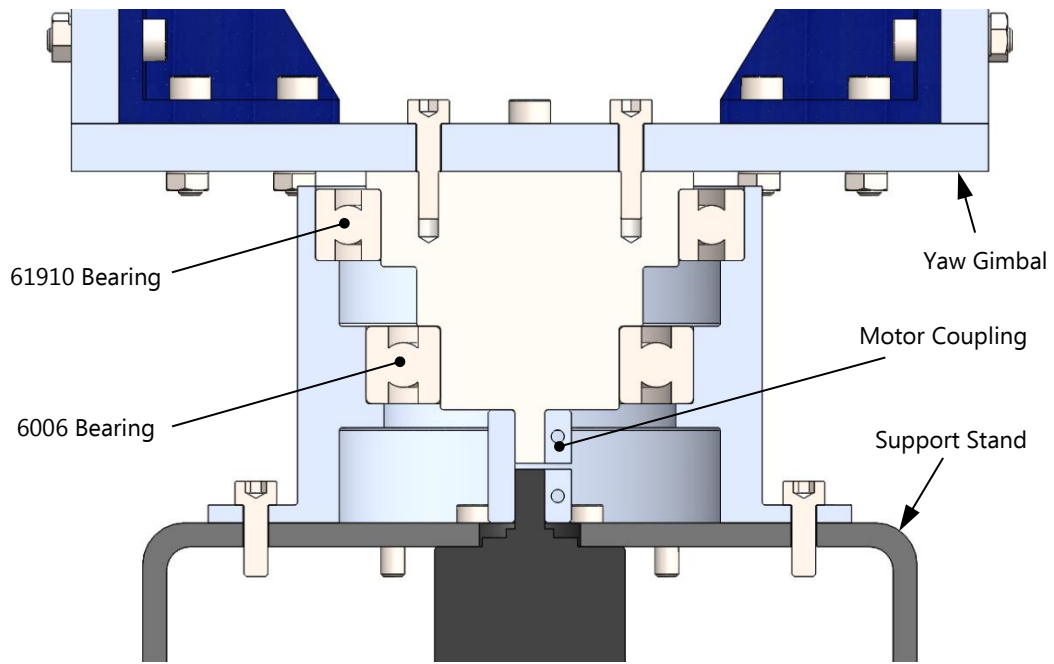
Figure 4-20: Section view of the yaw gimbal mounted on the support stand
