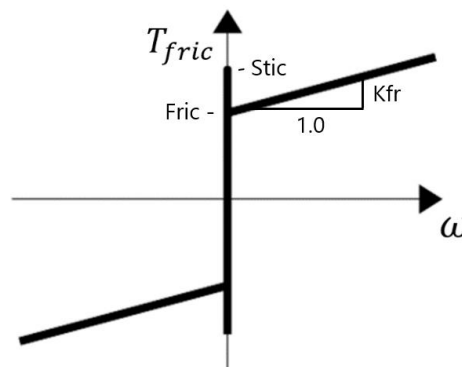
Figure 6-2: Stiction function friction model (Adapted from [103])
