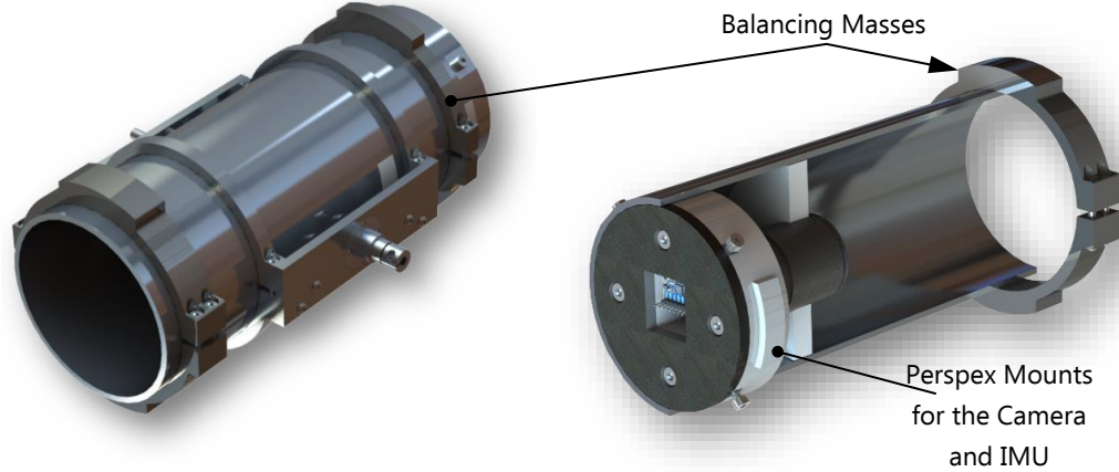
Figure 4-11: Final ETX90 modelling camera mounting platform
