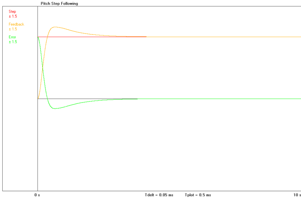
Figure 6-7: Step response of the pitch manual position controller
