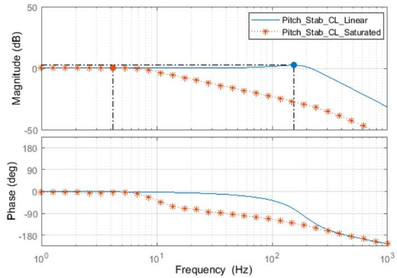
Figure 5-43: Motor selection simulation - Pitch rate closed-loop bode plot
