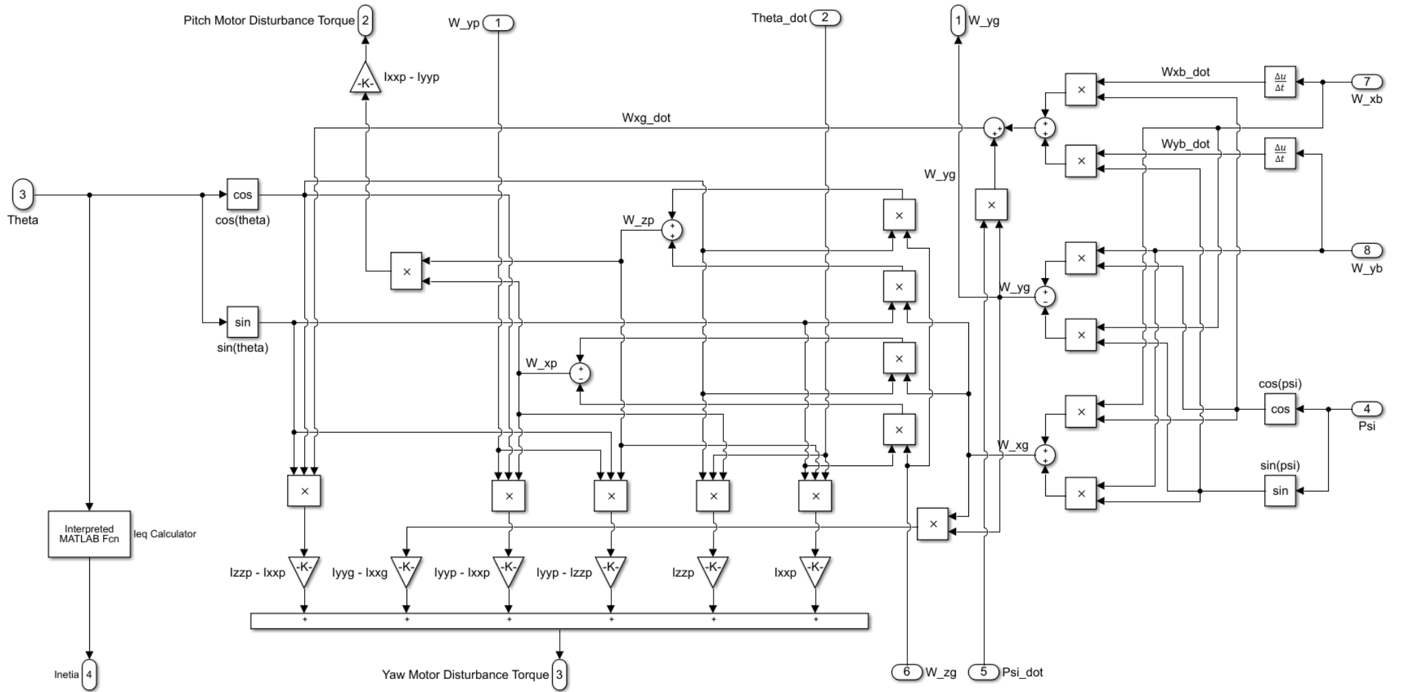
Figure 5-36: Gimbal dynamics block diagram
