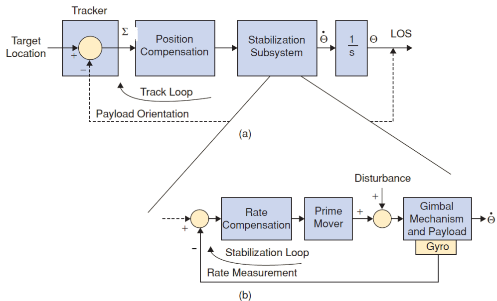
Figure 2-7: Cascade control structure [7]
