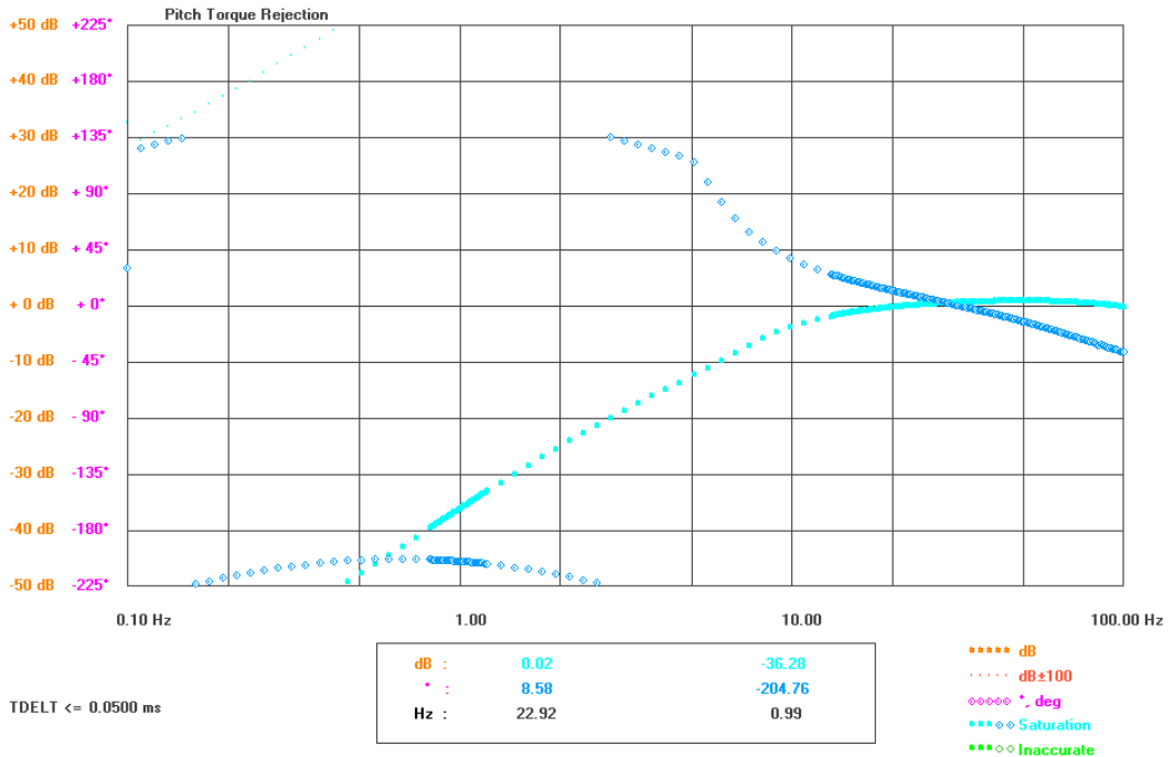
Figure 6-37: Pitch torque rejection- Pitch rate command to rate error (1.0 rad/s)
