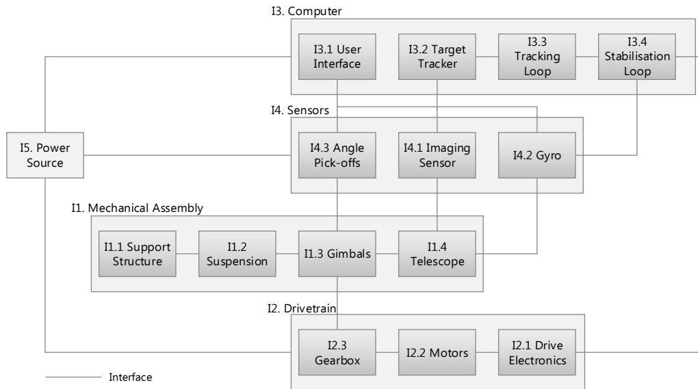
Figure A-1: Prime item diagram
