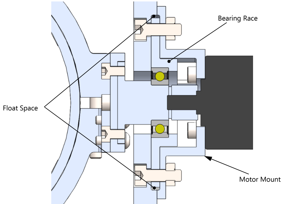
Figure 4-18: Detailed section view of the motor-side mounting of the telescope modeller
