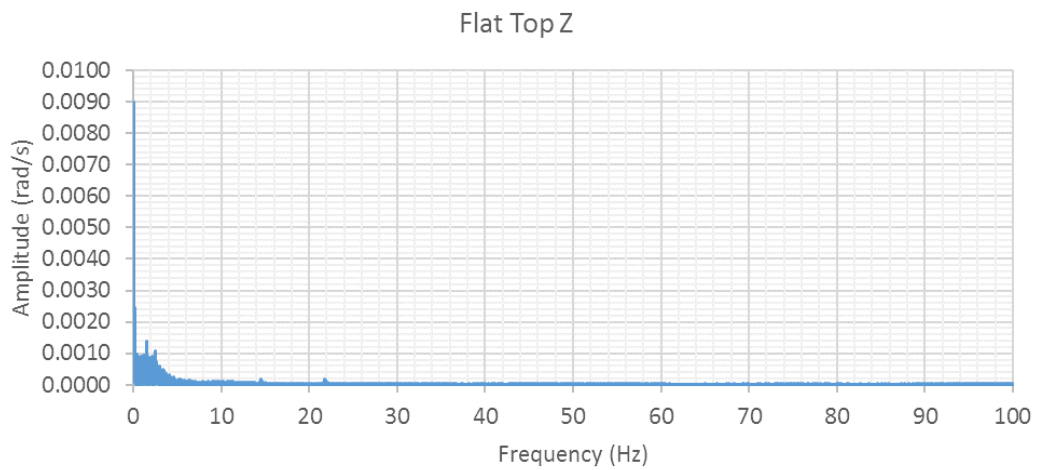
Figure 5-27: Amplitude vs Frequency of the z_{imu} data of Test 2 under the Flat Top window
