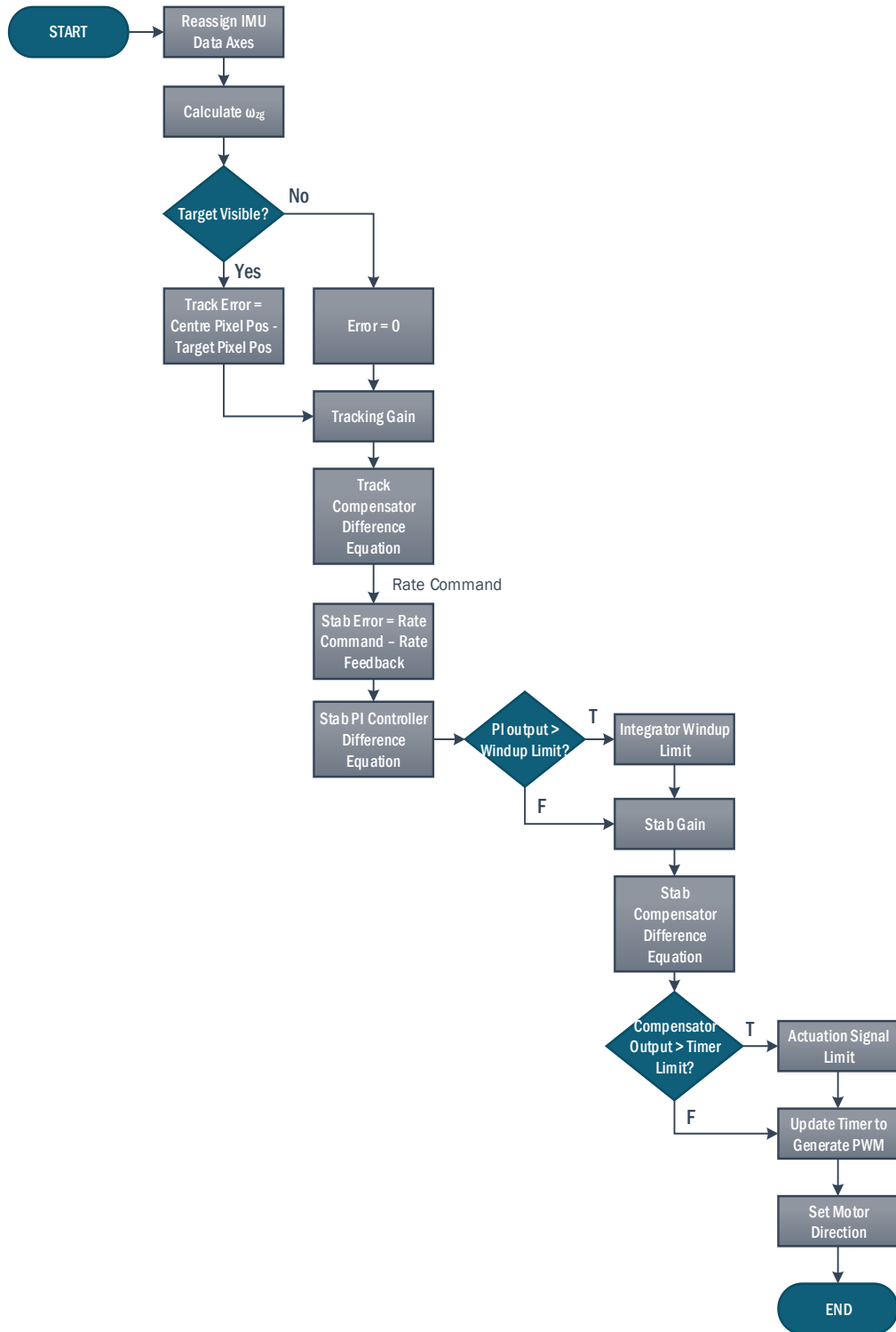
Figure 7-6: Implementation of the Controller function which runs the tracking and stabilisation control loops
