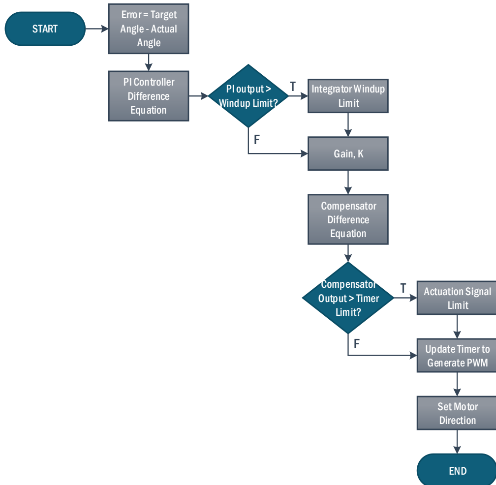
Figure 7-4: Gimbal positioning servo loop implementation
