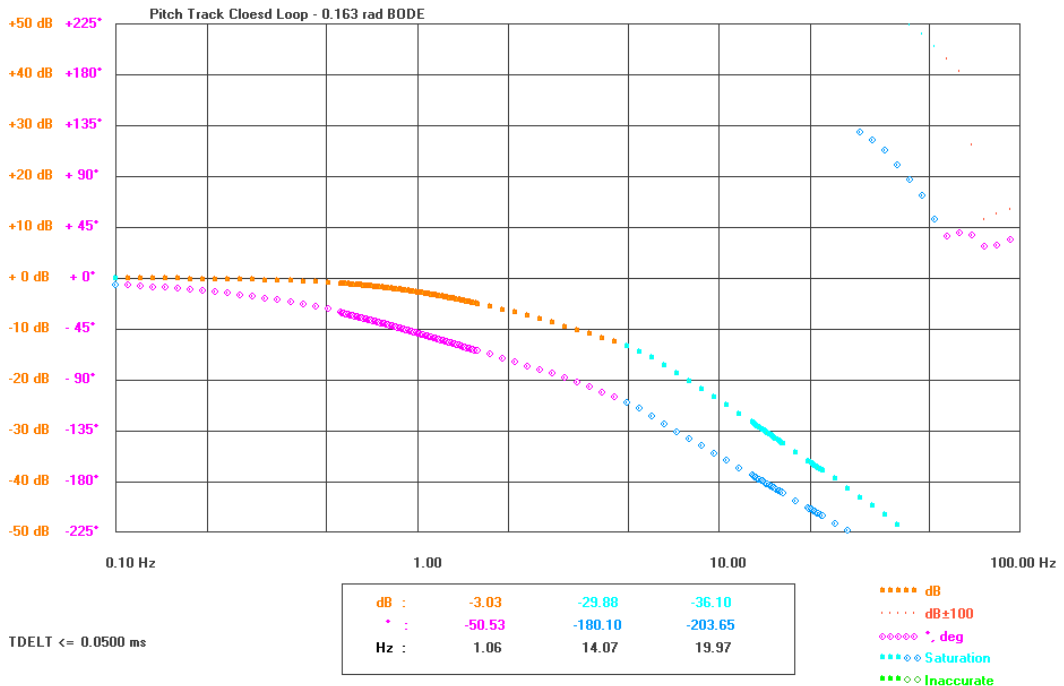
Figure 6-48: Pitch track closed-loop Bode plot - Saturated Response
