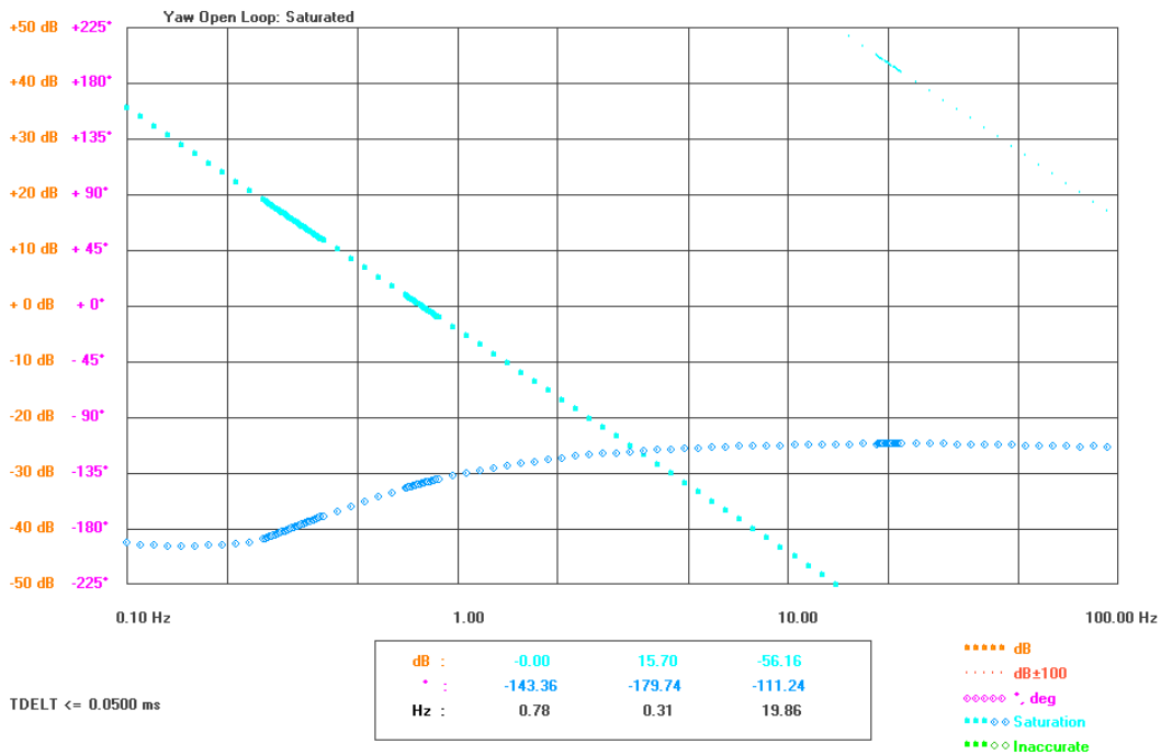
Figure 6-9: Saturated open-loop responses of the yaw manual position controller
