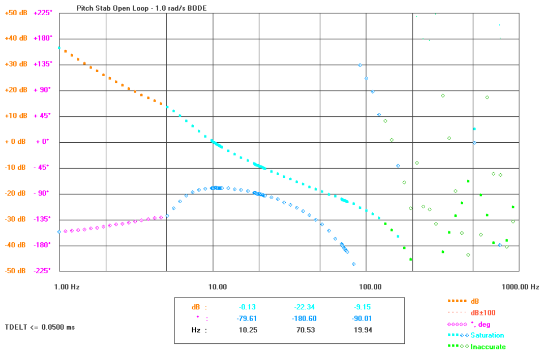
Figure 6-25: Pitch rate open-loop Bode plot - Saturated Response
