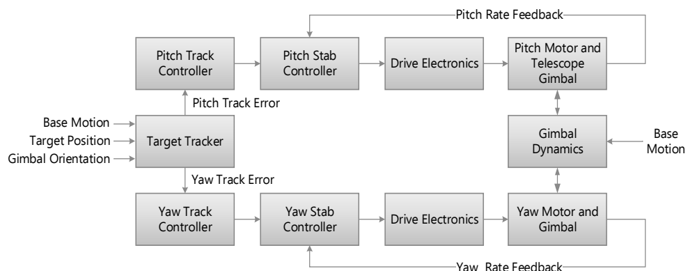
Figure 6-53: System Identification Diagram of the model with the Target Tracker included
