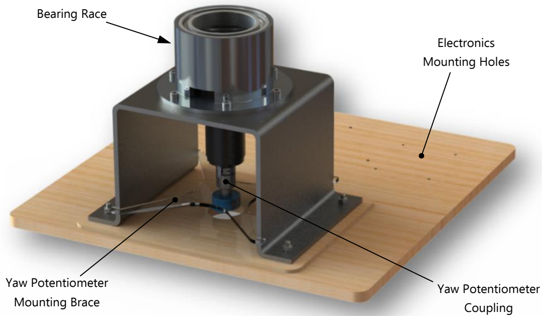
Figure 4-19: Support stand final design
