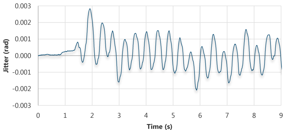
Figure 8-16: Yaw channel jitter estimation
