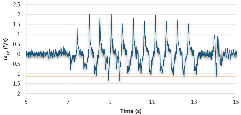
Figure 8-8: Inertial rate, \omega_{yb} , for the pitch channel BMI test
