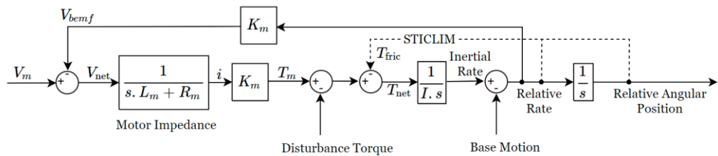
Figure 6-14: Motor model used for the ISP system simulation
