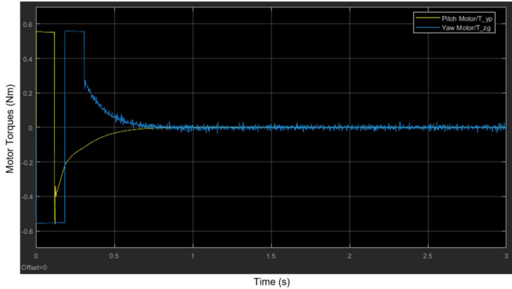
Figure 5-57: Motor Torques for the worst-case position
