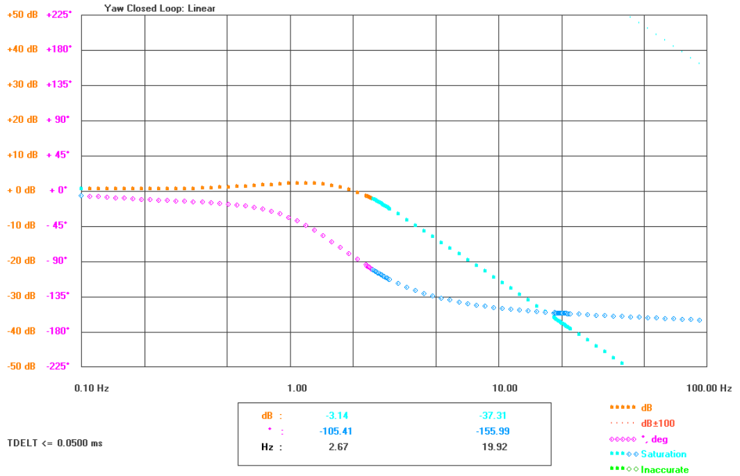
Figure 6-10: Linear closed-loop response of the yaw manual position controller
