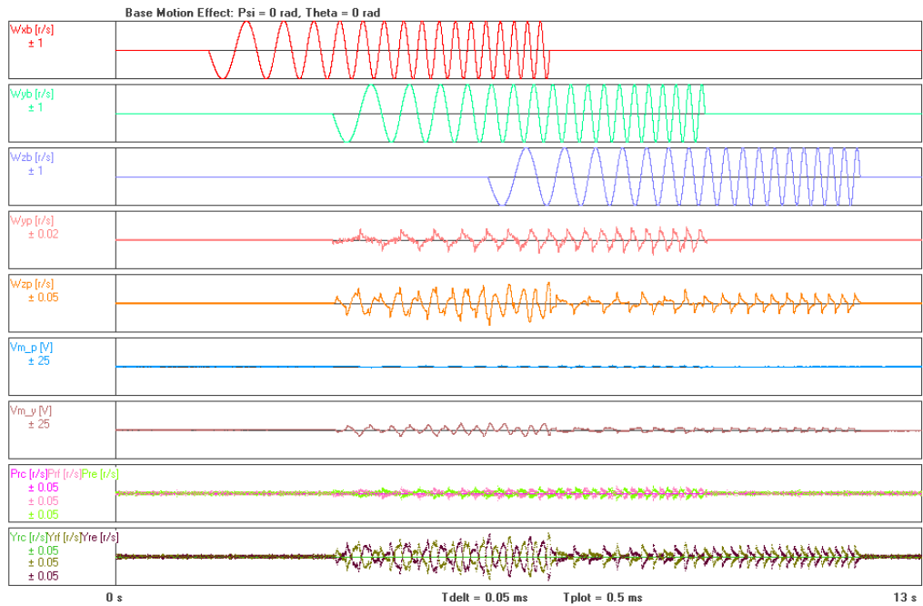
Figure 6-28: 1.0 rad/s base motion effects when \psi = \theta = 0^\circ
