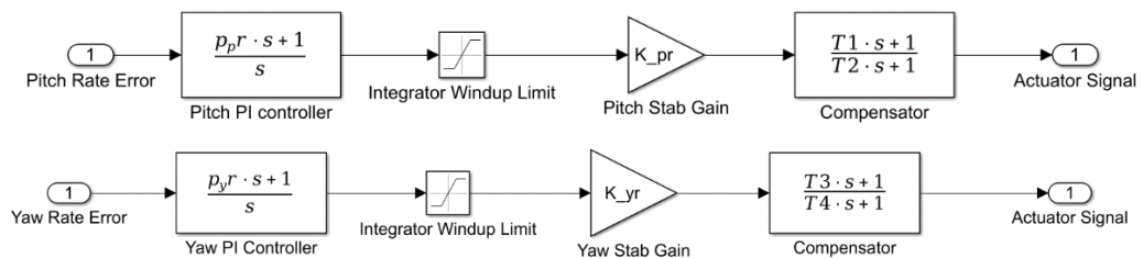
Figure 5-34: Pitch and Yaw stabilisation controllers
