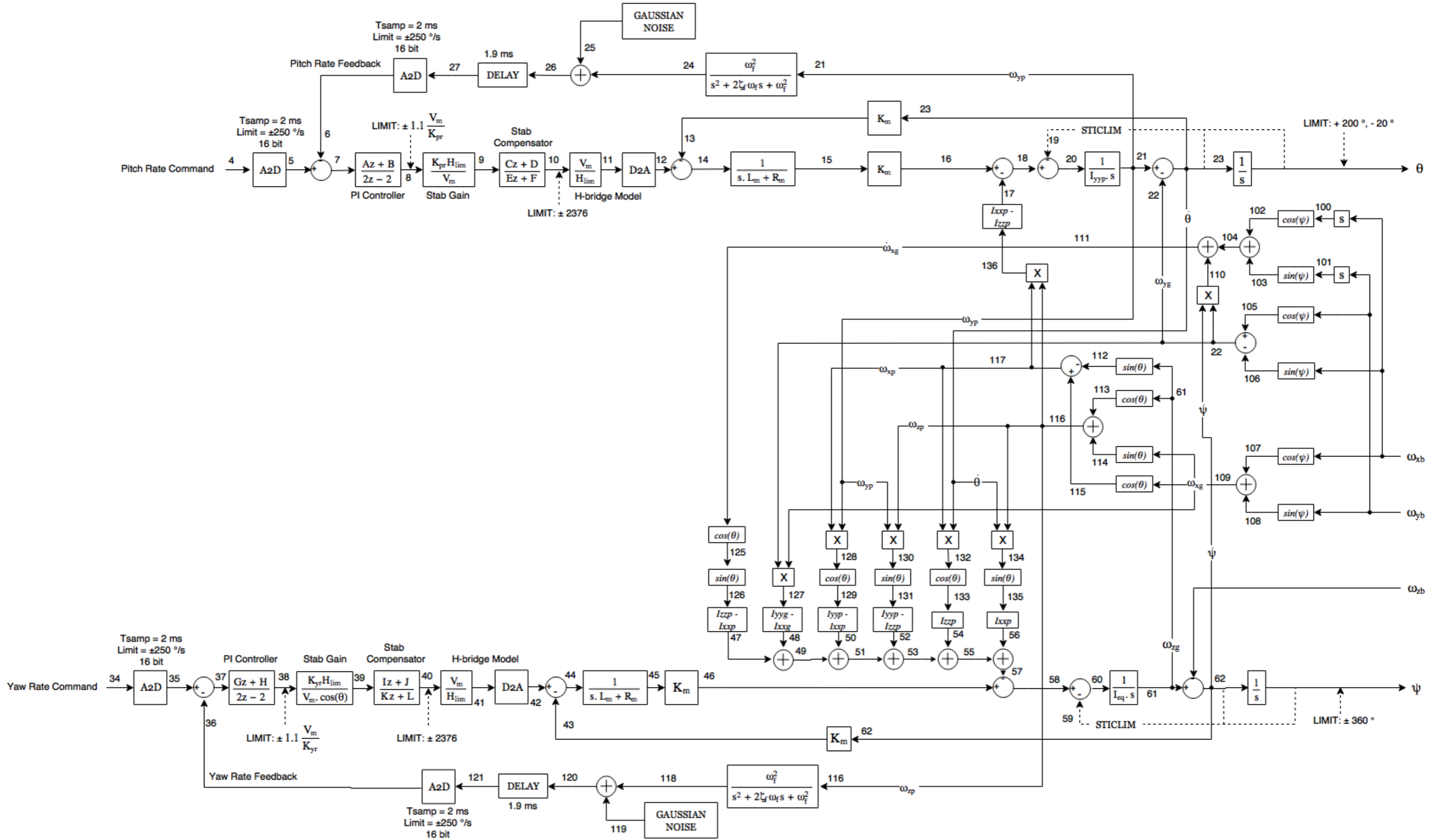
Figure 6-17: Final ISP stabilisation loop block diagram
