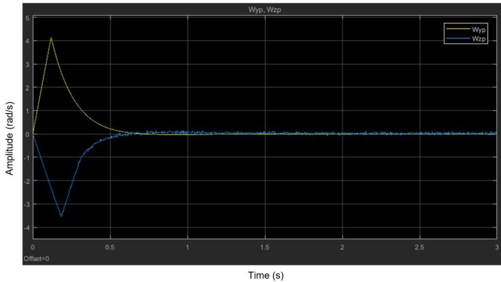
Figure 5-56: Inertial rates of the telescope in the worst-case position
