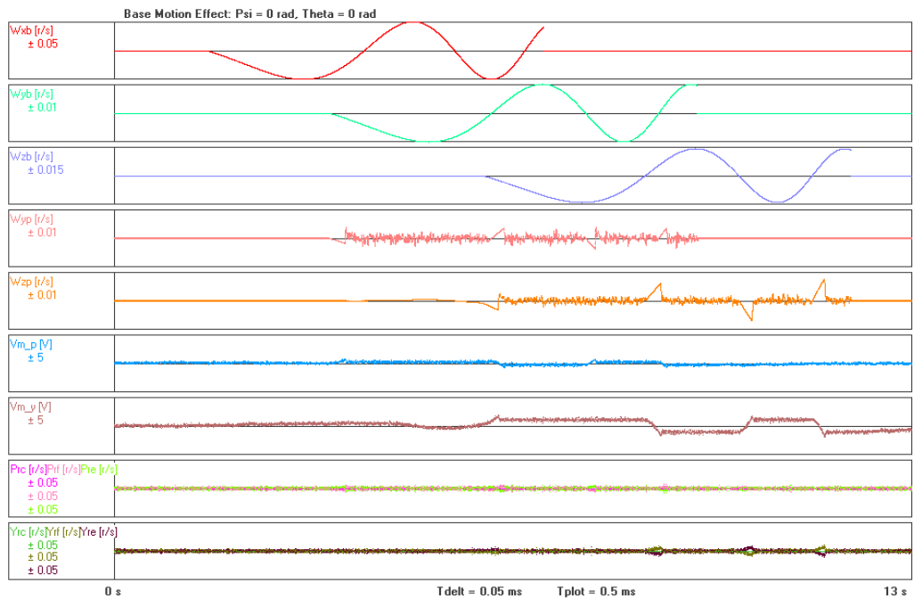
Figure 6-29: Simulated base motion signal peak effects when \psi = \theta = 0^\circ
