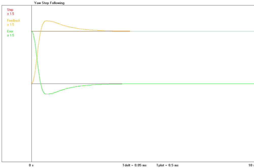
Figure 6-12: Step response of the yaw manual position controller
