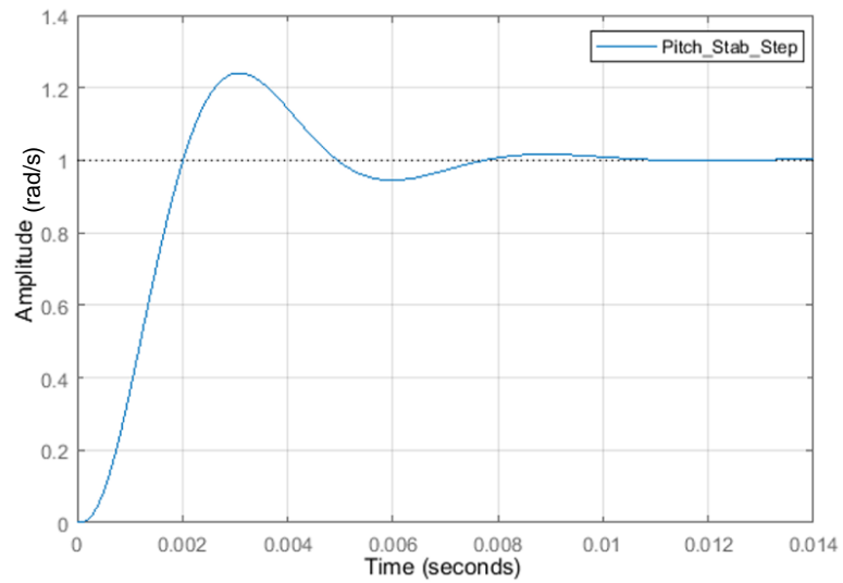
Figure 5-44: Motor selection simulation - Pitch rate step following
