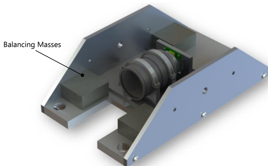
Figure 4-6: Raspberry Pi Camera mounted on Mounting Concept 1
