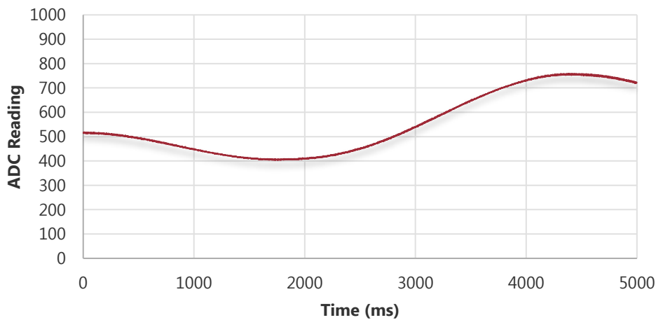
Figure 5-68: ADC readings with pot rails connected to VSSA and VDDA in parallel with C8 and C9
