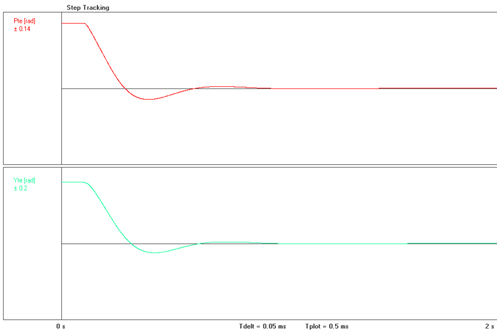
Figure 8-3: Simulated step tracking with the test command signals
