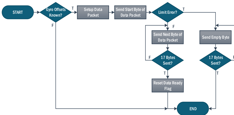
Figure 7-3: STM32 to UI data transfer function
