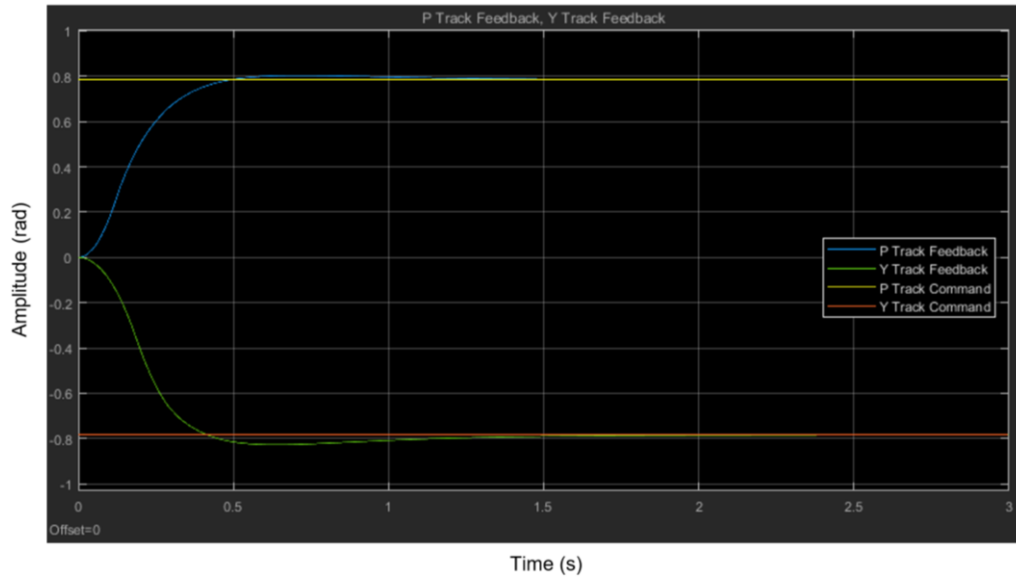
Figure 5-55: Position command following for the worst-case position
