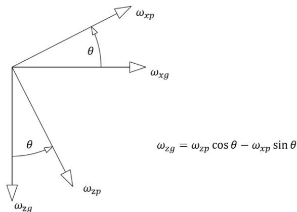
Figure 6-18: Derivation of \omega_{zg} from \omega_{zp} and \omega_{xp}
