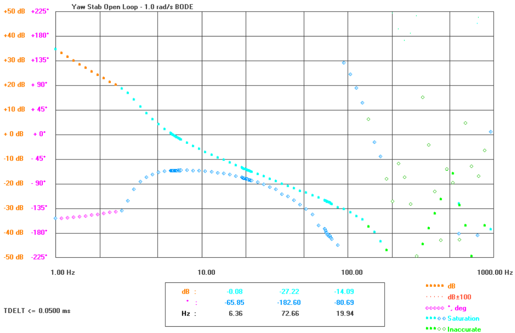
Figure 6-21: Yaw rate open-loop Bode plot - Saturated Response
