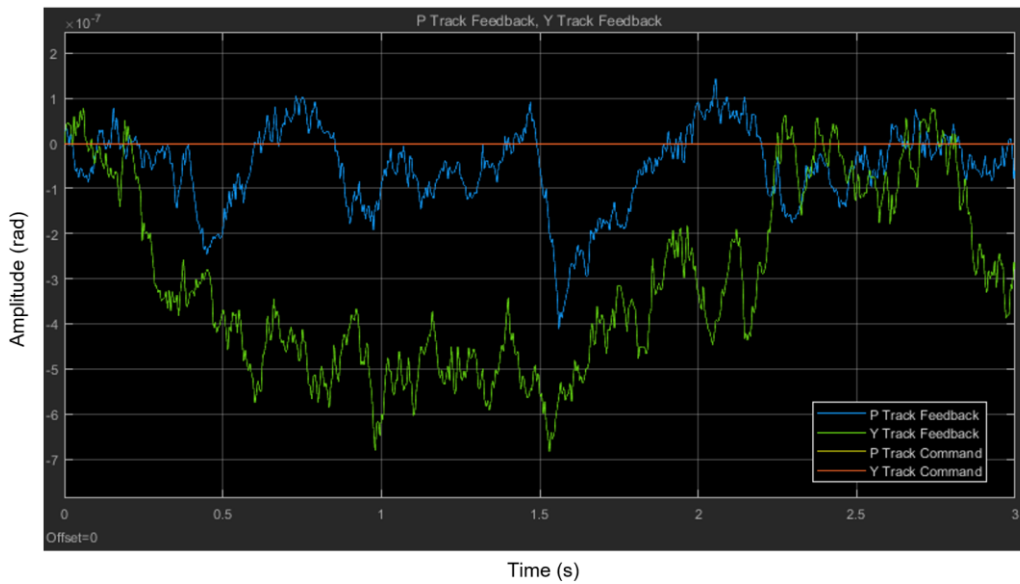
Figure 5-52: Home orientation position command following
