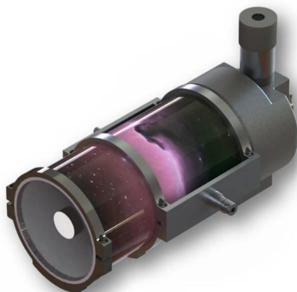
Figure 4-9: ETX90 final mounting design
