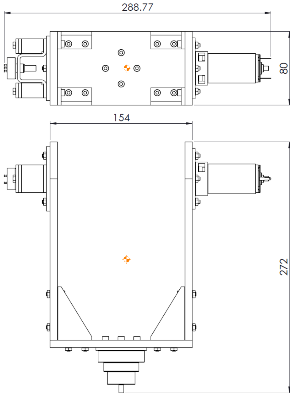
Figure 4-15: Yaw gimbal overall dimensions
