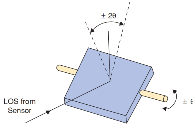
Figure 2-5: Optical doubling effect [7]
