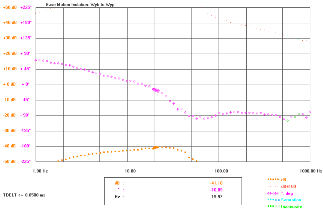
Figure 6-32: Pitch base motion isolation Bode plot with a 1.0 rad/s amplitude signal
