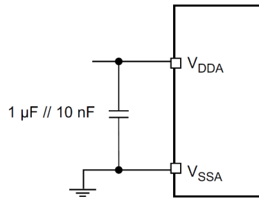
Figure 5-67: Power supply decoupling capacitors recommended by STMicroelectronics for 36, 48, and 64 pin package STM32 microcontrollers such as the STM32F051 [101]
