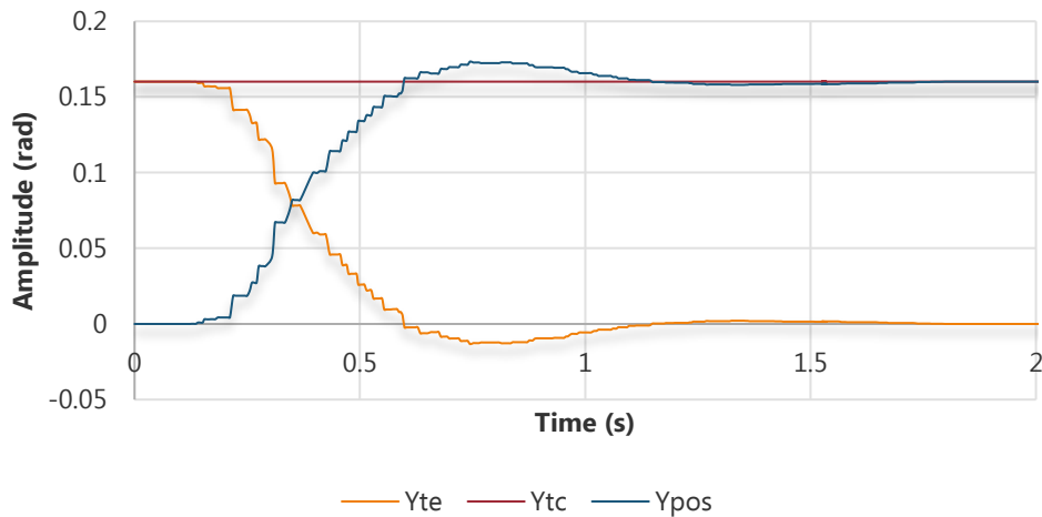
Figure 8-2: Step tracking response of the pitch channel
