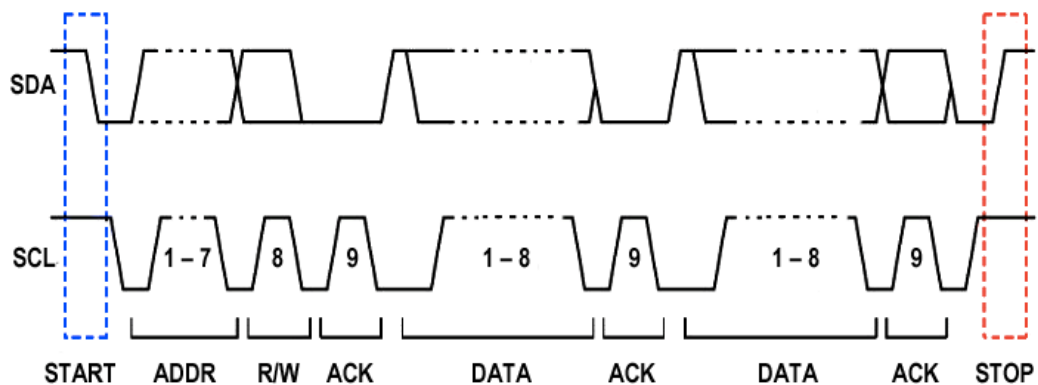
Figure 5-64: I 2 C protocol for 7-bit address devices [99]
