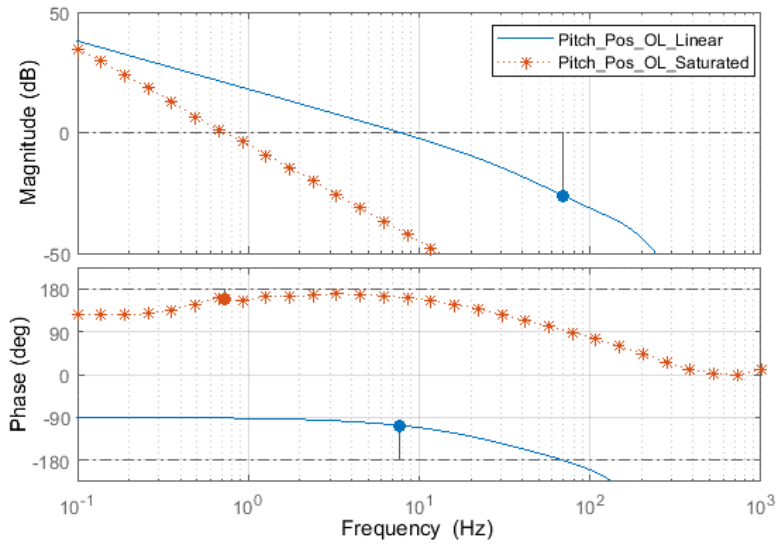
Figure 5-48: Motor selection simulation - Pitch position open-loop bode plot
