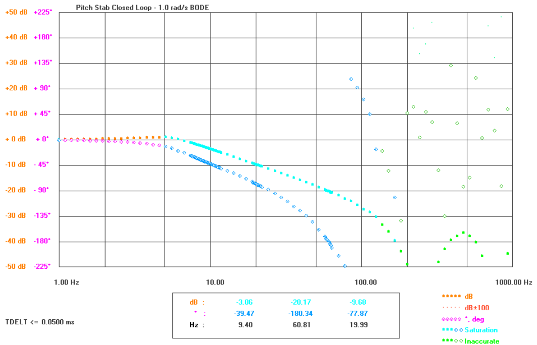
Figure 6-26: Pitch rate closed-loop Bode plot - Saturated Response
