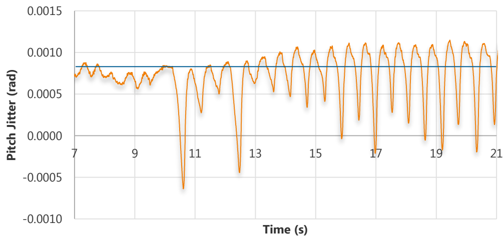
Figure 8-23: Pitch jitter estimate from the worst-case test
