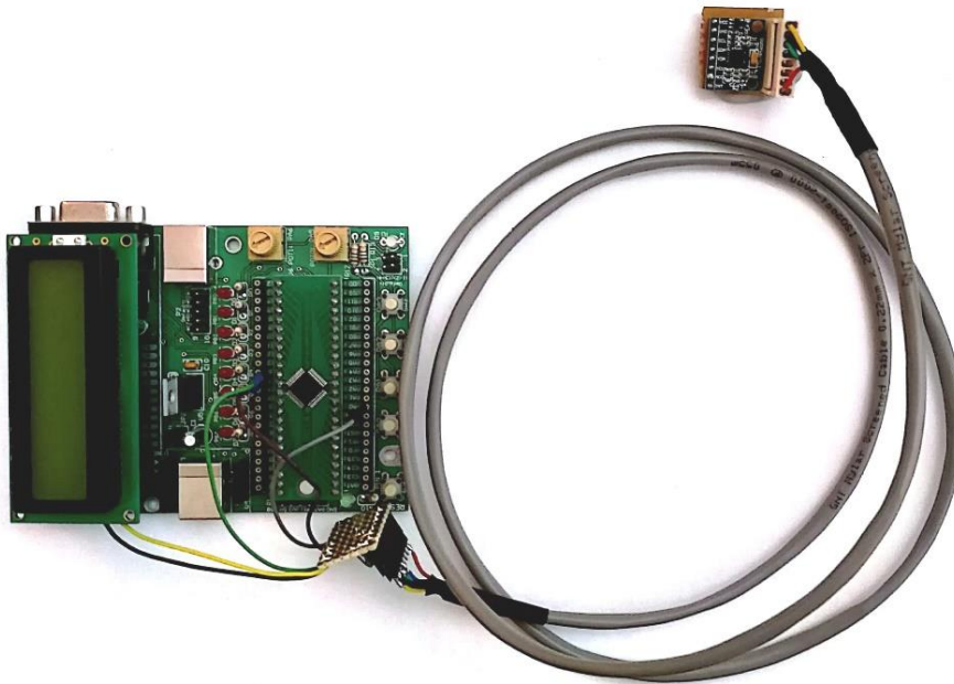
Figure 5-65: MPU-9150 to STM32F051 connection
