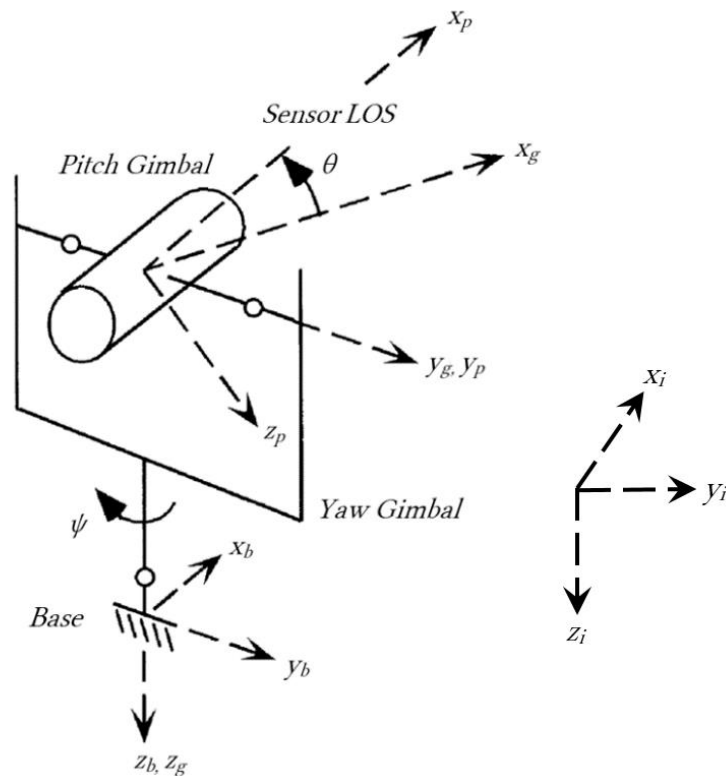
Figure 2-21: Double gimbal schematic. Adapted from [53]
