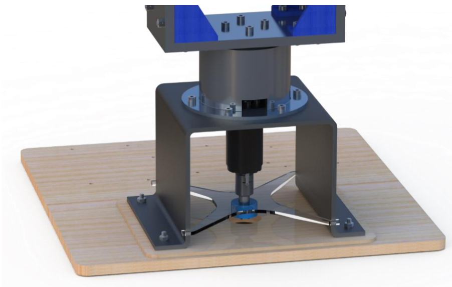
Figure 5-17: Yaw pot mounting position
