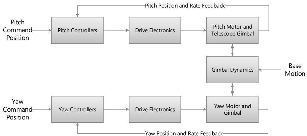
Figure 5-31: System identification diagram for a two-axis gimbal system
