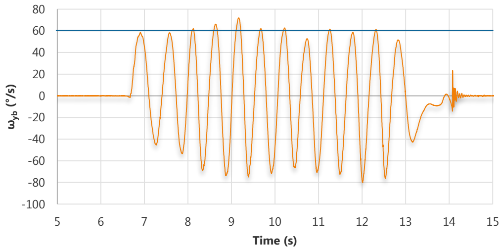
Figure 8-7: Base motion, \omega_{yb} , for the pitch channel BMI test in the home position
