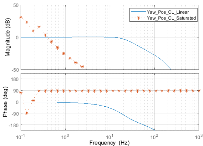
Figure 5-46: Motor selection simulation - Yaw position closed-loop bode plot
