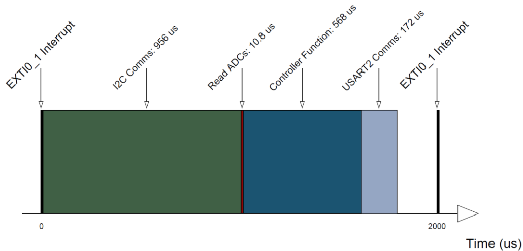
Figure 7-7: Automatic state firmware timing
