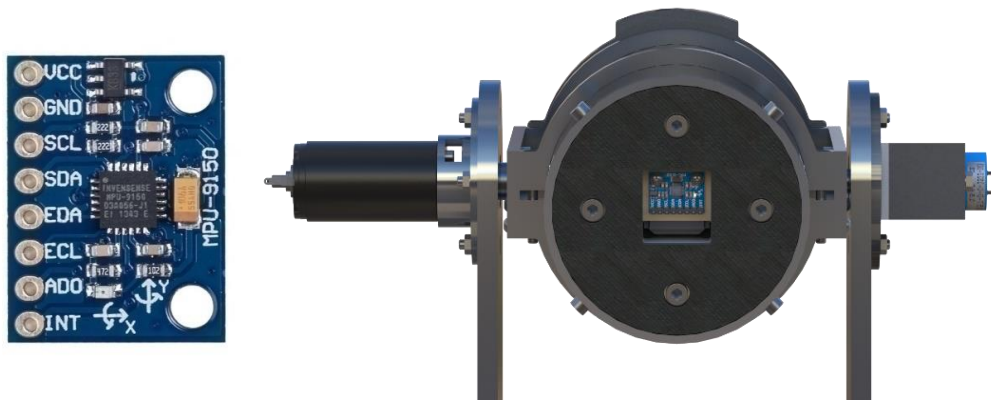
Figure 5-10: MPU-9150 [75] and its mounted location
