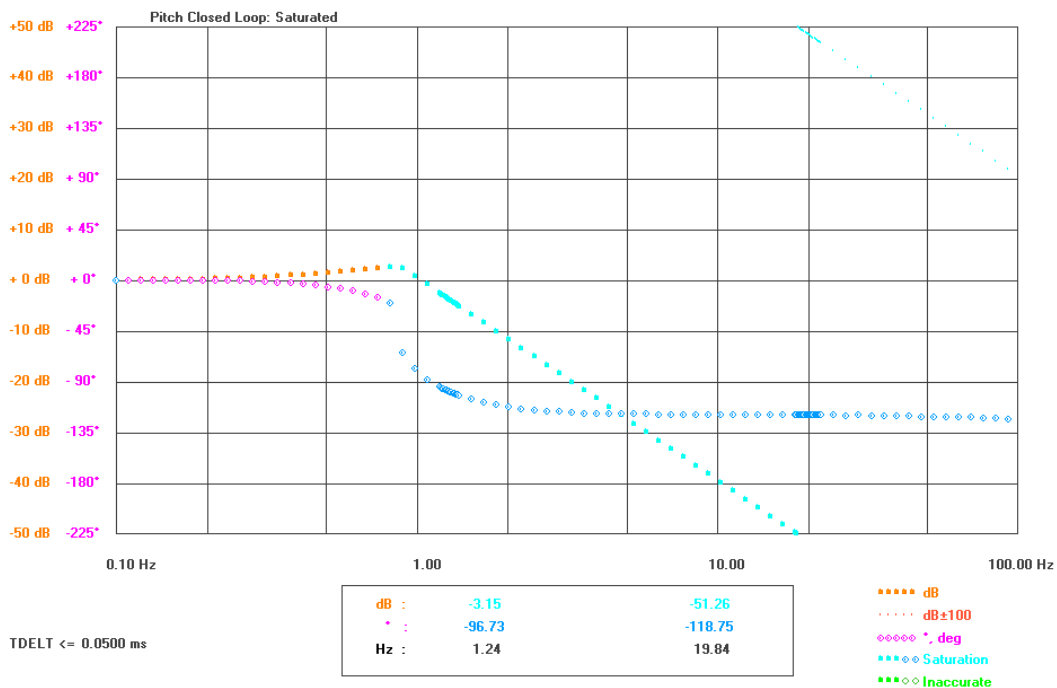
Figure 6-6: Saturated closed-loop responses of the pitch manual position controller
