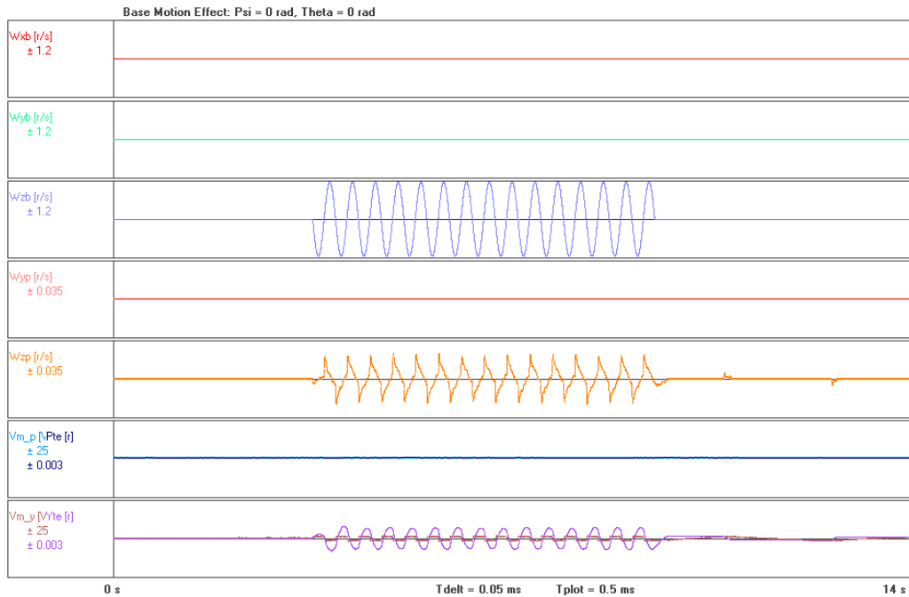
Figure 8-14: Simulation response to a 2.5 Hz, 66.50 °/s \omega_{zb} signal
