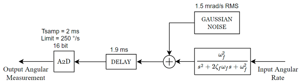
Figure 6-16: Final gyro model used in the ISP simulation
