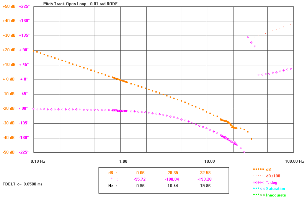
Figure 6-45: Pitch track open-loop Bode plot - Linear Response
