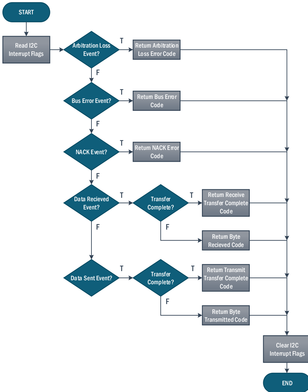
Figure 7-5: I2C interrupt cause determination function
