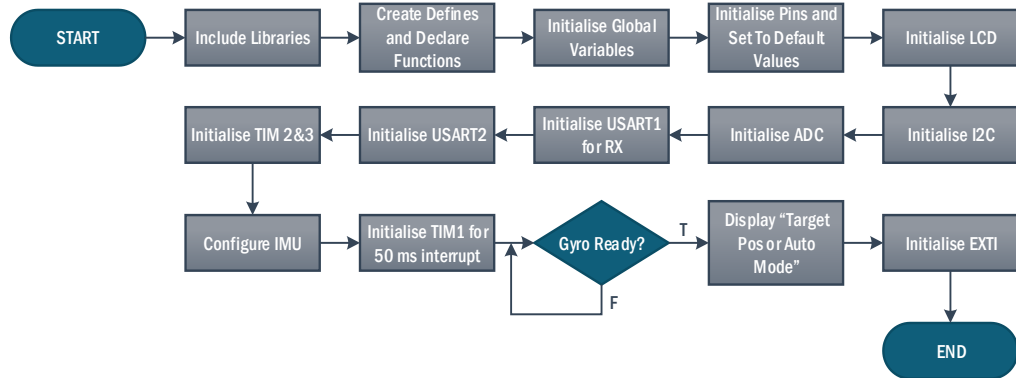
Figure 7-2: Setup and Initialisation subprocess
