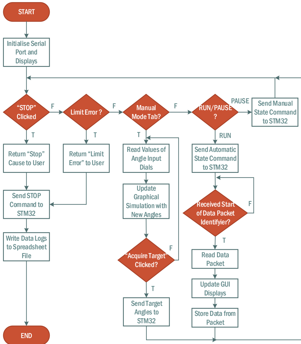
Figure 7-22: Functional flowchart of the User Interface software operation
