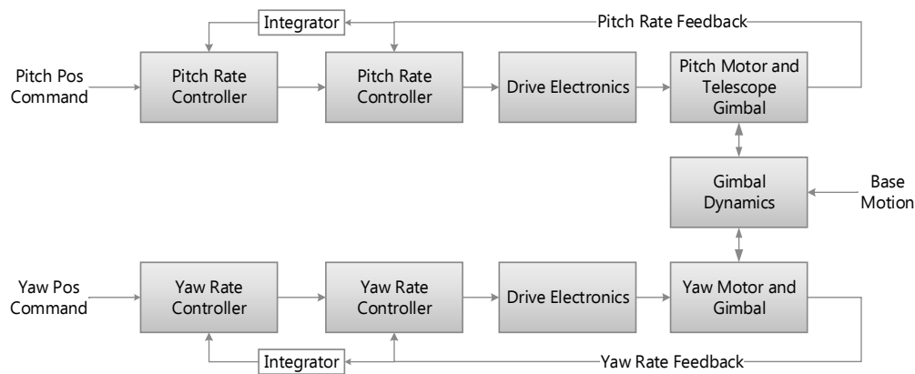
Figure 6-39: System identification block diagram for the ISP control system
