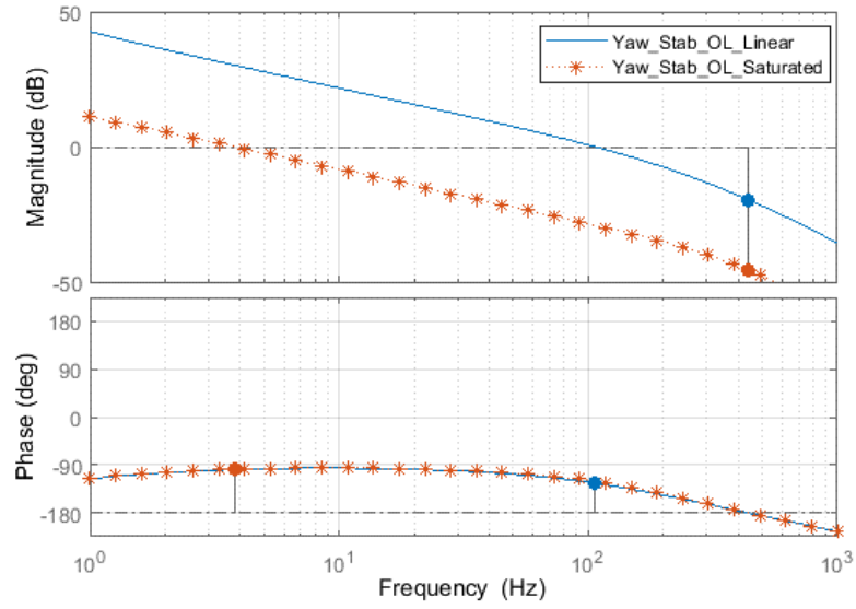
Figure 5-39: Motor selection simulation - Yaw rate open-loop bode plot
