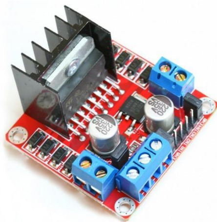
Figure 5-58: L298 Dual Full Bridge Driver [95]
