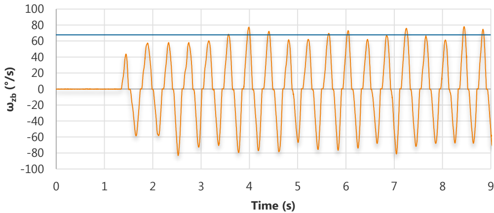
Figure 8-12: Base motion, \omega_{zb} , for the yaw channel BMI test in the home position
