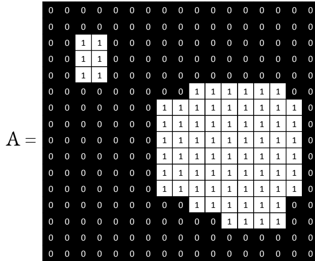
Figure 7-11: Binary image before erosion or dilation
