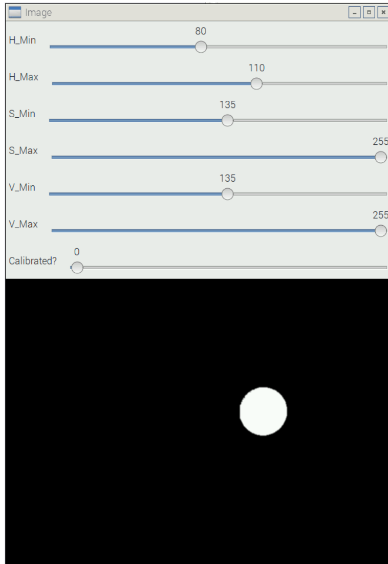
Figure 7-15: Calibration mode of the image processing script
