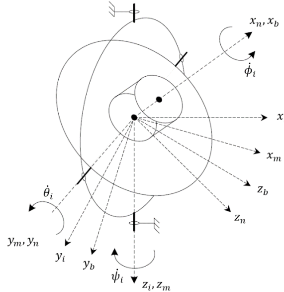
Figure 6-54: Host vehicle modelled as a three-axis gimbal (adapted from [104])
