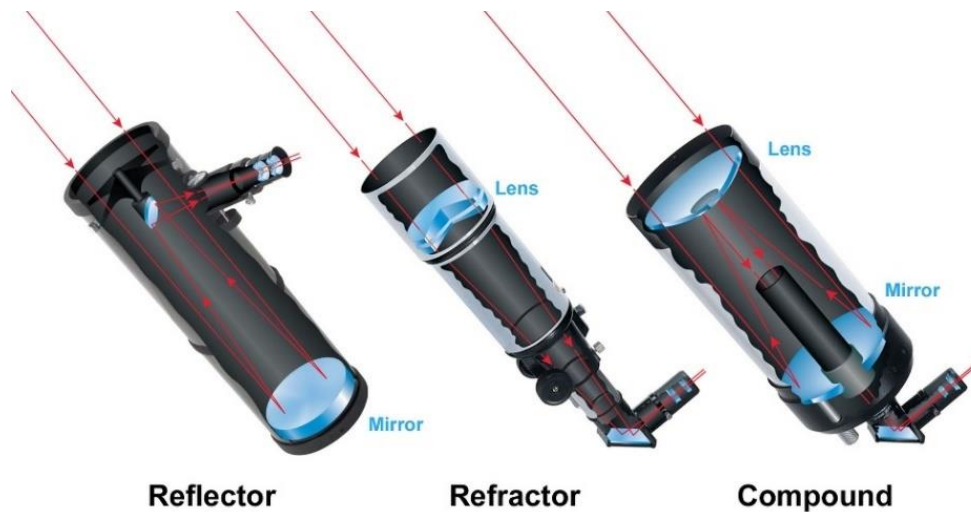
Figure 2-19: Optical telescope designs [46]
