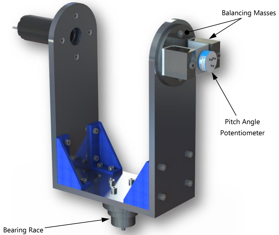
Figure 4-13: Yaw gimbal final design (front)
