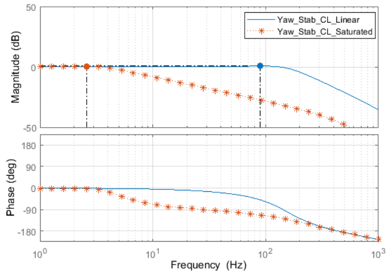
Figure 5-40: Motor selection simulation - Yaw rate closed-loop bode plot
