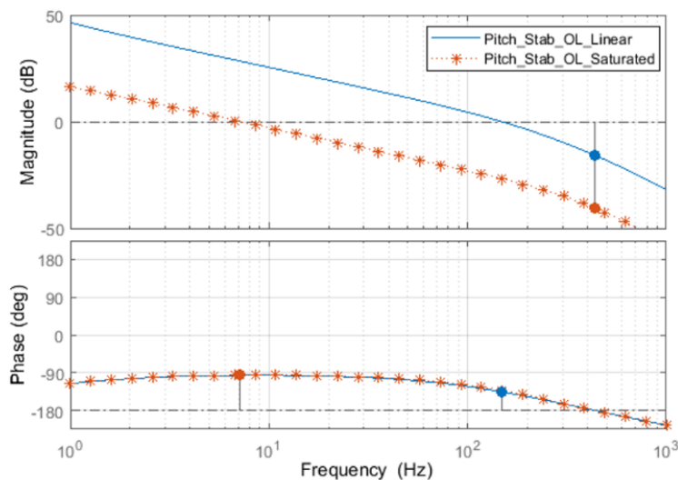
Figure 5-42: Motor selection simulation - Pitch rate open-loop bode plot
