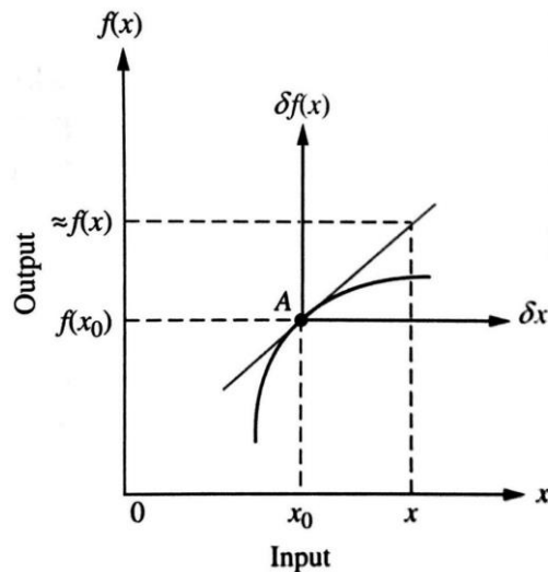
Figure 5-38: Linear approximation of a non-linear curve about point A [94]
