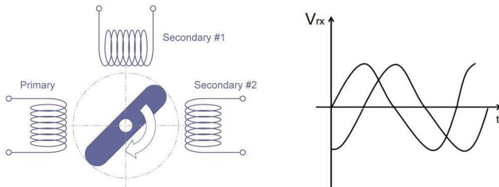
Figure 5-14: Workings of an Inductive Resolver [80]
