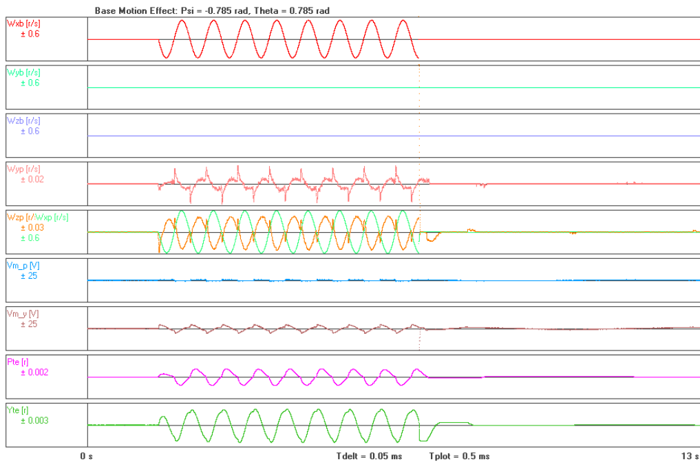
Figure 8-22: Base motion effects about the x_b axis in the worst-case orientation
