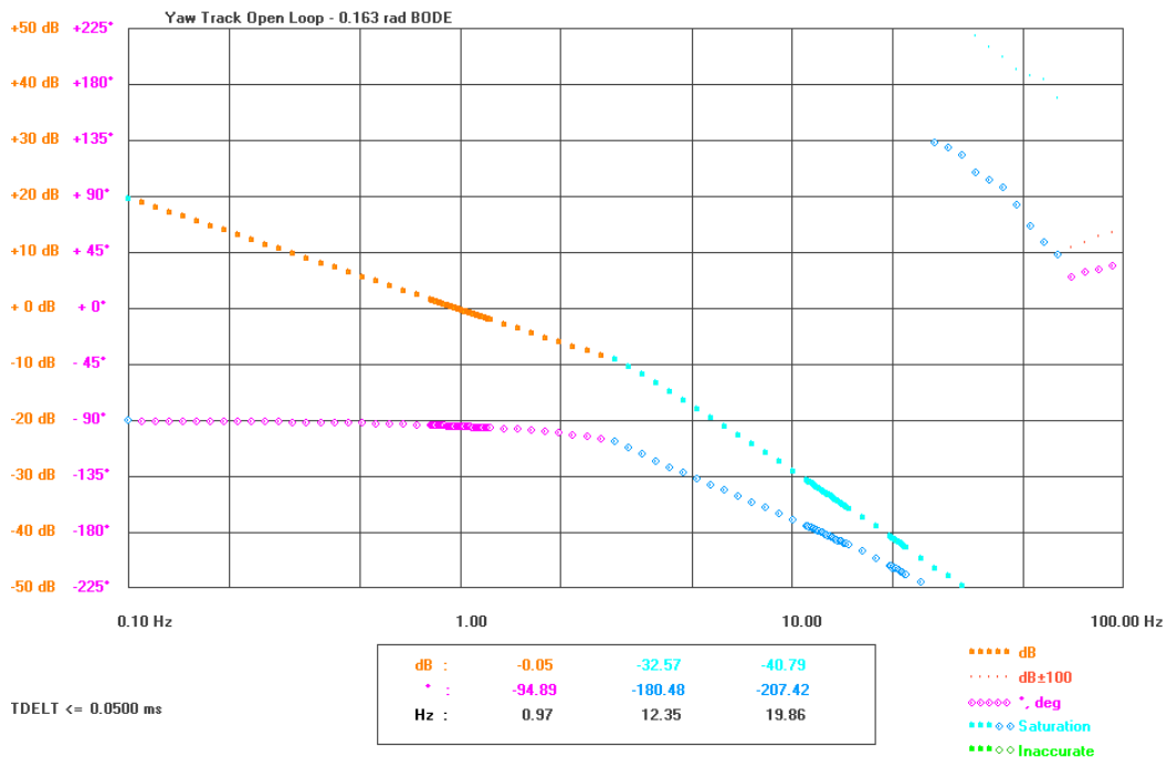
Figure 6-43: Yaw track open-loop Bode plot - Saturated Response
