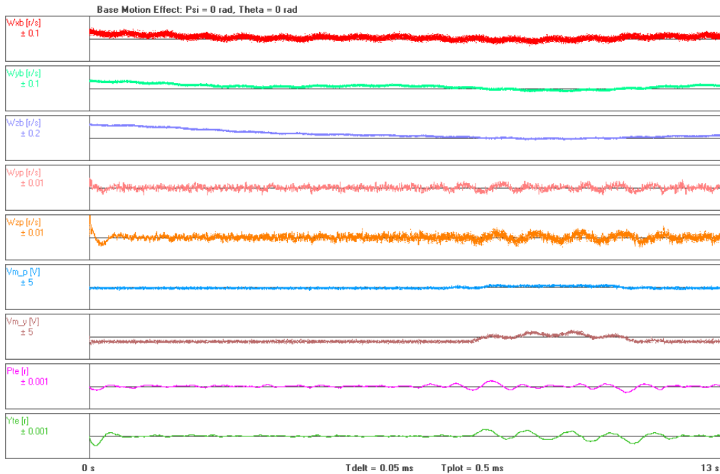
Figure 6-61: Base motion effect of the simulated base motion signal on the ISP in the home position
