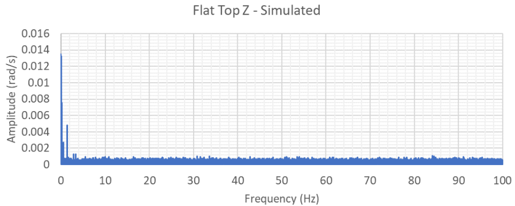
Figure 5-30: Frequency domain representation of the simulated signal z axis
