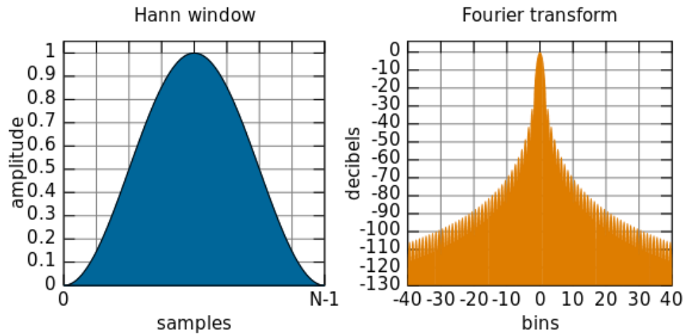
Figure 5-22: Hanning window function [91]
