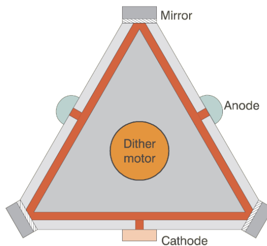
Figure 2-10: Ring Laser Gyro schematic [28]
