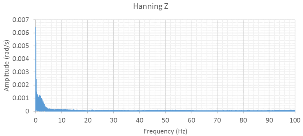
Figure 5-26: Amplitude vs Frequency of the z_{imu} data of Test 2 under the Hanning window
