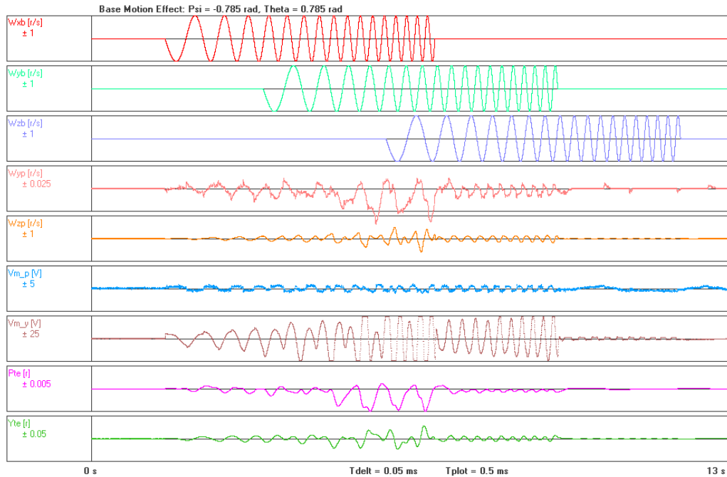
Figure 6-57: 1.0 rad/s base motion effect with the relative geometry model
