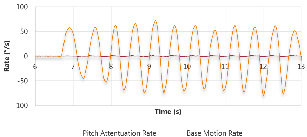
Figure 0-2: Typical disturbance attenuation of the pitch channel
