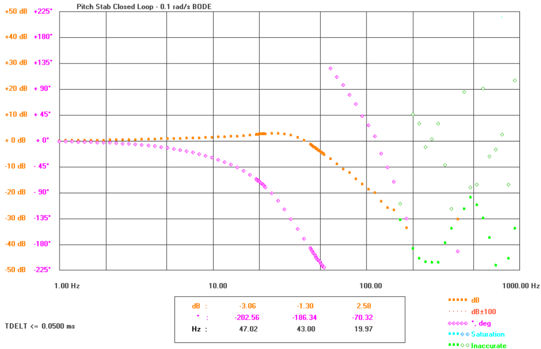
Figure 6-24: Pitch rate closed-loop Bode plot - Linear Response
