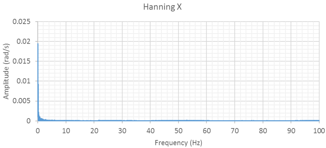
Figure 5-24: Amplitude vs Frequency of the x_{imu} data of Test 2 under the Hanning window
