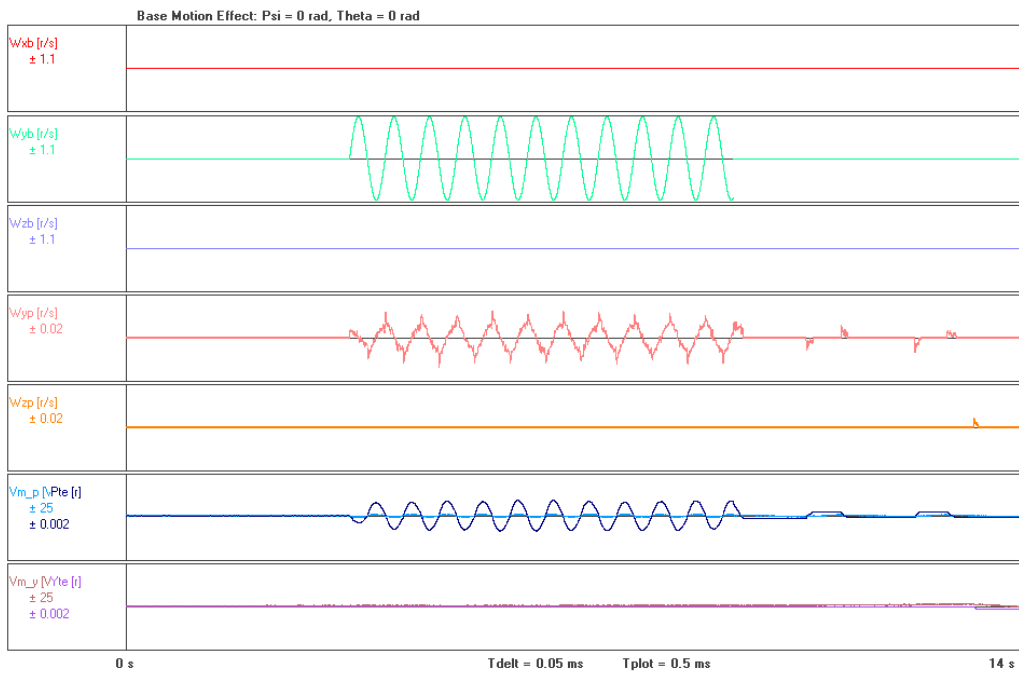
Figure 8-9: Simulation response to a 1.8 Hz, 60.89 ^{\circ}/s \omega_{yb} signal
