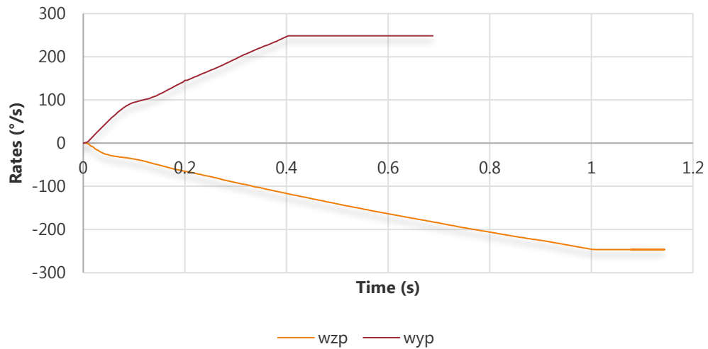
Figure 8-6: Maximum rates of the gimbals
