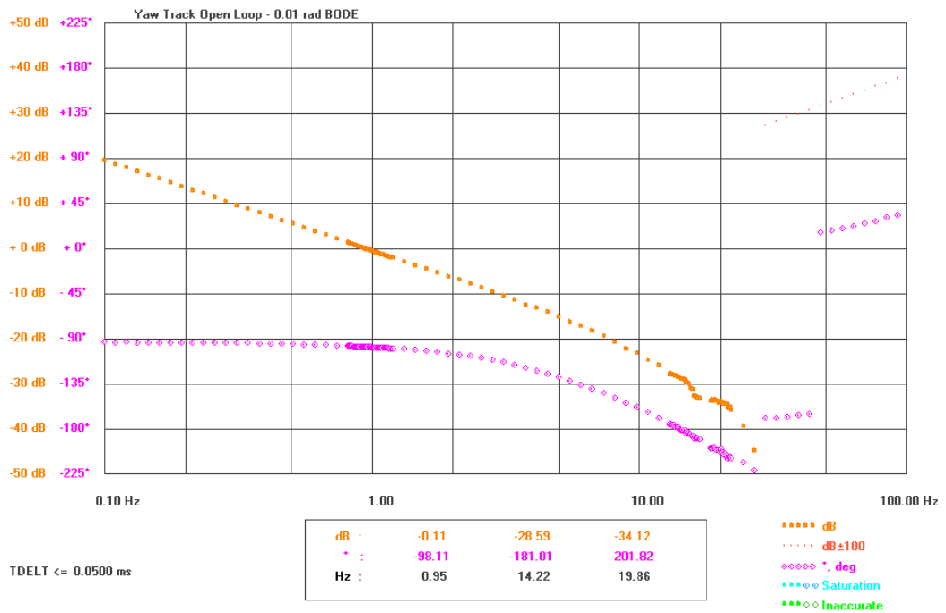
Figure 6-41: Yaw track open-loop Bode plot - Linear Response
