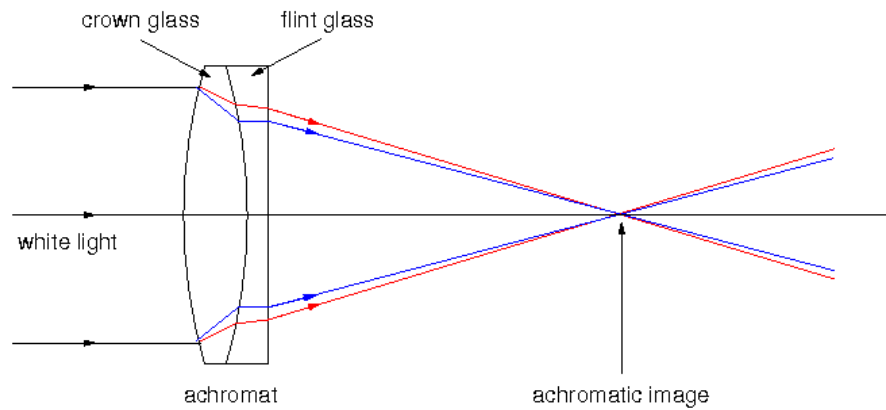
Figure 2-18: Achromatic lens [45]
