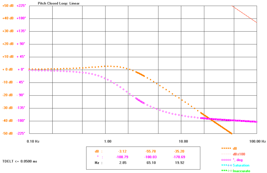
Figure 6-5: Linear closed-loop responses of the pitch manual position controller
