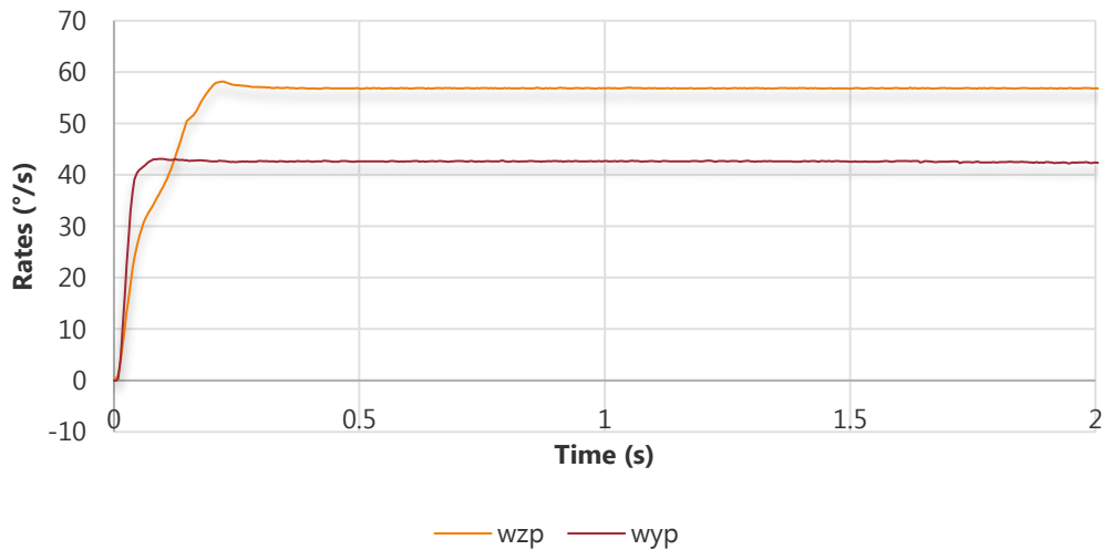
Figure 8-5: Yaw tracking rate test results
