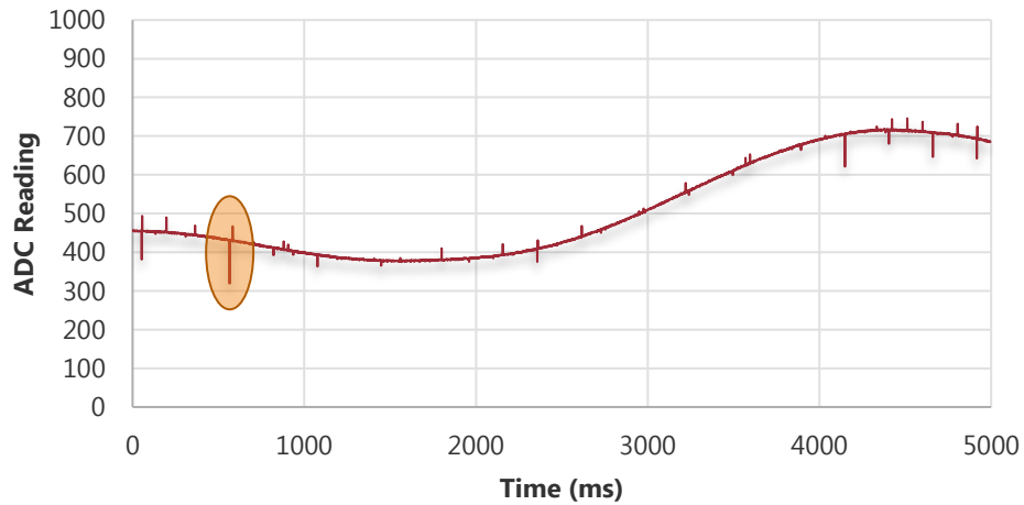
Figure 5-66: ADC readings with pot rails directly connected to VSSA and VDDA
