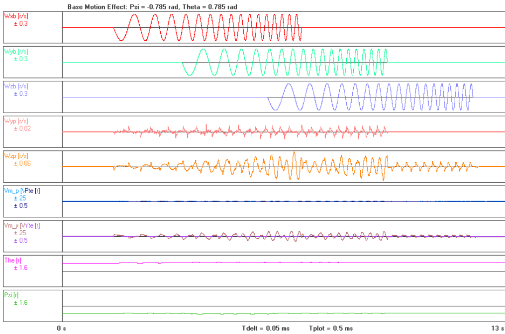
Figure 6-51: 0.25 rad/s base motion effect in the worst-case position
