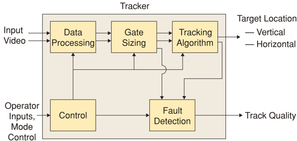
Figure 2-14: Target tracker operation
