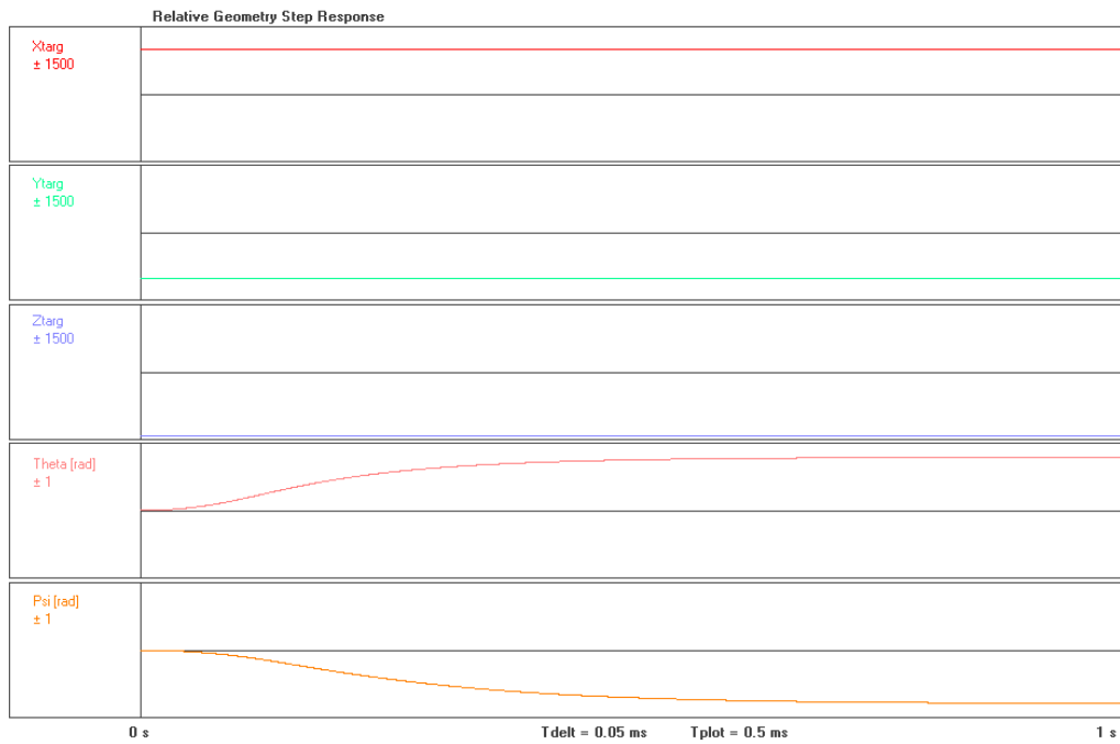
Figure 6-56: Tracking step response using a target and relative geometry
