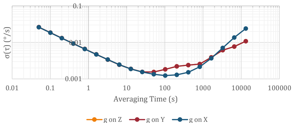
Figure 5-7: X-Axis Allan Deviation
