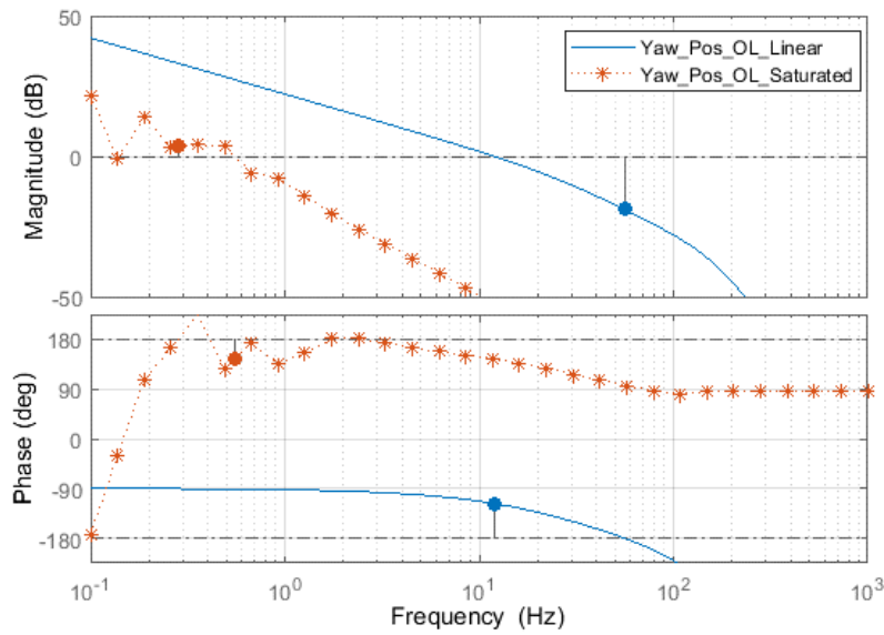
Figure 5-45: Motor selection simulation - Yaw position open-loop bode plot
