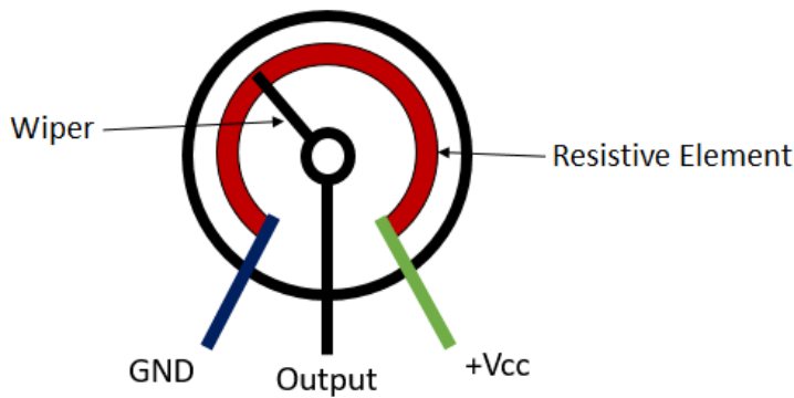
Figure 5-15: Workings of a potentiometer [81]
