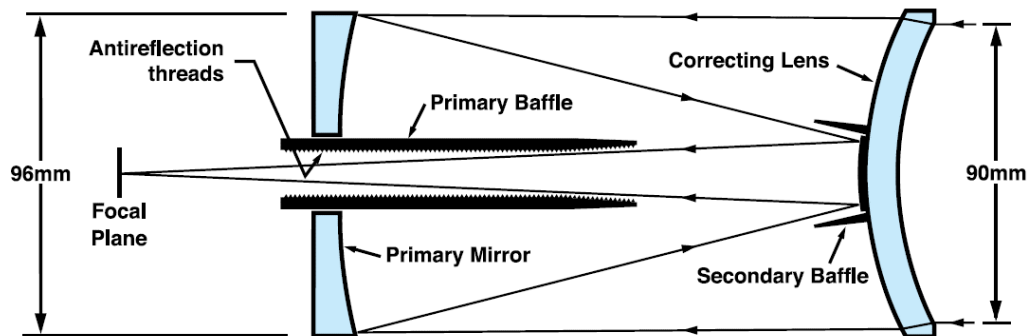
Figure 4-2: Lightpath through the Meade ETX90 [59]
