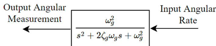
Figure 6-15: Initial gyro model used in the ISP simulation
