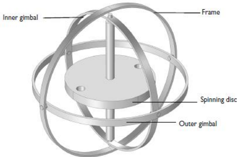
Figure 2-9: Mechanical gyroscope [26]
