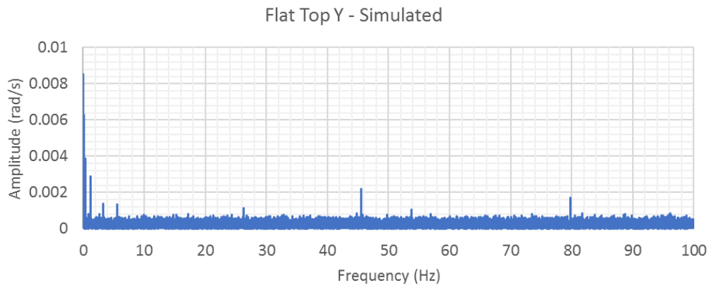
Figure 5-29: Frequency domain representation of the simulated signal y axis
