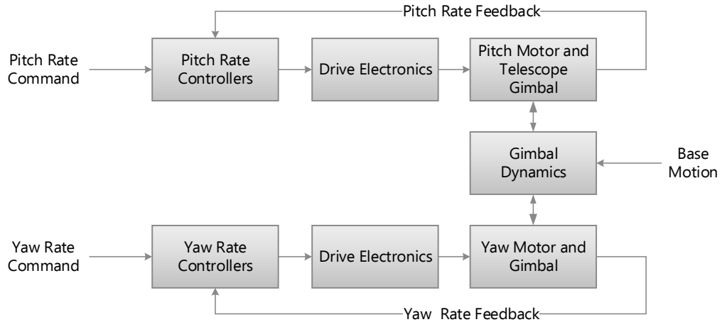
Figure 6-13: ISP stabilisation system identification diagram
