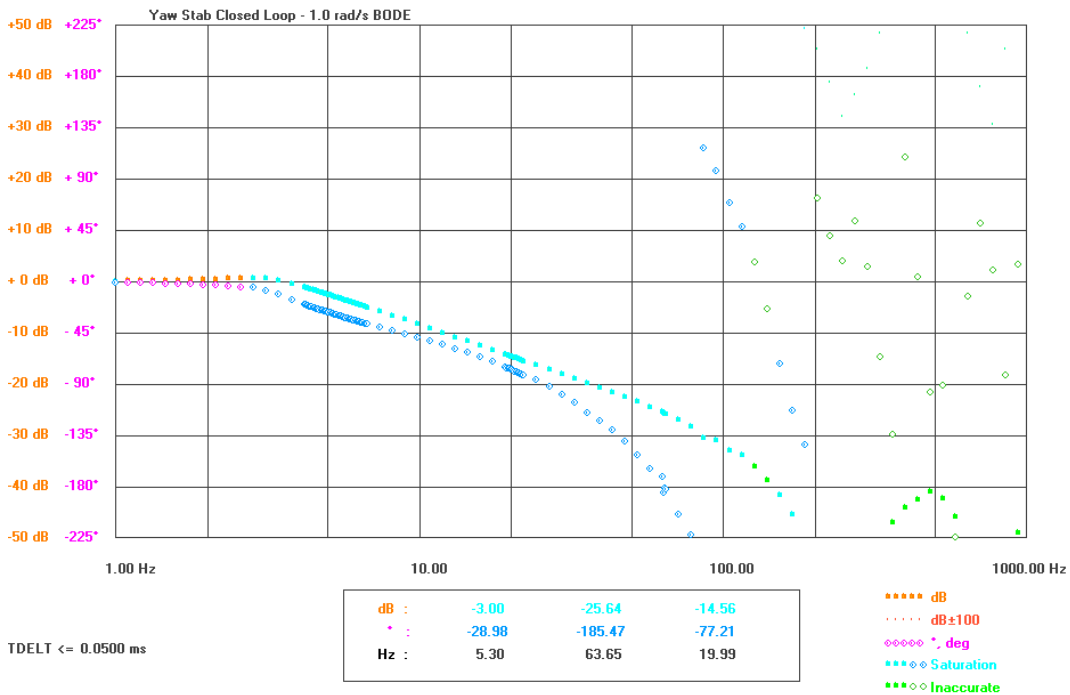
Figure 6-22: Yaw rate closed-loop Bode plot - Saturated Response
