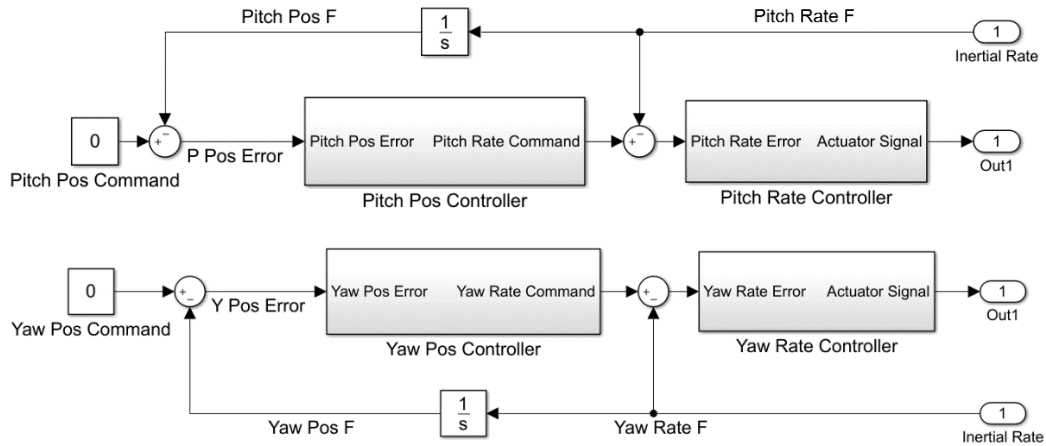
Figure 5-35: Controller structure for the Yaw and Pitch channels
