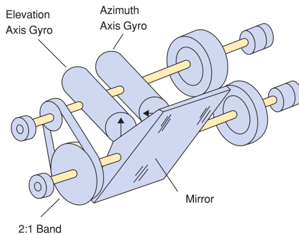
Figure 2-6: 2:1 drive linkage [7]
