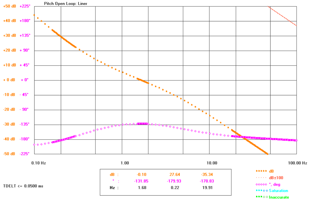
Figure 6-3: Linear open-loop responses of the pitch manual position controller
