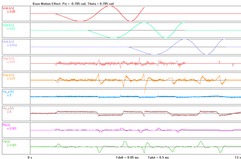
Figure 6-59: Base motion effect of peak simulation signal in the worst-case position with relative geometry
