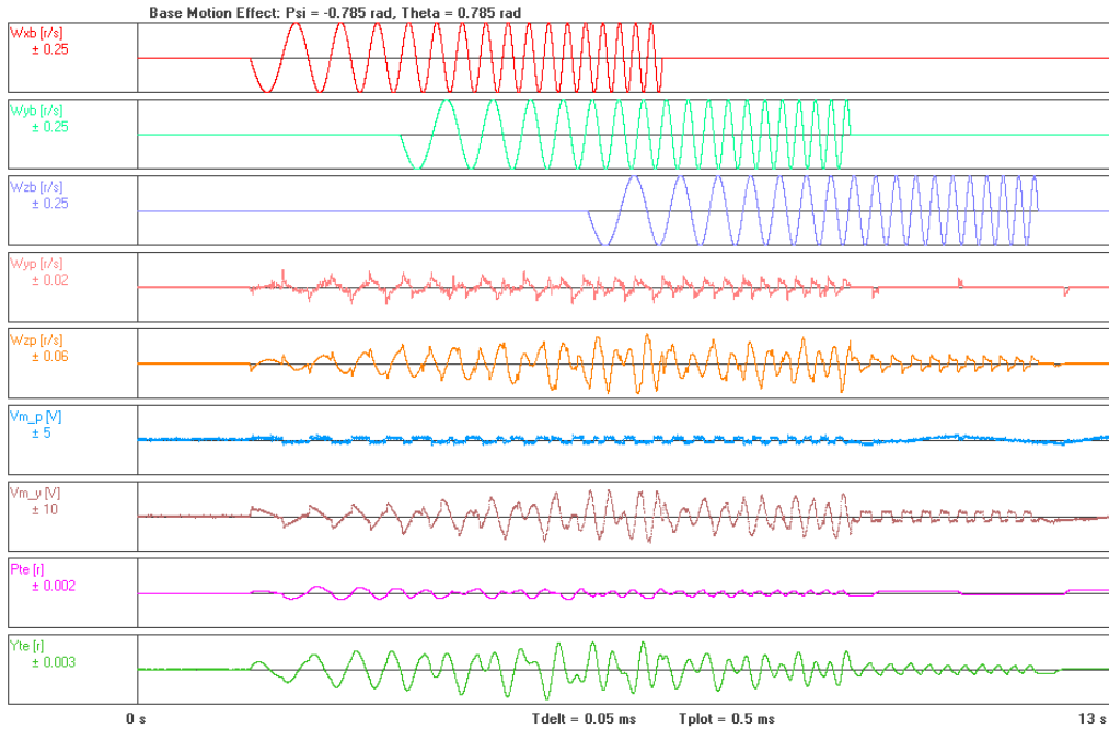
Figure 6-58: 0.25 rad/s base motion effect with the relative geometry model
