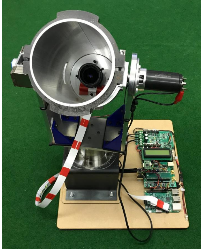
Figure 4-23: Final implementation of the ISP system
