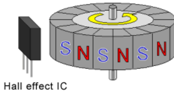
Figure 5-13: Hall-effect rotary sensor [79]
