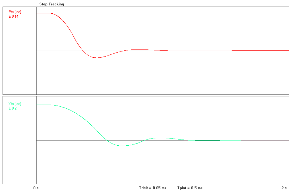
Figure 8-4: Step tracking with current limited motors
