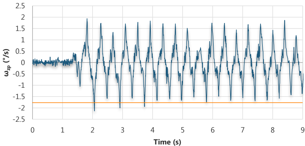
Figure 8-13: Inertial rate, \omega_{zp} , for the yaw channel BMI test
