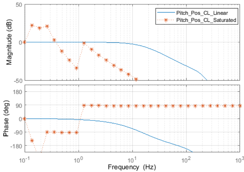
Figure 5-49: Motor selection simulation - Pitch position closed-loop bode plot
