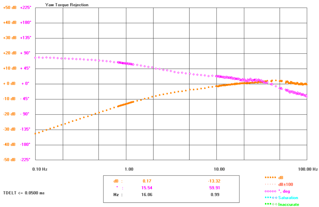
Figure 6-36: Yaw torque rejection– Yaw rate command to rate error (0.014 rad/s)
