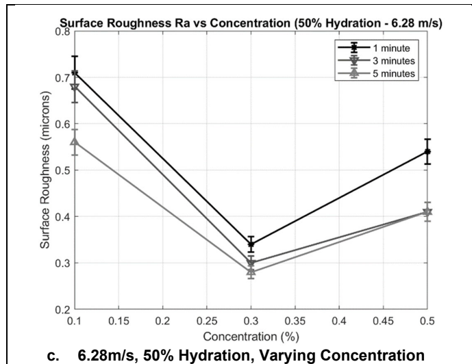
Figure 83 - 6.28 m/s Ra Changes (varying concentration)
