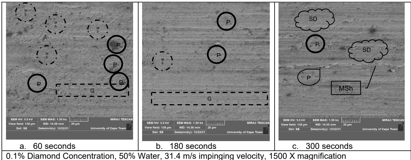
Figure 88 - 0.1%D, 50%H, 31.4 m/s, 1500 X SEM Images
