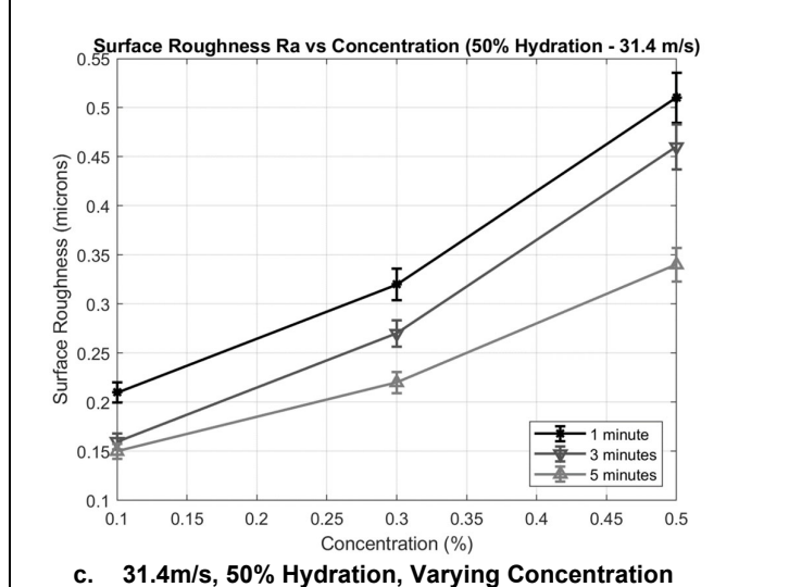
Figure 85 - 31.4 m/s Ra changes (varying concentration)
