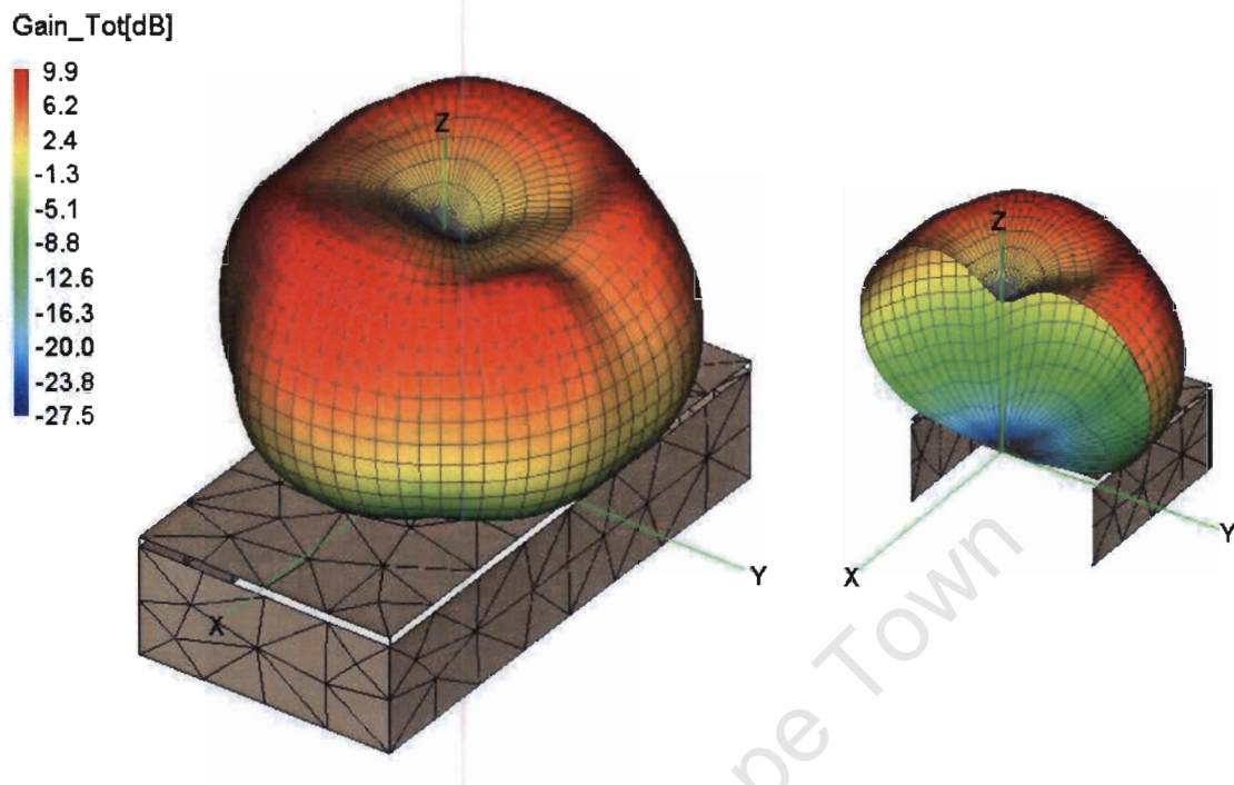
Figure 4.18: 3D radiation gain pattern indication the directivity of the cased fat dipole
