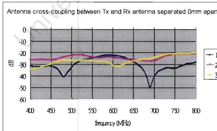
Figure 5.6: Cross-coupling of antennas at 0mm separation
