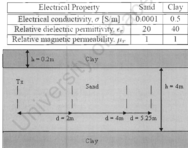
Figure 1.1: Subsurface media simulation configuration
