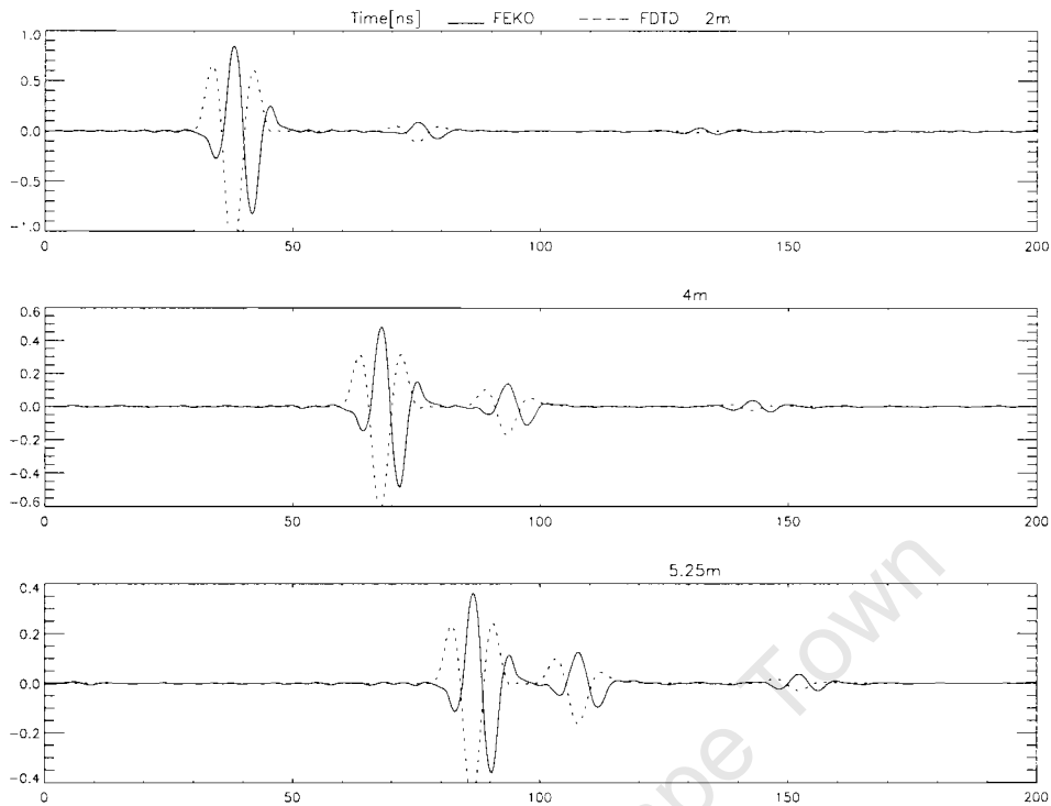
Figure 3.6: Over-plot of FEKO and FDTD receiver waveforms.
