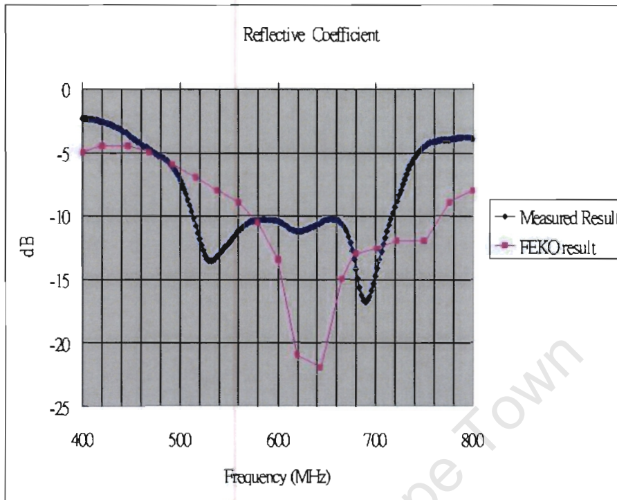
Figure 5.4: Validating the fabricated antenna S11 with the simulated result
