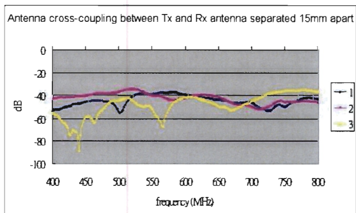
Figure 5.9: Cross-coupling of antenna at 15mm separation
