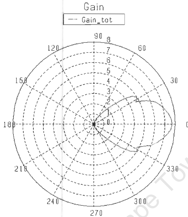
Figure 4.11: Fat dipole radiation pattern at 600MHz
