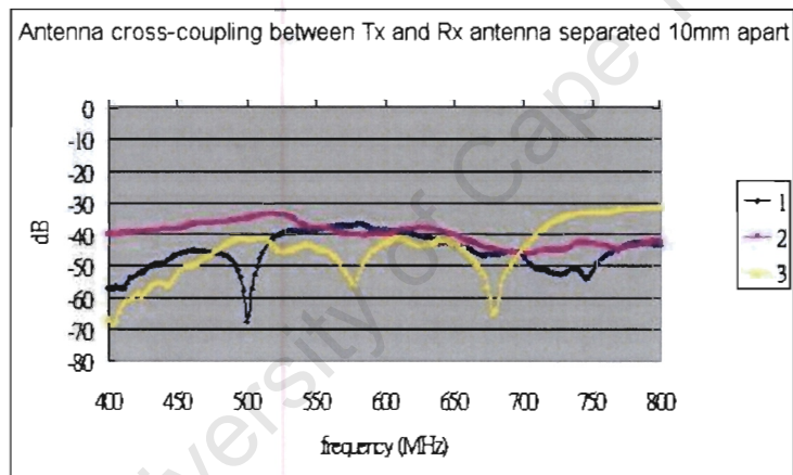
Figure 5.8: Cross-coupling of antennas at 10mm separation
