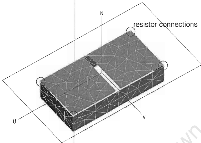
Figure 4.16: Edge termination resistor connections
