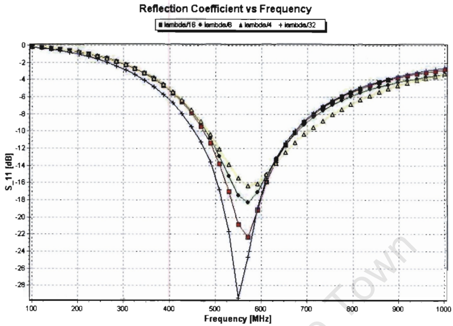
Figure 4.8: S11 of various fat dipole substrate heights
