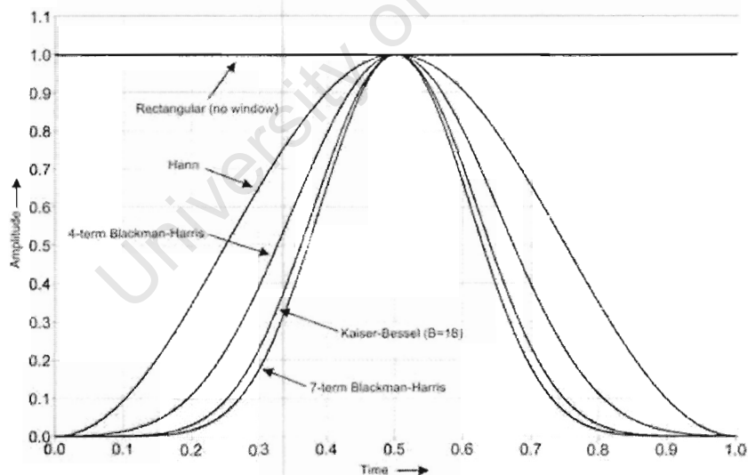
Figure 2.1: Common window functions[4]
