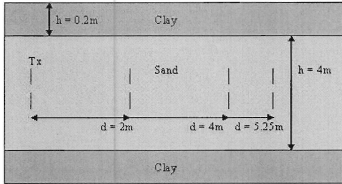
Figure 3.1: Dimensions of the layered media under investigation.
