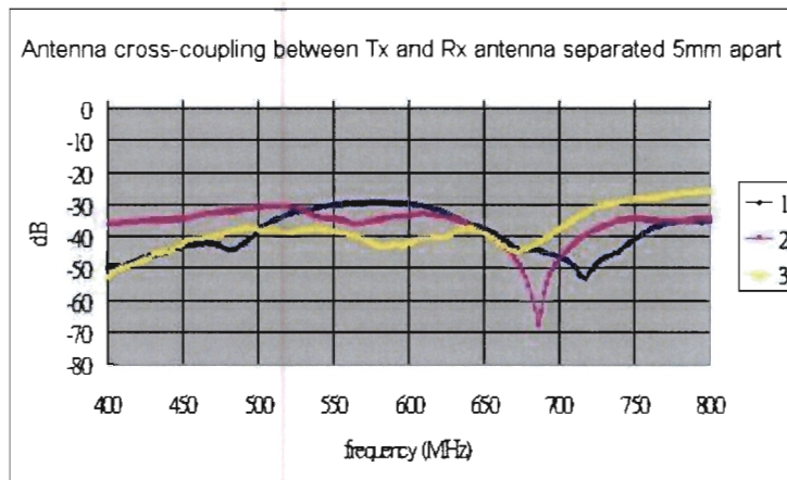
Figure 5.7: Cross-coupling of antennas at 5mm separation
