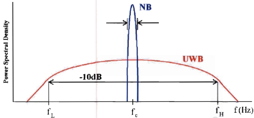
Figure 2.2: UWB definition[2]
