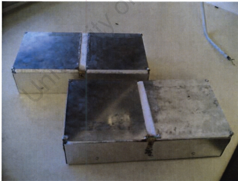
Figure 5.3: Photograph of the antennas and S11 sand box testing arrangement with Agilent E5062A network analyser
