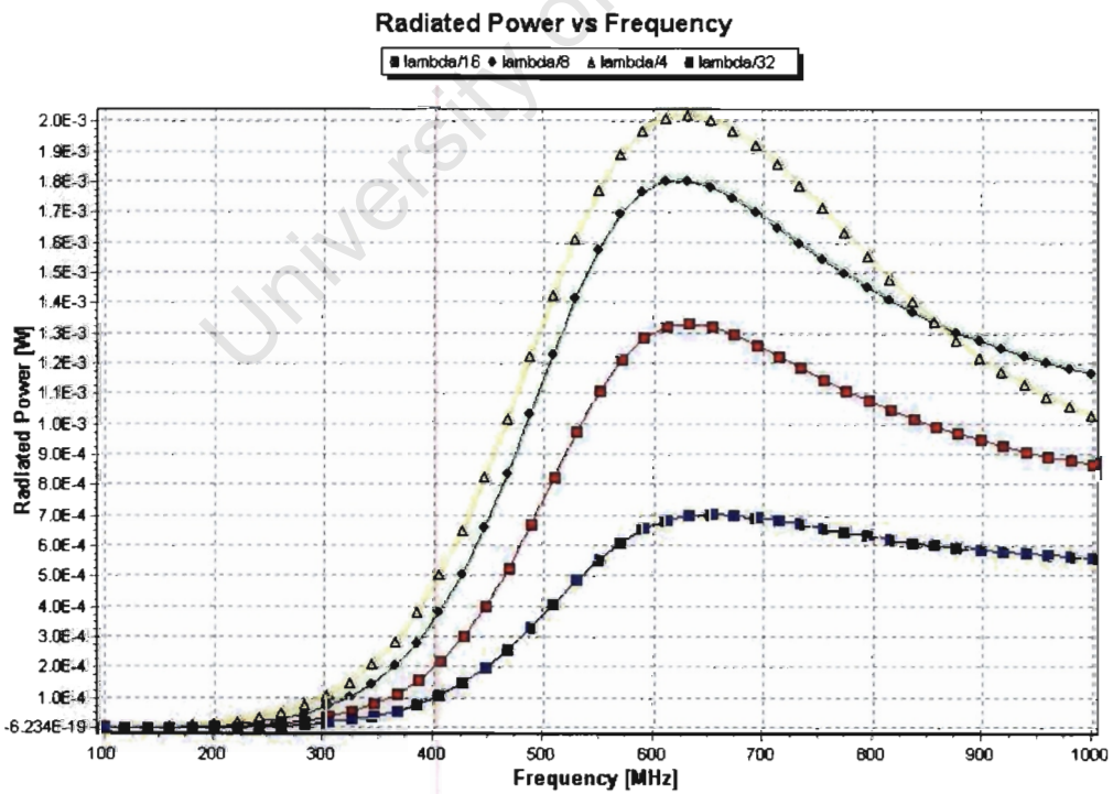
Figure 4.9: Power radiated
