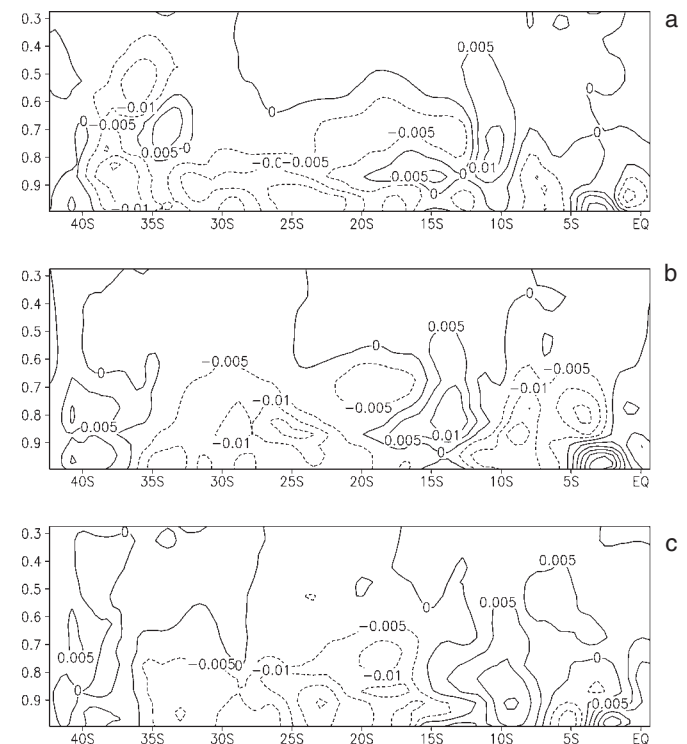
Fig. 5. Moisture flux differences through a transect along 40°E between the idealized and observed SST anomaly experiments: a, January; b, February; c, March 1981. Contour interval is 0.005 \text{ g kg}^{-1} \text{ m s}^{-1} and negative values represent westward transport towards southern Africa.
