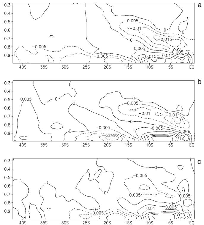
Fig. 4. Moisture flux differences through a transect along 10°E between the idealized and observed SST anomaly experiments: a, January; b, February; c, March 1981. Contour interval is 0.005 \text{ g kg}^{-1} \text{ m s}^{-1} and positive values represent eastward transport towards southern Africa.
