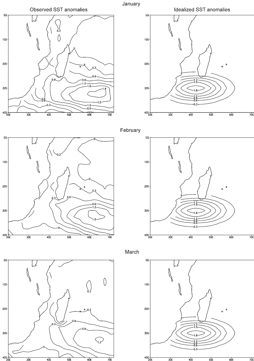
Fig. 1. The observed (left column) and idealized (right column) (contour interval 0.3^{\circ}\text{C} in each case) SST anomaly pattern for January–March 1981 used to force the MM5 model.
