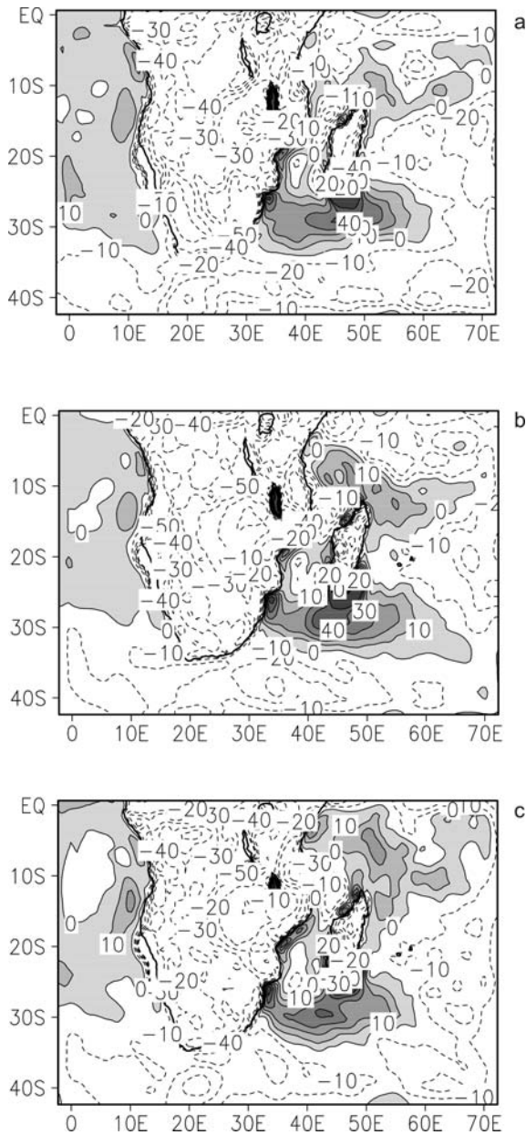
Fig. 8. Surface latent heat flux differences between the idealized and observed SST anomaly experiments: a , January; b , February; c , March 1981. Contour interval is 10 \text{ W m}^{-2} and shading represents positive differences or increased evaporation.
