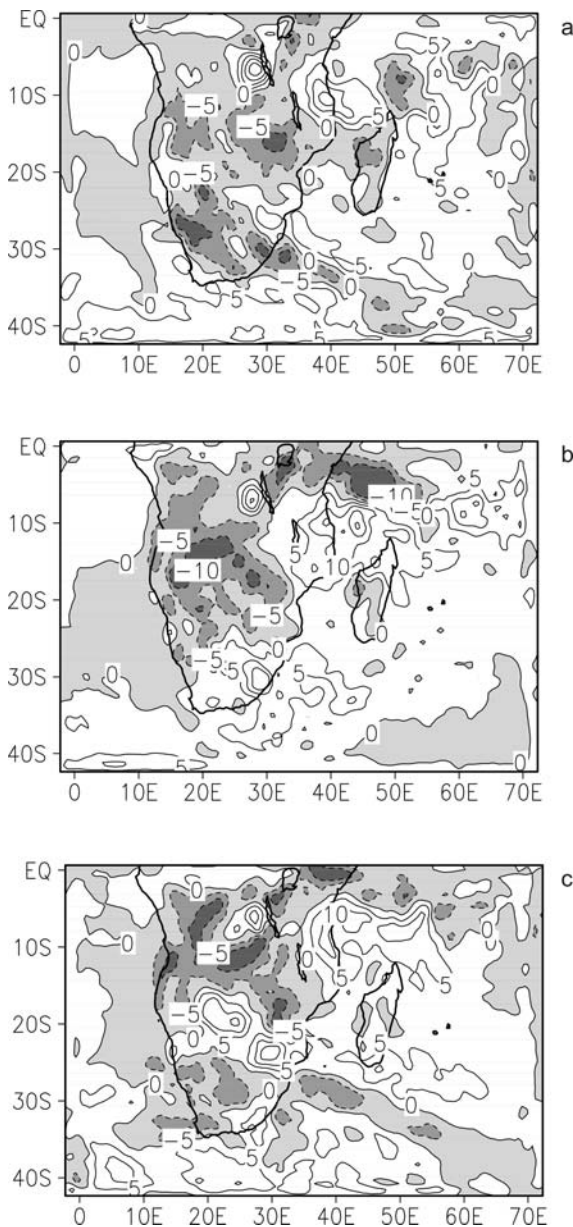
Fig. 10. Outgoing long-wave radiation differences between the idealized and observed SST anomaly experiments: a , January; b , February; c , March 1981. Contour interval is 5 W m -2 and shading represents negative differences or increased convective cloud.
