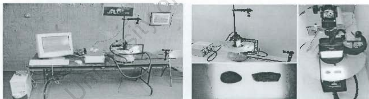
Figure 2.4: The WipFrag system. (Picture from Al Rousan [111])
