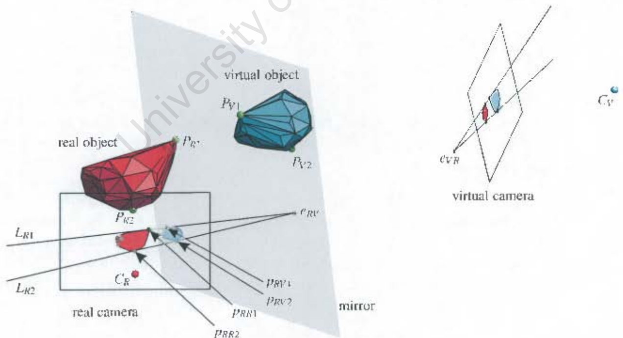
Figure 4.3: A camera viewing an object and its reflection. The epipole corresponding to the virtual camera can be computed from the silhouette bitangents L_{R1} and L_{R2} .
