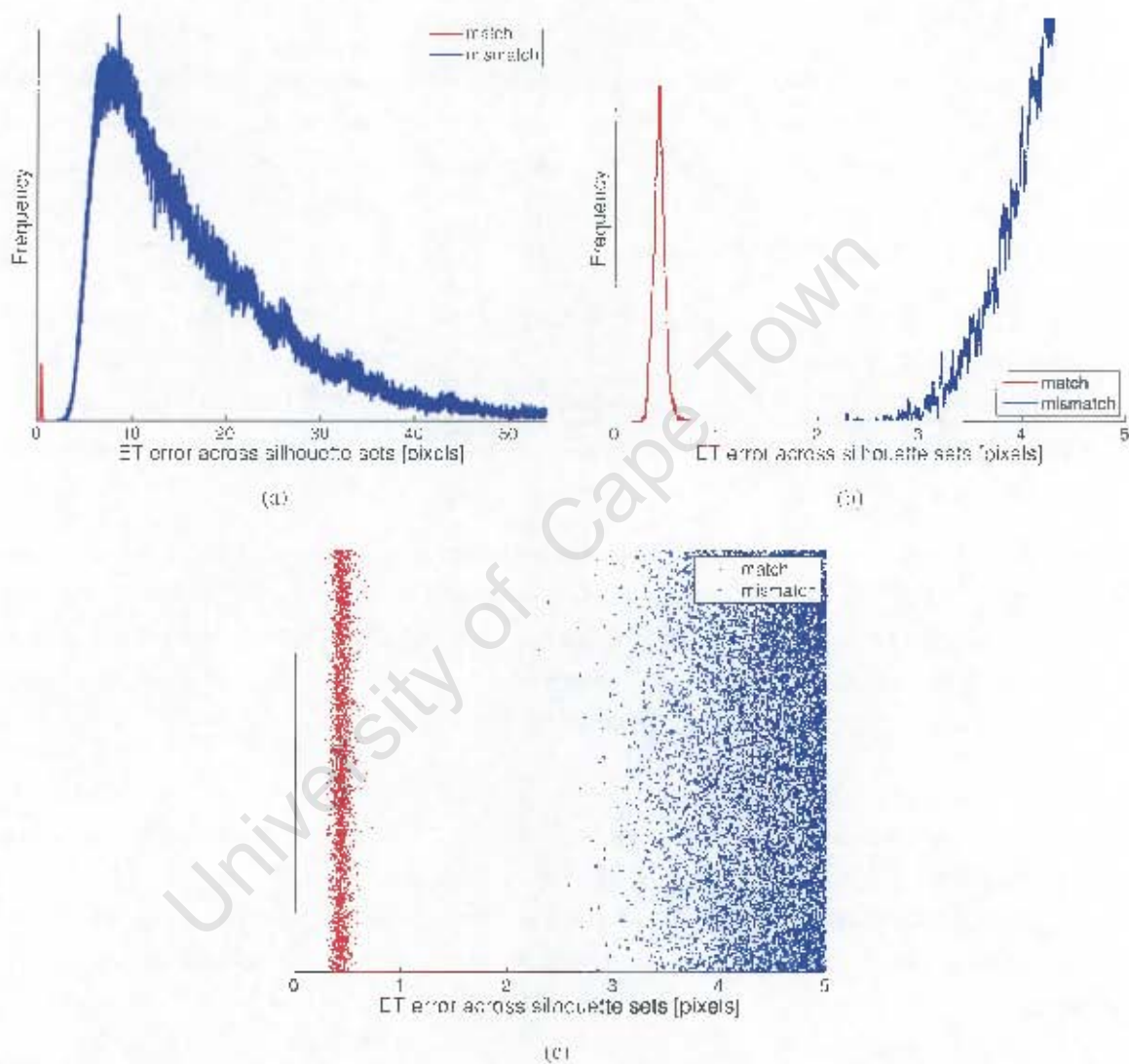
Figure 7.6: ET errors across silhouette set pairs after pose optimisation for 2460 match pairs and 602 700 mismatch pairs formed from the six-view garnet data set: (a) shows match and mismatch distributions estimated with a kernel smoothing method (a low variance Gaussian was used to limit over-smoothing); (b) shows a closeup of (a) in the region where the distributions are closest; (c) shows the data points in the region illustrated by (b) (the vertical component, which is random, is a visualisation aid).
