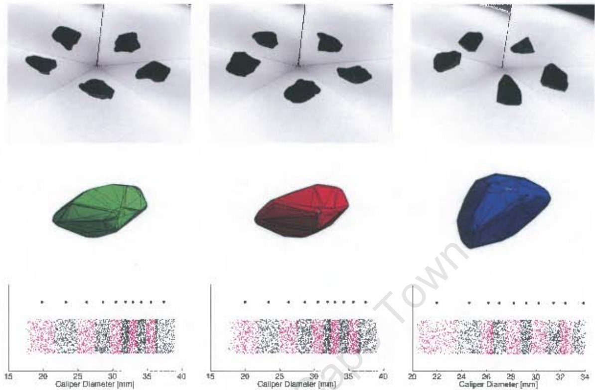
Figure 8.2: Three examples of input silhouette sets ( first row ), corresponding VEMHs ( second row ), and caliper diameter sample values and signature values ( third row ). The vertical component in the caliper diameter value plots is random (a visualisation aid). Larger dots represent signature values computed as the mean of corresponding deciles of caliper diameter values (10 signature elements are used). Decile colouring alternates to show correspondences with signature values. The silhouette set in the first column matches the silhouette set in the second column, but not the silhouette set in the third column. ET-based pose optimisation has been applied to align all VEMHs with the reference frame of the first column.
