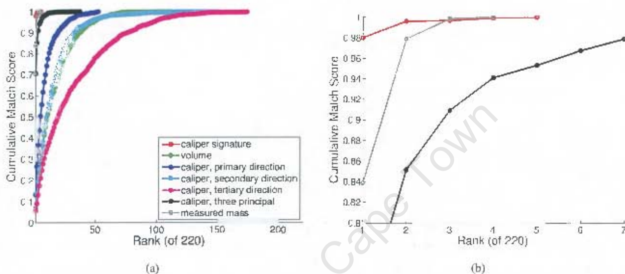
Figure 8.11: (a) Rank versus cumulative match score plot derived using various measures of dissimilarity; (b) a closeup of part of the plot shown in (a).
