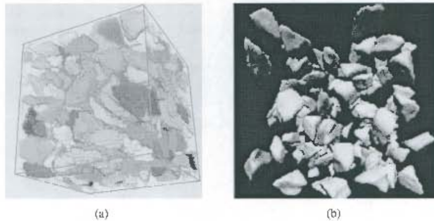
Figure 2.2: Computer simulations of concrete using 3D shapes based on real particles: (a) modelling concrete flow (picture from Bullard et al. [20]), (b) simulation of coarse aggregate in a mortar matrix flowing under mixing forces (picture from Giaboczi et al. [52]).
