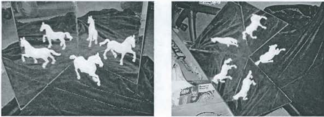
Figure 4.2: Two images of a two-mirror setup positioned so that five views of the object can be seen. Note that the camera has moved between shots, but the mirrors and object have not moved.
