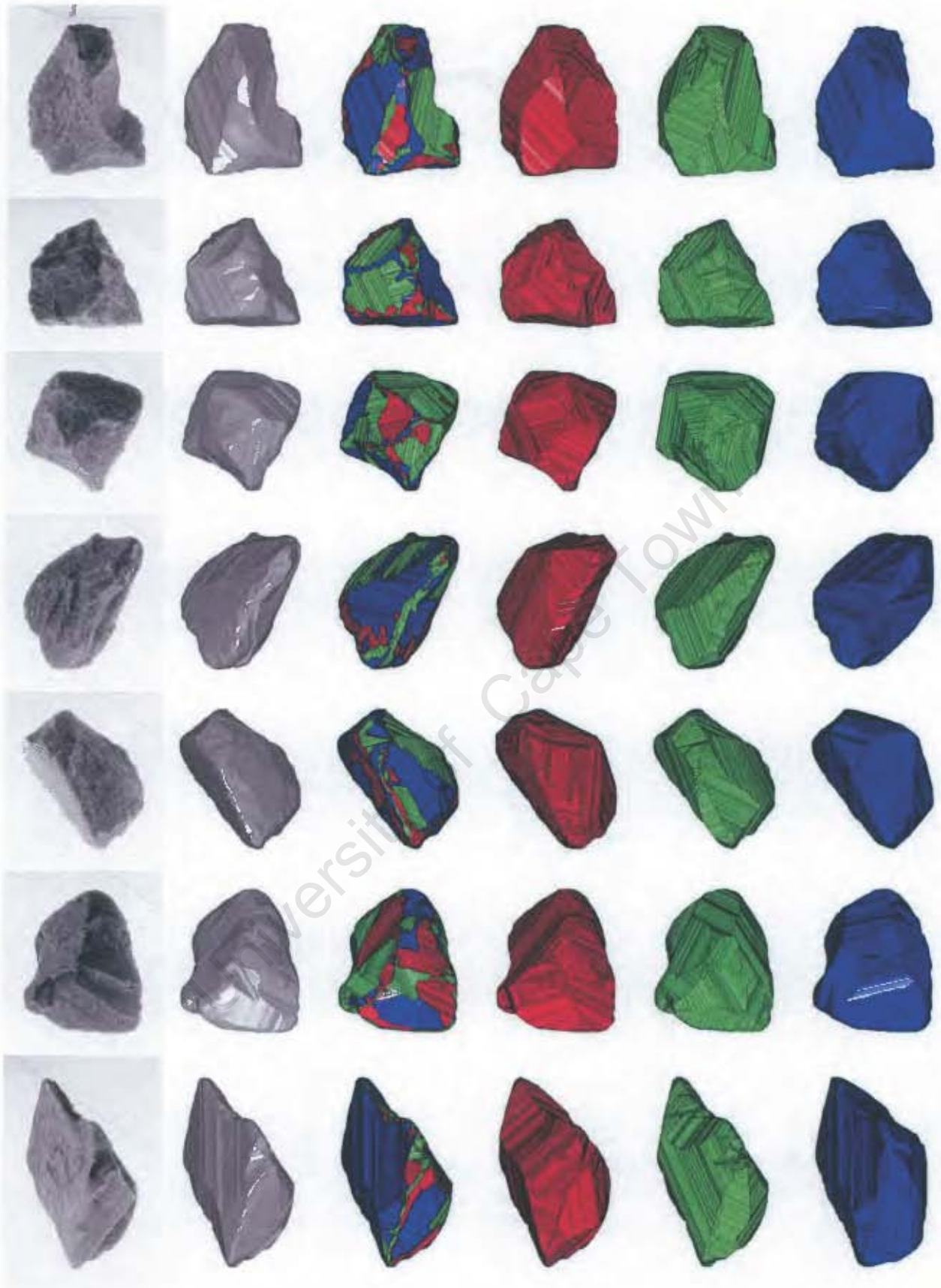
Figure 6.15: Some examples of visual hulls of pieces of gravel. The first column shows original images of the gravel. The second column shows the 15-view visual hull (formed from three 5-view silhouette sets) from the same viewpoint as the first column. The third column shows the 15-view visual hull surfaces coloured according to which of the three original 5-view visual hulls contributes to the surface region. The three original visual hull models are shown to the right in corresponding colours.
