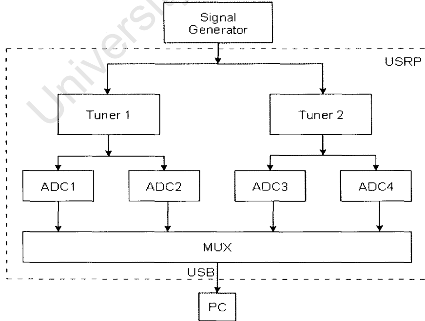
Figure 6.4: Block diagram of experimental setup
