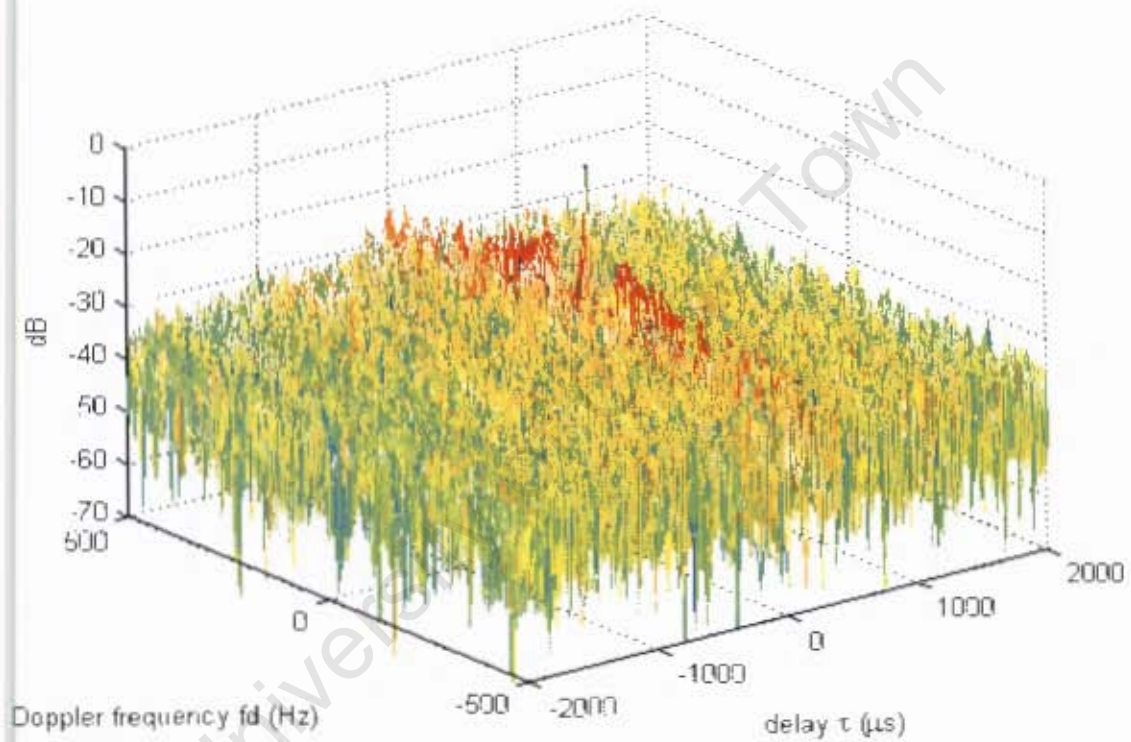
Figure A.3: Ambiguity plot of Umlhlobo-FM transmission
