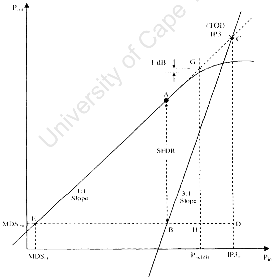
Figure 4.11: Spurious Free Dynamic Range [3]
