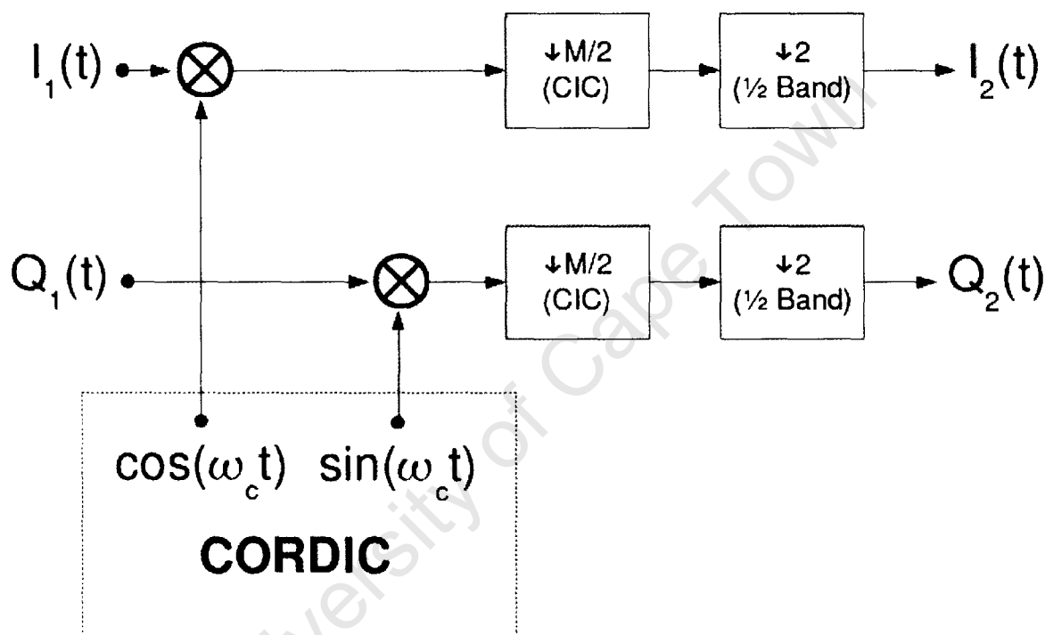
Figure 3.5: DDC block Diagram [39]
