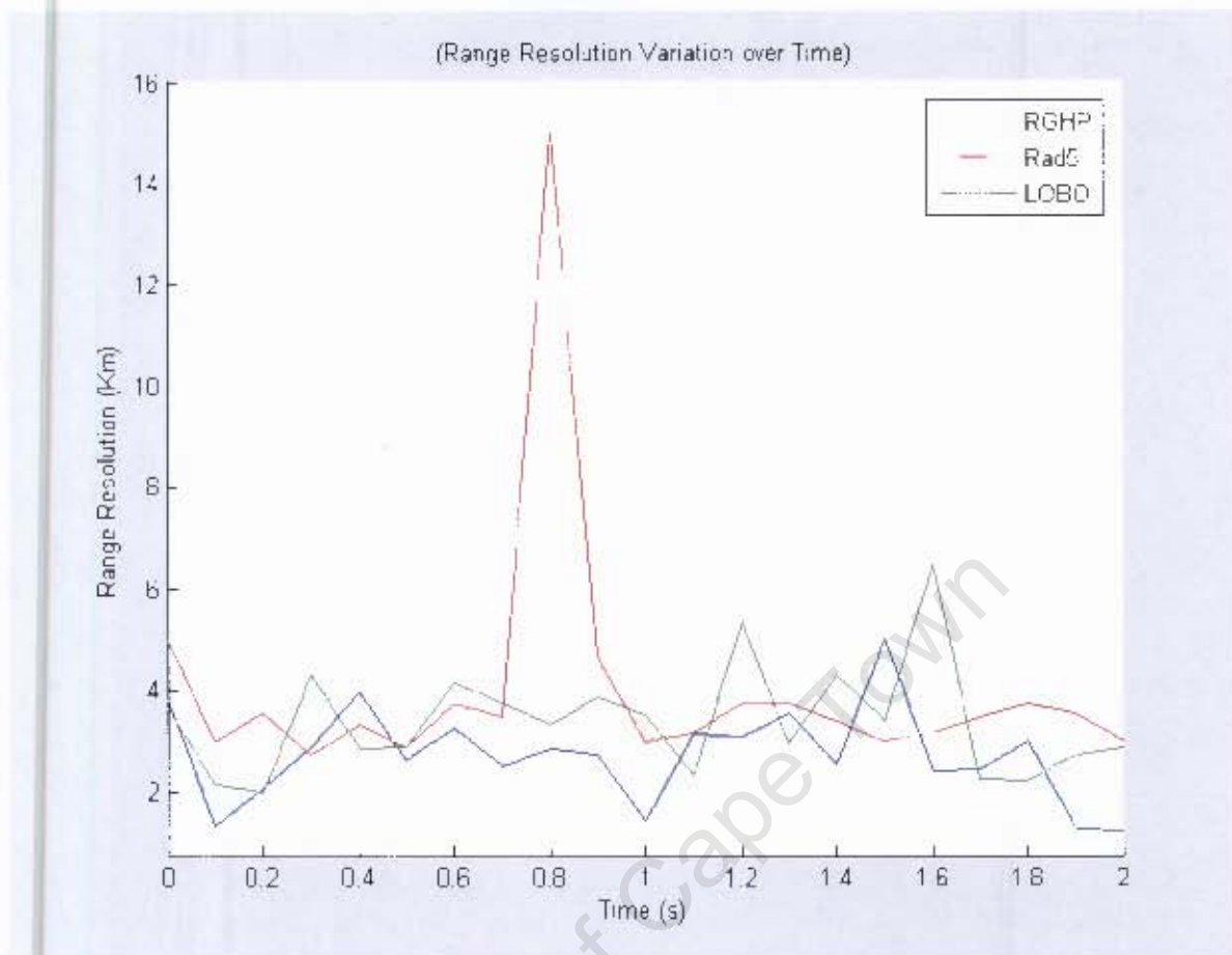
Figure 5.5b: Variation of signal range resolution with time
