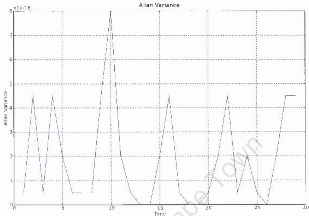
Figure 6.7: Allan Variance of the fractional frequencies
