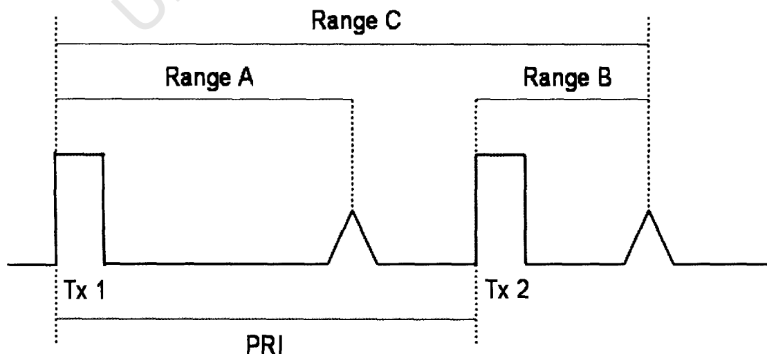
Figure 2.3: A target echo detected after the transmission of the second pulse results in ambiguous ranges at B and C.
