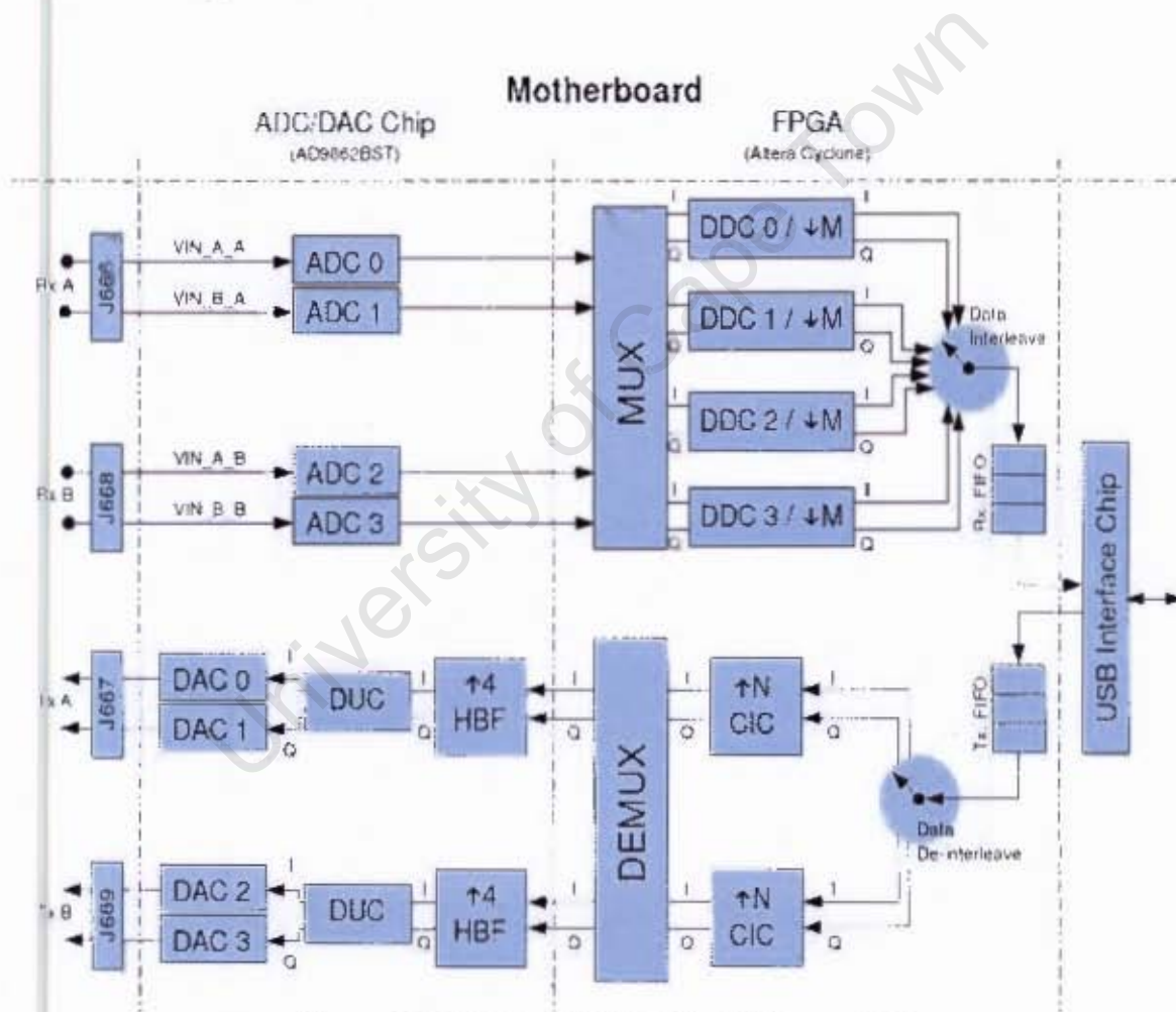
Figure 3.4: USRP and FPGA block Diagram [39]
