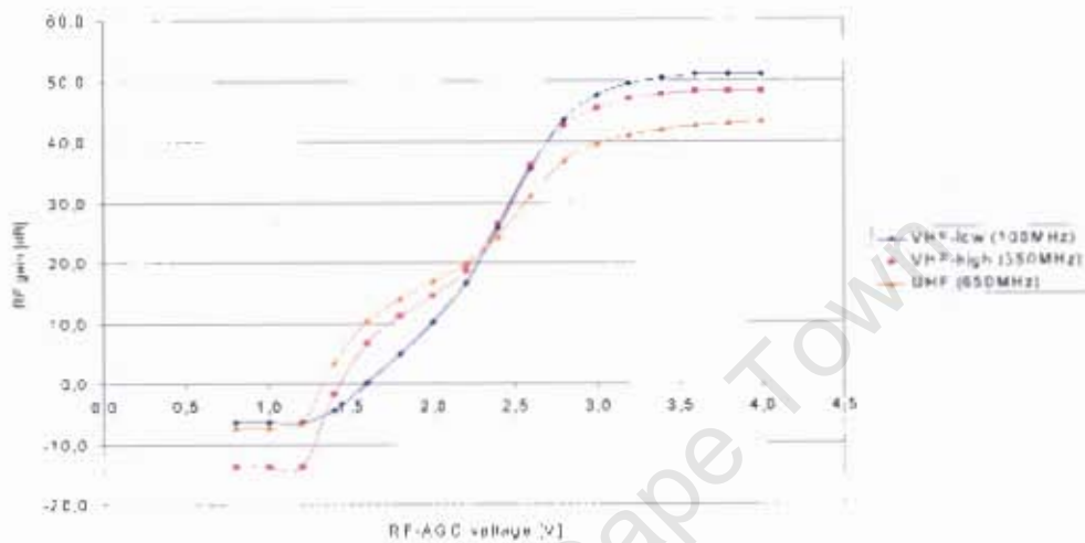
Figure 3 RF Gain vs. AGC Voltage
