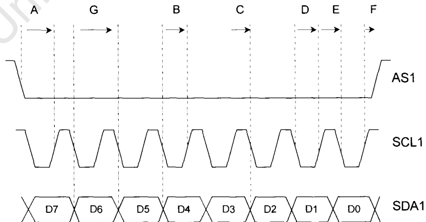
Figure 7 Serial Interface Timing
