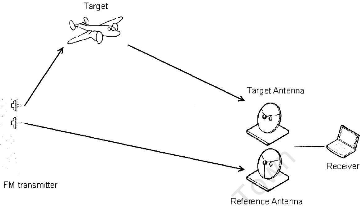
Figure 1.1: PCL block diagram
