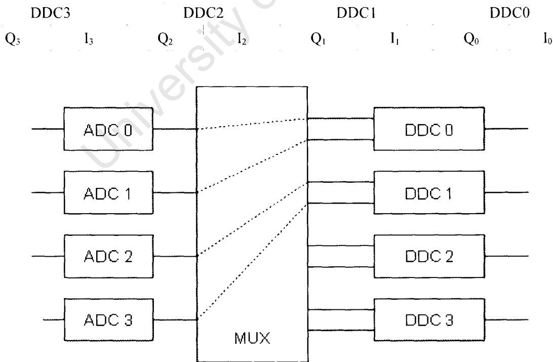
Figure 4.5: Multiplexer setup for two TVRx to DDC0 and DDC1
