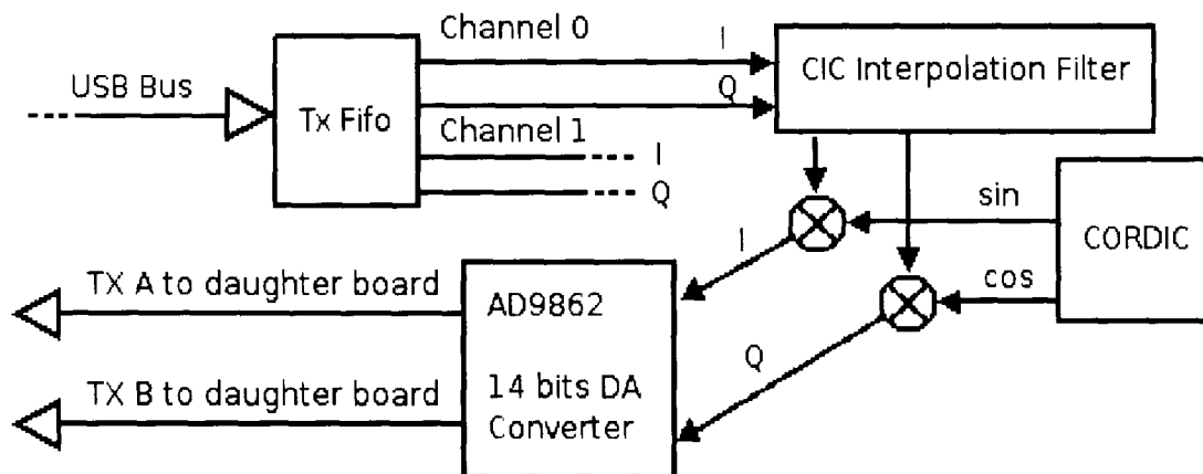
Figure 3.6: USRP transmit chain block Diagram [39]
