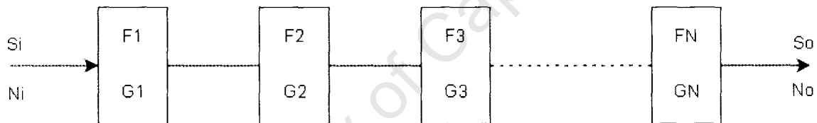
Figure 4.8: Cascaded components
