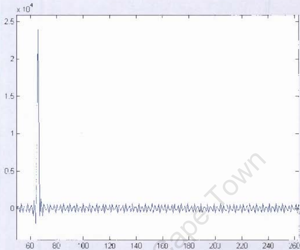
Figure 4.7: Closer look at the spurious signal generated by USRP on startup
