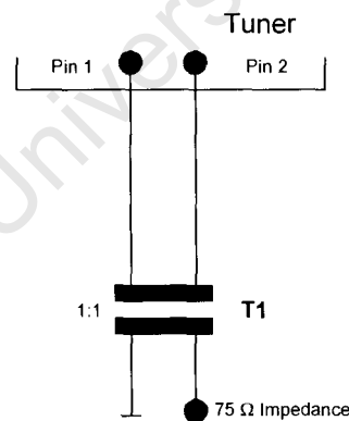
Figure 6 Test Circuit for Upstream Channel
