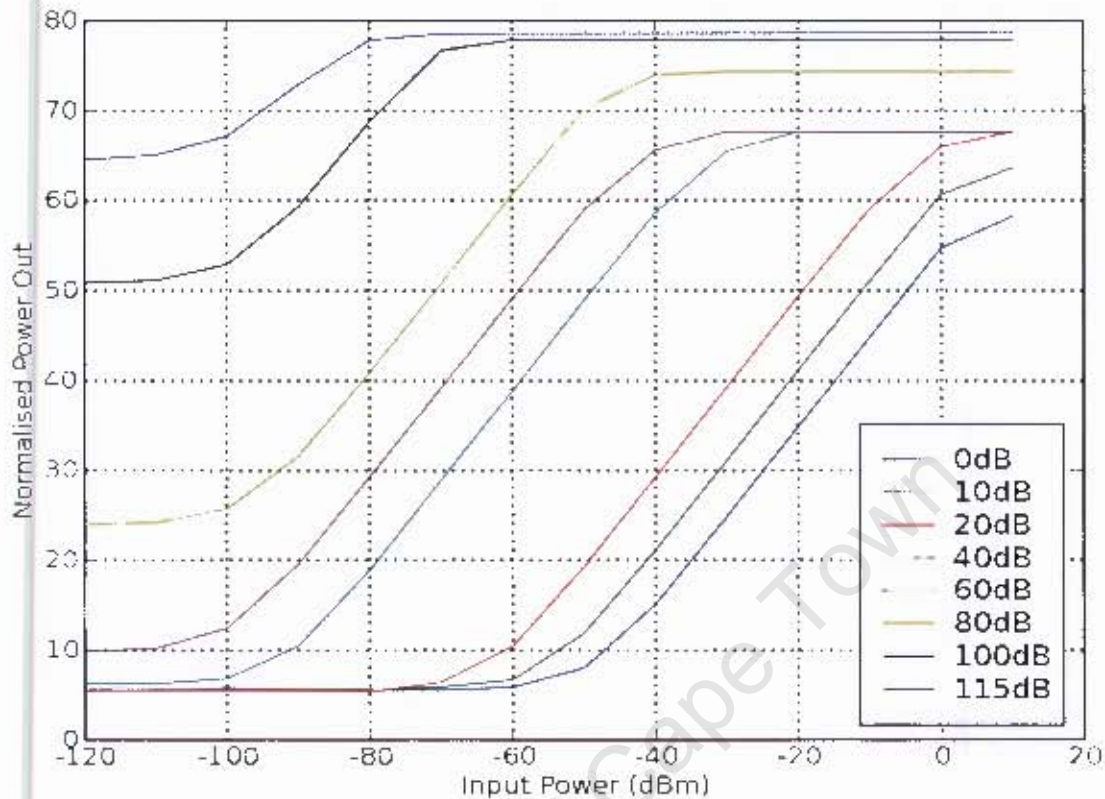
Figure 4.12: Input power against output power, showing receiver dynamic range
