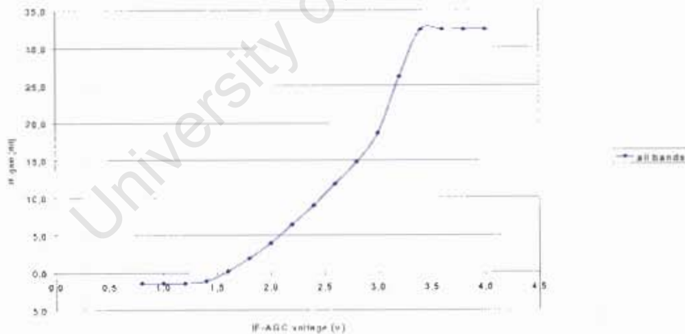
Figure 4 IF Gain vs. AGC Voltage
