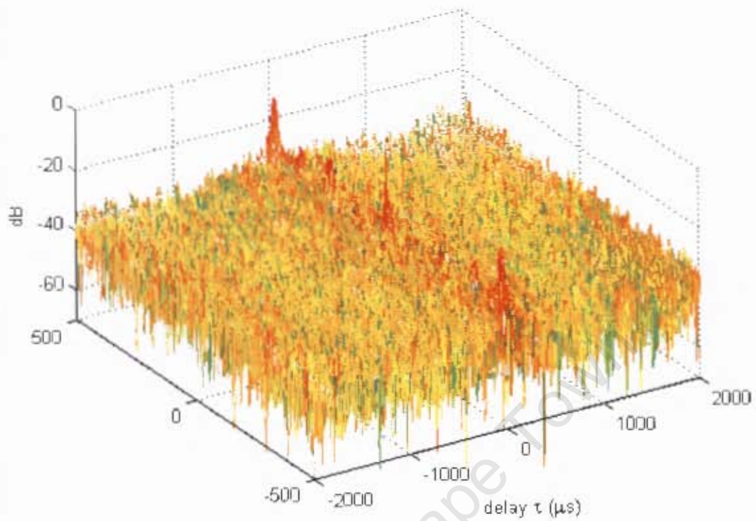
Figure A.2: Ambiguity plot of Classic FM transmission
