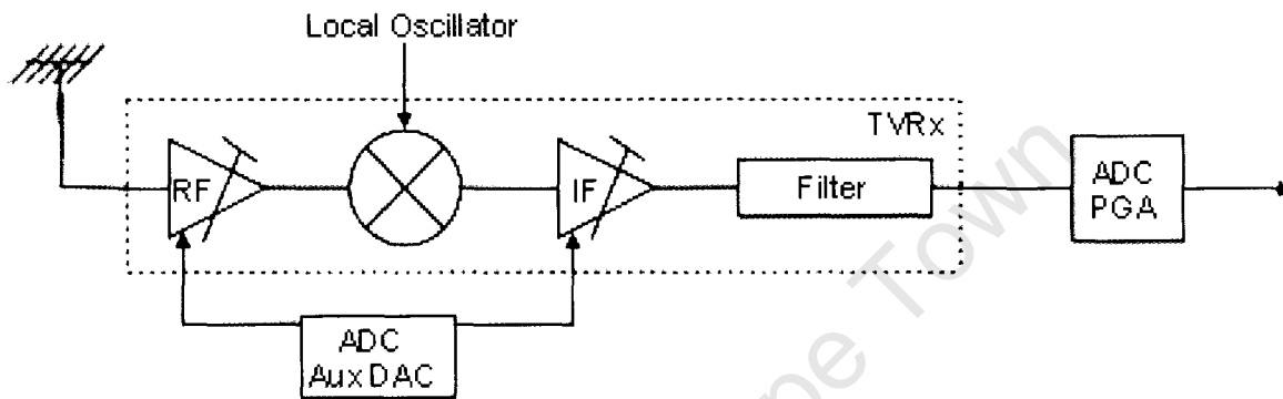
Figure 4.2: Block diagram showing TVRx gain stages
