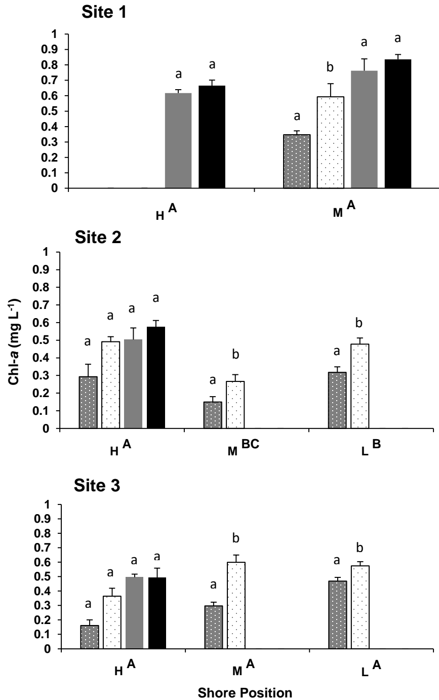
Figure 21: Differences in chl- a concentrations between flamingo foraging structures (channels: ■, pits: ■) and controls (channel controls: □, pit controls: ■) across the three sites and shore positions (H: high, M: mid, L: low). Different letters denote significant differences of total chl- a biomass between shore positions (in uppercase) and between a feeding structure and its control within a shore position (in lowercase). Means ± 1SE are shown.
