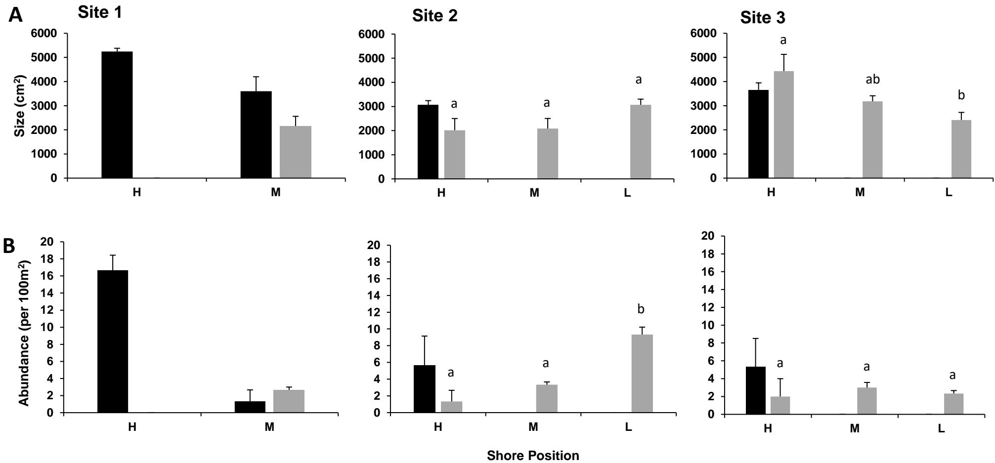
Figure 7: Differences in (A: size, B: abundance) of flamingo pit (■) and channel (■) foraging structures across the three sites and shore positions (H: high, M: mid, L: low). Different letters denote significant differences between shore positions. Means ± 1SE are shown.
