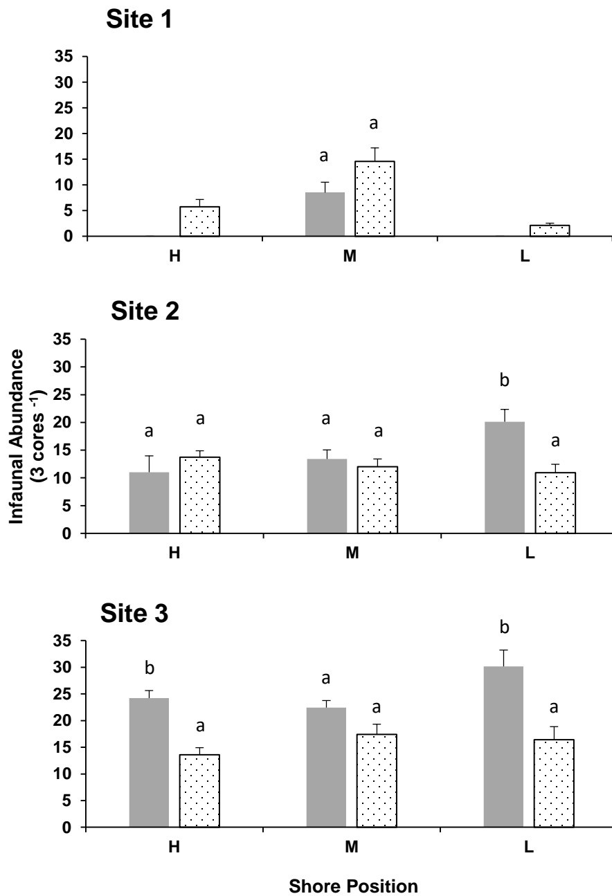
Figure 19: Differences in infaunal abundance between flamingo foraging structure controls (channels:■, pits:▨) and non-feeding controls (□) across the three sites and shore positions (H: high, M: mid, L: low). Different letters denote significant differences of abundance between a foraging structure control and non-feeding control within a shore position. Means \pm 1SE are shown.
