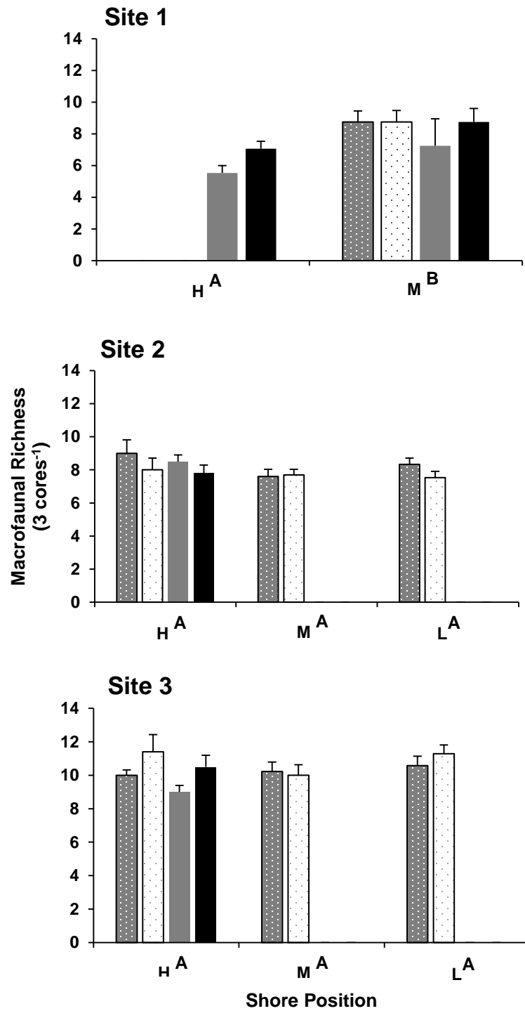
Figure 25: Differences in macrofaunal richness between flamingo foraging structures (channels: , pits : ) and controls (channel controls: , pit controls: ) across the three sites and shore positions (H: high, M: mid, L: low). Different letters denote significant differences of total richness between shore positions (in uppercase). Means \pm 1SE are shown.
