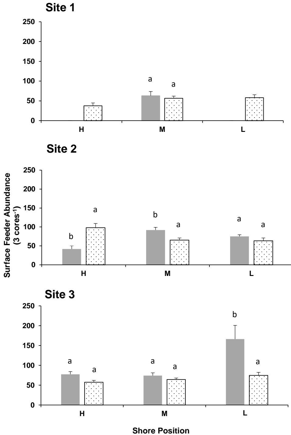
Figure 18: Differences in surface feeder abundance between flamingo channel-foraging controls (■) and non-feeding controls (▨) across the three sites and shore positions (H: high, M: mid, L: low). Different letters denote significant differences of abundance between channel-foraging controls and non-feeding controls within a shore position. Means \pm 1SE are shown.
