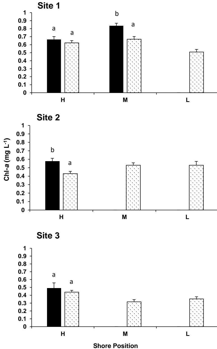
Figure 13: Differences in chl- a concentrations between flamingo pit-foraging controls (■) and non-feeding controls (▨) across the three sites and shore positions (H: high, M: mid, L: low). Different letters denote significant differences of chl- a between pit-foraging controls and non-feeding controls within a shore position. Means ± 1SE are shown.
