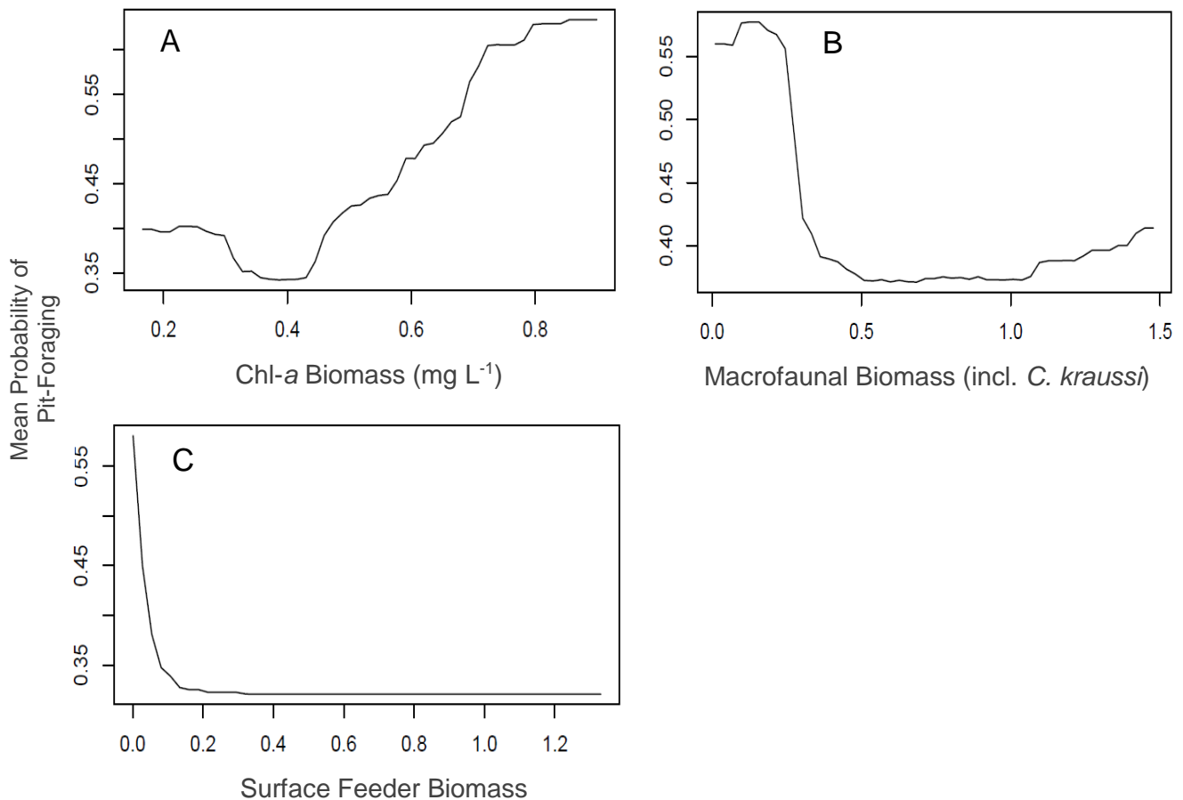
Figure 12: Best predictor variables (A: Chl- a Biomass, B: Macrofaunal Biomass (incl. C. kraussi ), C: Surface Feeder Biomass) of flamingo pit-foraging.
