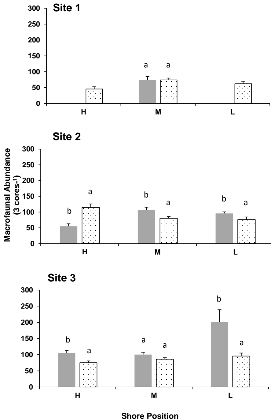
Figure 17: Differences in macrofaunal abundance between flamingo channel-foraging controls (■) and non-feeding controls (▨) across the three sites and shore positions (H: high, M: mid, L: low). Different letters denote significant differences of abundance between channel-foraging controls and non-feeding controls within a shore position. Means \pm 1SE are shown
