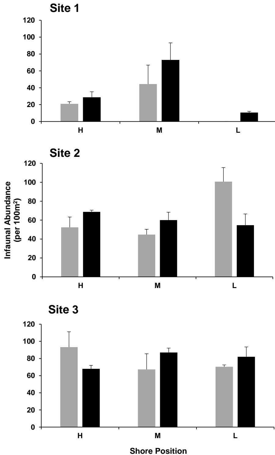
Figure 11: Differences in infaunal abundance between feeding (■) and non-feeding quadrats (■) across the three sites and shore positions (H: high, M: mid, L: low). Means \pm 1SE are shown.
