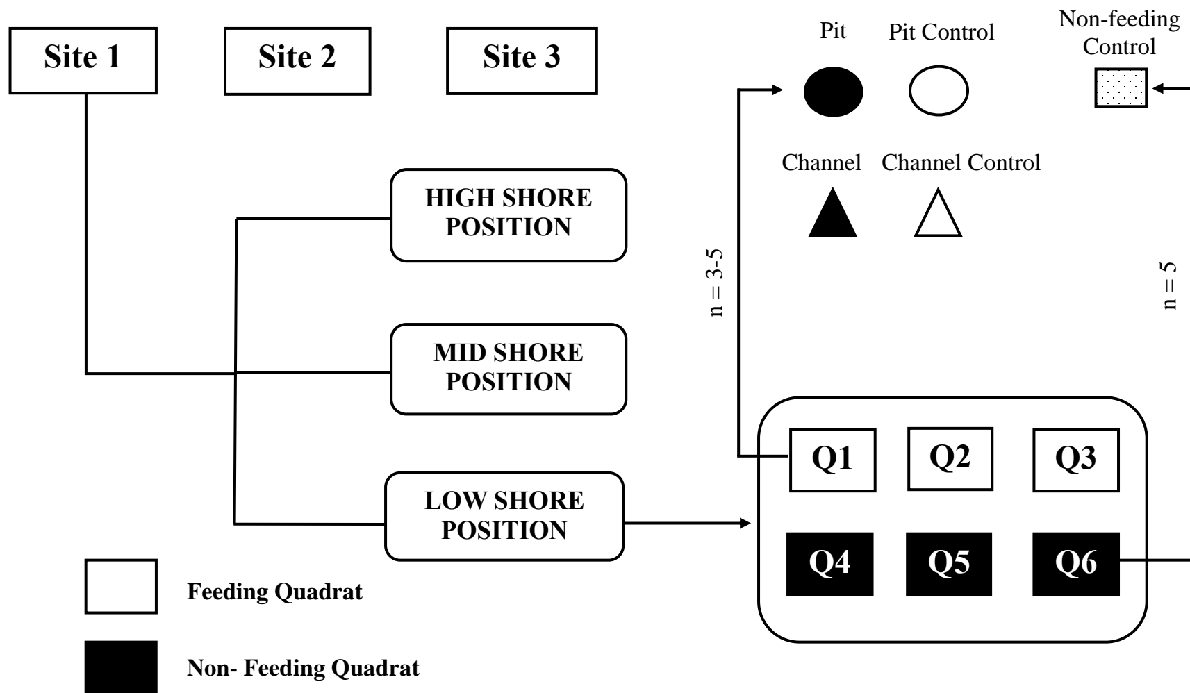
Figure 5: Schematic overview of nested sampling design used in the study. Three sites were sampled (Sites 1-3), comprising high-, mid- and low- water samples. Three feeding (Q1-3) and non-feeding quadrats (Q4-6) were sampled per shore position.
