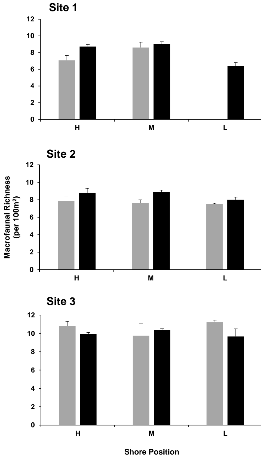
Figure 9: Differences in macrofaunal richness between feeding (■) and non-feeding quadrats (■) across the three sites and shore positions (H: high, M: mid, L: low). Means ± 1SE are shown.
