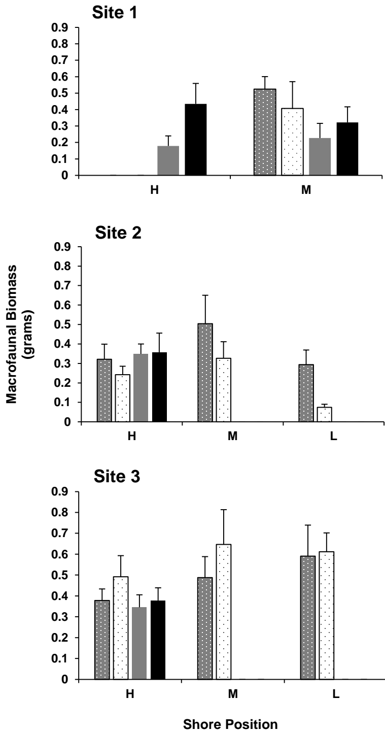
Figure 26: Differences in macrofaunal biomass between flamingo foraging structures (channels: , pits : ) and controls (channel controls: , pit controls: ) across the three sites and shore positions (H: high, M: mid, L: low). Means \pm 1SE are shown.
