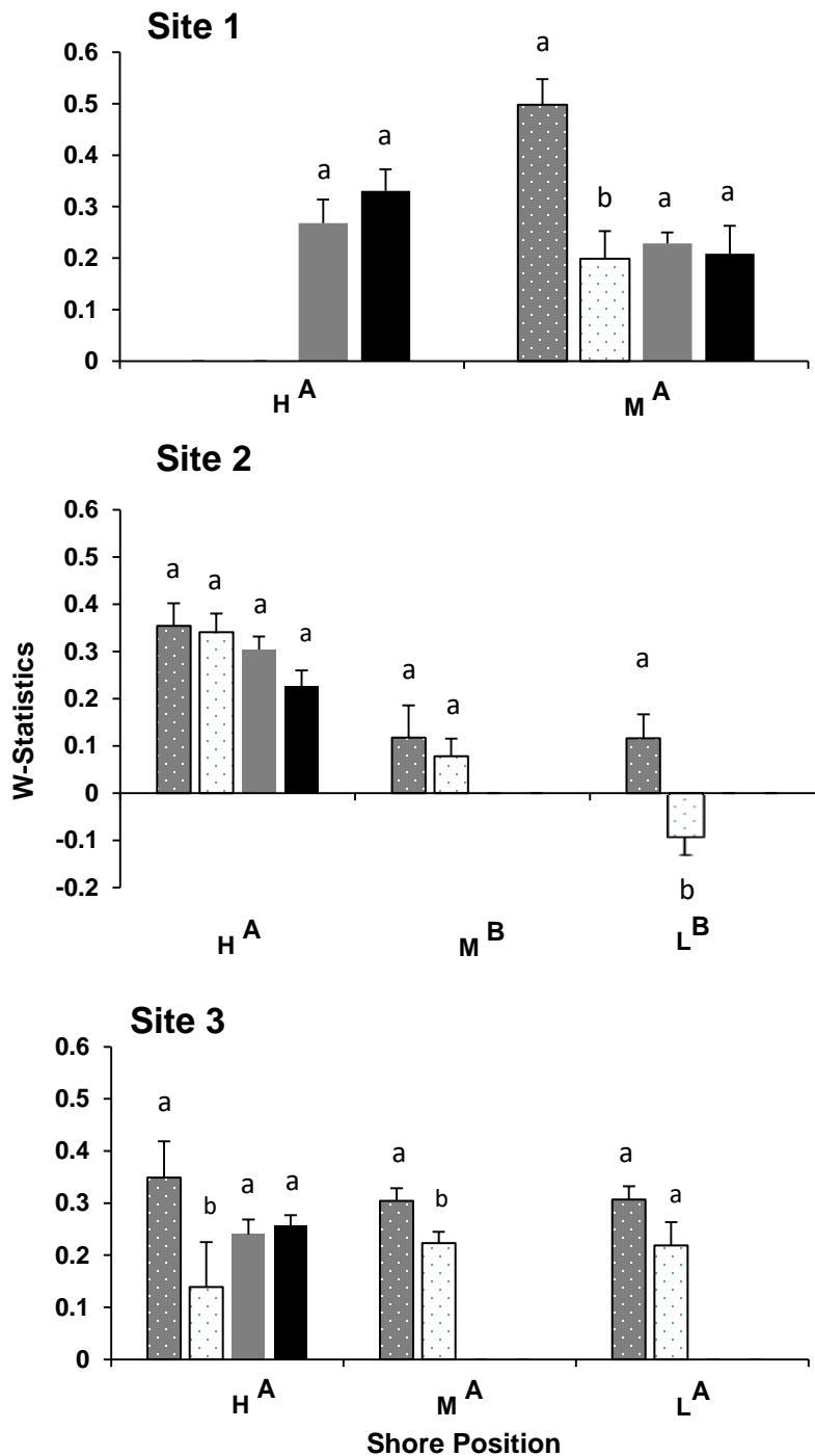
Figure 27: Differences in W-statistics between flamingo foraging structures (channels: , pits: ) and controls (channel controls: , pit controls: ) across the three sites and shore positions (H: high, M: mid, L: low). Different letters denote significant differences of total W-statistics between shore positions (in uppercase) and between a feeding structure and its control within a shore position (in lowercase). Means \pm 1SE are shown.
