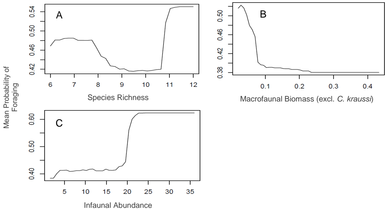
Figure 8: Best predictors (A: Species Richness, B: Macrofaunal Biomass (excl. C. kraussi ), C: Infaunal Abundance) of flamingo foraging.
