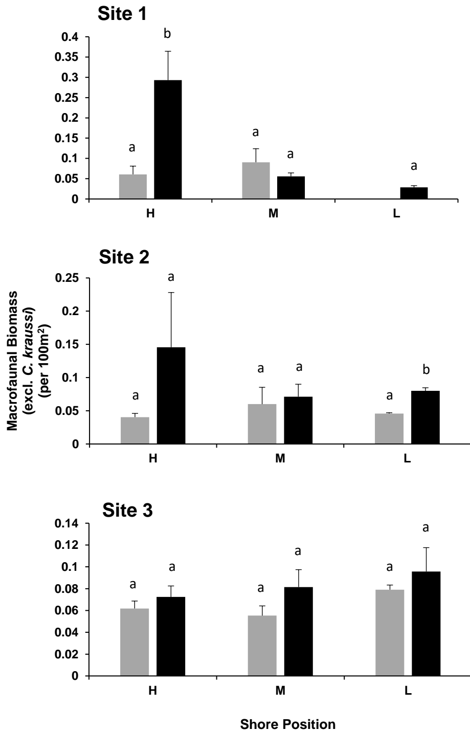
Figure 10: Differences in macrofaunal biomass (excl. C. kraussi ) between feeding (■) and non-feeding quadrats (■) across the three sites and shore positions (H: high, M: mid, L: low). Different letters denote significant differences of biomass between treatments within a shore position. Means \pm 1SE are shown.
