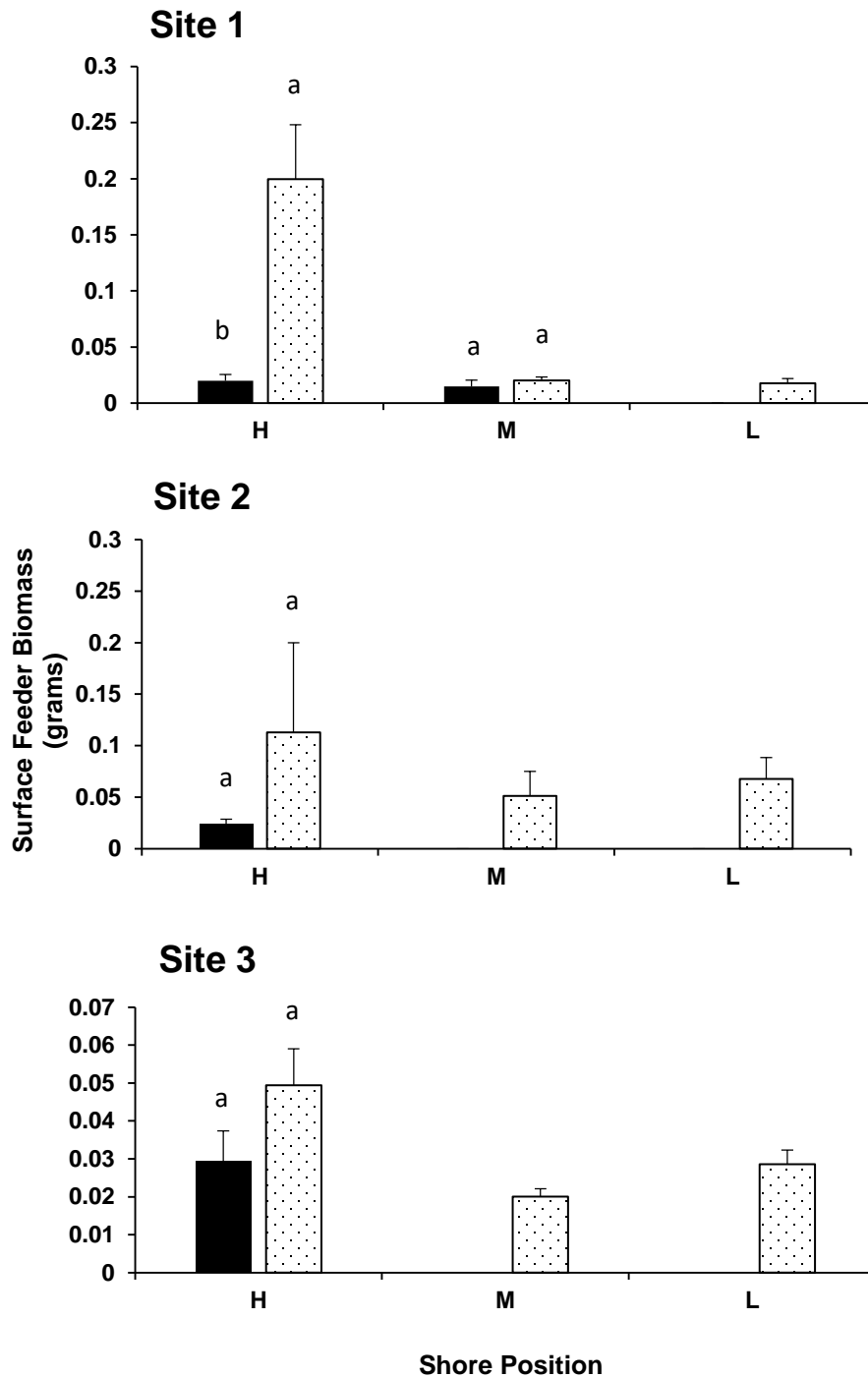
Figure 14: Differences in surface feeder biomass between flamingo pit-foraging controls (■) and non-feeding controls (▨) across the three sites and shore positions (H: high, M: mid, L: low). Different letters denote significant differences between pit-foraging controls and non-feeding controls within a shore position. Means \pm 1SE are shown.
