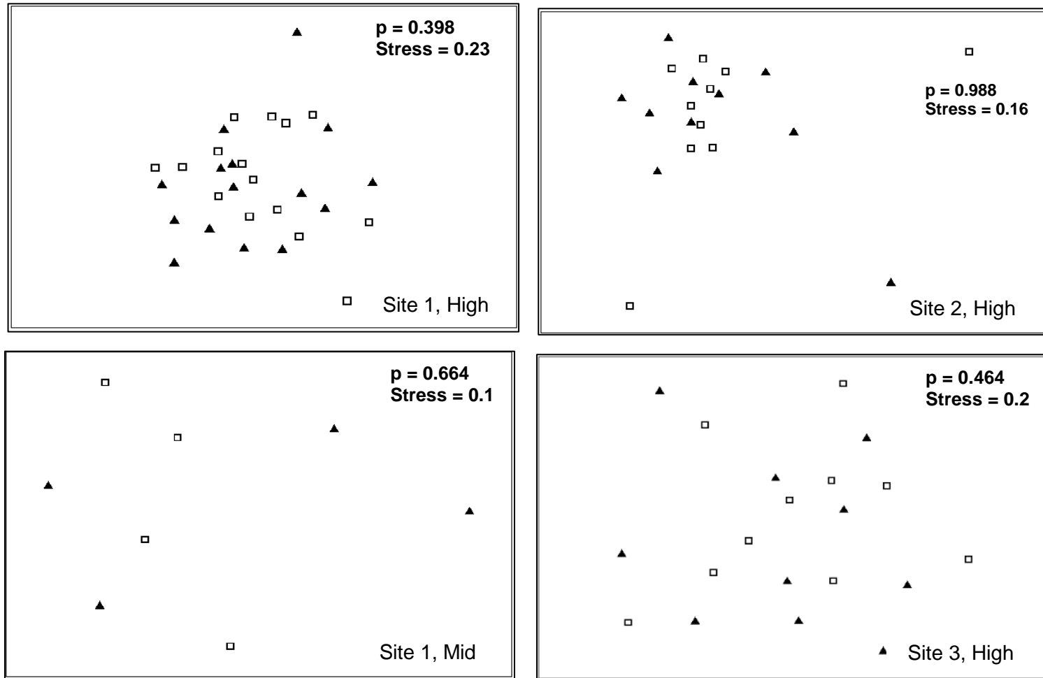
Figure 23: MDS ordinations showing differences in macrofaunal community structure between pits (▲) and pit controls (□) across the three sites at the high-and mid-shore position. Pair-wise testing with p values provided.
