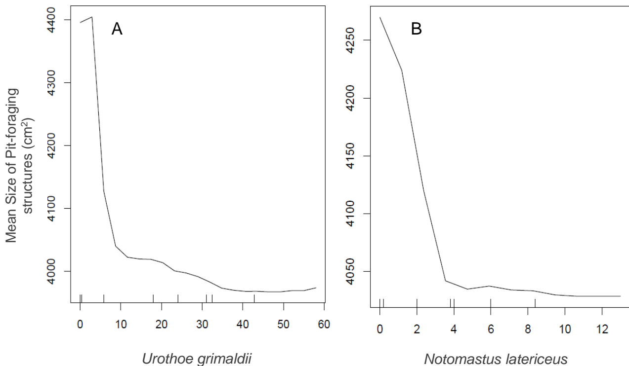
Figure 20: The abundance of (A: Urothoe grimaldii , B: Notomastus latericeus ) were the best predictor variables in driving the size variability of flamingo pit-foraging structures.
