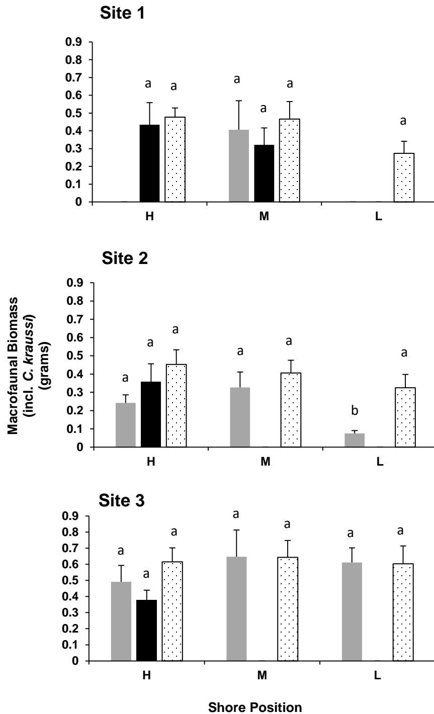
Figure 15: Differences in macrofaunal biomass (incl. C. kraussi ) between flamingo foraging structure controls (channels: ■, pits: ■) and non-feeding controls (▨) across the three sites and shore positions (H: high, M: mid, L: low). Different letters denote significant differences of biomass between a foraging structure control and non-feeding control within a shore position. Means \pm 1SE are shown.
