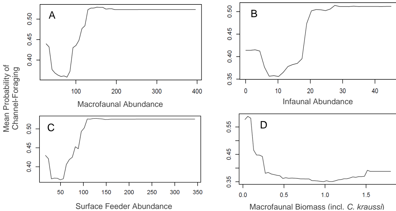
Figure 16: Best predictor variables (A: Macrofaunal Abundance, B: Infaunal Abundance, C: Surface Feeder Abundance, D: Macrofaunal Biomass (incl. C. kraussi )) of flamingo channel-foraging.
