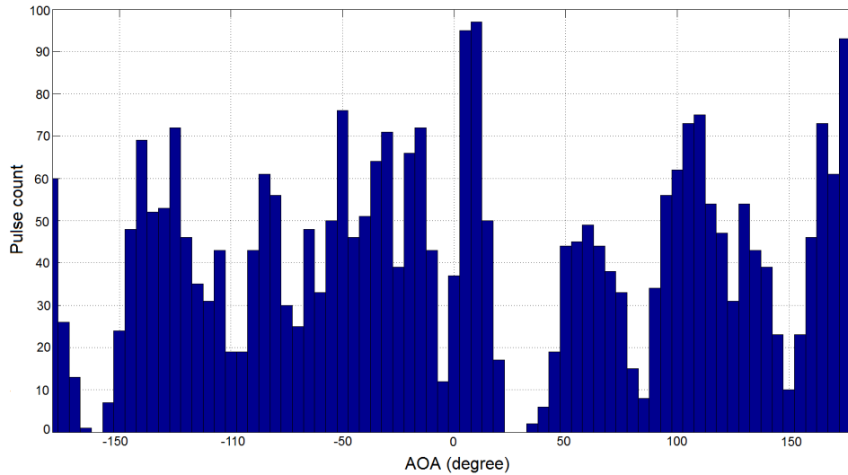
Figure 4.1: AOA histogram of randomly located emitters (30 emitters). The accuracy of AOA is 5^\circ .
