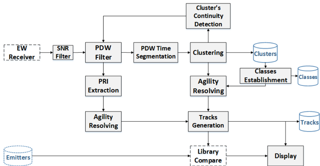
Figure 4.3: Proposed De-interleaving System.
