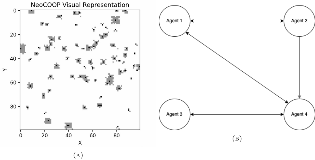
FIGURE 2.1: A figure showing the different types of ABM environments. (A) showcases a spatially-explicit grid-world environment where black pixels represent settlements, grey pixels represent farmland and white pixels represent uninhabited land. (B) showcases a spatially-implicit relationship graph where agents must be connected if they are to interact with each other. These relationships may be bidirectional ( Agent1 < - > Agent4 ) or unidirectional ( Agent2 - > Agent4 )
