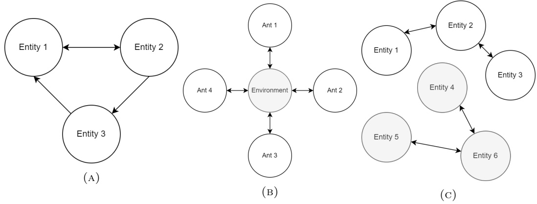
FIGURE 3.8: Various types of information exchange networks. (a) Showcases an example of direct exchange. Connections are directed meaning that Entity 1 and Entity 2 can exchange information while Entity 3 can only receive information from Entity 2 and send information to Entity 1. (b) Showcases an example of indirect exchange. Ants do not directly exchange information amongst themselves. They instead communicate indirectly by exchanging information with the environment entity. (c) Showcases exclusive exchange whereby Entities 1, 2 and 3 are able to exchange information amongst themselves but unable to exchange information with Entities 4, 5 and 6 which form their own sub-network.
