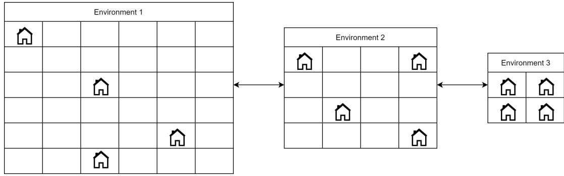
FIGURE 5.2: An example of the proposed "Islands" Model. Here we have three environments of decreasing size (increased resource stress). The environments are represented as a graph such that an agent in Environment 3 would first need to migrate to Environment 2 before migrating to Environment 1.
