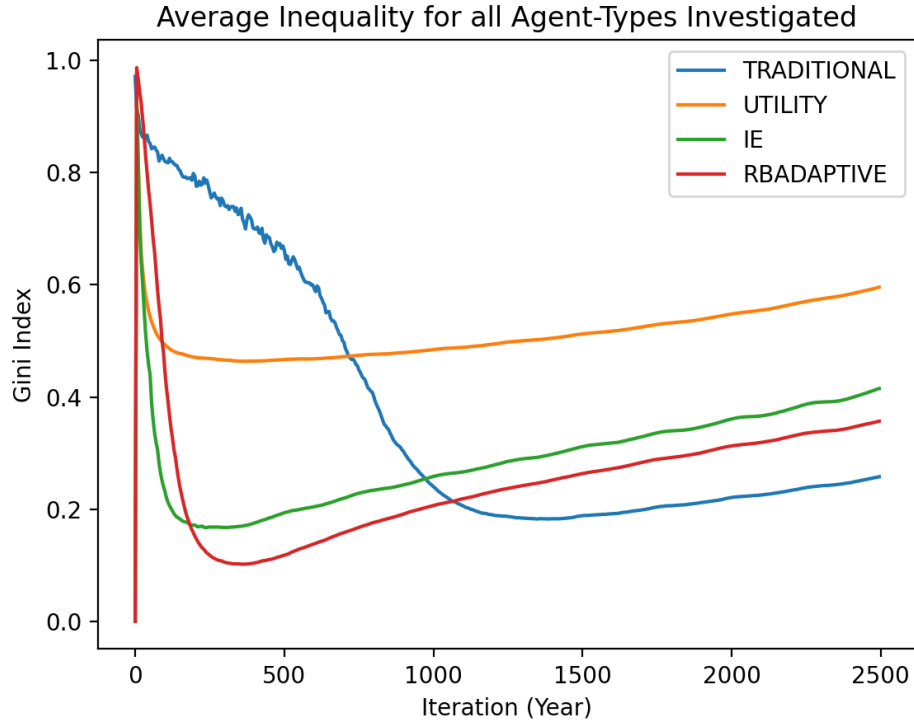
FIGURE 4.7: Average Gini-Index of each agent-type investigated.
