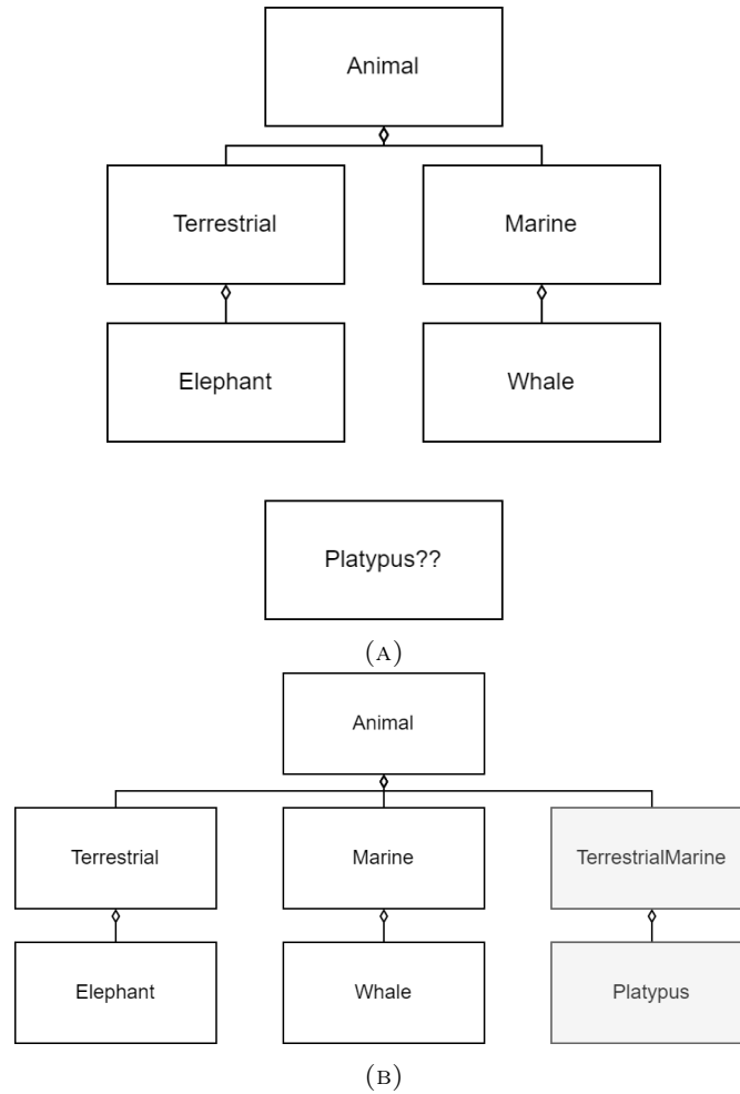
FIGURE 3.1: A figure showing the difficulty of maintaining inheritance trees for certain types of software. (a) Demonstrates that the Platypus class can't be created without inheriting from both Terrestrial and Marine . (b) Shows the inelegant solution of creating a third class called TerrestrialMarine which the Platypus class can inherit from.
