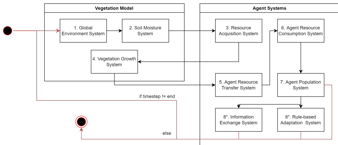
FIGURE 3.20: A figure depicting the execution order of NeoCOOP 's systems. The number that prefixes the system's name indicates its position in the execution queue. The Information Exchange System and Rule-based Adaptation systems are present when the type of agent being investigated are the IE and rb-adaptive agents respectively.
