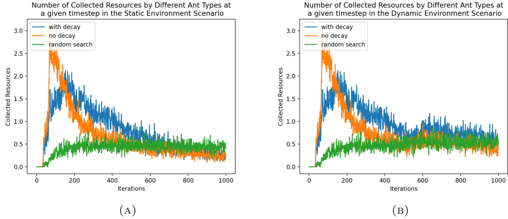
FIGURE 3.14: Rate of resource collection for each Ant-type across both the static (a) and dynamic (b) scenarios.
