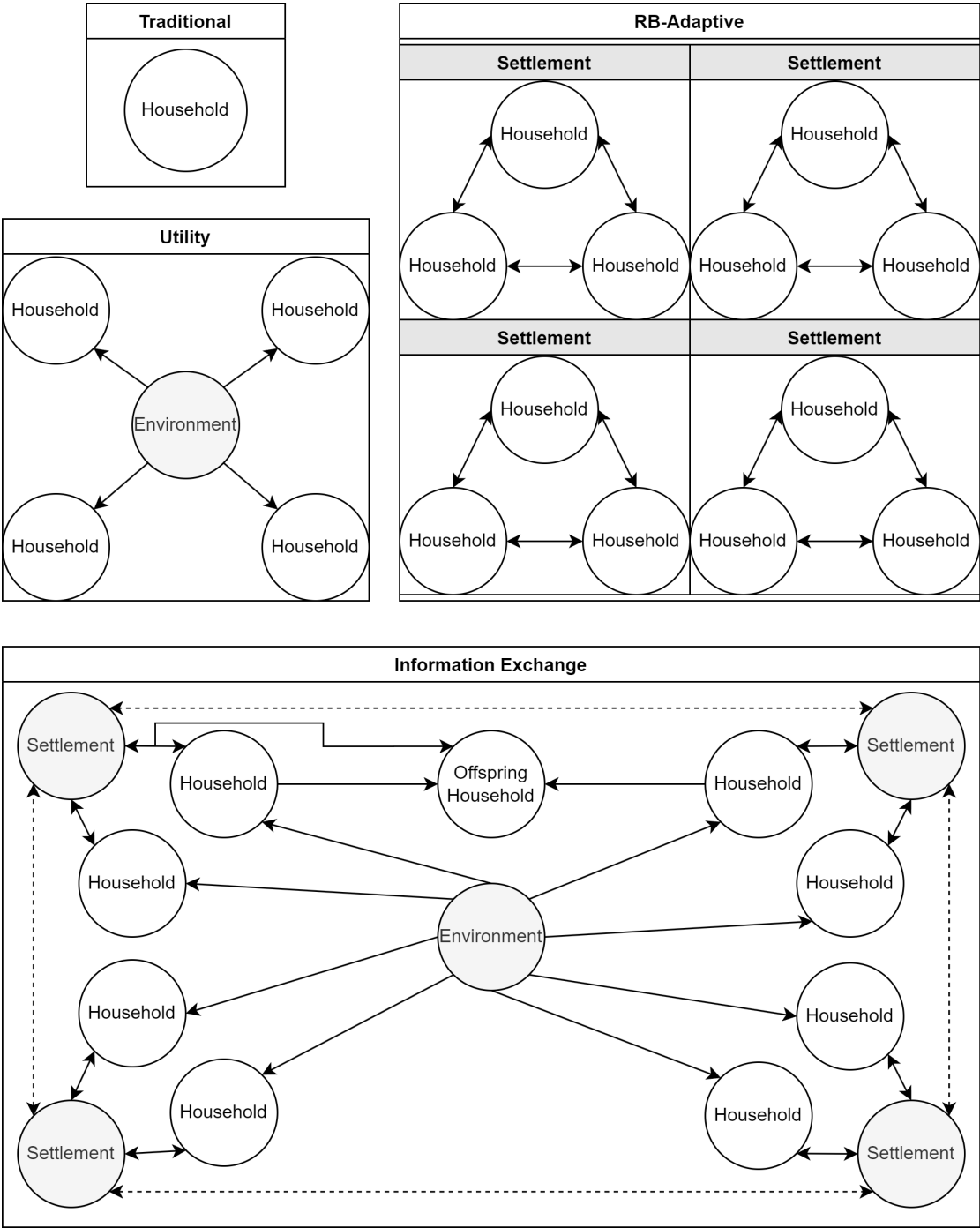
FIGURE 3.19: An information exchange perspective of the agent-types at some arbitrary timestep. Note: All settlement entities in the Information Exchange agent network should be linked. The diagonal connections were omitted for visual clarity.
