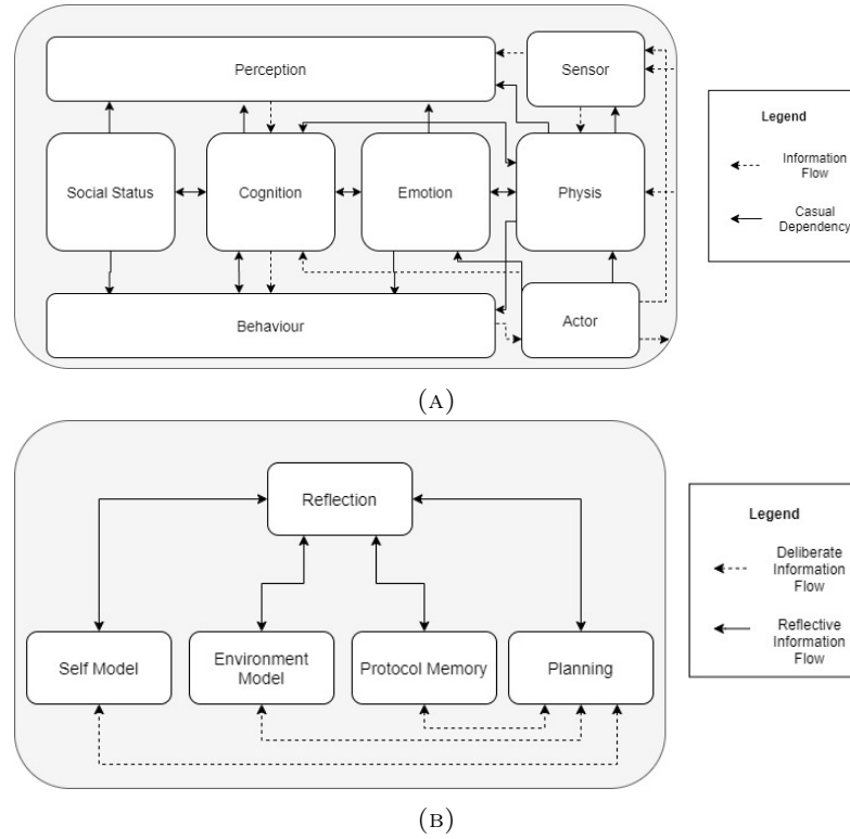
FIGURE 2.3: A figure showing the PECS [2, 3] Model (A) and a closer look at the Cognition component (B)
