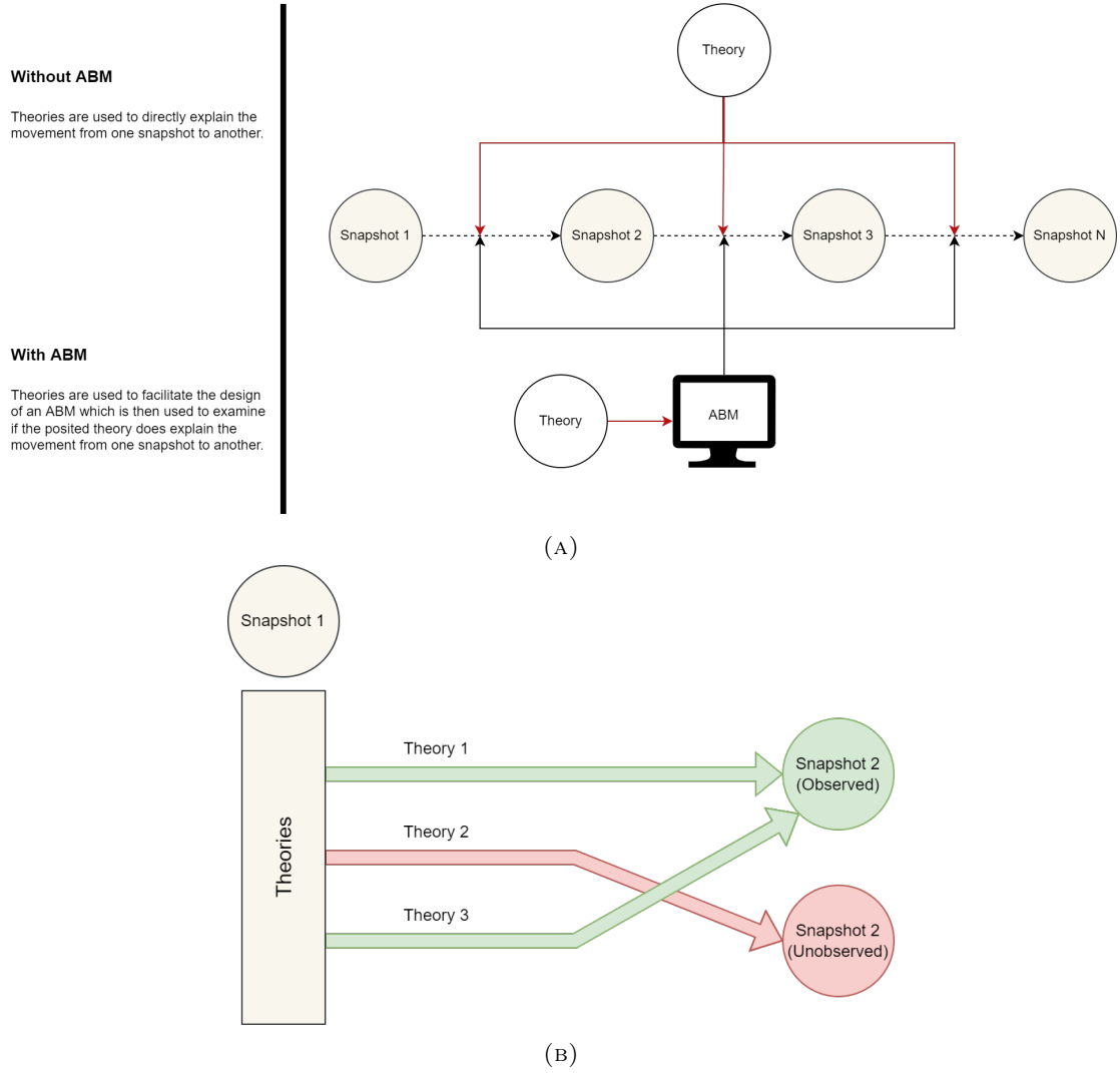
FIGURE 1.2: Figures of topics surrounding the usage of ABM in Computational Archaeology. (a) Demonstrates how ABM are used to provide empirical evidence to support theoretical constructions of snapshot (the state of the environment at some timestep) transitions while (b) illustrates the concept of Equifinality which states that multiple theories (indicated in green) might explain the transition from one snapshot to another.
