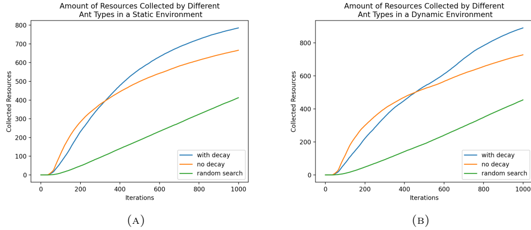
FIGURE 3.12: Number of collected resources for each Ant-type across both the static (a) and dynamic (b) scenarios.
