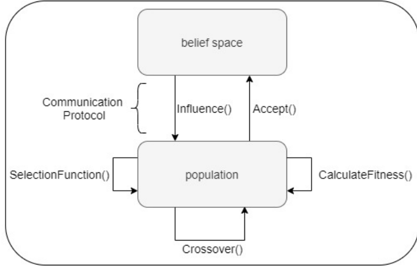
FIGURE 2.6: A component view of a CA. (Adapted from Reynolds et al.[5])
