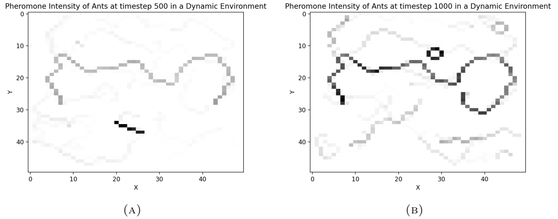
FIGURE 3.15: The pheromone intensity of the 'with decay' ant type at timestep 500 (a) and timestep 1000 (b).
