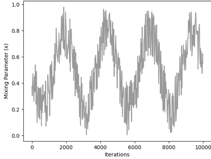
FIGURE 4.2: An example of how the mixing parameter x is generated over the course of a simulation run for a single vegetation model property (temperature, rainfall, flood height). In this example, f = 2500 .
