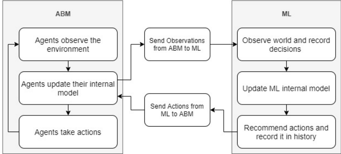
FIGURE 2.4: A "model refinement" design for a ML integrated adaptive ABM as described by Rand [4]
