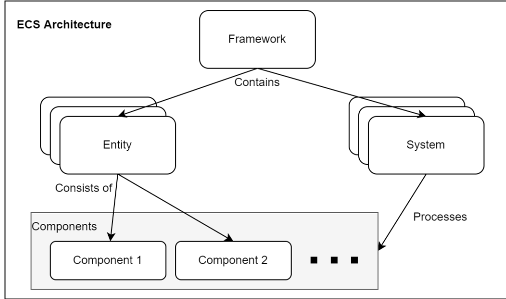
FIGURE 3.2: The structure of a typical ECS framework. Adapted from Hatledal et al. [6].
