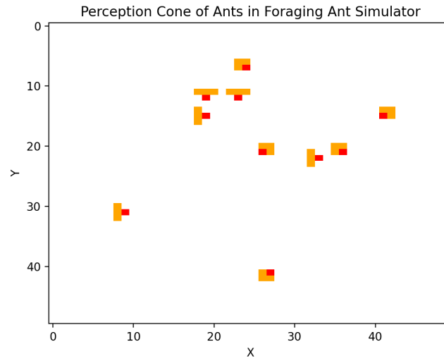
FIGURE 3.10: A Figure demonstrating the perception cone of the Ant agents. The red pixels are ant agents and the orange pixels are the cells they query to determine which path to follow.
