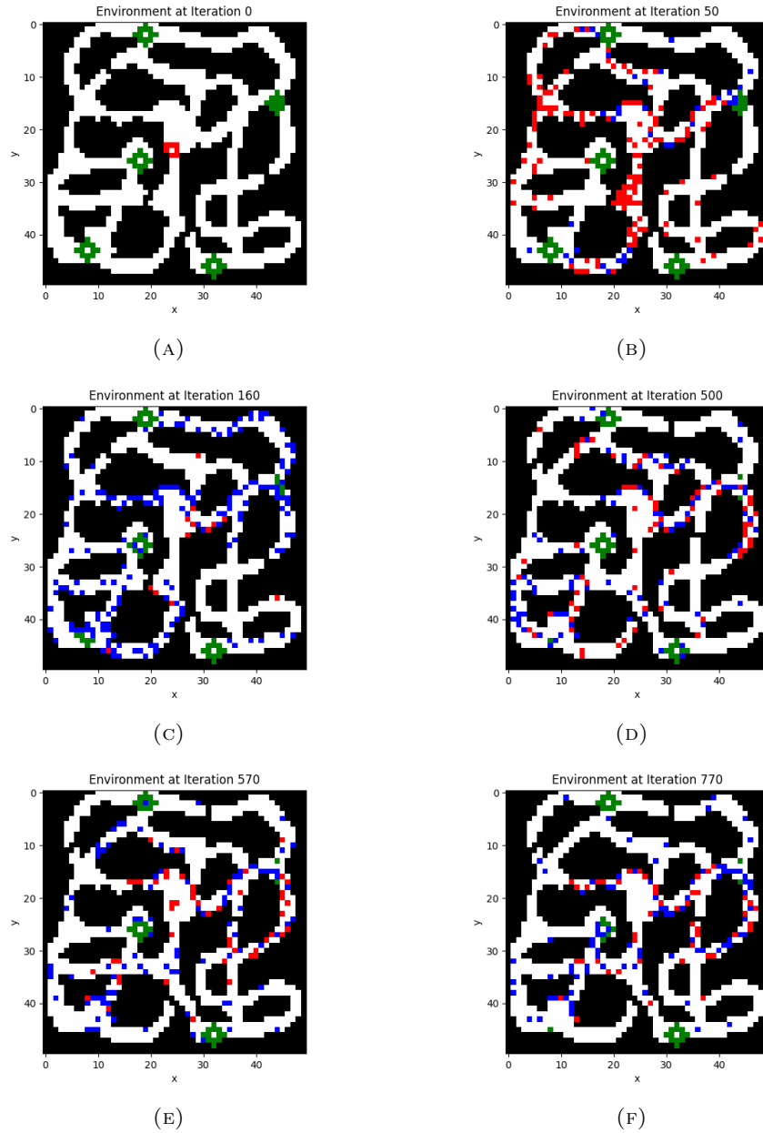
FIGURE 3.13: Figures showcasing the 'with decay' Ants at various stages in a typical model run. Red pixels are ants looking for resources, blue pixels are ants carrying resources and green pixels are cells that contain resources.
