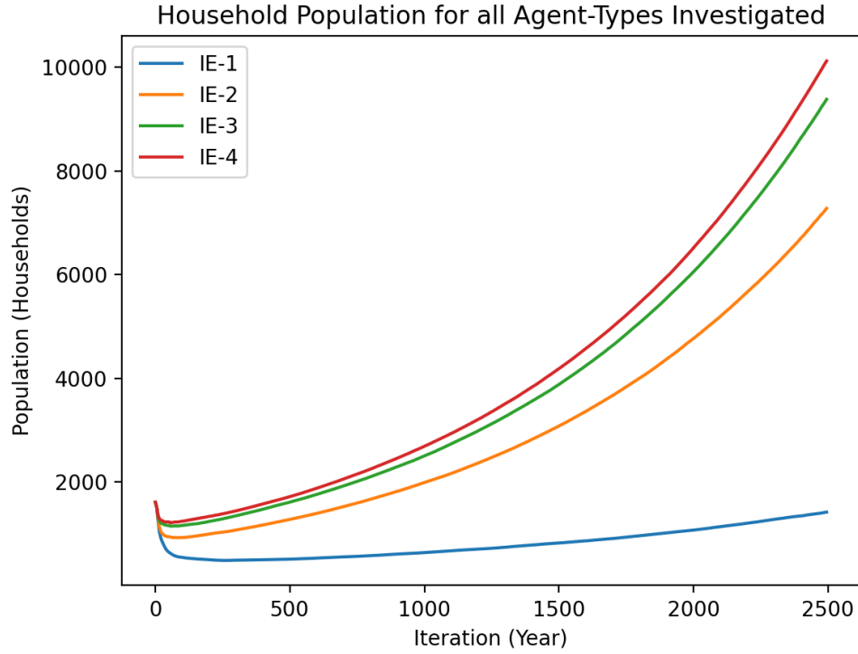
FIGURE 4.5: Household population levels for farming production rate supplementary experiments. Note: The Figure is labelled such that IE-N indicates that the IE agent-type was used with a farm_production_rate of N .
