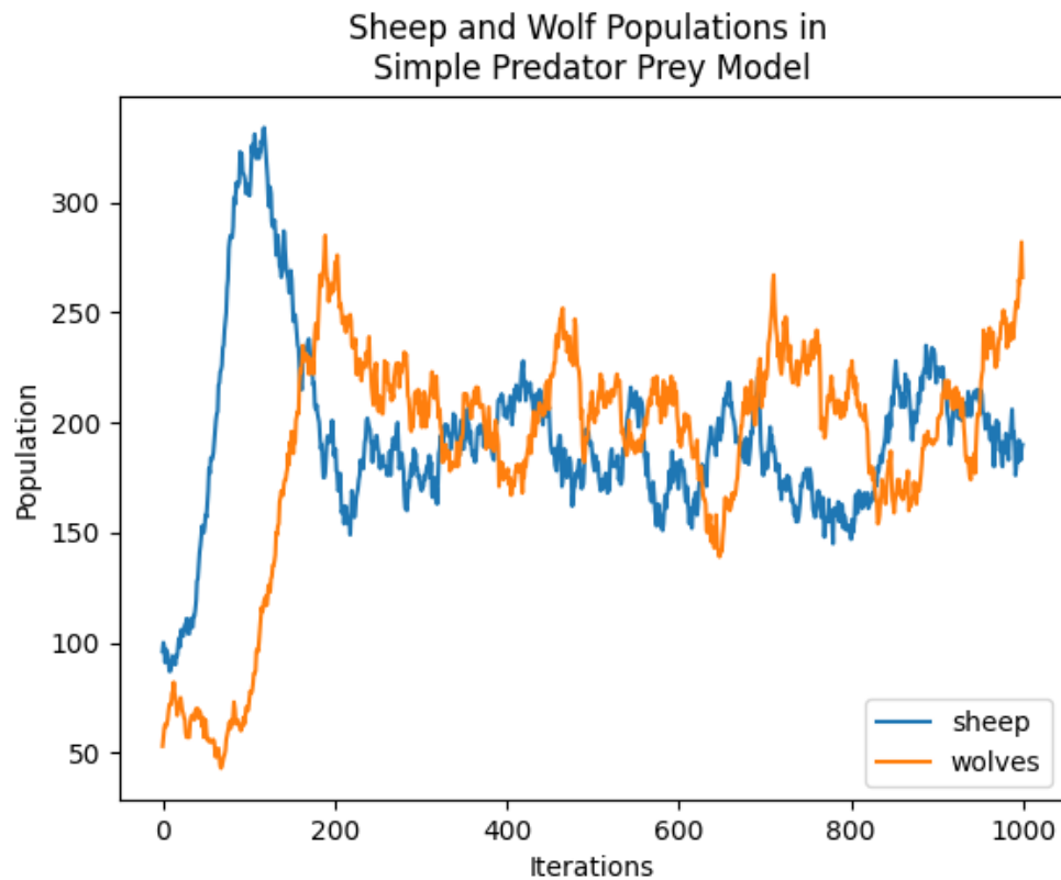
FIGURE 3.6: Wolf and Sheep populations simulated over 1000 iterations.
