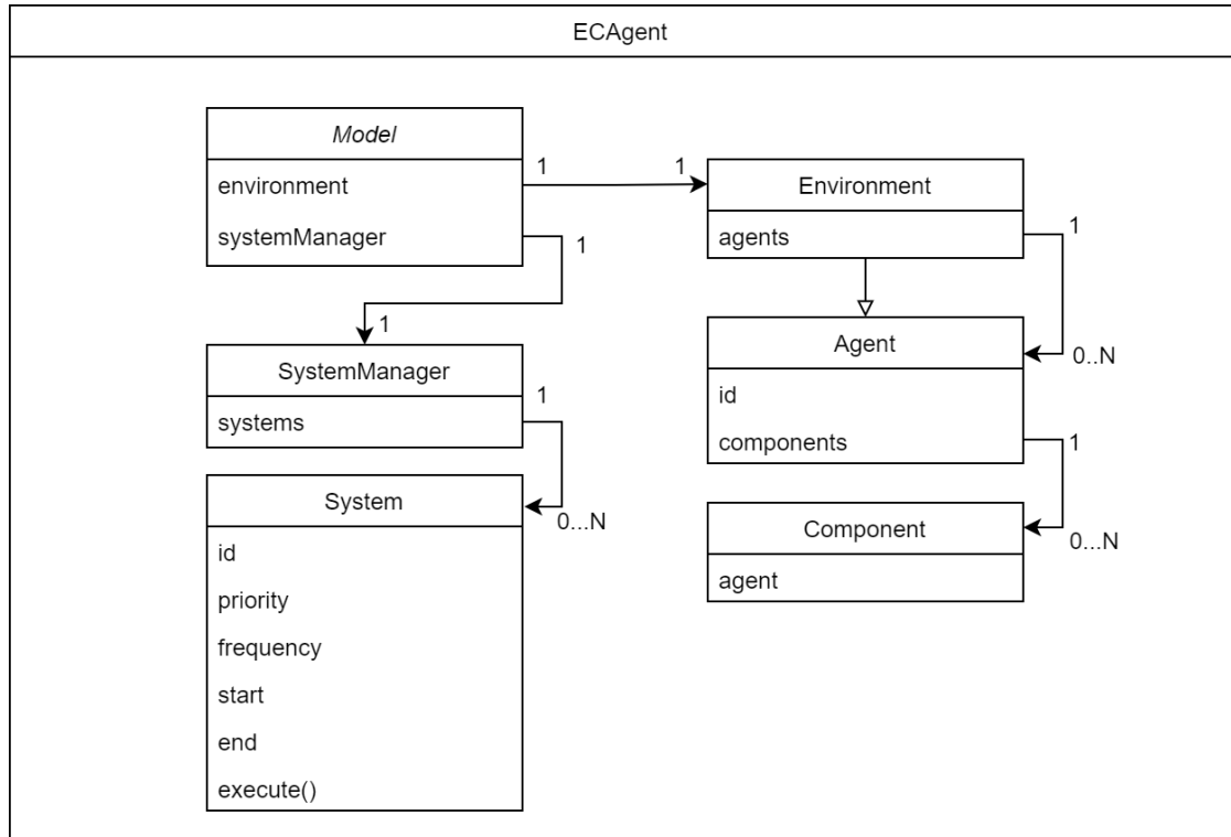
FIGURE 3.3: High-level overview of ECAgent .
