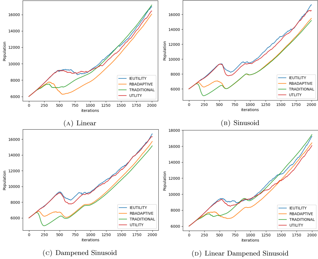
FIGURE D.1: Final Individual population levels for the exploratory experiments.
