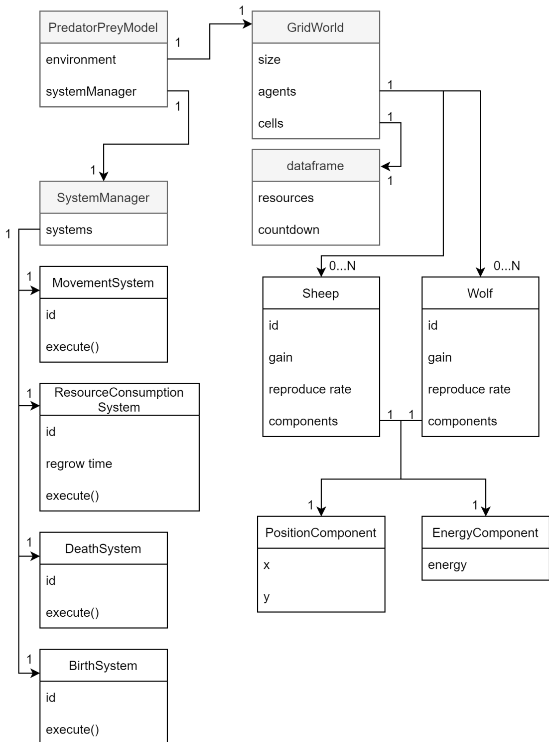
FIGURE 3.5: UML Diagram of the Simple Predator-Prey Model implemented in ECAgent . Classes highlighted in grey are included with ECAgent .
