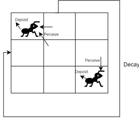
FIGURE 3.11: The information exchange network of the Foraging Ant Model. Ants deposit pheromones onto grid cells they visit. They perceive the pheromones on grid cells in the direction they're facing and, if enabled, the environment will decay the amount of pheromones on each of its grid cells in accordance with the decay_factor .
