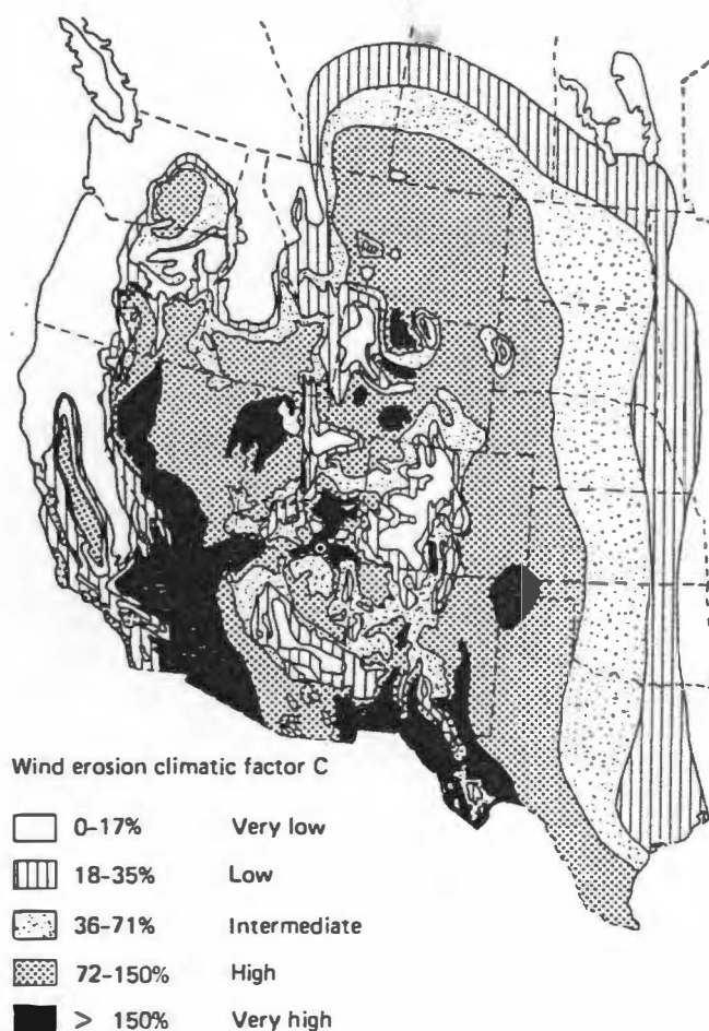
FIGURE 4.3 Wind erosion climatic factor C', as a percentage of the value at Garden City, Kansas (taken from Chepil et al 1962).
