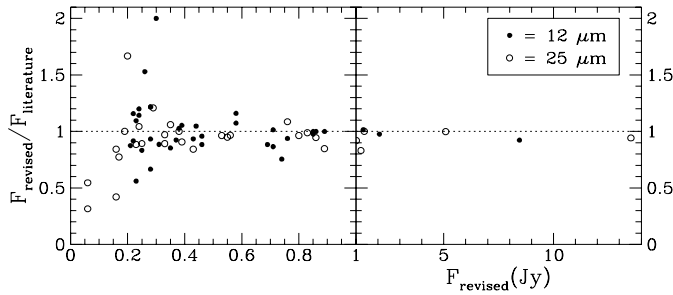
Fig. 1. A comparison of the estimates of IRAS flux densities given here and values from the IRAS Point Source Catalogue and Schwing & Israel (1990), at 12 (solid symbols) and 25 \mu\text{m} (open symbols).
