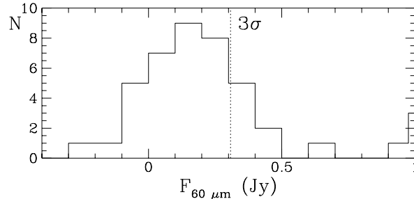
Fig. 3. Histogram of the distribution of ISO 60 \mu\text{m} flux densities (chopped measurements). The dotted vertical line indicates 3- \sigma flux density derived from the distribution of negative flux densities. All flux densities over 1 Jy are piled up in the last bin.
