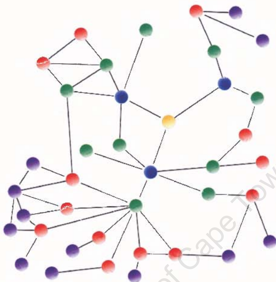
Figure 28. An egocentric subgraph of radius four centred on the orange node
