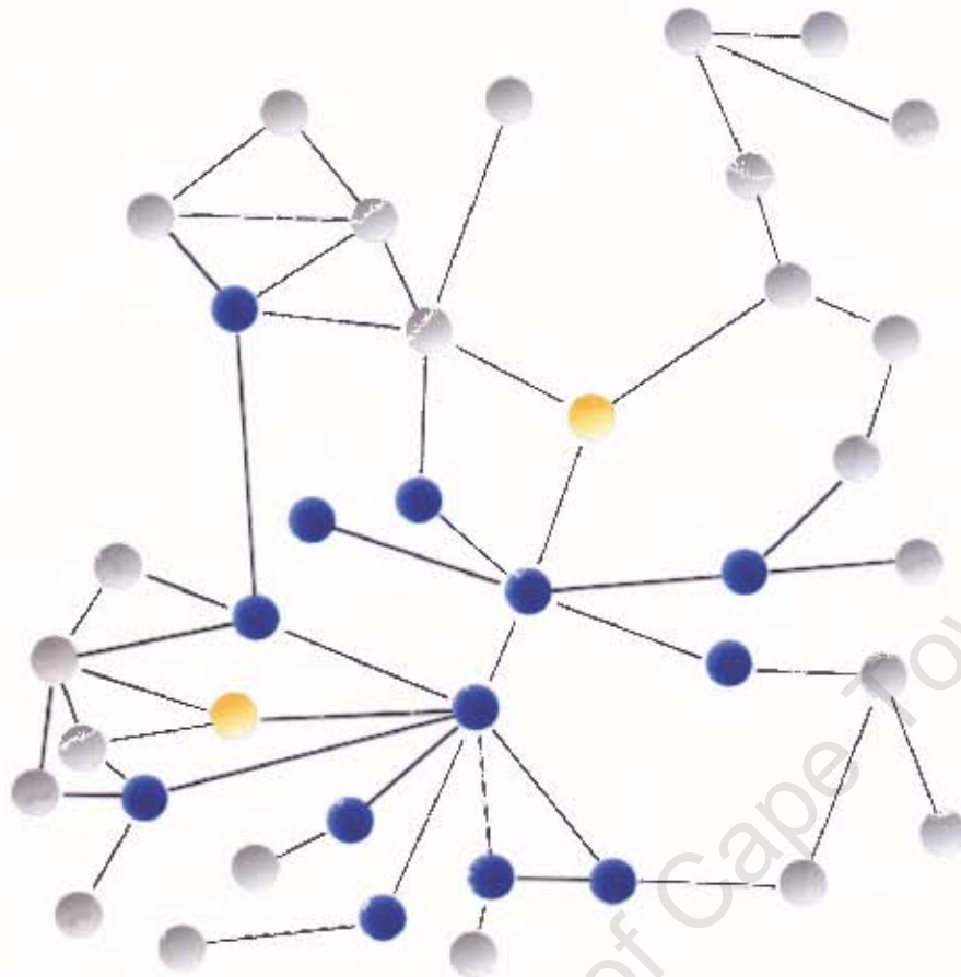
Figure 32. Radius three common neighbours
