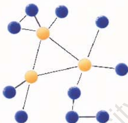
Figure 5. A scale-free graph
