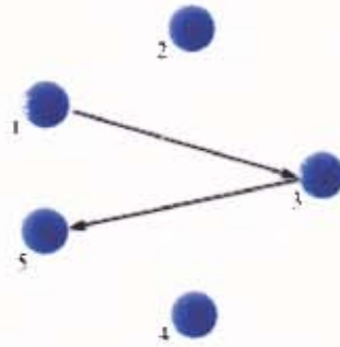
Figure 3. A directed labelled five node graph
