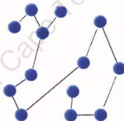
Figure 6. A non scale-free graph
