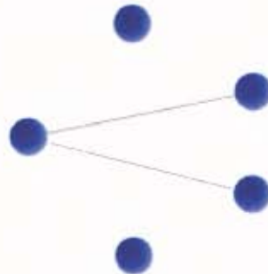
Figure 1. A graph with five nodes and two edges
