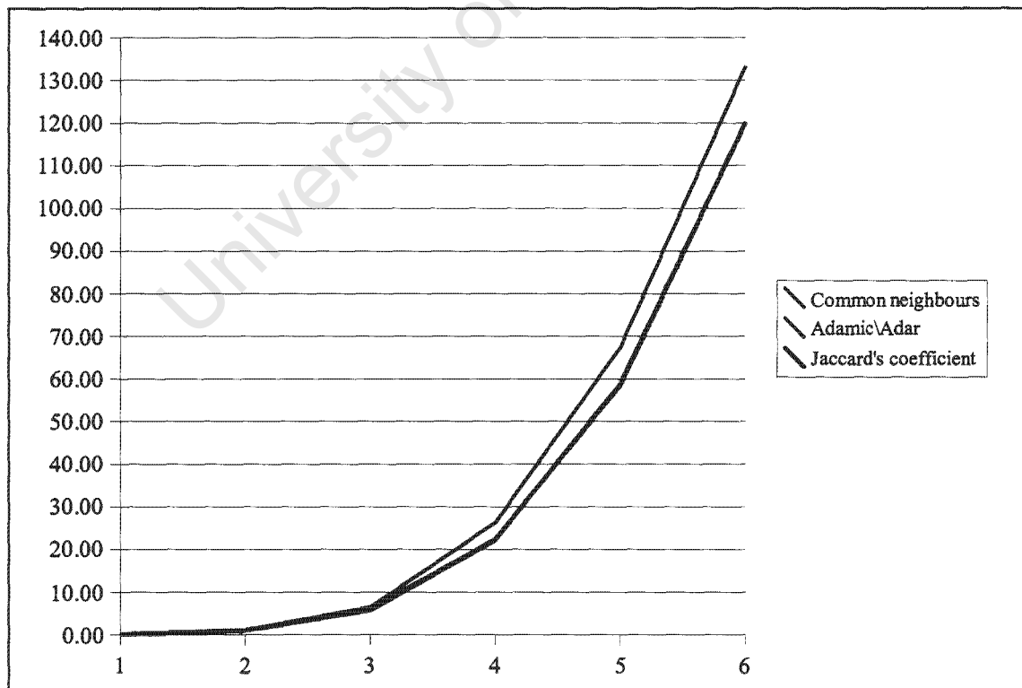
Figure 35. Computational time in milliseconds per radius
