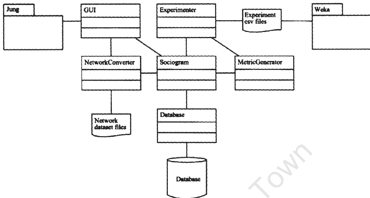
Figure 12. Sociogram sequence analysis system overview
