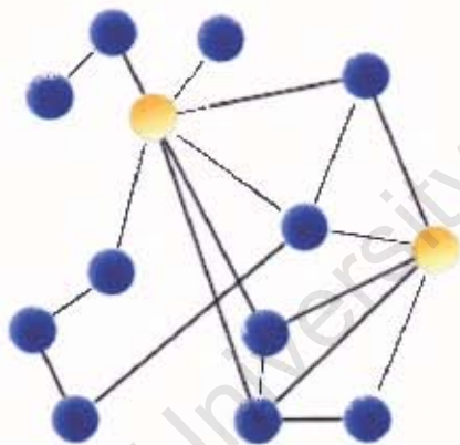
Figure 9. A graph at time step t where a new link is forming
