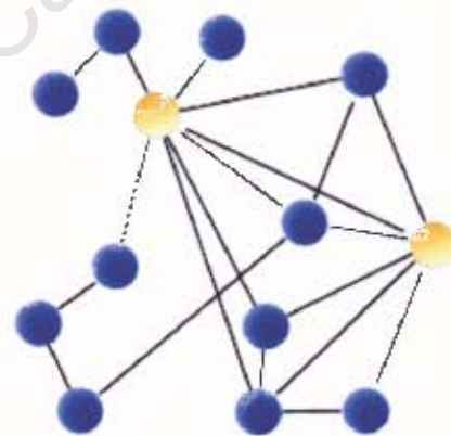
Figure 10. A graph at time step t+1 where a new link has formed
