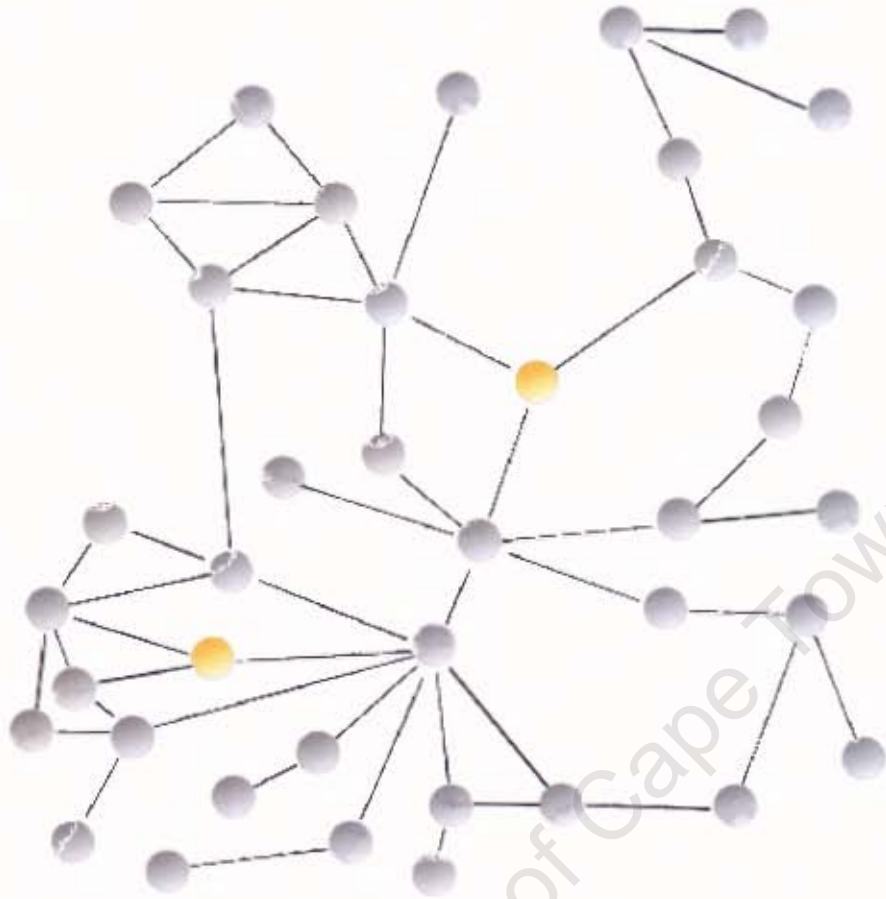
Figure 30. Radius one common neighbours
