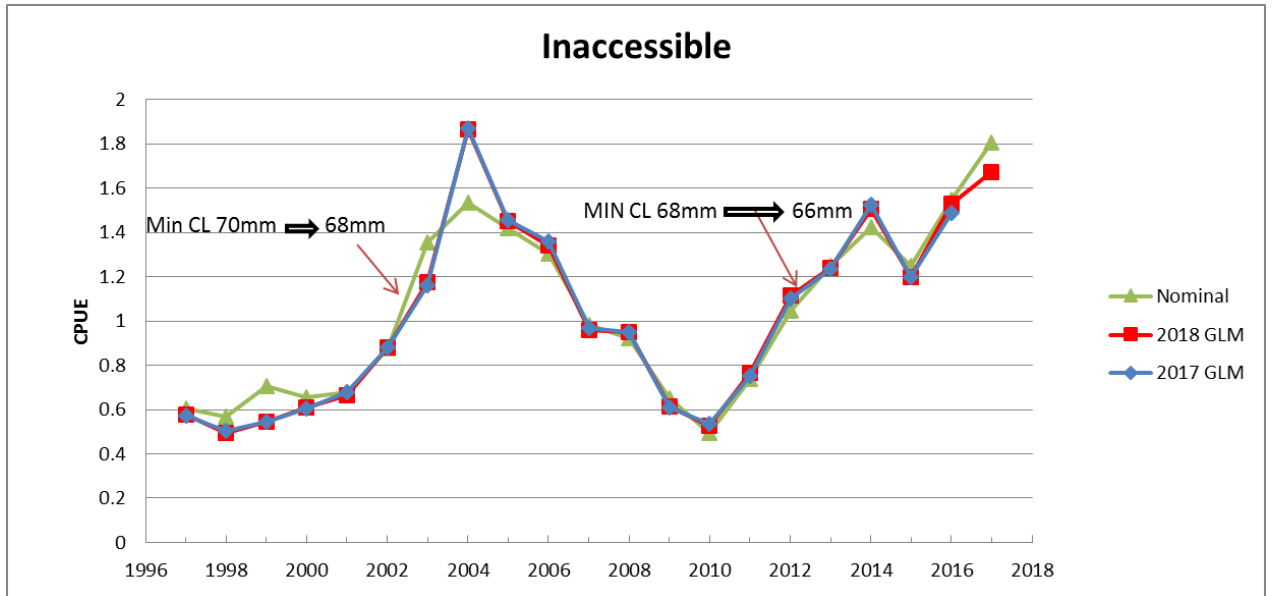
Figure 1a: Comparative plot of the adjusted nominal and GLMM standardised longline CPUE series for Inaccessible Island. All series have been renormalised to a mean of 1 (for 1997-2016) for easier comparison of trends. Note that here and below the standardised 2018 results for certain years are not visible as they are covered by the values for standardisations in earlier years. [Note that the minimum legal carapace size changed from 70mm to 68mm CL in 2003 and from 68mm to 66mm CL in 2012.]
