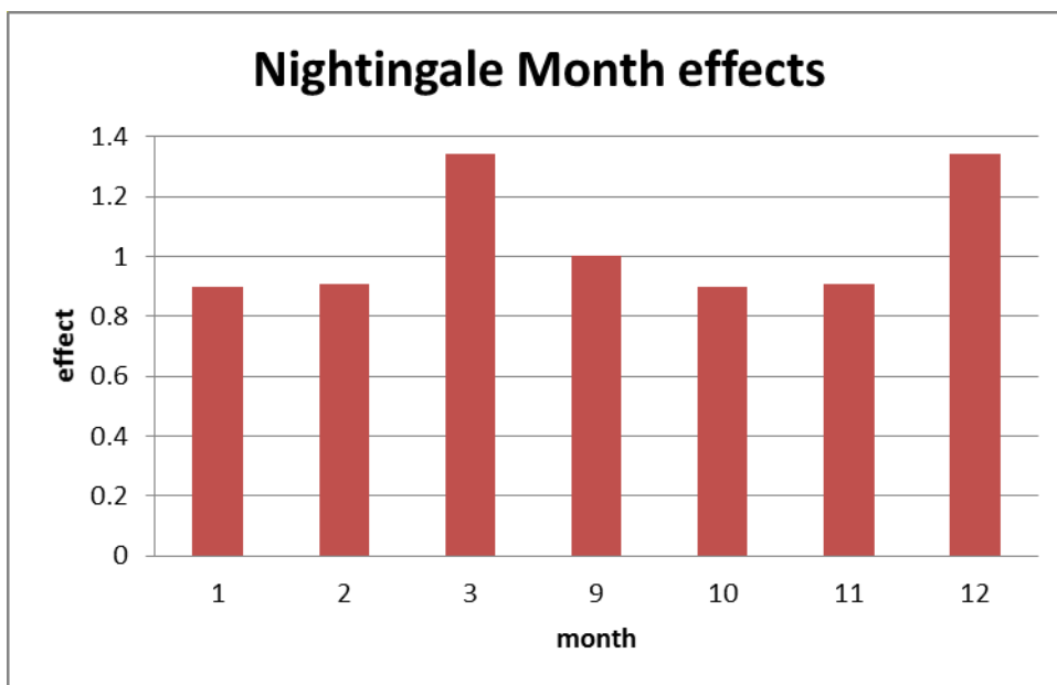
Figure 2b: GLMM month effects for Nightingale Island.
