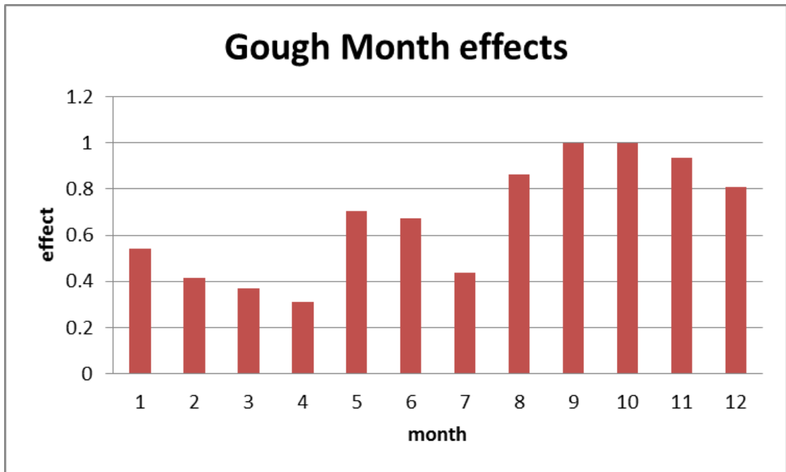
Figure 2c: GLMM month effects for Gough Island.
