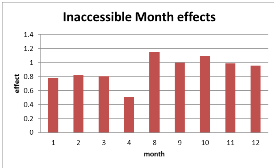
Figure 2a: GLMM month effects for Inaccessible Island.
