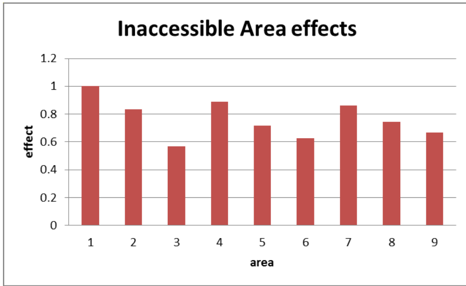
Figure 3a: GLMM area effects for Inaccessible Island (see Table 1a for area definitions).
