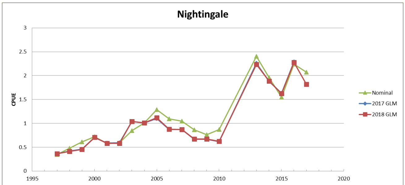
Figure 1b: Comparative plot of the adjusted nominal and GLMM standardised longline CPUE series for Nightingale Island. All series have been renormalised to a mean of 1 (for 1997-2016) for easier comparison of trends.
