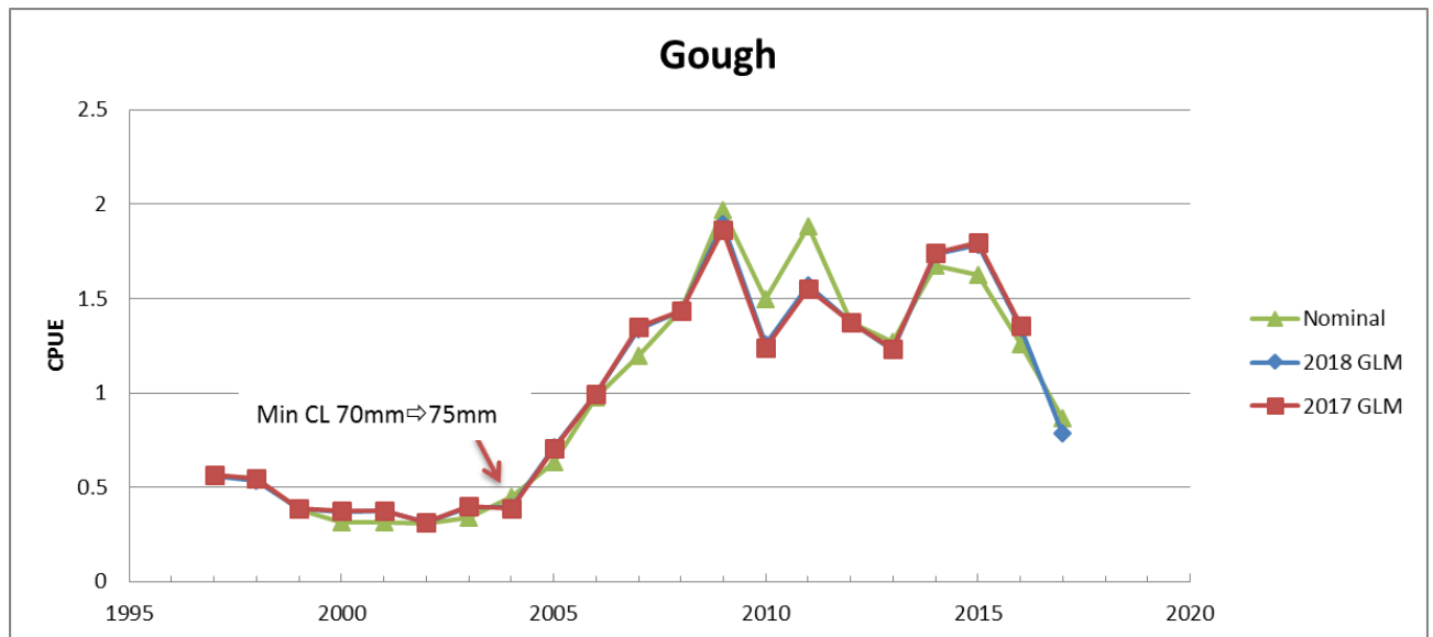
Figure 1c: Comparative plot of the adjusted nominal and GLMM standardised longline CPUE series for Gough Island. All series have been renormalised to a mean of 1 (for 1997-2016) for easier comparison of trends. [Note that the minimum legal carapace size changed from 70mm to 75mm in 2003.]
