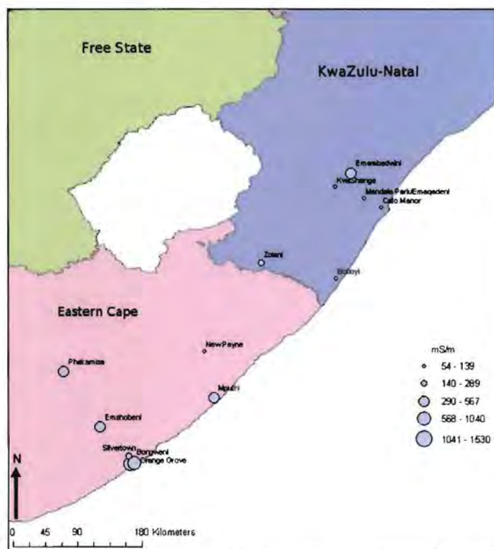
Figure B3.17: Electrical conductivity figures for Eastern Cape and KZN sites (Loudon, 2006)
