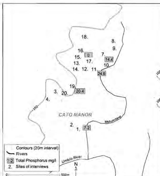
Figure 4.1.6: Cato Manor study showing sites of 19 interviews and Total Phosphorous as P (mg/l) at selected sites (Winter, 2006)
