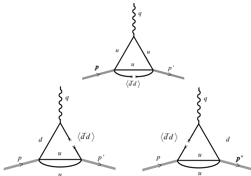
Figure 3: Non-vanishing terms proportional to the down-quark condensate, equation (19).
