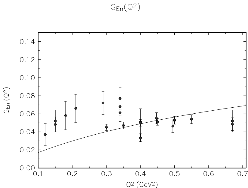
Figure 5: Experimental data on G_E(Q^2) for the neutron [10], together with the theoretical results from equations (24-25).
