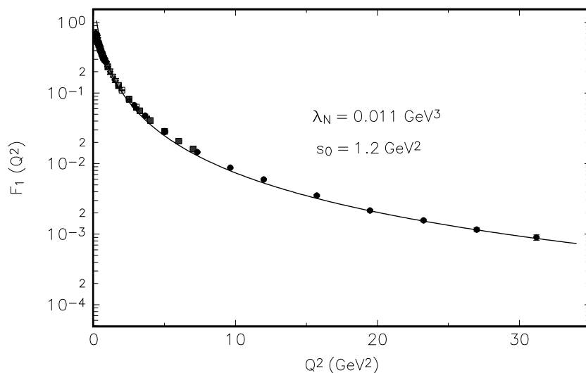
Figure 4: Corrected experimental data on F_1(Q^2) for the proton, [9], together with the theoretical result from equation (16) (solid line).
