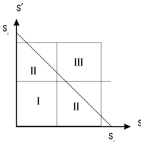
Figure 2: Triangular and rectangular integration regions of the Finite Energy Sum Rules, equation (15).
