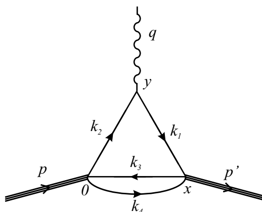
Figure 1: The three-point function, equation (1), to leading order in perturbative QCD.
