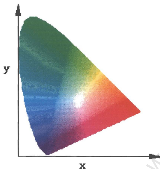
Figure 3.3: CIE chromaticity diagram
