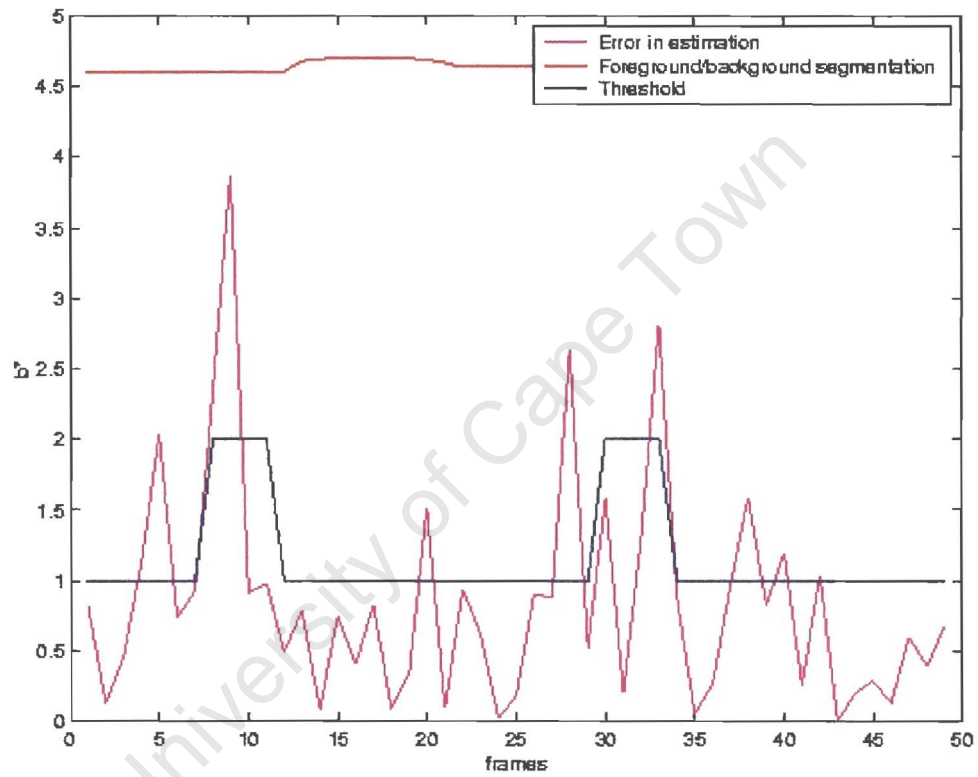
Figure 5.8: Estimation error and threshold for one pixel
