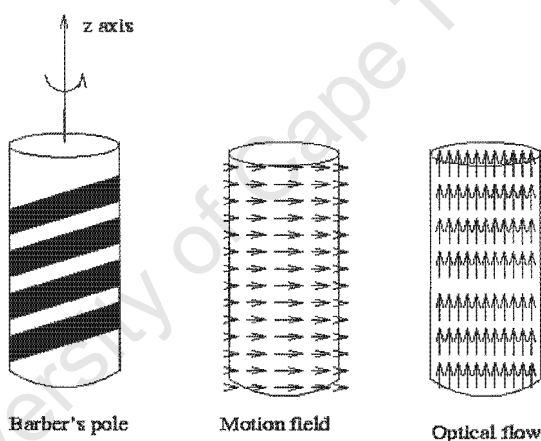
Figure 5.1: Illustration of the difference between optical flow and motion field [55]
