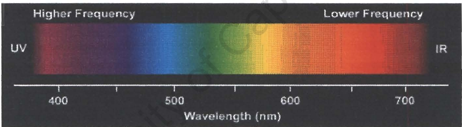
Figure 3.1: The spectrum of visible light [85]
