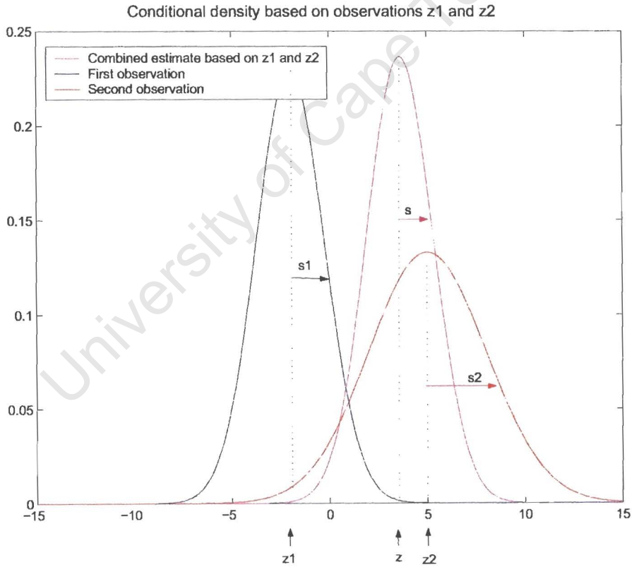
Figure 5.4: Conditional density with variance s (corresponding to \sigma in the text) of a one-dimensional measurement based on observations z_1 and z_2 with variances s_1 and s_2 .
