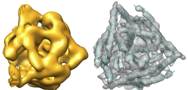
FIG 8 Comparison of VP5 from the AHSV-7 tVP2 empty-particle reconstruction and from a BTV-1 reconstruction (72). The VP5 densities were segmented from their respective reconstructions in Chimera (54). The AHSV-7 tVP2 protein is shown as a gold isosurface, and the BTV protein is shown as a gray transparent solid (EMDB accession code 5147), with blue wire showing the C-α backbone of VP5 (PDB accession code 3IYK).
