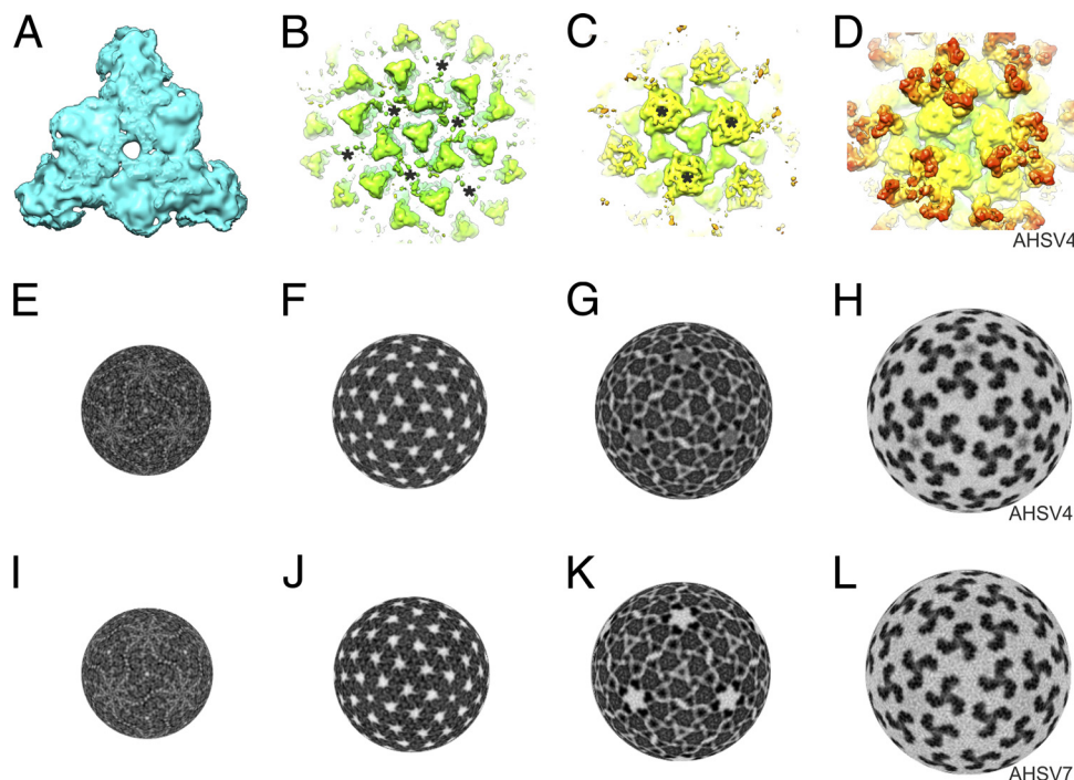
FIG 5 Comparison of protein layers within the structures of AHSV-4 and AHSV-7 tVP2, looking down a 3-fold axis of symmetry. (A) Three molecules of VP3 from AHSV-7 tVP2 are shown at a threshold of 1\sigma above the mean. The density was cut out using a 12-Å zone radius around the homology model of a VP3 trimer fitted into the density in Chimera (54). (B) AHSV-4 shown at a threshold of 3.2\sigma above the mean so that the organization of the green VP7 trimers is evident. (C) AHSV-4 shown at a threshold of 2.5\sigma above the mean so that the organization of VP7 with the intervening VP5 trimers (yellow) sitting on the quasi-6-fold axes of symmetry (indicated with black asterisks in panels B and C) is evident. (D) AHSV-4 shown at a threshold of 1\sigma above the mean so that the organization of VP2 (red) is evident. (E to L) Radial shells of the AHSV-4 and AHSV-7 tVP2 reconstructions. Proteins are black. (E to H) AHSV-4; (I to L) AHSV-7 tVP2. (E and I) VP3 layer at 26.2-nm radius; (F and J) VP7 trimers visible at 29.4-nm radius; (G and K) VP5 trimers visible at 35.3-nm radius, where the additional density plugging the 5-fold vertices in AHSV-4 is obvious compared to the case in AHSV-7 tVP2, which has holes on the 5-fold vertices; (H and L) VP2 triskelions at 38.9-nm radius.
