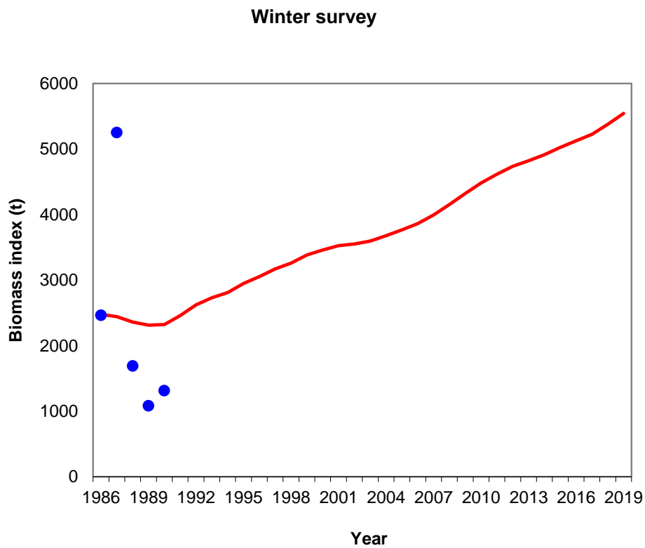
Figure 2. Observed (dots for the old gear, triangles for the new gear and diamonds for the industry vessel) and model estimated (line) trend of Africana survey abundance indices fitted to data for the period 1986 to 2019 for the kingklip off the West coast of South Africa.
