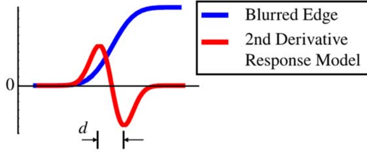
Fig. 46 Model for distance between second-derivative extrema [60]
