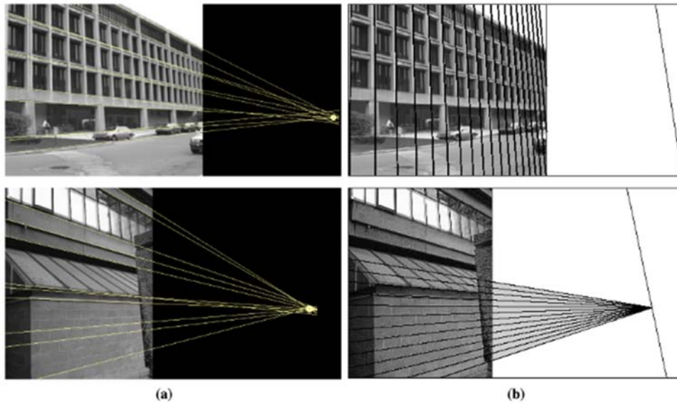
Fig. 72 Training set 2. (a) Results of proposed method. (b) Results from Schaffalitzky and Zisserman [59].
