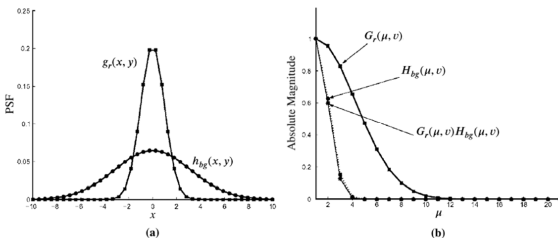
Fig. 44 Gaussian Blur [42]. (a) Two PSF with different blur parameters ( \sigma_{hbg} = 3.16 and \sigma_{gr} = 1 ). (b) Corresponding Fourier transforms.
