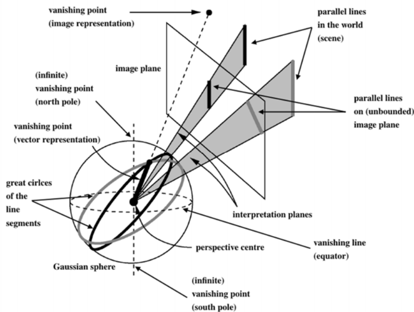
Fig. 64 Gaussian-sphere as an accumulator space [154].
