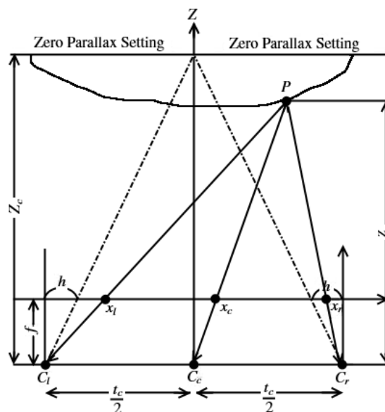
Fig. 80 Camera configuration for rendering of virtual stereoscopic images [48].
