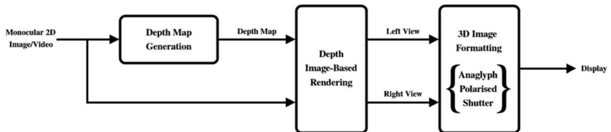
Fig. 4 Overview of the 2D-to-3D Conversion Process [37].
