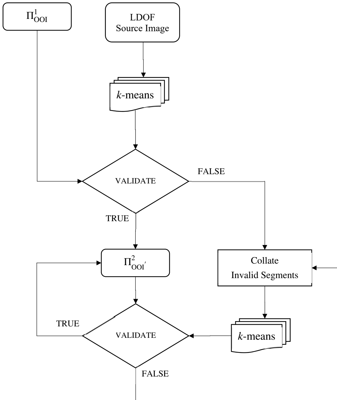
Fig. 30 OOI Matting: Stage 2a.
