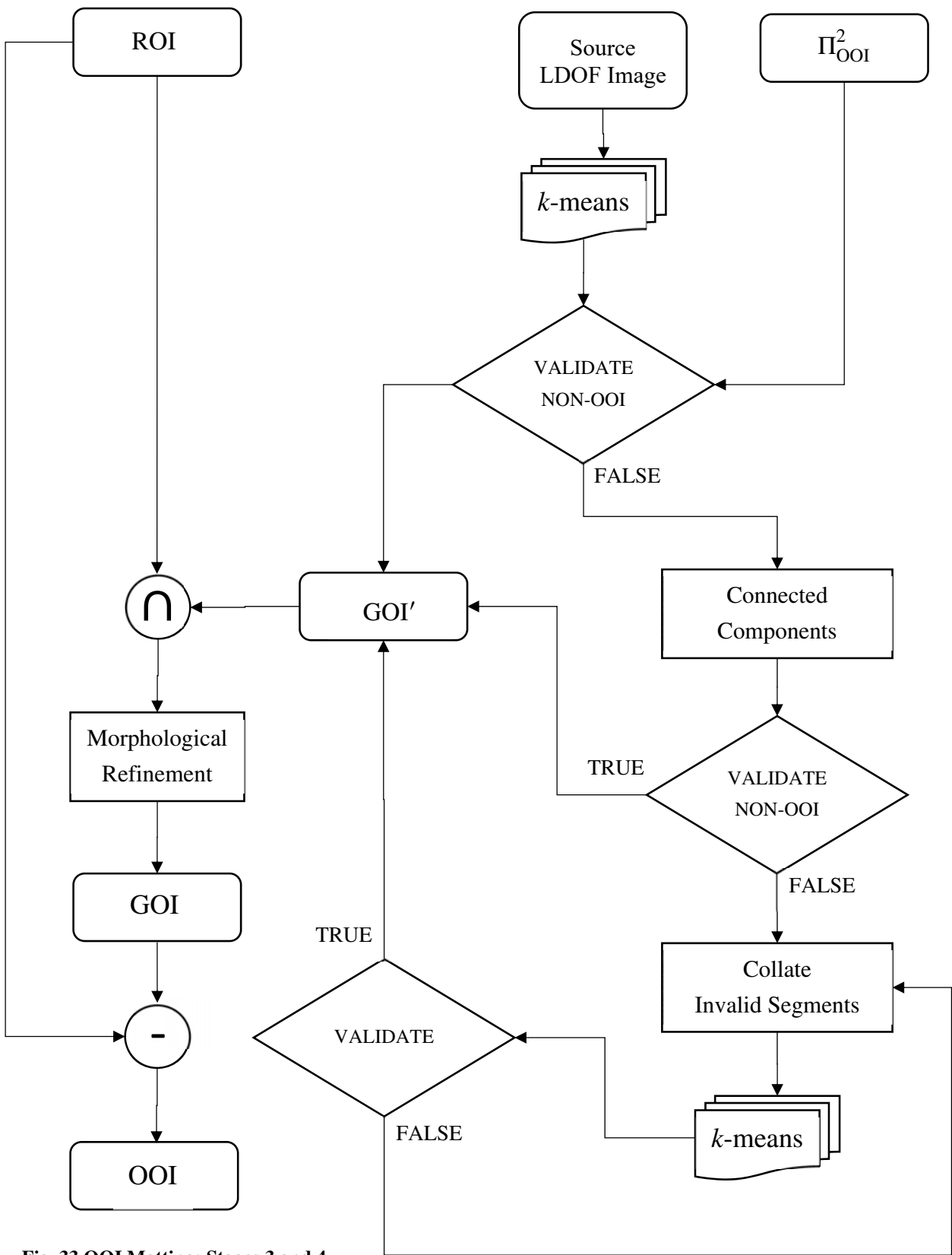
Fig. 33 OOI Matting: Stages 3 and 4.
