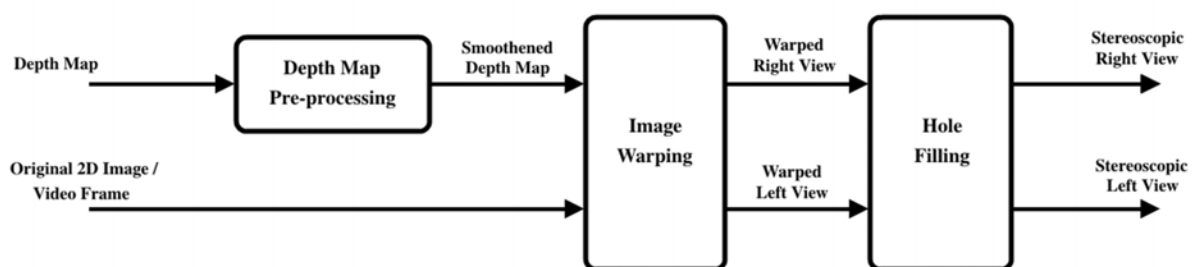
Fig. 79 Depth image-based rendering (DIBR) System (Image adapted from [47])
