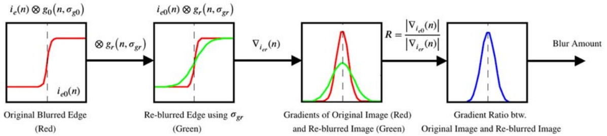
Fig. 45 Blur Estimation (Image adapted from [63]).
