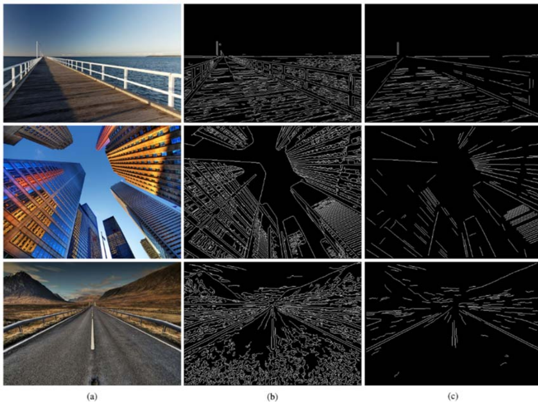
Fig. 67 Detection of straight line edges. (a) Original images; (b) Full edge maps; (c) Straight line segments.
