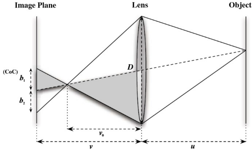
Fig. 43 Geometry of (real) finite-aperture imaging system [121]
