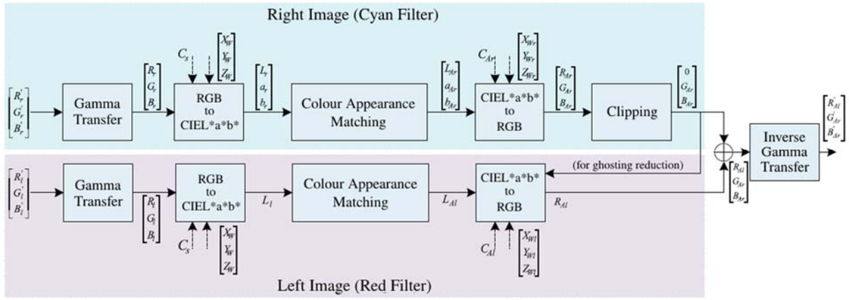
Fig. 100 Colour Appearance Attributes CIEL*a*b* Anaglyph Method [50]
