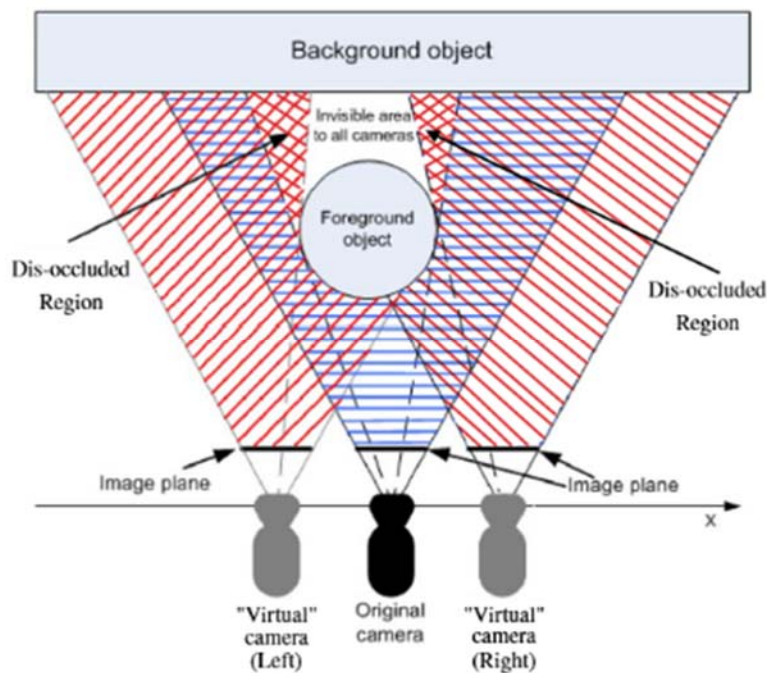
Fig. 78 Extrapolation scenario of virtual cameras views from original camera (Image adapted from [165])
