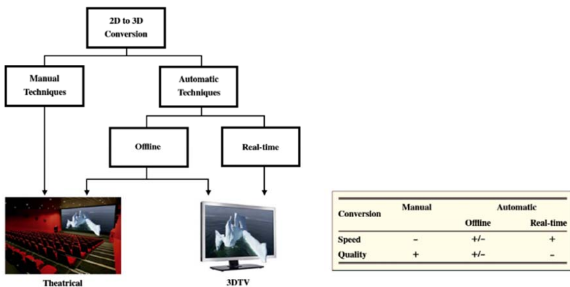
Fig. 3 Overview of the 2D-to-3D conversion approaches with comparison of trade-offs [32].
