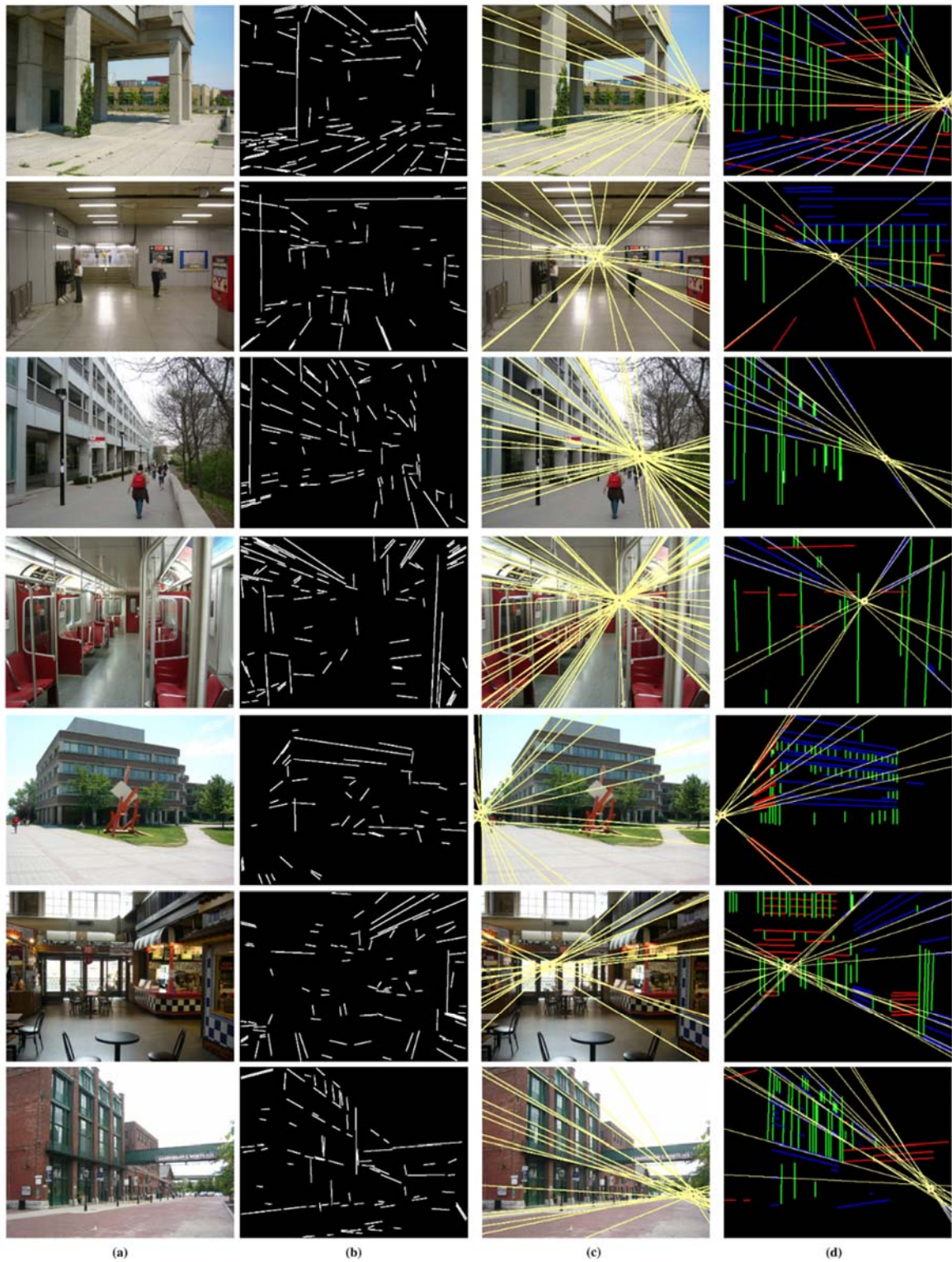
Fig. 77 York urban database. (a) Original image; (b) Refined straight edges extracted using the proposed method; (c) Results of proposed method; (d) Results of proposed method applied to the respective York urban ground-truth.
