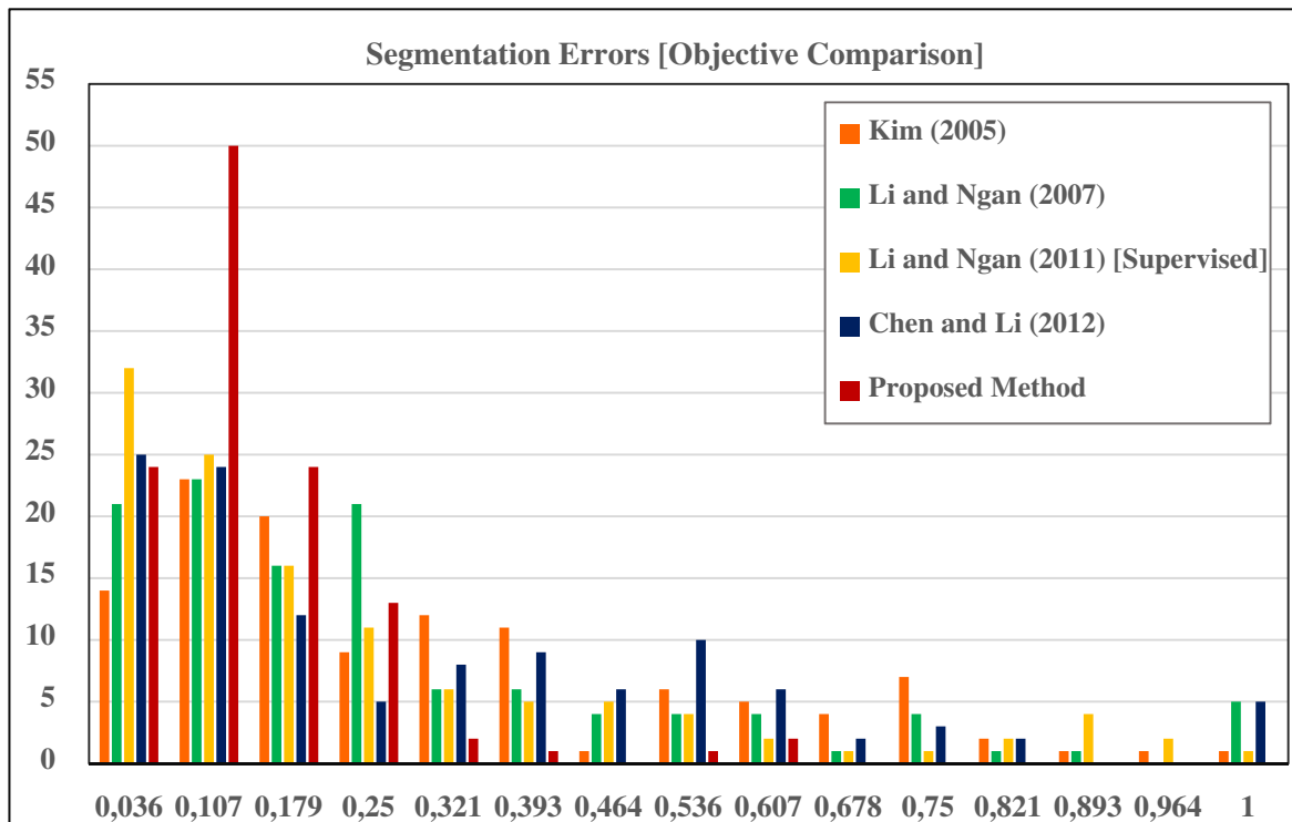
Fig. 20 Objective comparison. Segmentation errors of the 117 test images for Kim (2005) [41], Li and Ngan (2007) [42], Li and Ngan (2011) – supervised approach [52], Chen and Li (2012) [51] and the proposed method.
