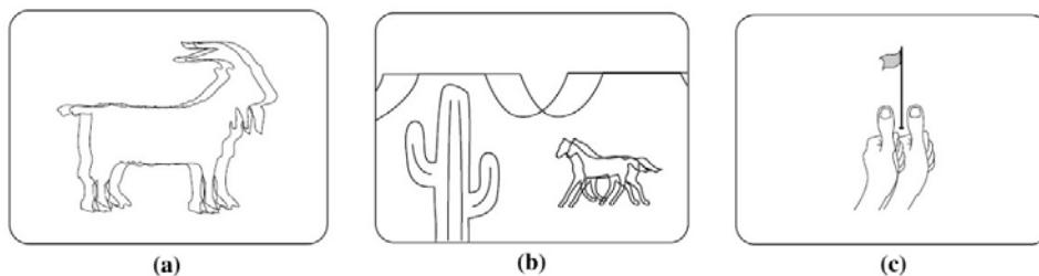
Fig. 1 Stereopsis [10]. (a) Retinal disparity. Overlaid left and right retinal images; (b) Focus on cactus in front. Positive parallax. Horse and mesas will appear blurry; (c) Focus on flag in distance. Negative parallax. Thumbs will appear blurry. In the case of (b) and (c), should focus be maintained and only one eye kept open, the parallax will be negated; however, the defocus will remain.
