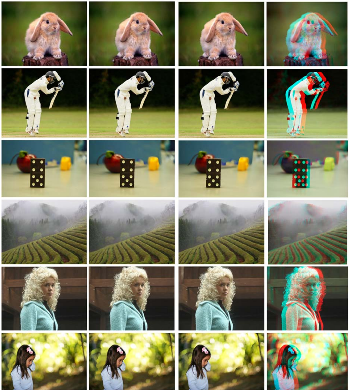
Fig. 102 3D images of test data – Set 3. The original images, synthesised left and right disparity images and associated 3D anaglyph interpretations are presented.
