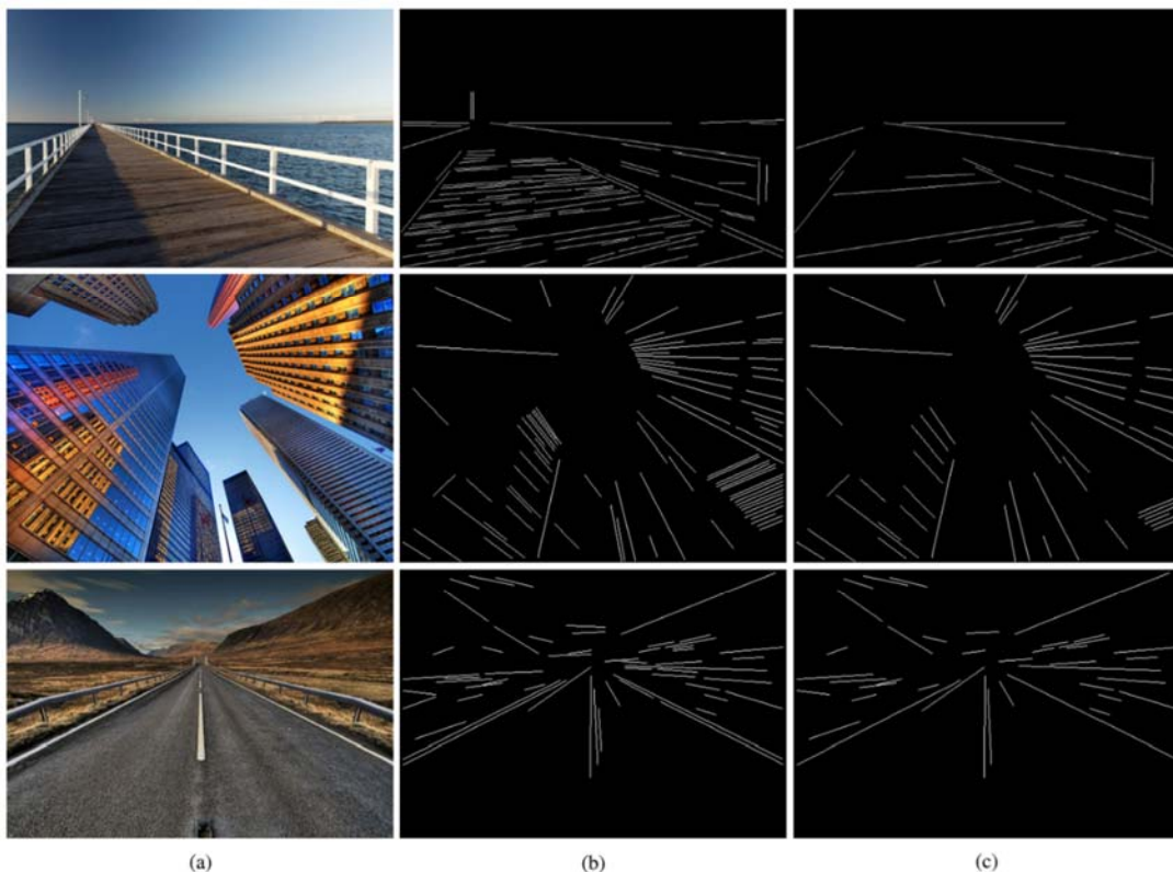
Fig. 68 Digital straight lines. (a) Original images; (b) Digital straightened segments; (c) Refined digital straight lines.
