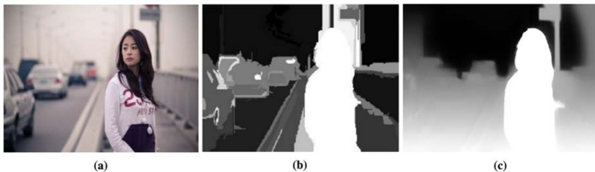
Fig. 59 Subjective comparison 2. (a) Original image; (b) Depth map generated by Ko et. al [65]; (c) Depth map generated using proposed method.
