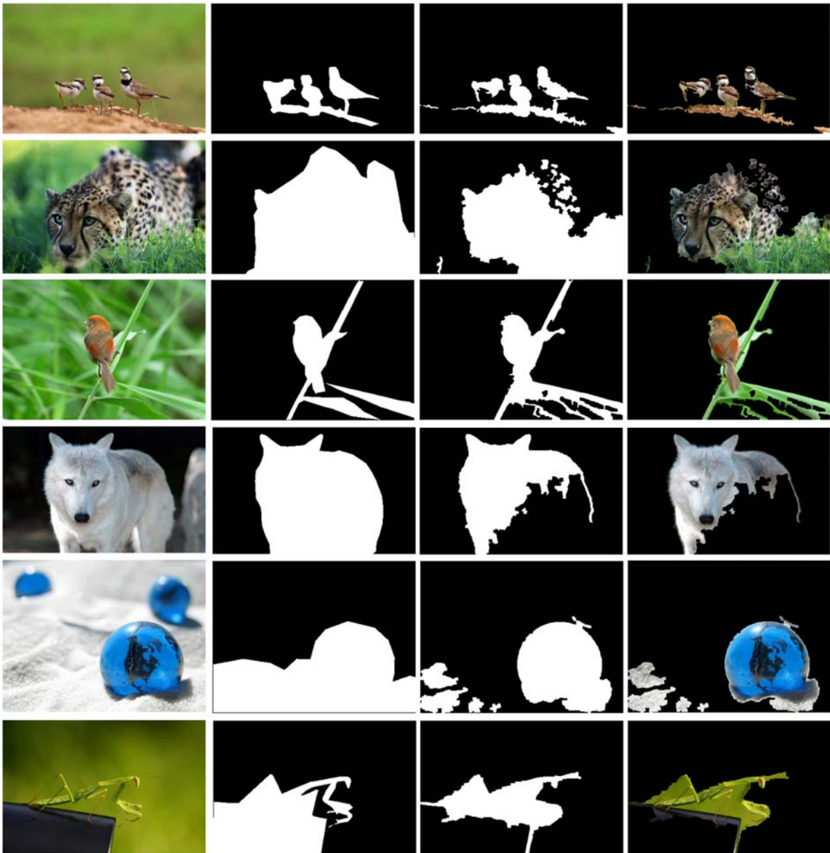
Fig. 23 Segmentation results from the 117 test images with error greater than 0.25: Three-Birds, Crouching-Cheetah, Bird-Reed, Albino-Wolf, Marbles and Mantis (from top to bottom).
