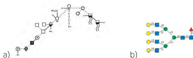
Figure 4.1: Complex carbohydrates are the largest group of biomolecules on earth and structural schematics are represented by the a) Oxford symbol nomenclature [65] and the b) CFG system [64].
