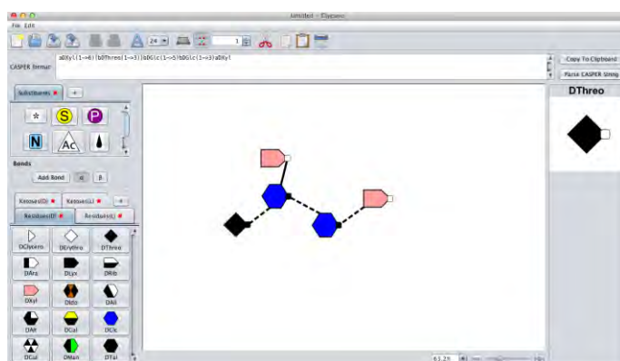
Figure 4.3: The Glycano UI of the Java based software installed on a PC.
