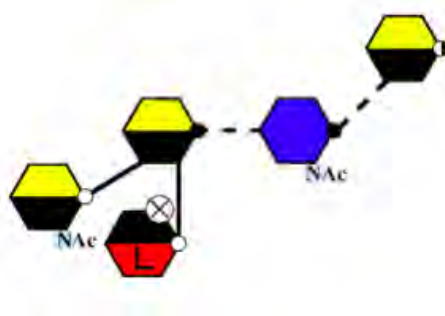
Figure 4.2: An example of a carbohydrate representations in Glycano. Solid black lines joining residues represents \alpha bonds and the dotted lines represent \beta bonds.
