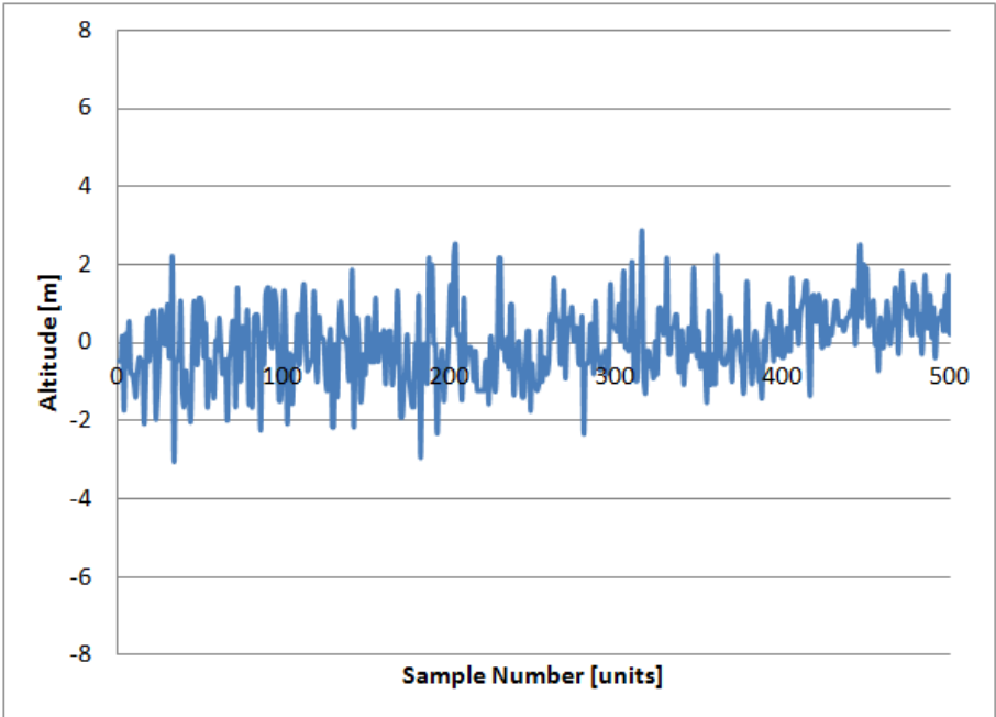
Figure 7.2: Figure showing unfiltered altitude readings from the Bosch BMP085 pressure sensor under steady state conditions.
