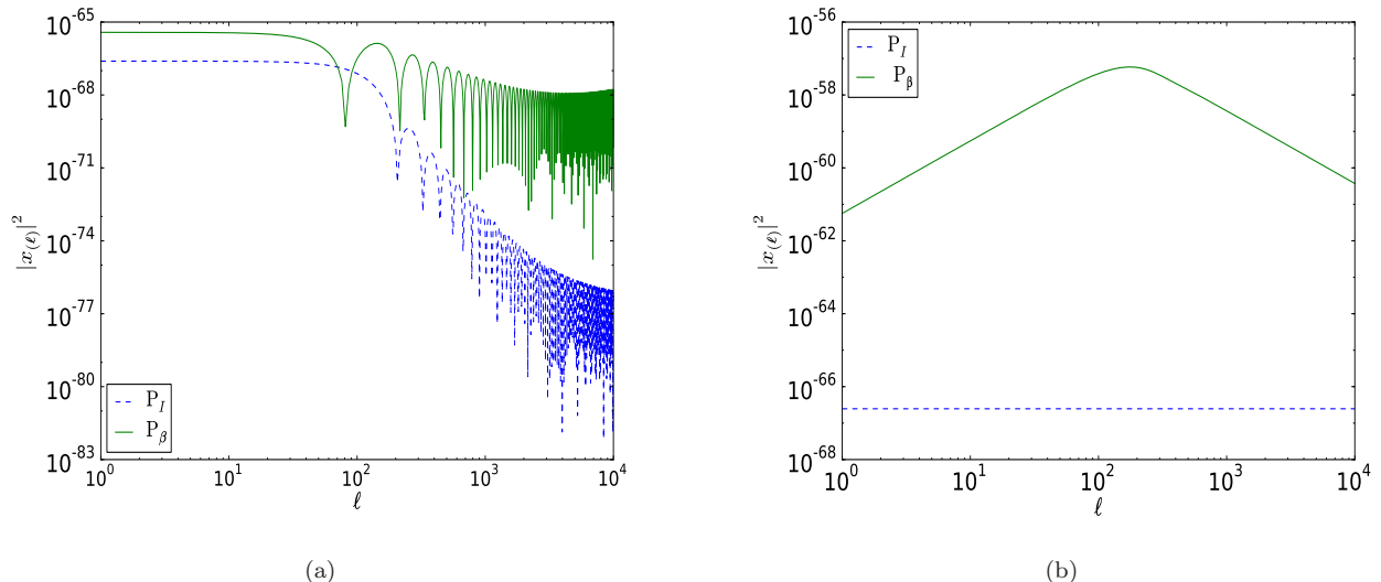
FIG. 2: Plots of Power vs scale ( \ell ); we define the power as P_x = |x(\ell)|^2 . (a): Power spectra of the magnetic field variable \beta_{(\ell)} (green, solid), and the interaction variable I_{(\ell)} (blue, dashed) at redshift z = 0 for the tensor case. (b): Power spectra of the magnetic field variable \beta_{(\ell)} (green, solid), and the interaction variable I_{(\ell)} (blue, dashed) at redshift z = 0 for the scalar case.
