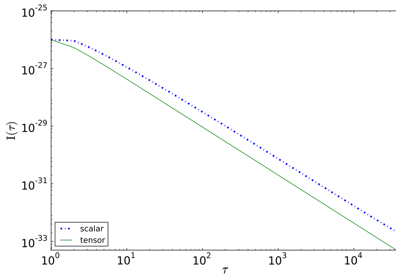
FIG. 1: Time evolution of the interaction variable in log-log axes. Note that for the interaction with scalars, the decay is slightly slower than for tensors.
