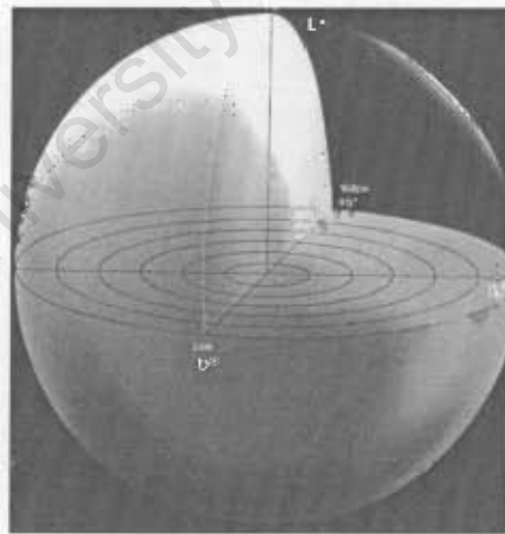
Figure 2.8: CIE L^*a^*b^* colour sphere.
