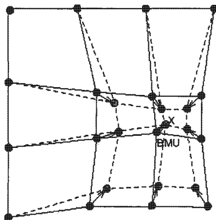
Figure A.1: Updating the Best Matching Unit (BMU) and its neighbours for input vector \mathbf{x} [43].
