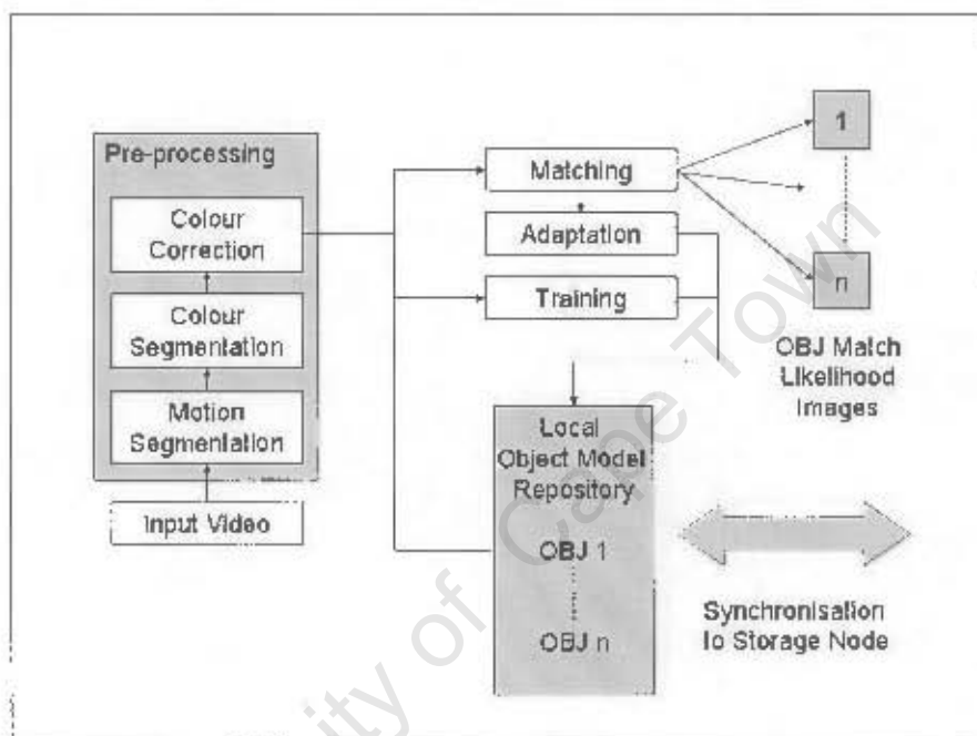
Figure 3.4: Processing Node Data Flow Diagram.
