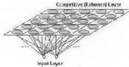
Figure 2.9: Structure of a Self-Organising Map (SOM).
