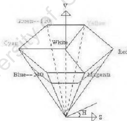
Figure 2.4: HSV hexcone.
