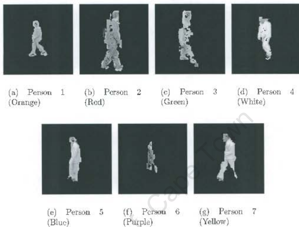
Figure 8.16: Training Set
