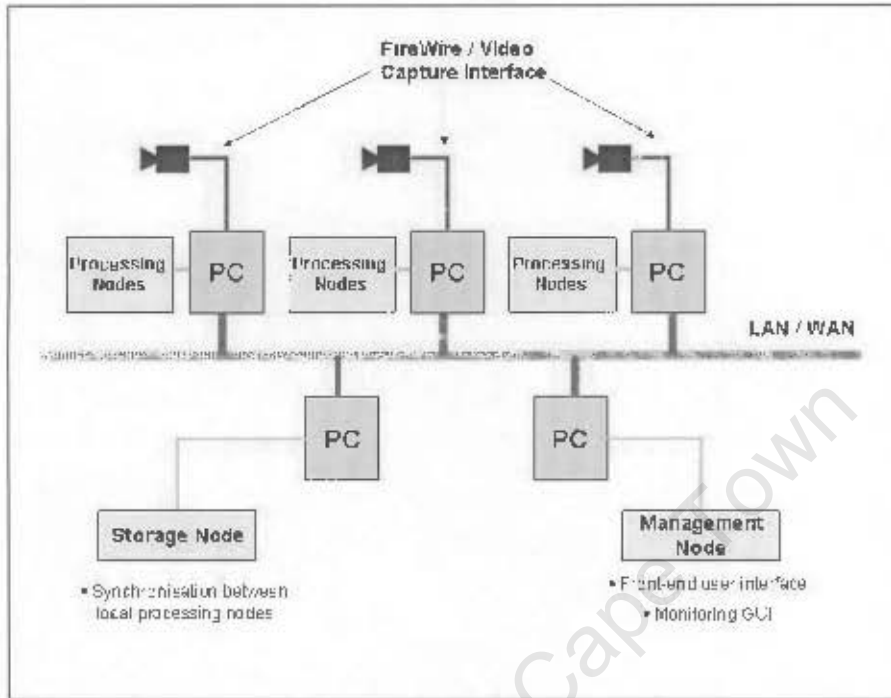
Figure 3.3: Distributed Framework.
