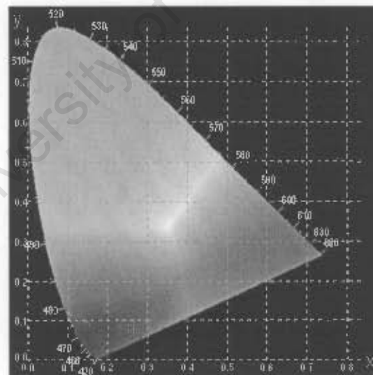
Figure 2.7: CIE chromaticity diagram.
