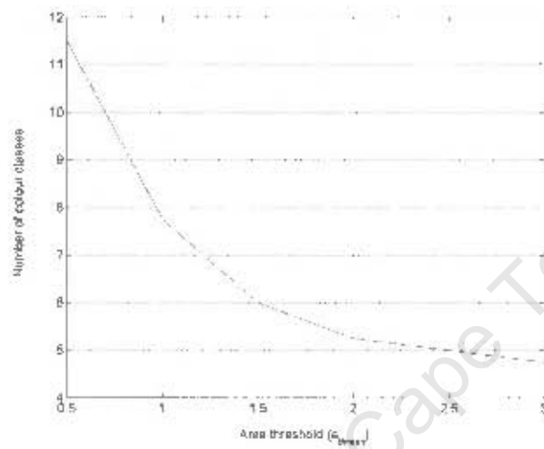
Figure 8.5: Tuning of area threshold. A value of a_{thresh} = 2.5 provides a reasonable estimate to the ideal value for the cartoon characters.
