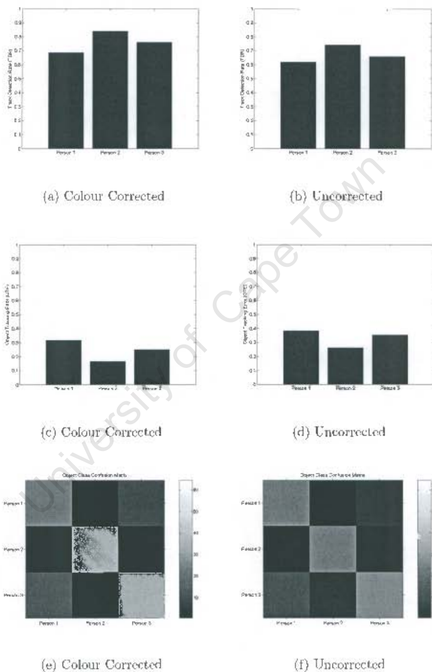
Figure 8.22: (a),(b) Track Detection Rate (TDR); (c),(d) Object Tracking Error (OTE) (e),(f) Object Model Confusion Matrix.
