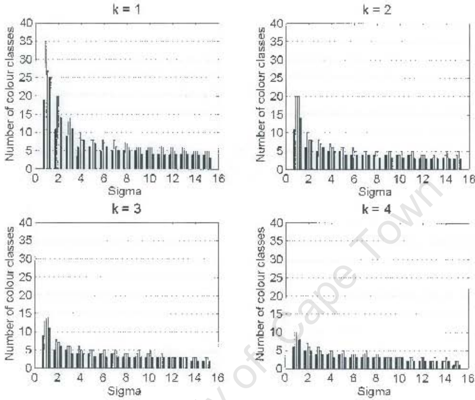
Figure 8.3: Tuning training parameters. Each graph shows the results for k_{train} = 1 to 4. The number of trained colour classes per character is shown by the vertical bars and is evaluated for \sigma_{train} from 1 to 15.
