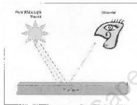
Figure 2.1: Surface colour example.
