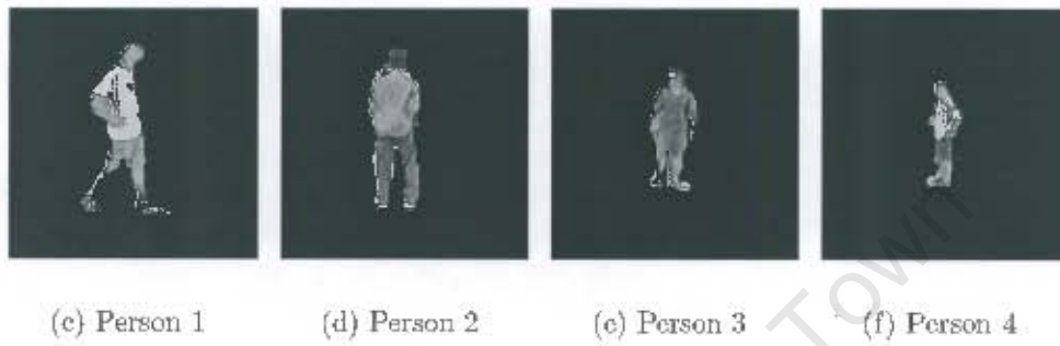
Figure 8.11: Training Set
