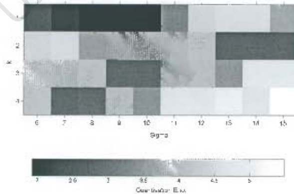
Figure 8.4: Quantisation error between trained classes and actual pixel data versus the \sigma_{train} and k_{train} parameters.
