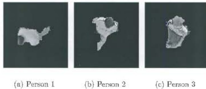
Figure 8.20: Training Set
