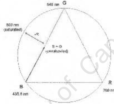
Figure 2.5: Matching 500 nm wavelength using Newton's colour circle.
