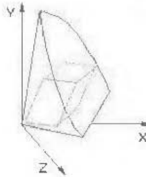
Figure 2.6: CIE Colour Space w.r.t. RGB cube.
