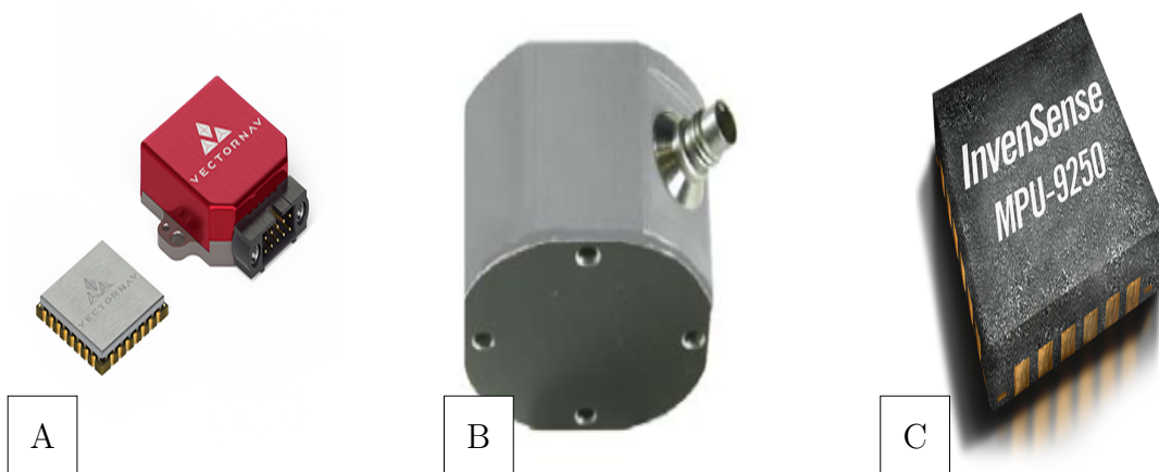
Figure 2.10: Diagram showing examples of the different types of inertial measurement systems (IMUs) available for commercial use such as (A) an Attitude Heading Reference System (AHRS) VN100 (VECTORNAV, 2019) used by (Rabault et al., 2019), (B) an analog capacitive accelerometer 8330B3 Servo-KBeam accelerometer used by (Kohout et al., 2015) (Kistler, 2011) and (C) a 9 degree of freedom MPU9250 (TDK InvenSense, 2016) used by (Kohout et al., 2015).
