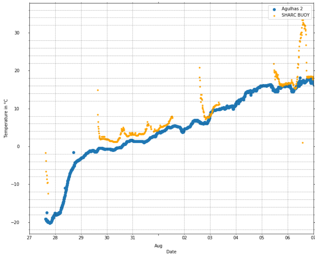
Graph Showing Air Temperature Recorded By SHARC BUOY VS. Air Temperature Recorded By The 'Agulhas 2' From 27 July 2019 - 07 August 2019
