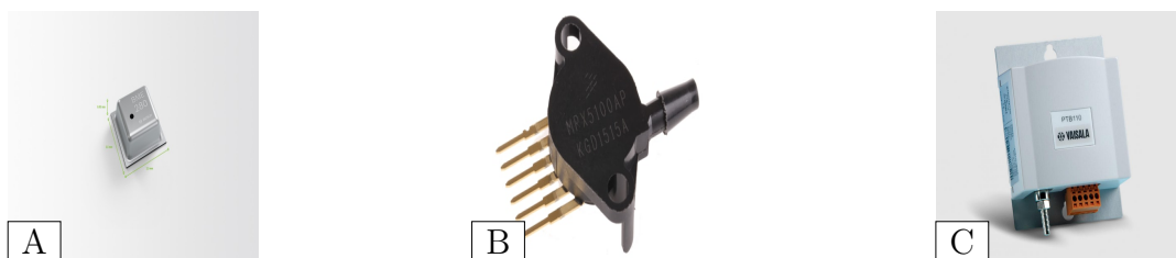
Figure 2.14: Examples of pressure sensing technologies using a diaphragm based MEMS with different methods of measuring the strain. These are piezoresistive sensors: (A) the BME280 (image source: (Bosch Sensortec, 2021)), (B) the MPX-5100-AP (image source: (RS Components, 2021)) or capacitive sensors: (C) the PTB100 (image source: (Vaisala, 2018))
