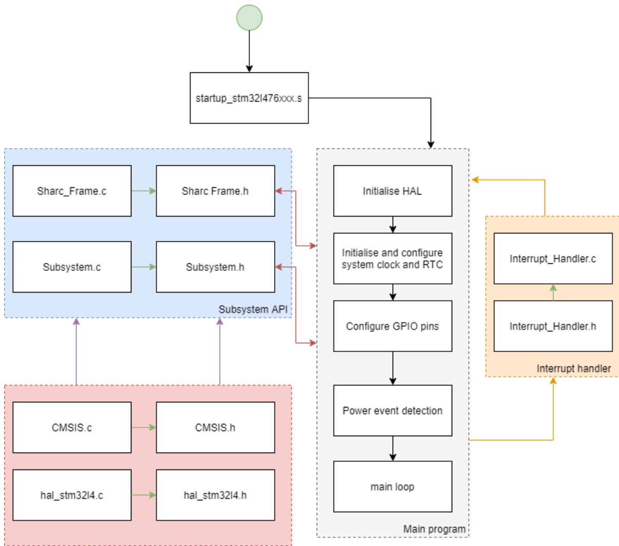
Figure 5.3: Diagram showing the firmware execution from (green) start. On start up, the startup_stm321476xxx.s file executes and loads the main program. This program runs in a continuous loop until the power supply to the device is turned off. This diagram shows the interaction of the firmware layers (see Figure 5.2): (blue) subsystem API, (red) HAL and (grey) the main program. Also shown are arrows indicating (black) the main flow of the program, (green) references to functions, (red) calls to function prototypes and (orange) interrupts.
