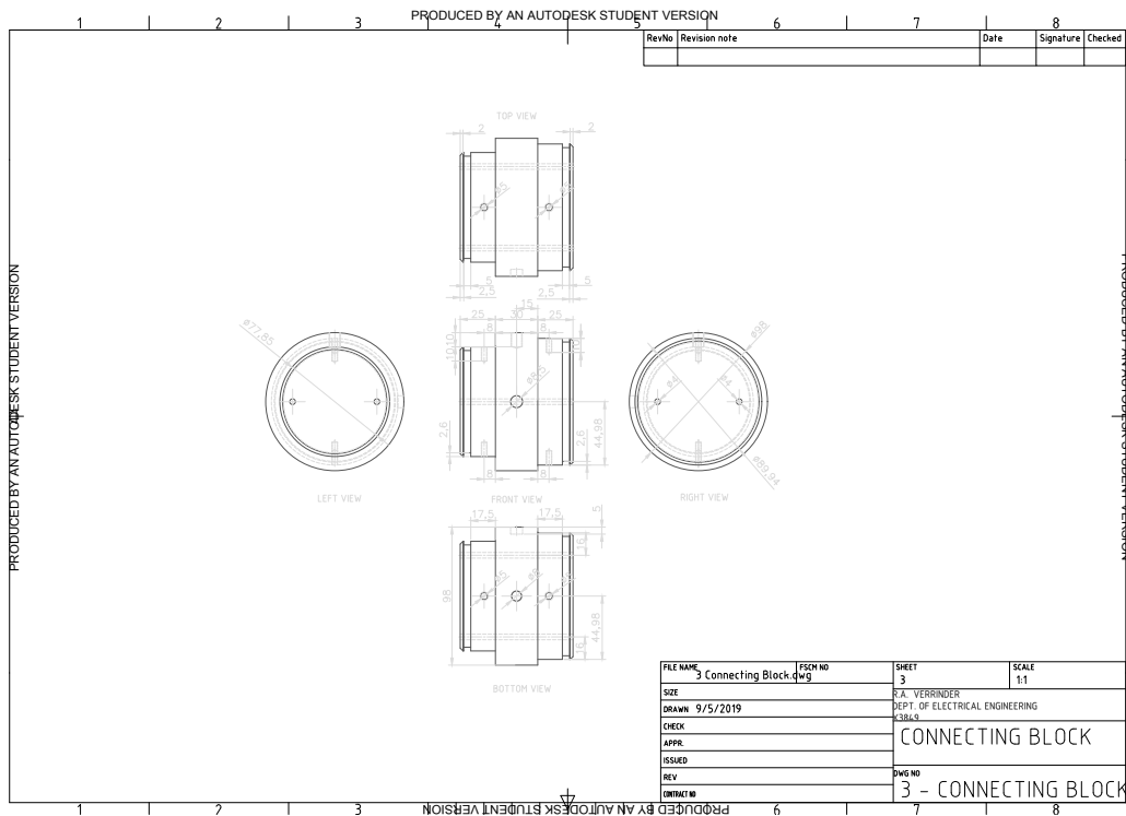
Figure B.3: Schematic of the connector block which provides a base for the electronics to be mounted on.
