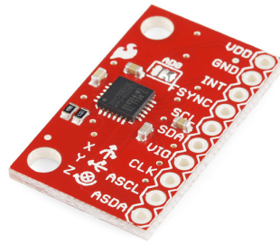
Figure 4.7: A TDK Invensense MPU6050 6 degrees of freedom inertial measurement unit on a Sparkfun development board. The board allows for fast prototyping with communication performed via I 2 C. Image source: (Sparkfun, 2021).
