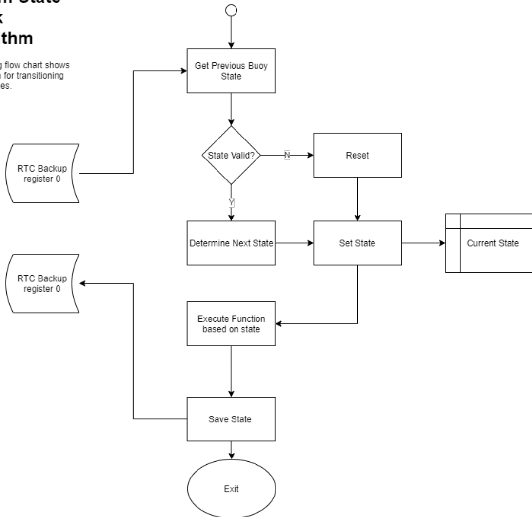
Figure 5.8: Flow chart for the state-check algorithm
