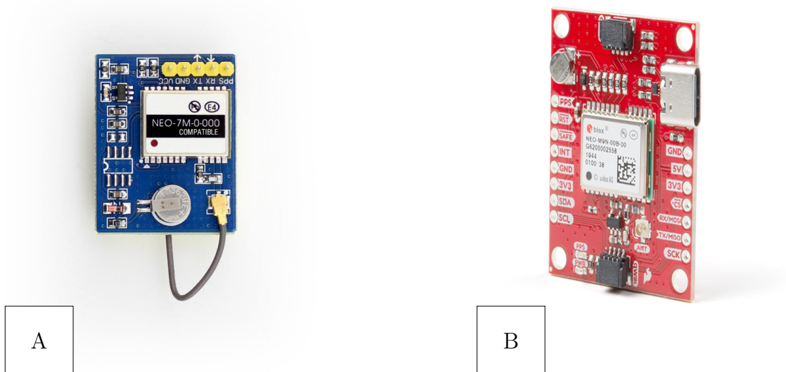
Figure 4.3: The u-blox GPS Modules selected for this project which are: (A) the u-blox NEO-7M on a Waveshare breakout board (Waveshare, 2016) and (B) a u-blox NEO-M9N on a Sparkfun breakout board (u-blox, 2020).
