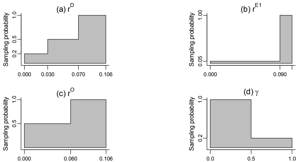
Fig. 3. Importance functions used when sampling the r^D , r^{E1} , r^O and \gamma parameters. The horizontal axis shows the step values at which the importance function increases, and the vertical axis shows the probability of accepting a sample from a particular range. Note that that the importance functions for r^D and r^{E1} were implemented for both the base case model and the original model. Importance functions for r^O and \gamma were implemented for the base case model only.
