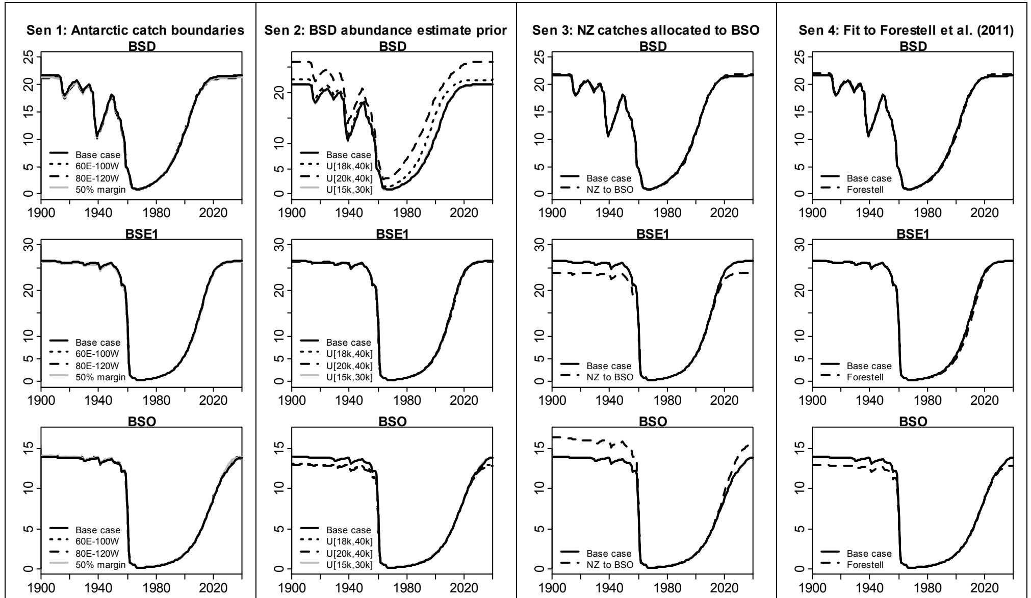
Fig. 6: Median population ‘trajectories’ for each of the four sensitivity runs (note that strictly these are not actual trajectories, but juxtaposition of successive values form posterior probability distributions for each year). For each plot, the solid line corresponds to the base case run.
