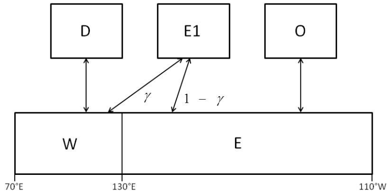
Fig. 3. Diagrammatic representation of the alternative three-stock model developed by the sub-committee.
