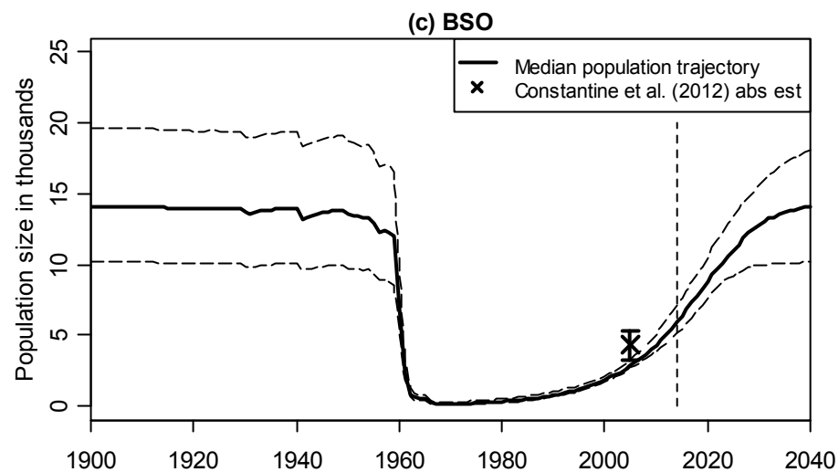
Fig. 5: Figures (a)-(c) show the median population trajectories for the base case three-stock model. 90% probability envelopes are indicated by the dashed lines. The model is fit to the Bannister and Hedley (2001) and the Hedley et al. (2011) relative abundance series for BSD (fits shown in Figure (a)); the Noad et al. (2011) absolute and relative abundance series for BSE1 (fits shown in Figure (b)), and to the Constantine et al. (2012) mark-recapture data for BSO (Figure (c)). In Figure (c), the cumulative observed re-sightings are marked by X's. Fits to the Hedley et al. (2011) absolute abundance estimate (Figure (a)); the Chittleborough (1965) relative abundance series (Figure (a) and (b)); and the Constantine et al. (2012) absolute abundance estimate (Figure (c)) are shown as consistency checks.
