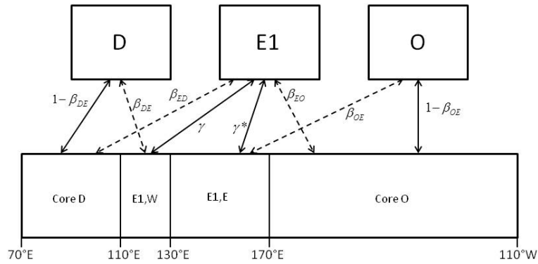
Fig. 2. Diagrammatic representation of the original three-stock model.
