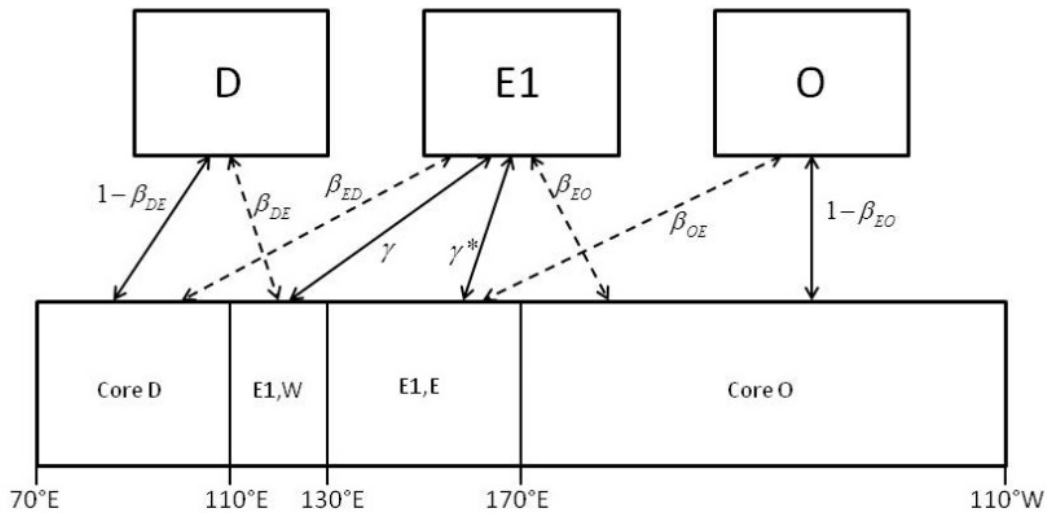
Fig. 2. Diagrammatic representation of the original three stock-model used in SC/65b/SH04addendum.
