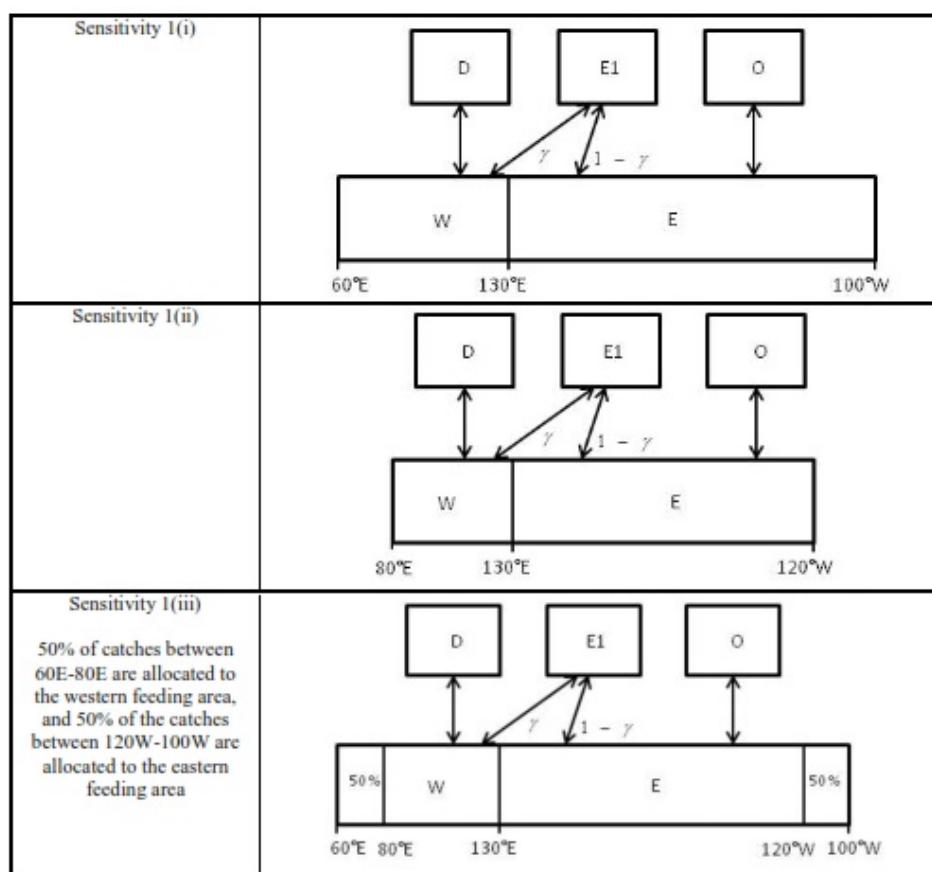
Fig. 3. Diagrammatic illustrations of the alternative Antarctic catch boundaries that were explored in the catch allocation sensitivity runs.
