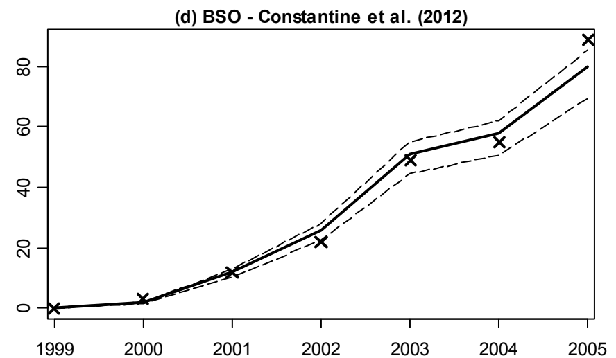
Fig. 5: Figures (a)-(c) show the median population trajectories for the base case three-stock model. 90% probability envelopes are indicated by the dashed lines. The model is fit to the Bannister and Hedley (2001) and the Hedley et al. (2011) relative abundance series for BSD (fits shown in Figure (a)); the Noad et al. (2011) absolute and relative abundance series for BSE1 (fits shown in Figure (b)), and to the Constantine et al. (2012) mark-recapture data for BSO (Figure (c)). In Figure (c), the cumulative observed re-sightings are marked by X's. Fits to the Hedley et al. (2011) absolute abundance estimate (Figure (a)); the Chittleborough (1965) relative abundance series (Figure (a) and (b)); and the Constantine et al. (2012) absolute abundance estimate (Figure (c)) are shown as consistency checks.
