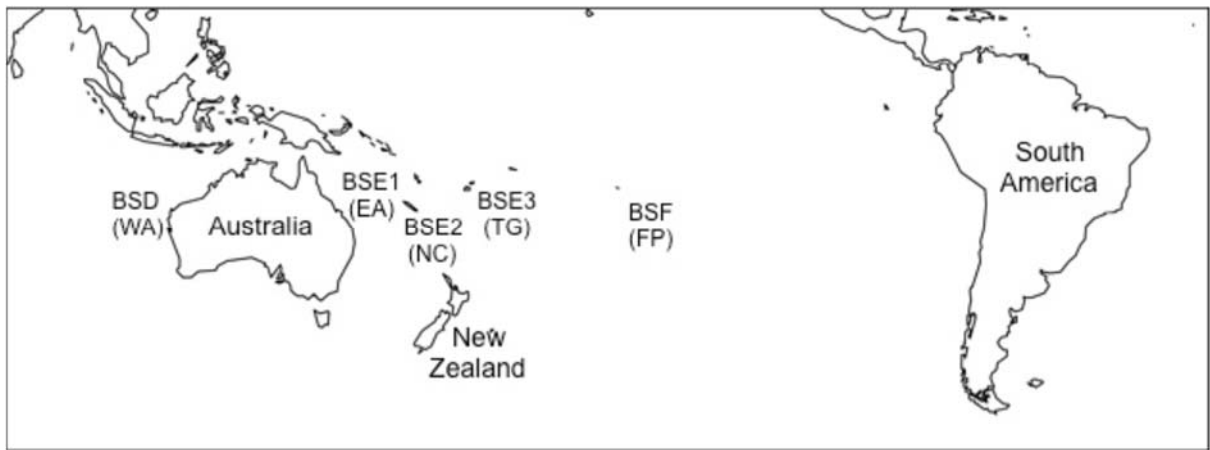
Fig. 1. Distribution of Southern Hemisphere humpback whales breeding stocks grounds BSD, BSE1, BSO (BSE2, BSE3 and BSF). Note the following abbreviations: WA = Western Australia, EA = Eastern Australia, NC = New Caledonia, TG = Tonga and FP = French Polynesia.
