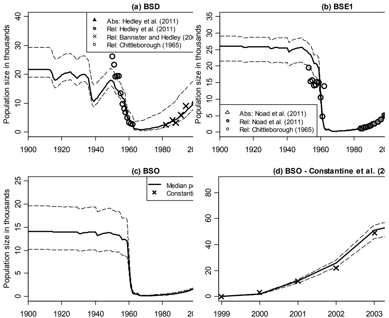
Fig. 4: (a)-(c) show the median population trajectories for the base case three-stock model. 90% probability envelopes are indicated by the dashed lines. The model is fit to the Bannister and Hedley (2001) and the Hedley et al. (2011) relative abundance series for BSD (fits shown in Fig. (a)); the Noad et al. (2011) absolute and relative abundance series for BSE1 (fits shown in Fig. (b)), and to the Constantine et al. (2012) mark-recapture data for BSO (Fig. (d)). In Fig. (d), the cumulative observed re-sightings are marked by X's. Fits to the Hedley et al. (2011) absolute abundance estimate (Figure (a)); the Chittleborough (1965) relative abundance series (Fig. (a) and (b)); and the Constantine et al. (2012) absolute abundance estimate (Fig. (c)) are shown as consistency checks.
