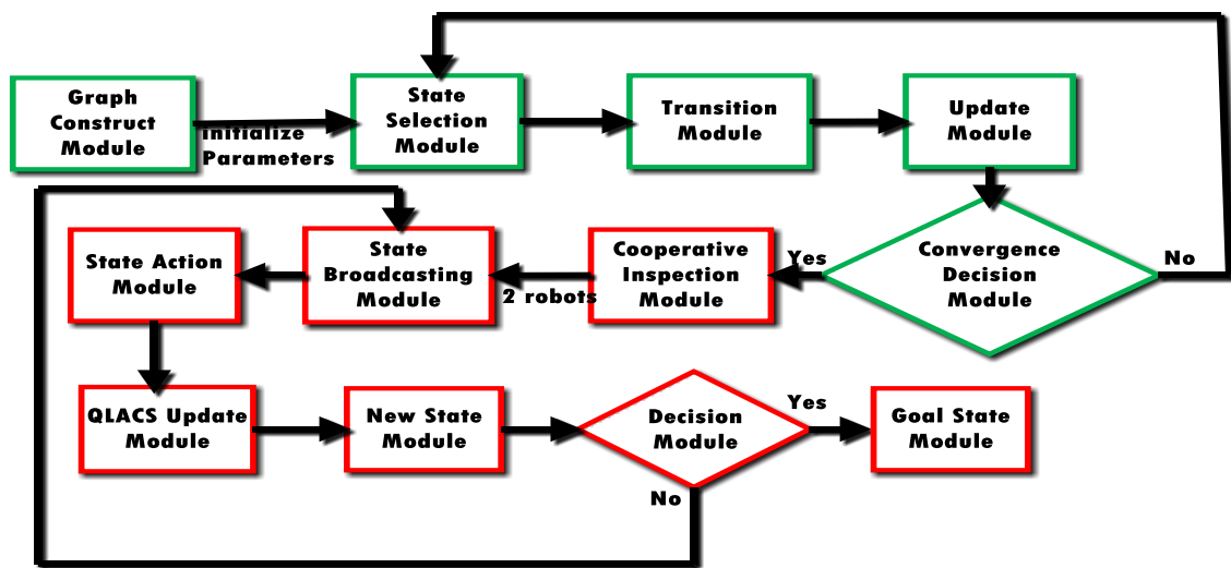
Figure 3.10: Hybrid Architecture
