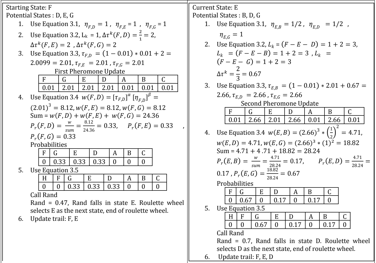
Figure 3.12: QLACS example I navigational analytical solution
