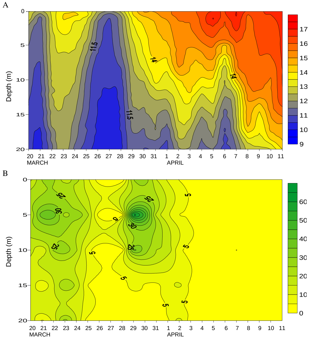
Figure 3.1: A daily time series of (A) temperature ( ^{\circ}\text{C} ) and (B) chlorophyll- a ( \text{mg.m}^{-3} ) at the mooring off Lambert's Bay from the 20 March - 11 April 2007. The contour maps were created using Surfer v8.01.
