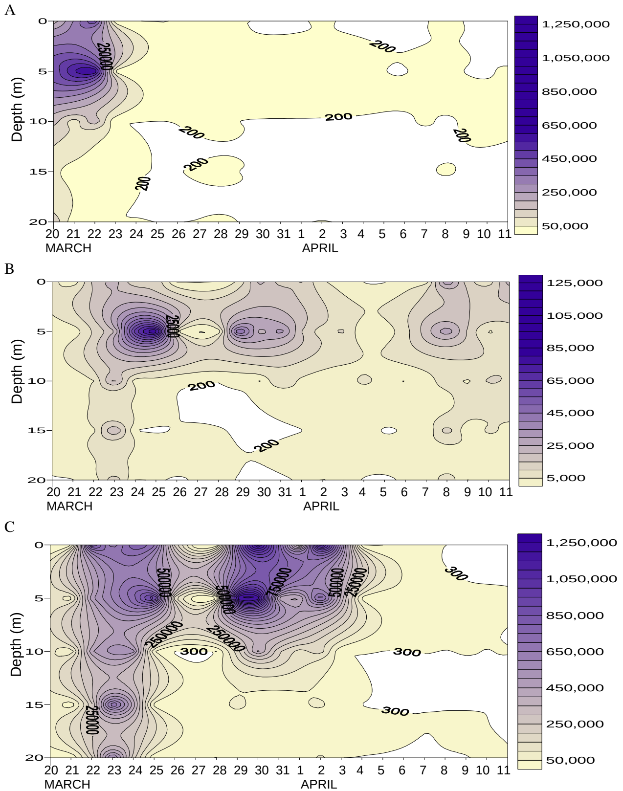
Figure 3.2: A daily time series of the toxic phytoplankton species (A) Alexandrium catenella , (B) Dinophysis spp., and (C) Pseudo-nitzschia spp., at the mooring off Lambert's Bay from 20 March - 11 April 2007. The contour maps were created using Surfer v8.01.
